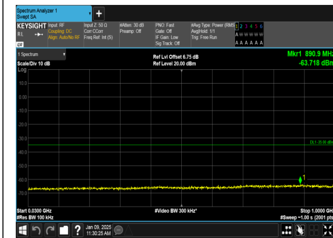
Band38-15MHz-16QAM-37825-1RB#74-30~1000-PASS
