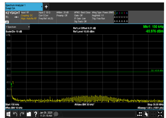
Band38-15MHz-QPSK-37825-75RB#0-0.15~30-PASS
