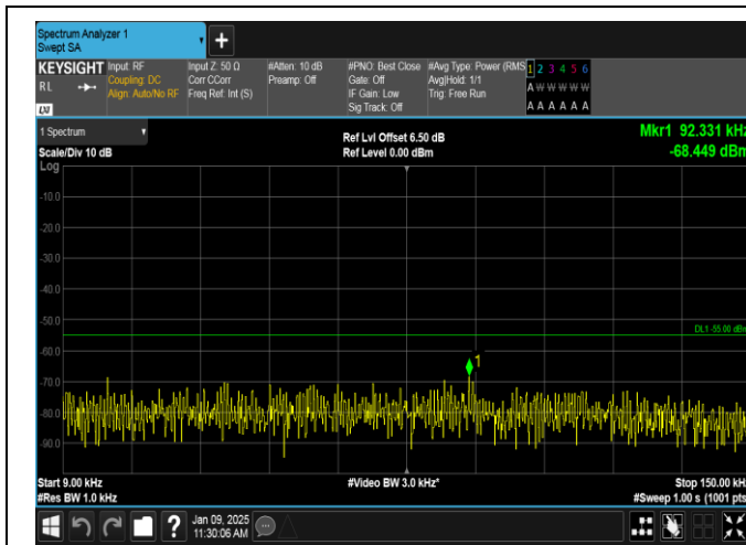
Band38-15MHz-16QAM-37825-1RB#74-0.009~0.15-PASS
