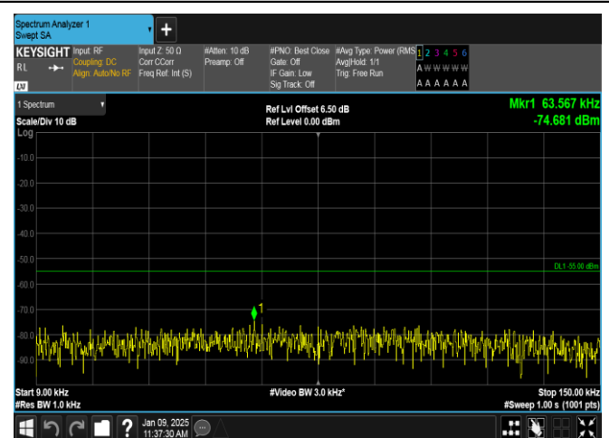
Band38-15MHz-QPSK-38000-75RB#0-0.009~0.15-PASS
