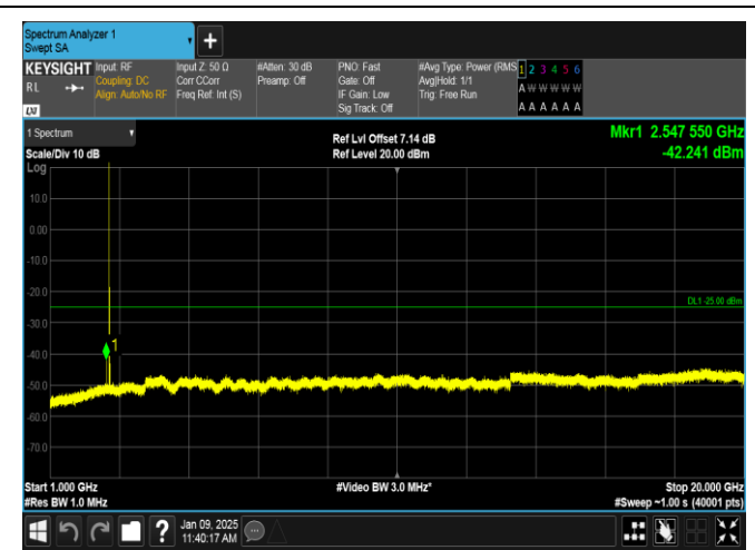
Band38-15MHz-QPSK-38175-1RB#0-1000~20000-PASS
