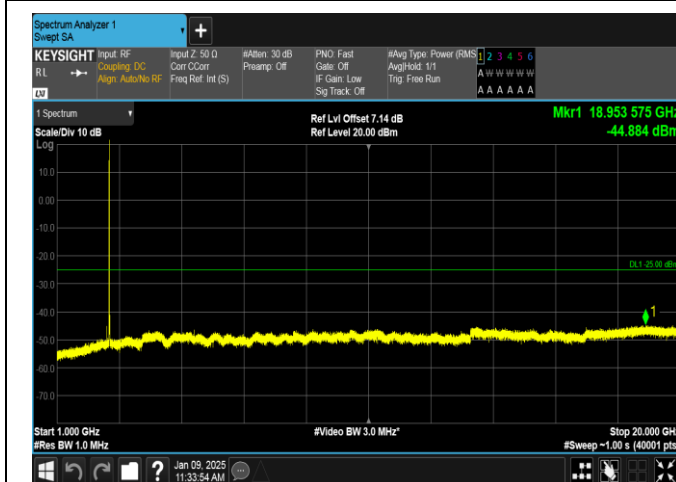
Band38-15MHz-QPSK-38000-1RB#0-1000~20000-PASS
