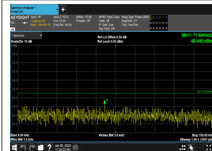
Band38-15MHz-16QAM-38000-1RB#0-0.009~0.15-PASS
