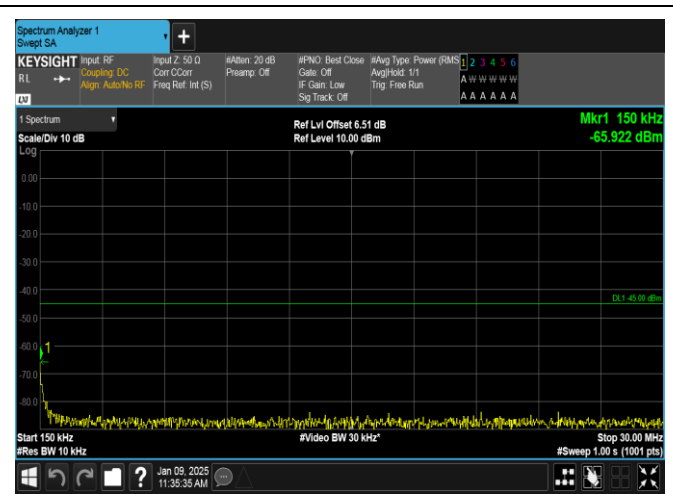
Band38-15MHz-QPSK-38000-1RB#74-0.15~30-PASS
