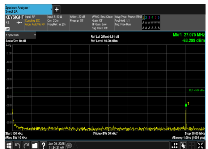
Band38-15MHz-16QAM-38000-1RB#0-0.15~30-PASS
