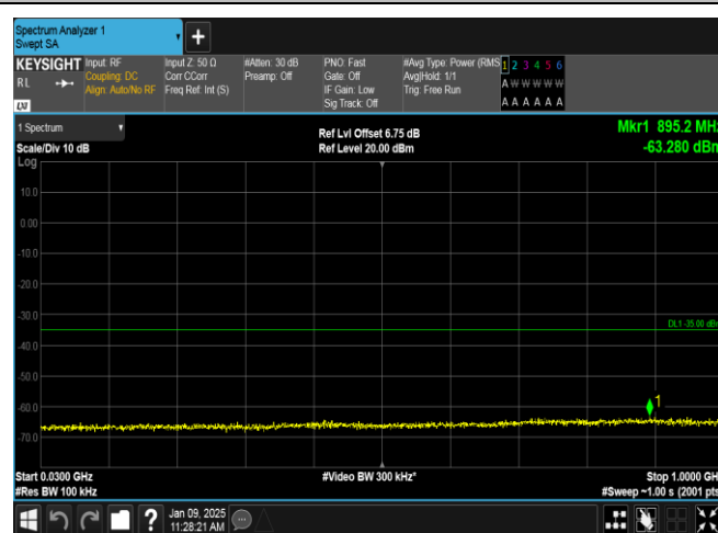
Band38-15MHz-16OAM-37825-1RB#0-30~1000-PASS
