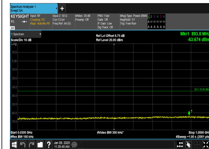
Band38-15MHz-QPSK-38000-1RB#74-30~1000-PASS
