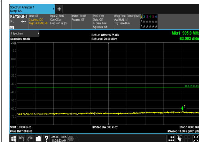
Band38-15MHz-16QAM-38000-75RB#0-30~1000-PASS
