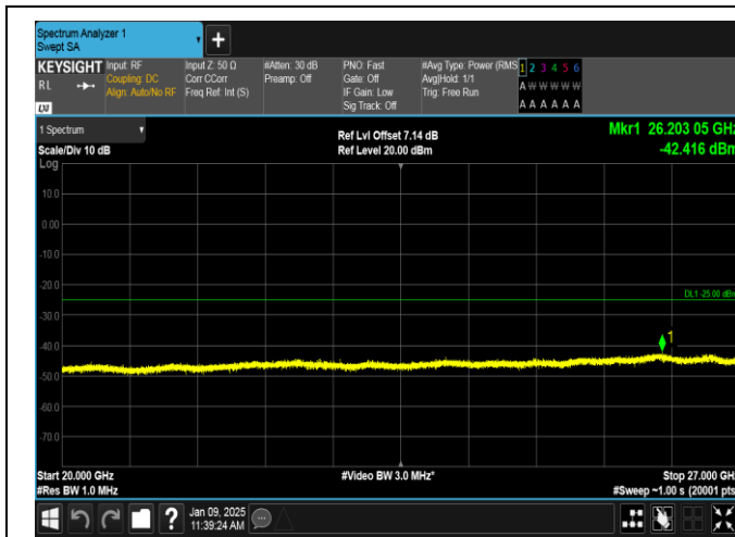
Band38-15MHz-16QAM-38000-75RB#0-20000~27000-PASS
