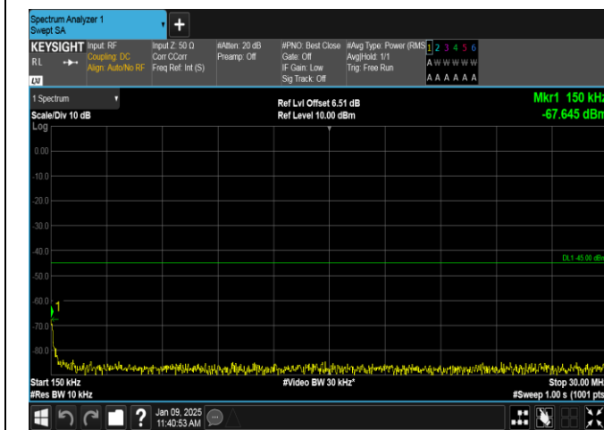
Band38-15MHz-16QAM-38175-1RB#0-0.15~30-PASS
