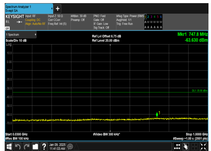
Band38-15MHz-16QAM-38175-1RB#0-30~1000-PASS
