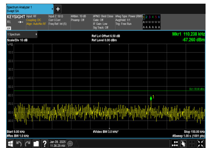
Band38-15MHz-16QAM-38000-1RB#74-0.009~0.15-PASS
