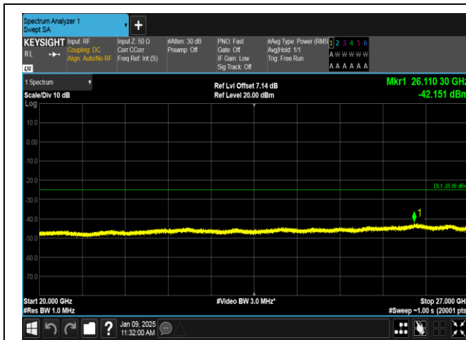
Band38-15MHz-QPSK-37825-75RB#0-20000~27000-PASS
