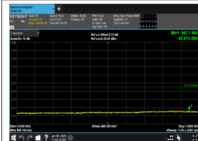
Band38-15MHz-QPSK-38175-75RB#0-30~1000-PASS
