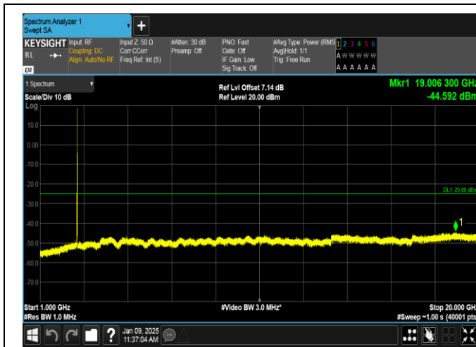
Band38-15MHz-16QAM-38000-1RB#74-1000~20000-PASS
