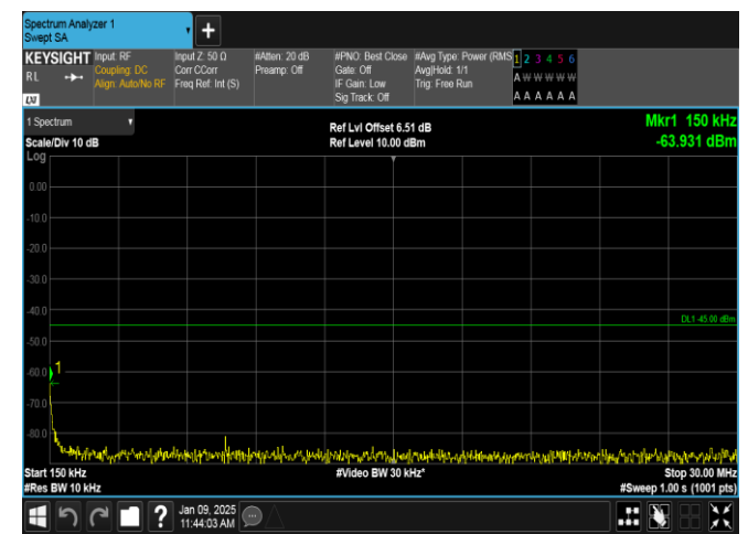
Band38-15MHz-QPSK-38175-75RB#0-0.15~30-PASS
