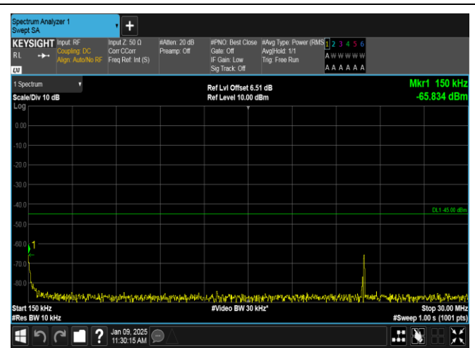
Band38-15MHz-16QAM-37825-1RB#74-0.15~30-PASS
