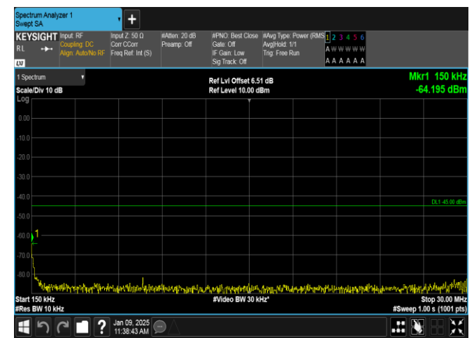
Band38-15MHz-16QAM-38000-75RB#0-0.15~30-PASS
