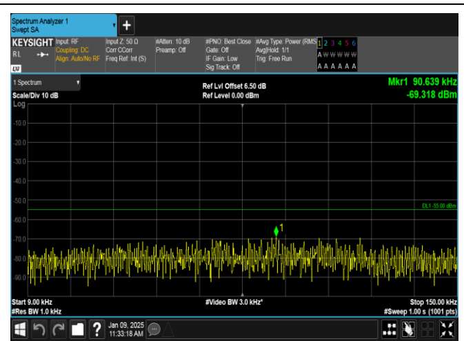
Band38-15MHz-QPSK-38000-1RB#0-0.009~0.15-PASS
