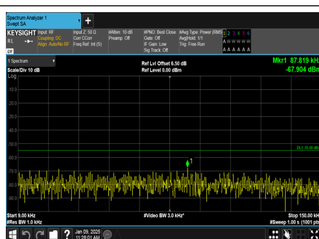
Band38-15MHz-16OAM-37825-1RB#0-0.009~0.15-PASS
