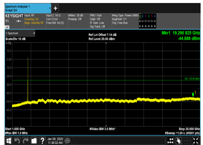
Band38-15MHz-QPSK-38000-1RB#74-1000~20000-PASS
