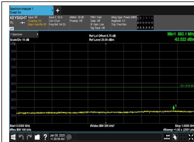
Band38-15MHz-QPSK-38175-1RB#0-30~1000-PASS
