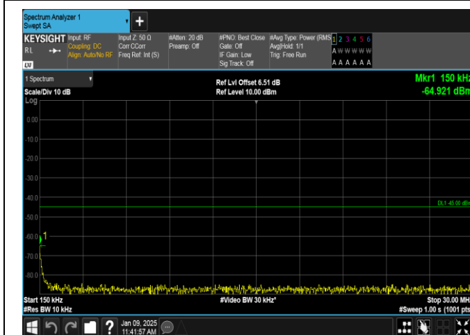
Band38-15MHz-QPSK-38175-1RB#74-0.15~30-PASS
