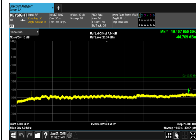
Band38-15MHz-16QAM-37825-75RB#0-1000~20000-PASS
