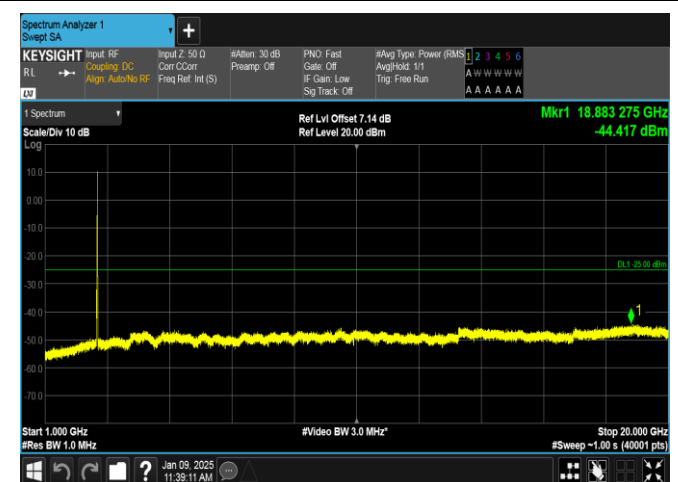
Band38-15MHz-16QAM-38000-75RB#0-1000~20000-PASS
