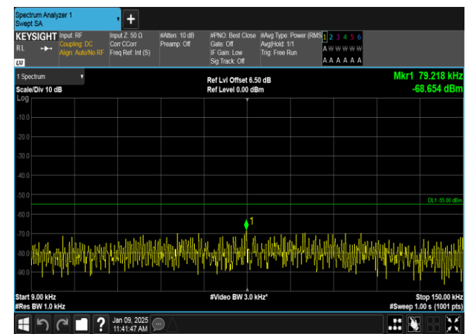
Band38-15MHz-QPSK-38175-1RB#74-0.009~0.15-PASS
