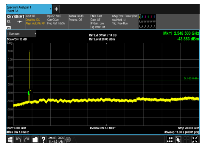
Band38-15MHz-QPSK-38175-75RB#0-1000~20000-PASS
