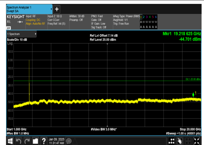
Band38-15MHz-QPSK-37825-75RB#0-1000~20000-PASS
