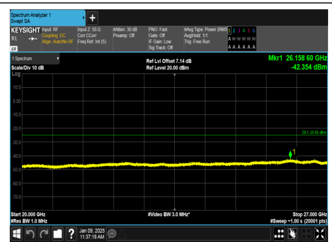
Band38-15MHz-16QAM-38000-1RB#74-20000~27000-PASS
