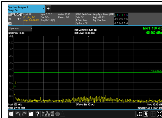
Band38-15MHz-16QAM-37825-75RB#0-0.15~30-PASS
