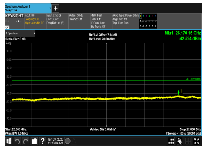
Band38-15MHz-16QAM-37825-75RB#0-20000~27000-PASS
