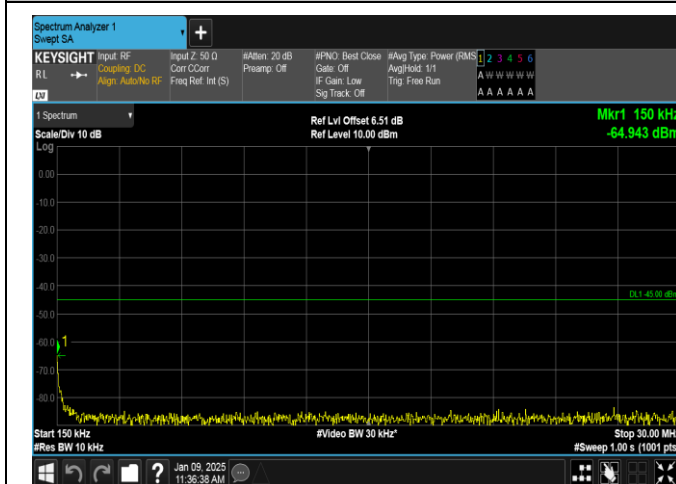
Band38-15MHz-16QAM-38000-1RB#74-0.15~30-PASS
