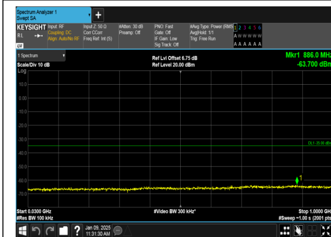
Band38-15MHz-QPSK-37825-75RB#0-30~1000-PASS
