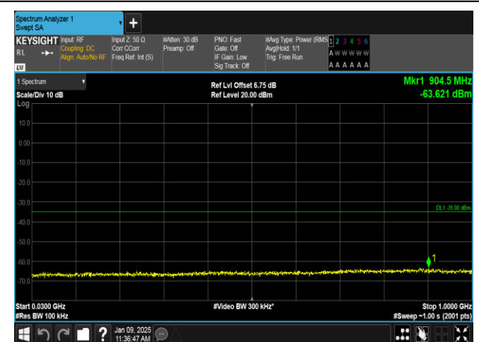
Band38-15MHz-16QAM-38000-1RB#74-30~1000-PASS
