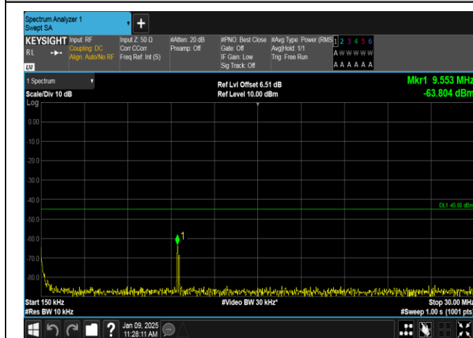
Band38-15MHz-16OAM-37825-1RB#0-0.15~30-PASS
