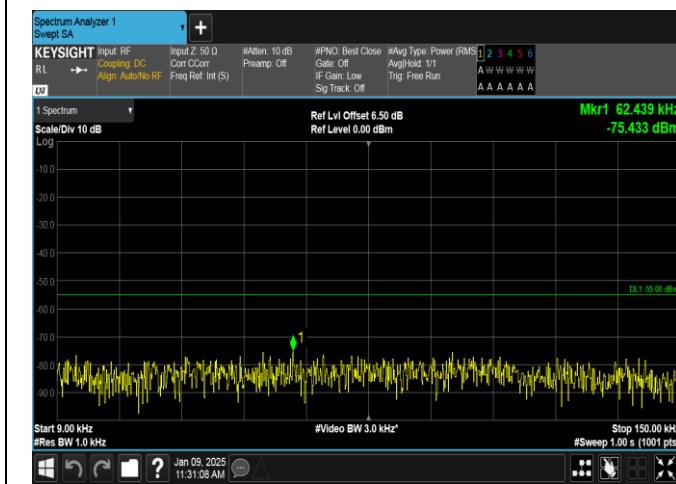
Band38-15MHz-QPSK-37825-75RB#0-0.009~0.15-PASS
