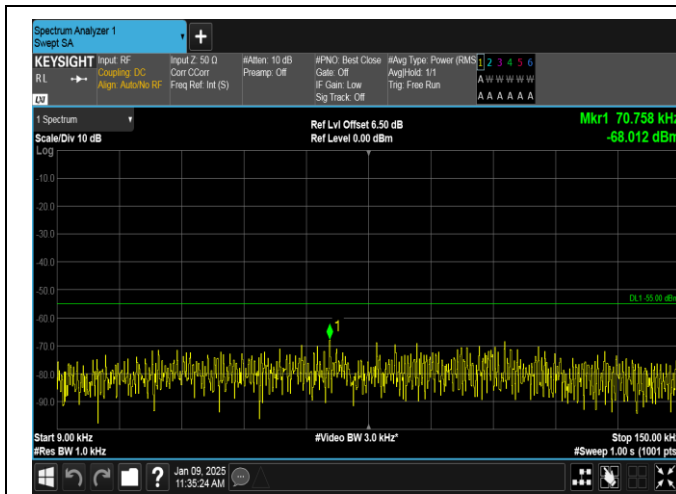
Band38-15MHz-QPSK-38000-1RB#74-0.009~0.15-PASS
