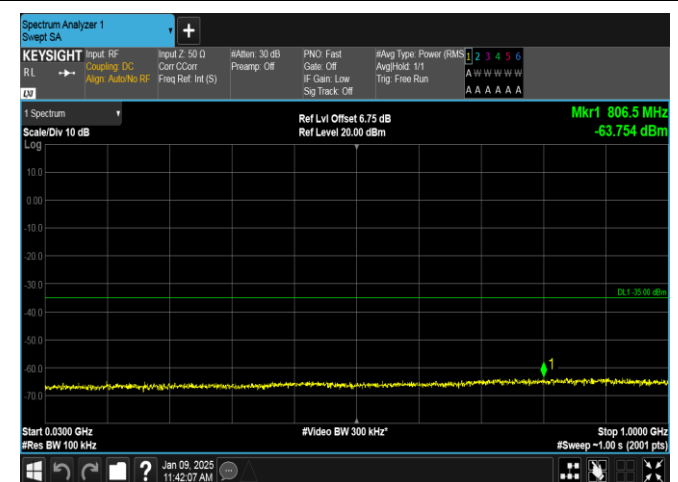
Band38-15MHz-QPSK-38175-1RB#74-30~1000-PASS
