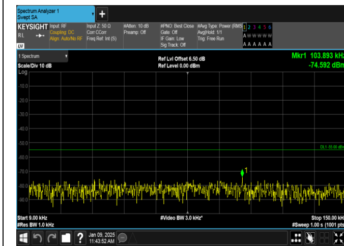
Band38-15MHz-QPSK-38175-75RB#0-0.009~0.15-PASS
