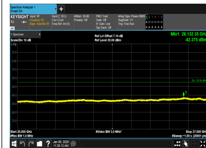
Band38-15MHz-16QAM-38000-1RB#0-20000~27000-PASS
