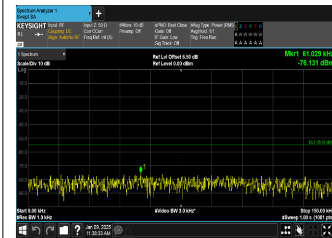
Band38-15MHz-16QAM-38000-75RB#0-0.009~0.15-PASS
