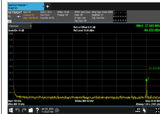
Band38-15MHz-QPSK-38000-1RB#0-0.15~30-PASS
