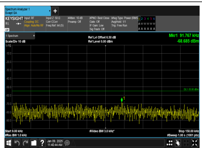
Band38-15MHz-16QAM-38175-1RB#0-0.009~0.15-PASS
