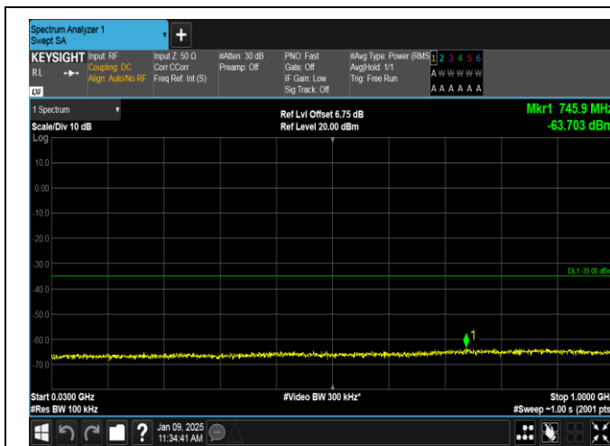
Band38-15MHz-16QAM-38000-1RB#0-30~1000-PASS
