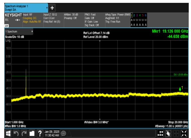
Band38-15MHz-16QAM-37825-1RB#74-1000~20000-PASS
