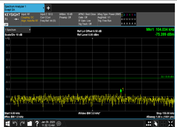
Band38-15MHz-16QAM-37825-75RB#0-0.009~0.15-PASS
