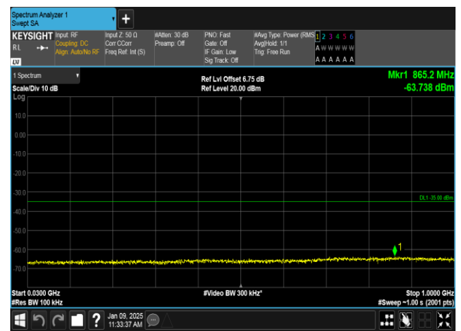
Band38-15MHz-QPSK-38000-1RB#0-30~1000-PASS
