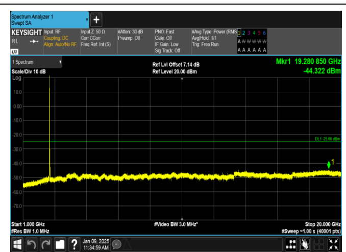
Band38-15MHz-16QAM-38000-1RB#0-1000~20000-PASS
