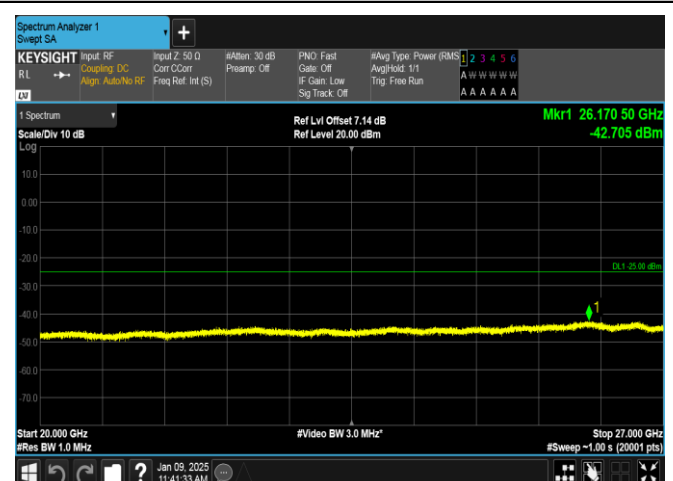
Band38-15MHz-16QAM-38175-1RB#0-20000~27000-PASS
