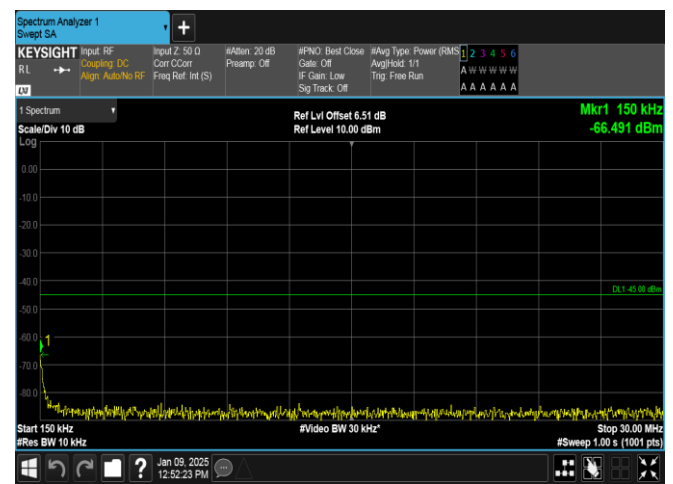
Band38-20MHz-QPSK-38150-100RB#0-0.15~30-PASS
