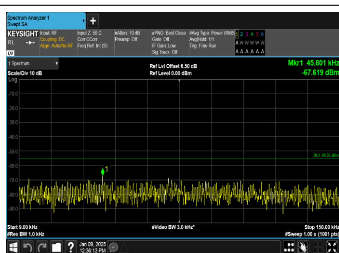
Band38-20MHz-16QAM-37850-1RB#0-0.009~0.15-PASS
