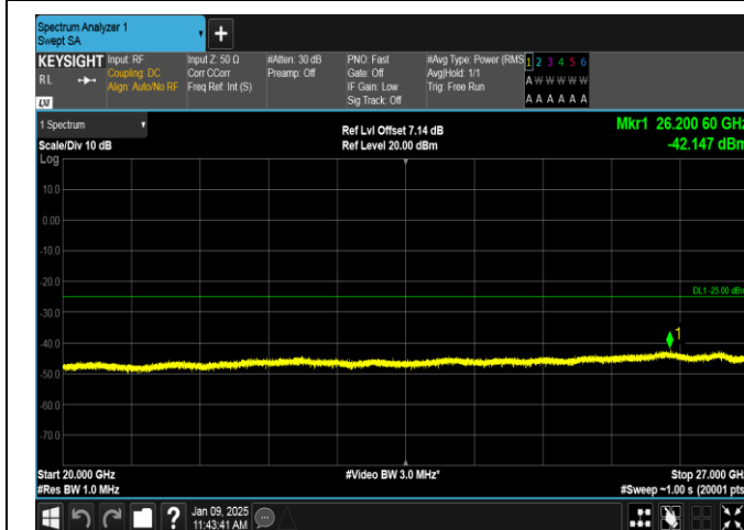
Band38-15MHz-16QAM-38175-1RB#74-20000~27000-PASS
