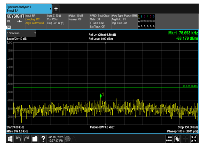
Band38-20MHz-QPSK-37850-1RB#99-0.009~0.15-PASS
