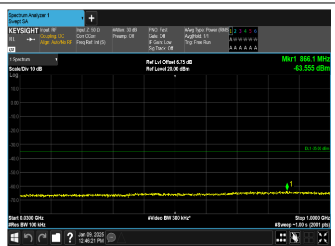
Band38-20MHz-QPSK-38000-100RB#0-30~1000-PASS
