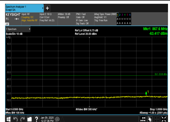
Band38-20MHz-QPSK-37850-1RB#99-30~1000-PASS
