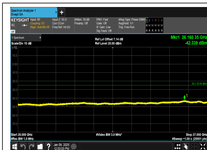
Band38-20MHz-OPSK-38150-100RB#0-20000~27000-PASS
