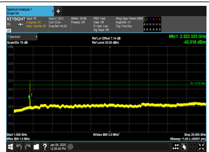
Band38-20MHz-QPSK-37850-1RB#0-1000~20000-PASS
