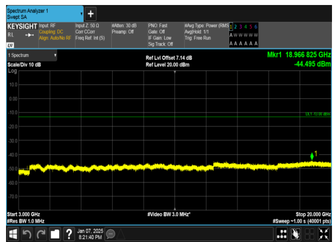
Band4-1.4MHz-16QAM-20175-1RB#5-3000~20000-PASS
