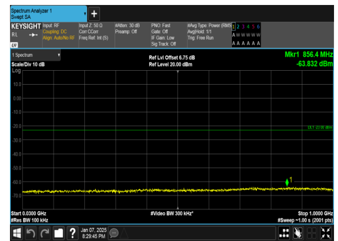
Band4-1.4MHz-16QAM-20393-6RB#0-30~1000-PASS
