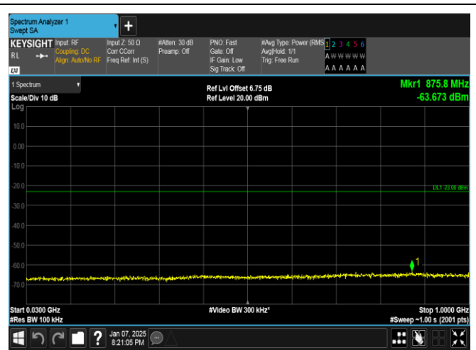
Band4-1.4MHz-16QAM-20175-1RB#5-30~1000-PASS
