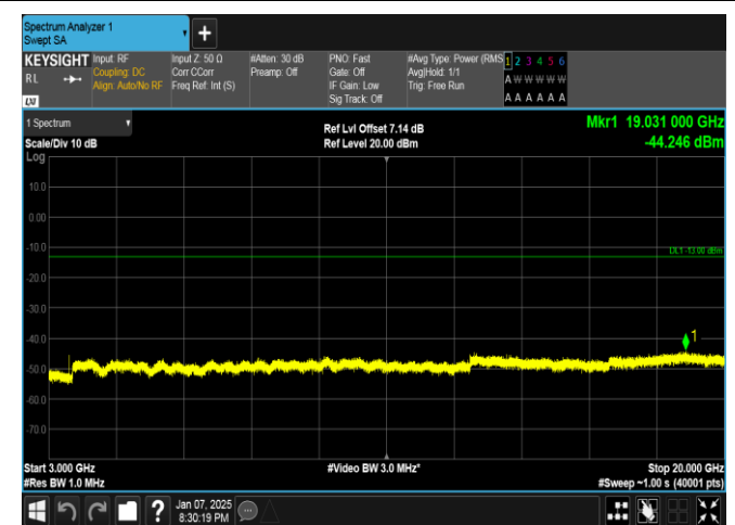
Band4-1.4MHz-16QAM-20393-6RB#0-3000~20000-PASS
