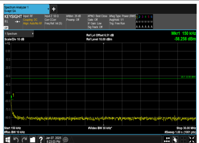
Band4-1.4MHz-16QAM-20175-6RB#0-0.15~30-PASS
