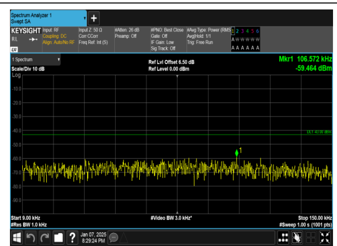
Band4-1.4MHz-16QAM-20393-6RB#0-0.009~0.15-PASS
