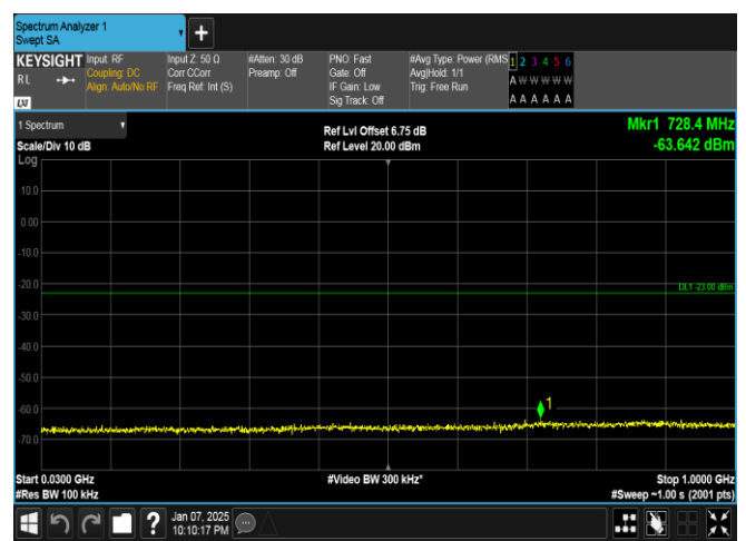
Band4-5MHz-16QAM-20375-25RB#0-30~1000-PASS
