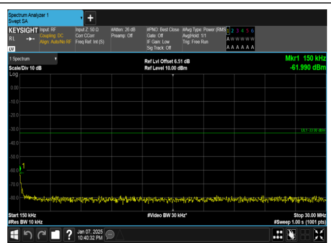
Band4-10MHz-QPSK-20000-1RB#0-0.15~30-PASS
