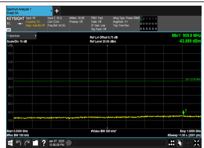
Band4-10MHz-QPSK-20350-1RB#49-30~1000-PASS
