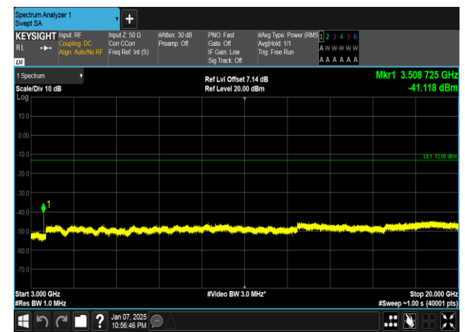
Band4-10MHz-QPSK-20350-1RB#49-3000~20000-PASS
