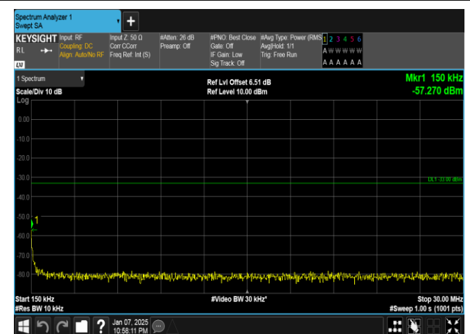
Band4-10MHz-QPSK-20350-50RB#0-0.15~30-PASS
