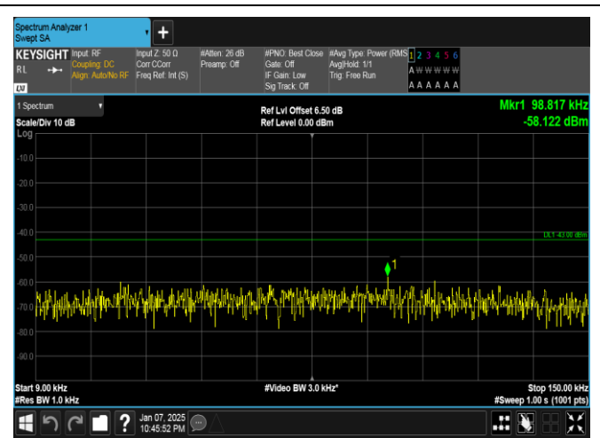
Band4-10MHz-16QAM-20000-50RB#0-0.009~0.15-PASS
