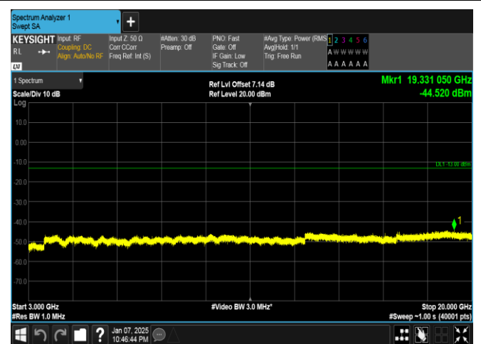
Band4-10MHz-16QAM-20000-50RB#0-3000~20000-PASS
