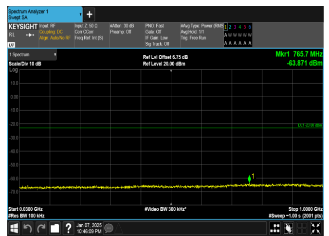
Band4-10MHz-16QAM-20000-50RB#0-30~1000-PASS
