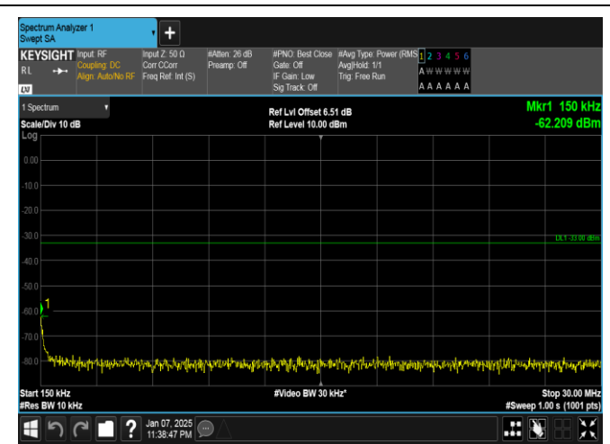
Band4-15MHz-16QAM-20175-1RB#0-0.15~30-PASS
