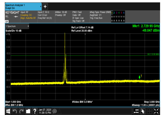
Band4-15MHz-16QAM-20175-1RB#0-1000~3000-PASS
