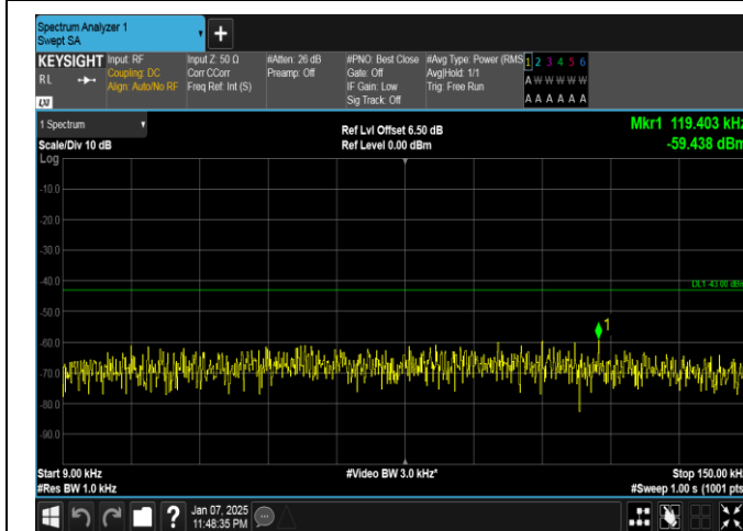
Band4-15MHz-QPSK-20325-75RB#0-0.009~0.15-PASS
