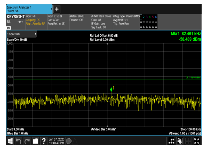
Band4-15MHz-16QAM-20175-1RB#74-0.009~0.15-PASS
