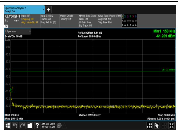
Band4-20MHz-QPSK-20300-1RB#0-0.15~30-PASS
