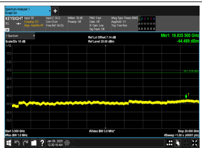
Band4-20MHz-QPSK-20175-1RB#0-3000~20000-PASS
