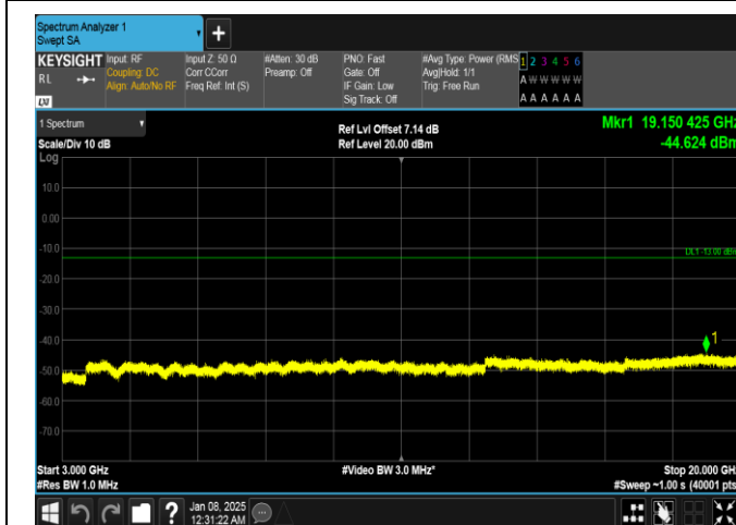
Band4-20MHz-16QAM-20175-1RB#0-3000~20000-PASS
