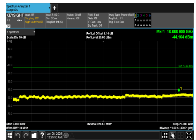
Band4-20MHz-QPSK-20050-1RB#99-3000~20000-PASS
