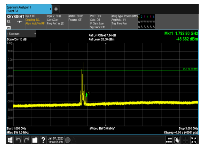
Band4-15MHz-16QAM-20325-1RB#74-1000~3000-PASS
