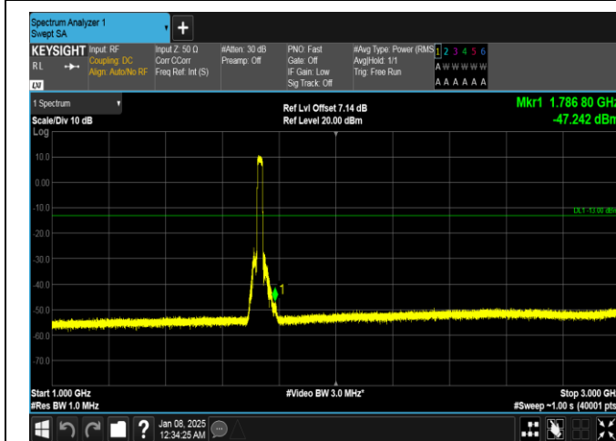
Band4-20MHz-QPSK-20175-100RB#0-1000~3000-PASS
