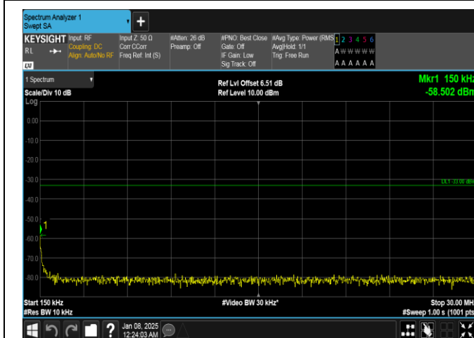
Band4-20MHz-16QAM-20050-1RB#0-0.15~30-PASS
