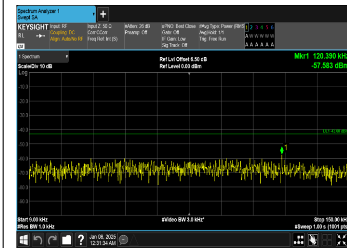
Band4-20MHz-QPSK-20175-1RB#99-0.009~0.15-PASS
