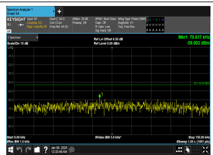
Band4-20MHz-QPSK-20175-100RB#0-0.009~0.15-PASS
