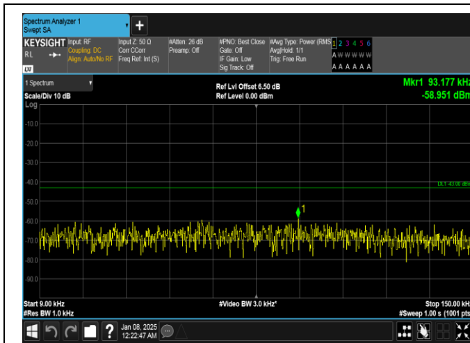
Band4-20MHz-QPSK-20050-1RB#0-0.009~0.15-PASS
