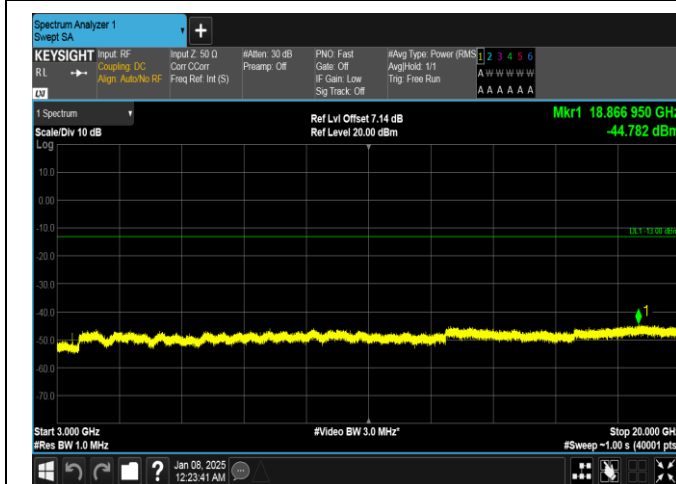
Band4-20MHz-QPSK-20050-1RB#0-3000~20000-PASS
