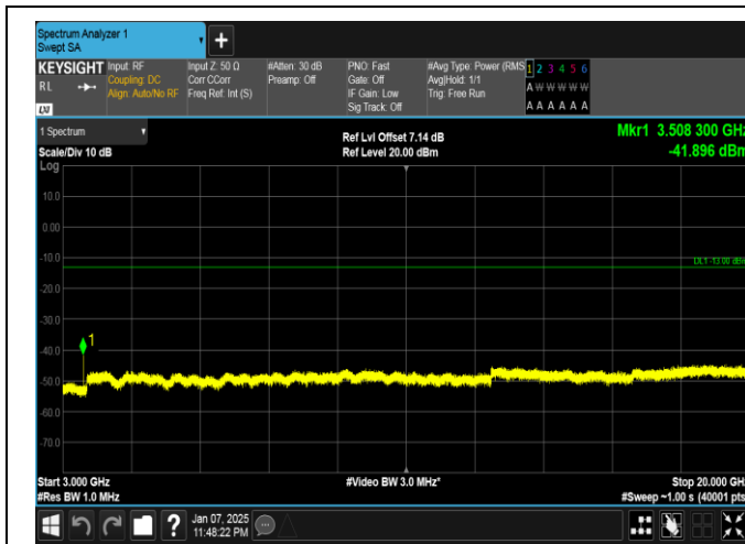
Band4-15MHz-16QAM-20325-1RB#74-3000~20000-PASS
