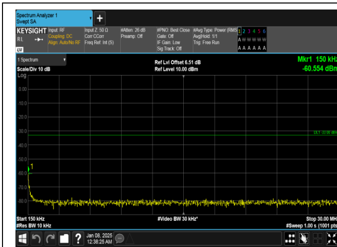
Band4-20MHz-QPSK-20300-1RB#99-0.15~30-PASS
