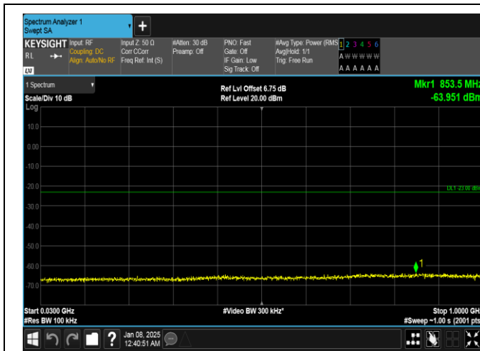
Band4-20MHz-QPSK-20300-100RB#0-30~1000-PASS
