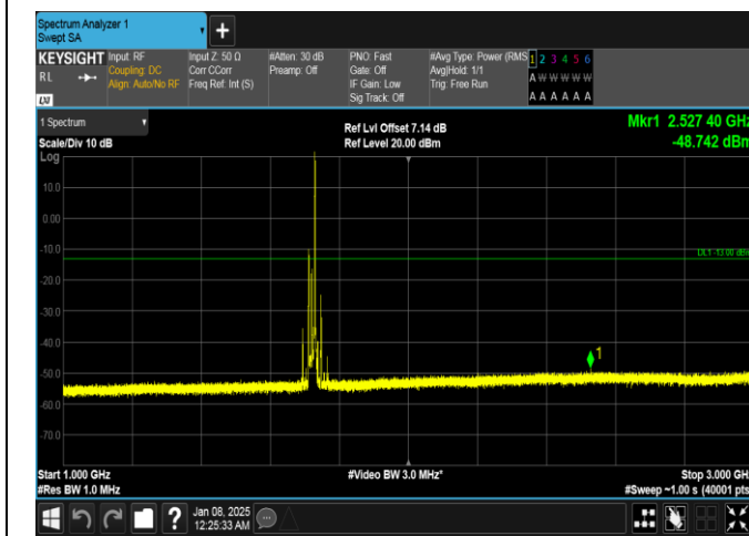
Band4-20MHz-QPSK-20050-1RB#99-1000~3000-PASS
