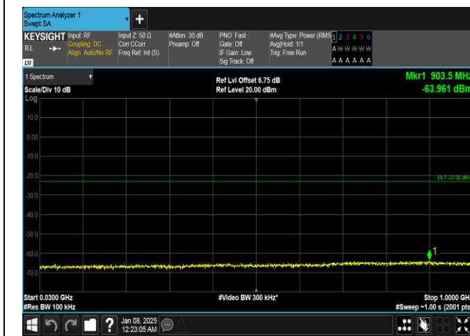
Band4-20MHz-QPSK-20050-1RB#0-30~1000-PASS
