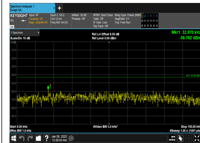
Band4-20MHz-16QAM-20050-1RB#99-0.009~0.15-PASS
