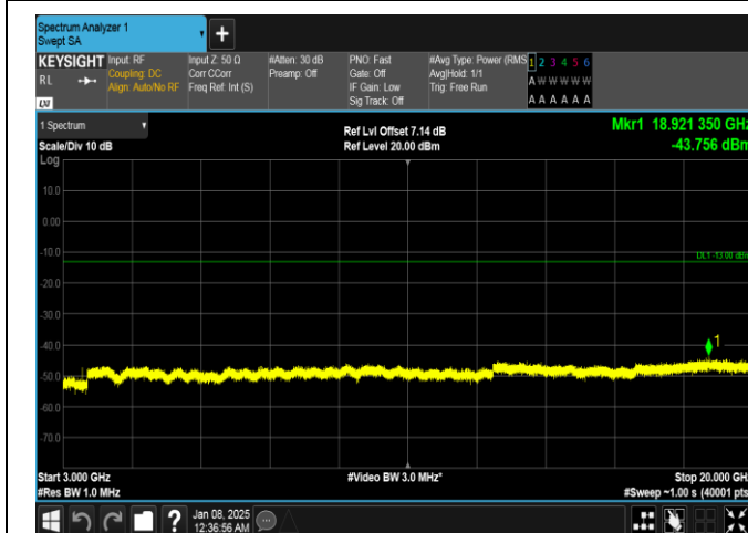
Band4-20MHz-QPSK-20300-1RB#0-3000~20000-PASS
