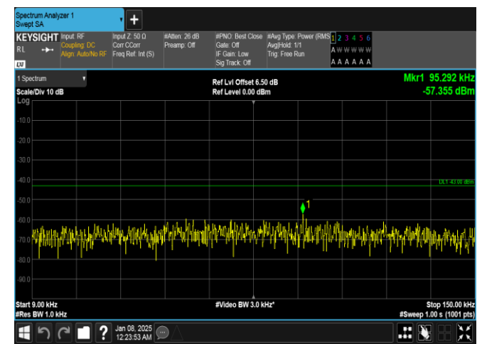
Band4-20MHz-16QAM-20050-1RB#0-0.009~0.15-PASS
