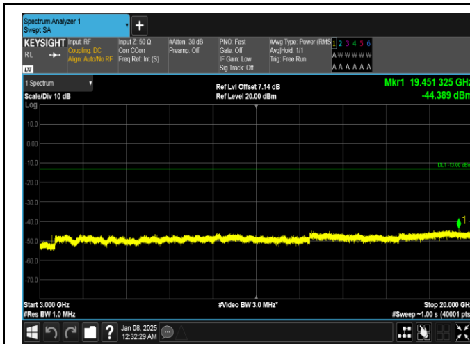
Band4-20MHz-QPSK-20175-1RB#99-3000~20000-PASS
