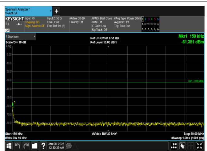
Band4-20MHz-16QAM-20175-1RB#0-0.15~30-PASS
