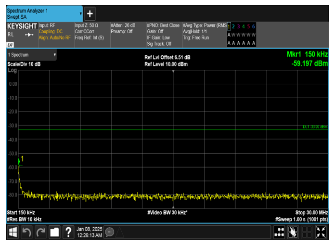
Band4-20MHz-16QAM-20050-1RB#99-0.15~30-PASS
