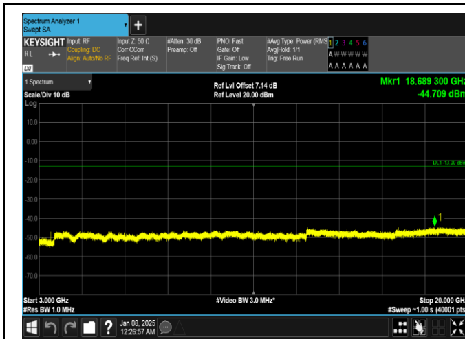
Band4-20MHz-16QAM-20050-1RB#99-3000~20000-PASS
