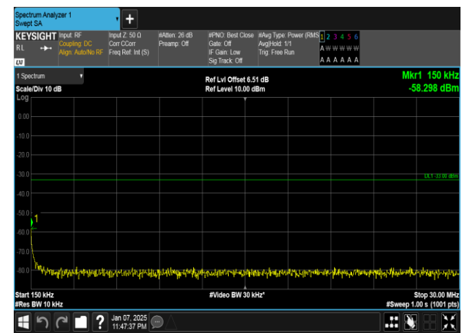
Band4-15MHz-16QAM-20325-1RB#74-0.15~30-PASS
