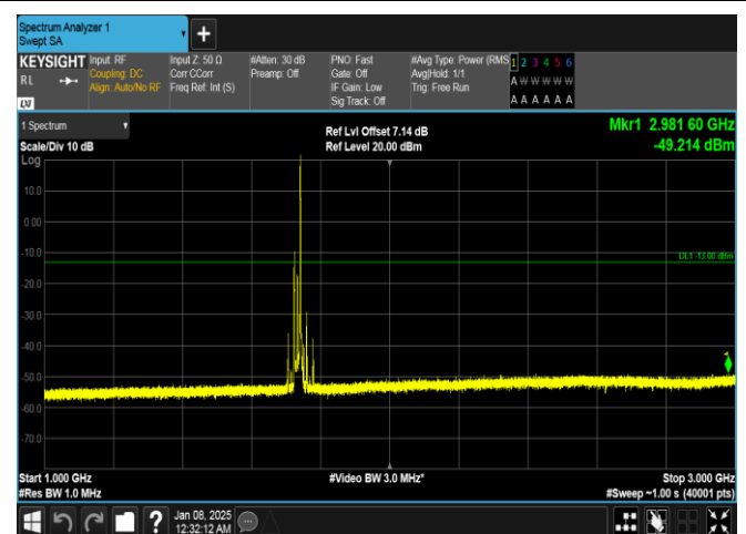
Band4-20MHz-QPSK-20175-1RB#99-1000~3000-PASS
