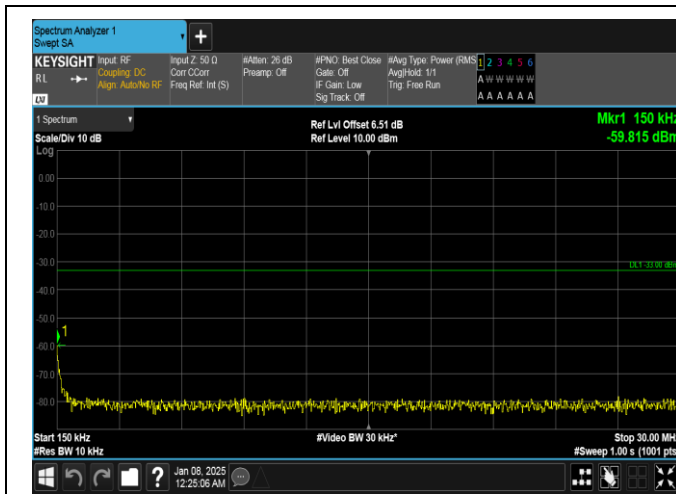
Band4-20MHz-QPSK-20050-1RB#99-0.15~30-PASS
