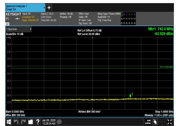
Band4-20MHz-16QAM-20050-100RB#0-30~1000-PASS
