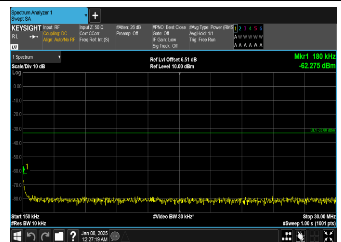
Band4-20MHz-QPSK-20050-100RB#0-0.15~30-PASS
