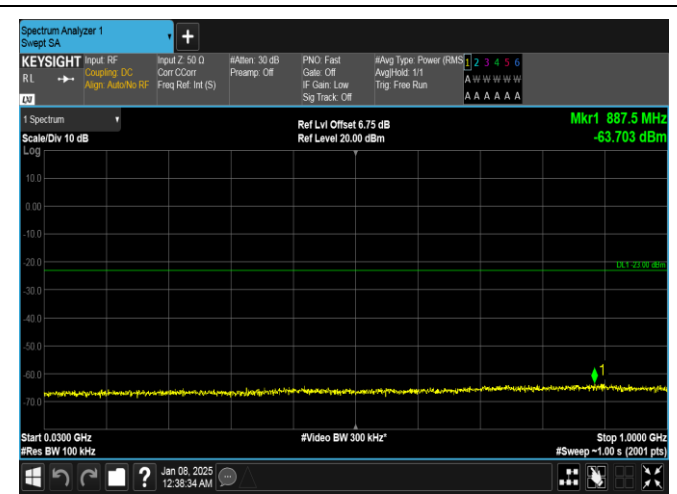
Band4-20MHz-QPSK-20300-1RB#99-30~1000-PASS
