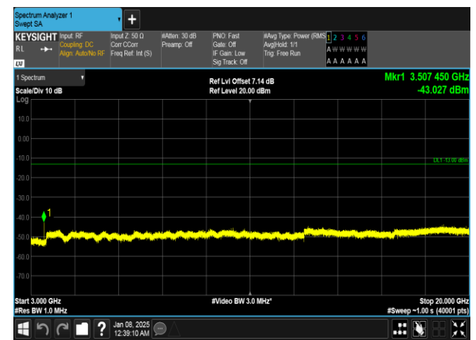
Band4-20MHz-QPSK-20300-1RB#99-3000~20000-PASS
