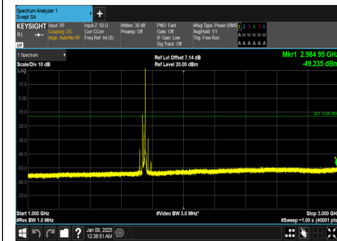
Band4-20MHz-QPSK-20300-1RB#99-1000~3000-PASS
