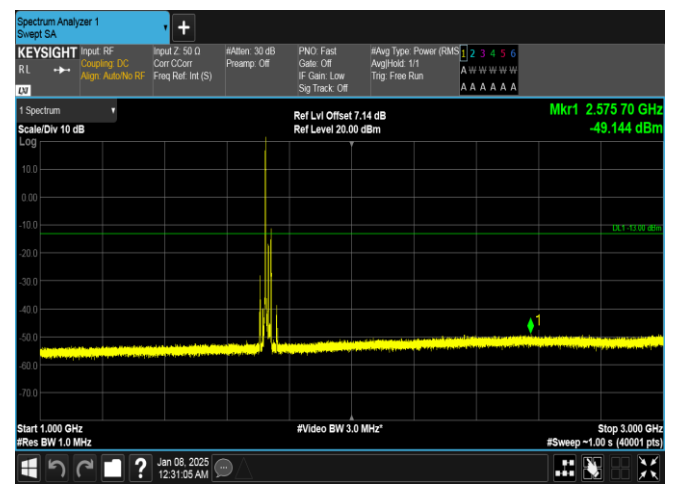
Band4-20MHz-16QAM-20175-1RB#0-1000~3000-PASS
