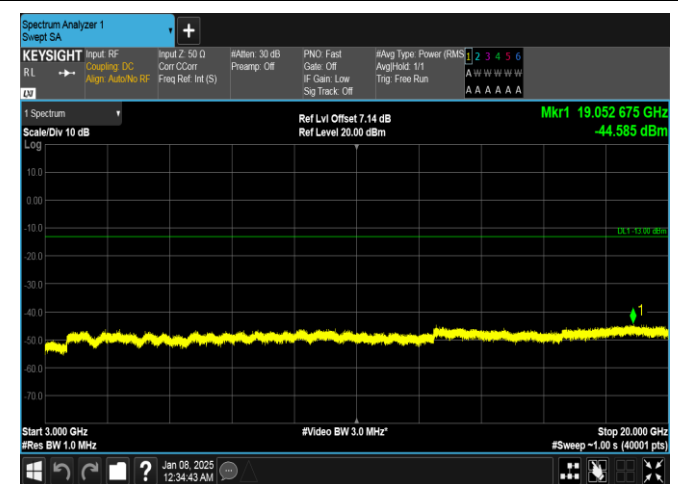
Band4-20MHz-QPSK-20175-100RB#0-3000~20000-PASS
