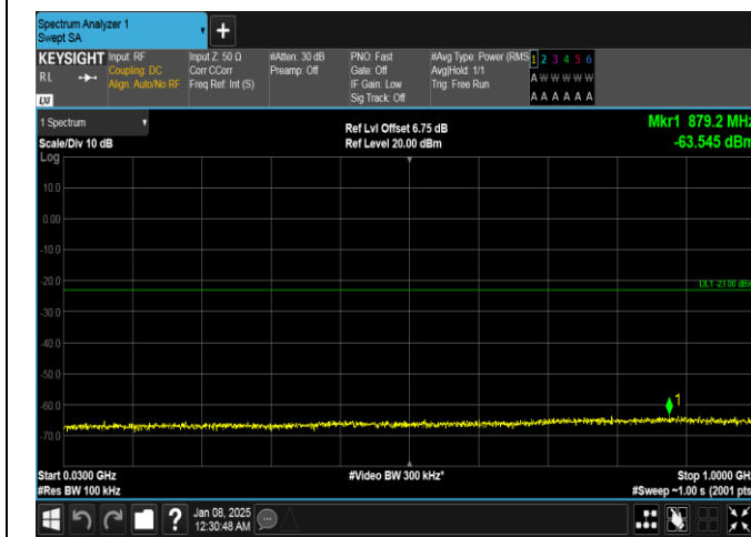
Band4-20MHz-16QAM-20175-1RB#0-30~1000-PASS
