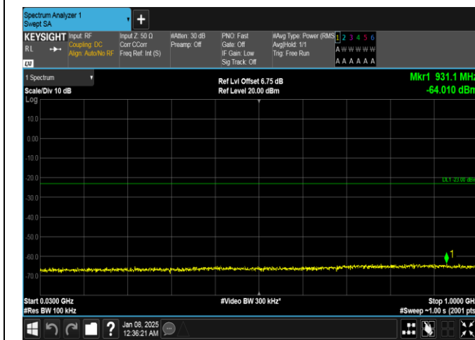
Band4-20MHz-QPSK-20300-1RB#0-30~1000-PASS
