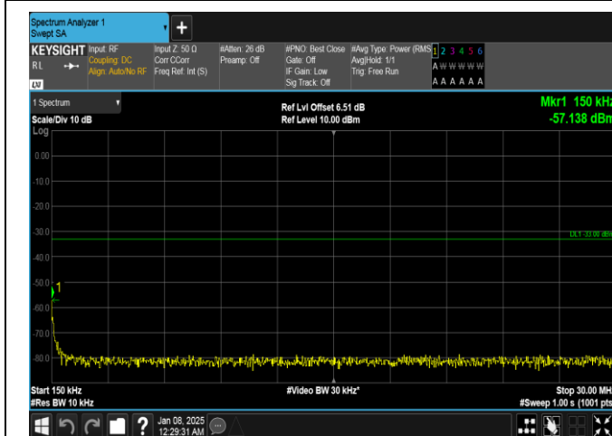
Band4-20MHz-QPSK-20175-1RB#0-0.15~30-PASS
