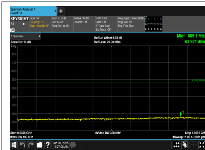
Band4-20MHz-QPSK-20050-100RB#0-30~1000-PASS
