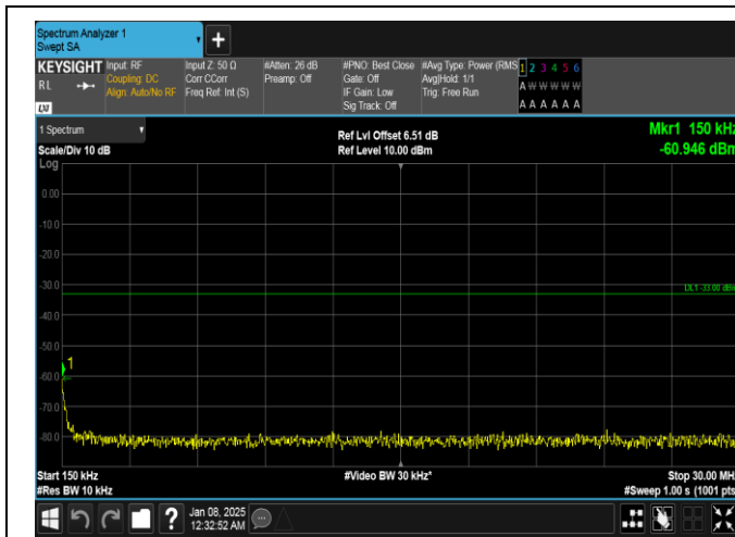
Band4-20MHz-16QAM-20175-1RB#99-0.15~30-PASS
