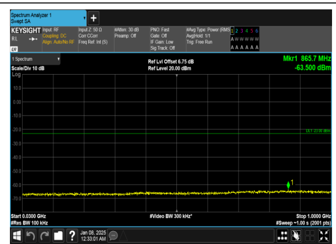
Band4-20MHz-16QAM-20175-1RB#99-30~1000-PASS
