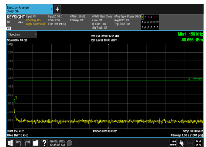
Band4-20MHz-16QAM-20175-100RB#0-0.15~30-PASS
