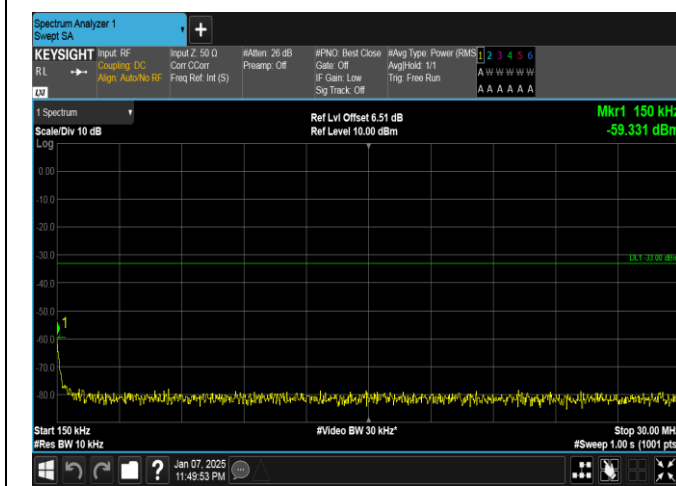
Band4-15MHz-16QAM-20325-75RB#0-0.15~30-PASS
