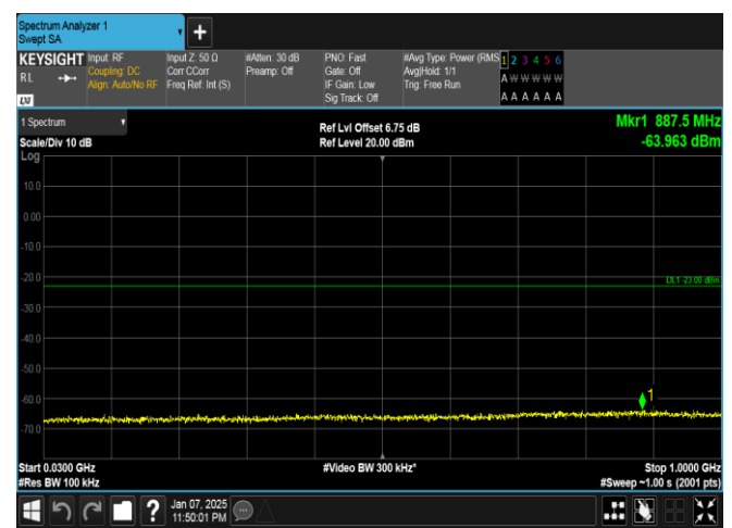
Band4-15MHz-16QAM-20325-75RB#0-30~1000-PASS
