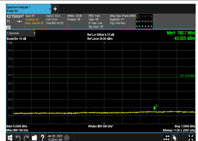
Band4-20MHz-QPSK-20175-1RB#0-30~1000-PASS
