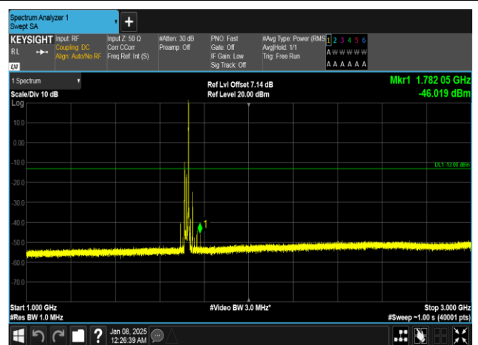
Band4-20MHz-16QAM-20050-1RB#99-1000~3000-PASS
