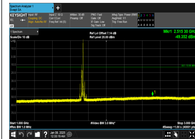
Band4-20MHz-16QAM-20175-1RB#99-1000~3000-PASS
