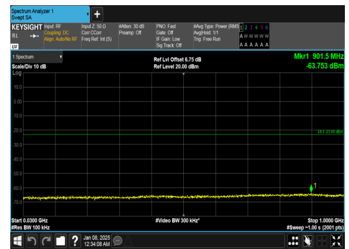
Band4-20MHz-QPSK-20175-100RB#0-30~1000-PASS
