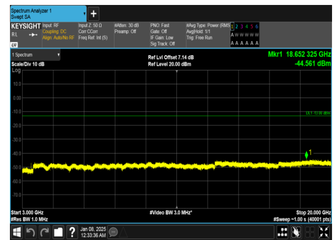
Band4-20MHz-16QAM-20175-1RB#99-3000~20000-PASS
