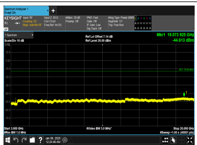
Band4-20MHz-16QAM-20050-1RB#0-3000~20000-PASS
