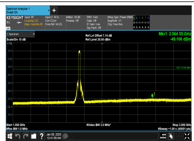
Band4-20MHz-QPSK-20300-100RB#0-1000~3000-PASS
