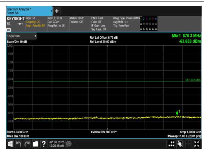
Band4-20MHz-QPSK-20050-1RB#99-30~1000-PASS
