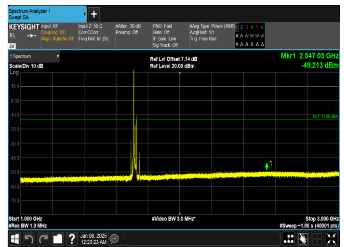
Band4-20MHz-QPSK-20050-1RB#0-1000~3000-PASS
