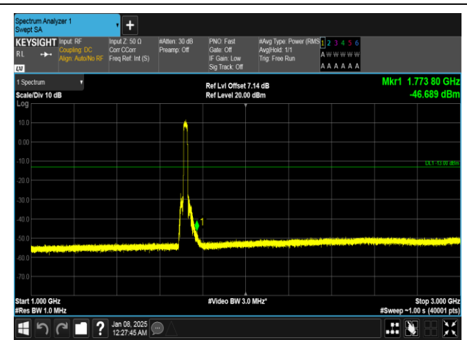
Band4-20MHz-QPSK-20050-100RB#0-1000~3000-PASS
