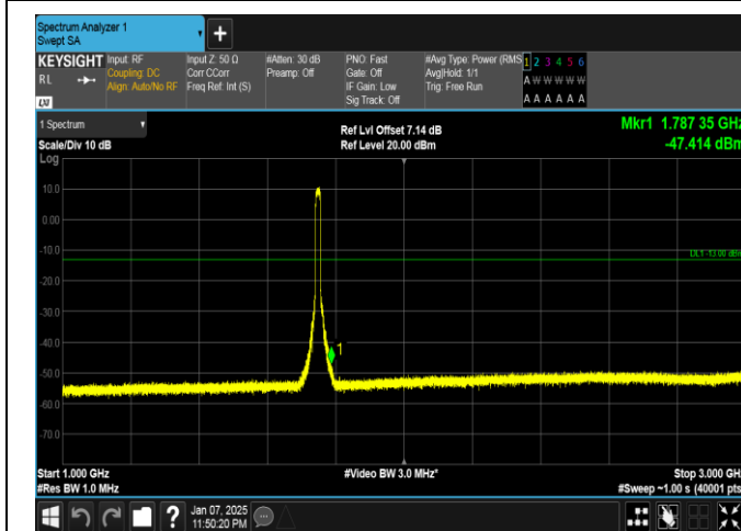
Band4-15MHz-16QAM-20325-75RB#0-1000~3000-PASS
