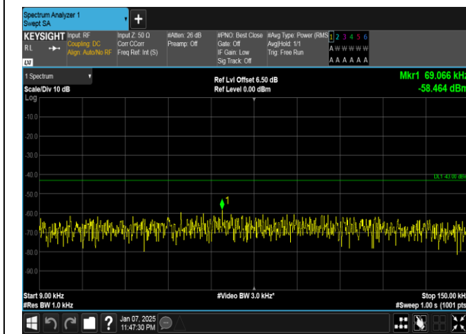
Band4-15MHz-16QAM-20325-1RB#74-0.009~0.15-PASS
