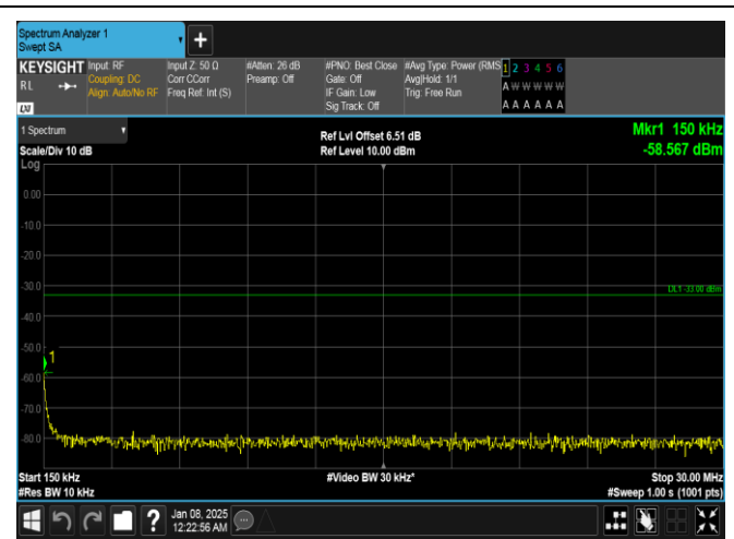
Band4-20MHz-QPSK-20050-1RB#0-0.15~30-PASS
