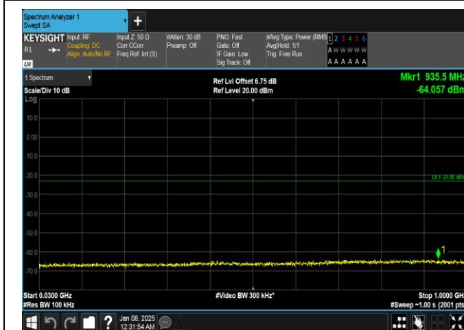
Band4-20MHz-QPSK-20175-1RB#99-30~1000-PASS
