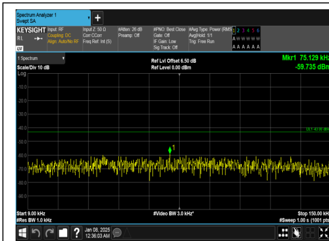
Band4-20MHz-QPSK-20300-1RB#0-0.009~0.15-PASS
