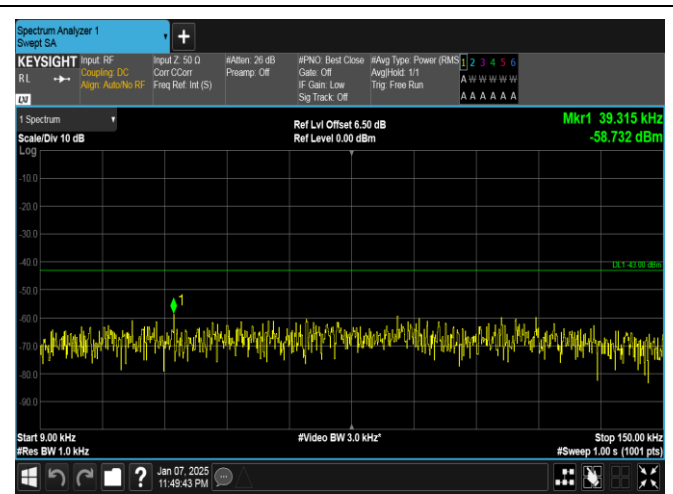
Band4-15MHz-16QAM-20325-75RB#0-0.009~0.15-PASS
