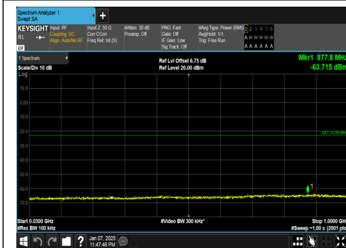
Band4-15MHz-16QAM-20325-1RB#74-30~1000-PASS
