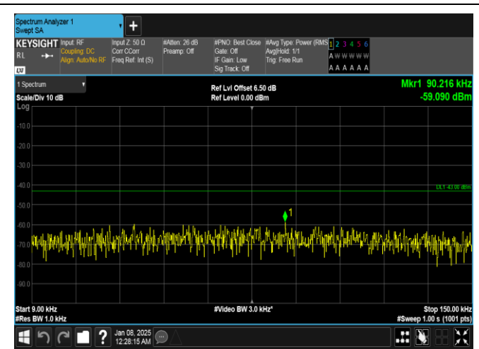
Band4-20MHz-16QAM-20050-100RB#0-0.009~0.15-PASS
