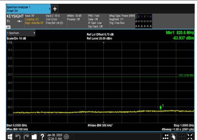
Band4-20MHz-16QAM-20050-1RB#0-30~1000-PASS
