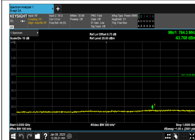
Band4-20MHz-16QAM-20050-1RB#99-30~1000-PASS
