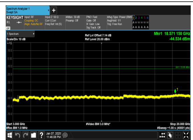
Band4-15MHz-16QAM-20325-1RB#0-3000~20000-PASS
