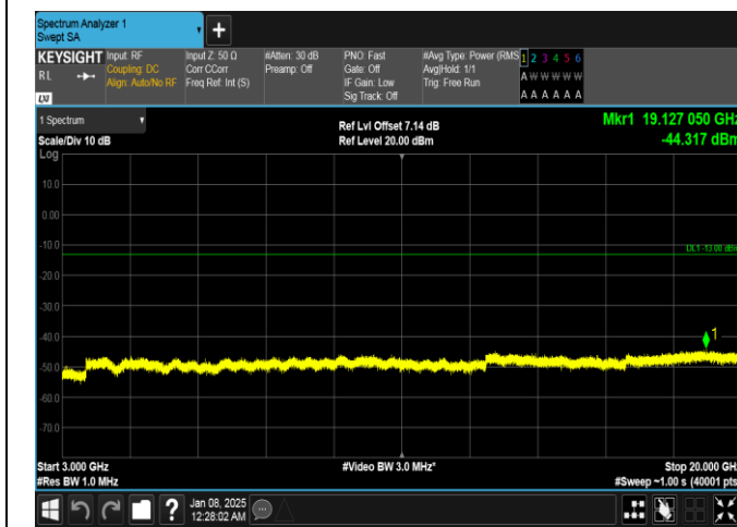
Band4-20MHz-QPSK-20050-100RB#0-3000~20000-PASS
