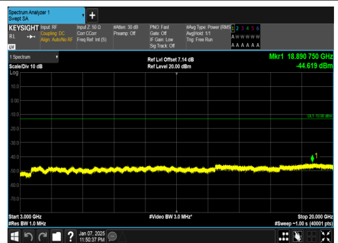
Band4-15MHz-16QAM-20325-75RB#0-3000~20000-PASS
