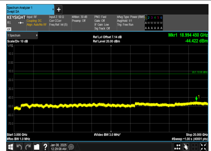
Band4-20MHz-16QAM-20050-100RB#0-3000~20000-PAS
