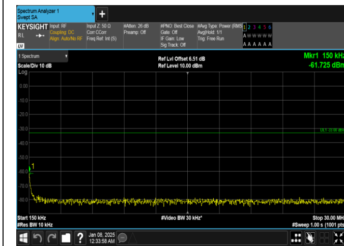
Band4-20MHz-QPSK-20175-100RB#0-0.15~30-PASS
