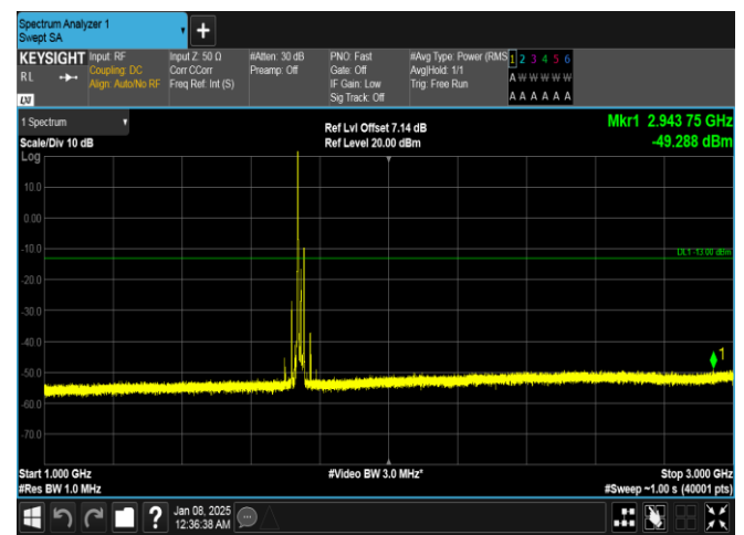
Band4-20MHz-QPSK-20300-1RB#0-1000~3000-PASS
