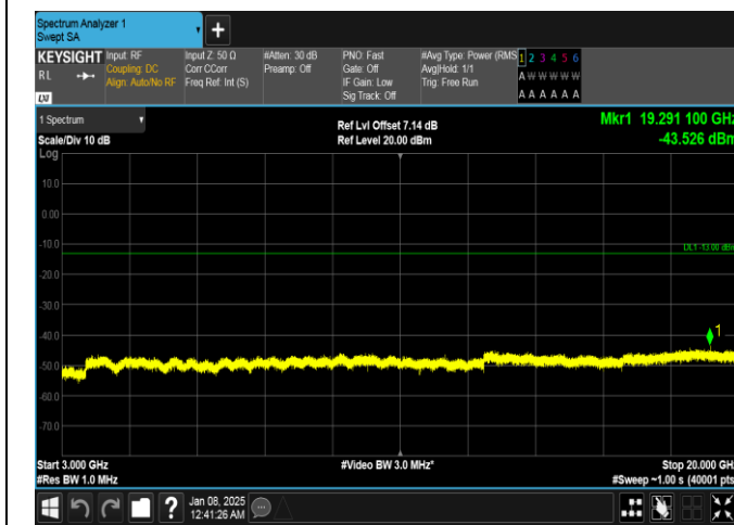
Band4-20MHz-QPSK-20300-100RB#0-3000~20000-PASS
