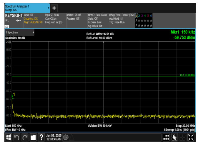
Band4-20MHz-QPSK-20175-1RB#99-0.15~30-PASS
