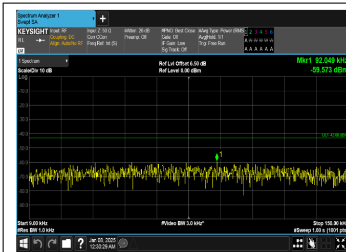
Band4-20MHz-16QAM-20175-1RB#0-0.009~0.15-PASS
