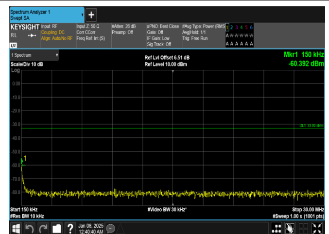
Band4-20MHz-QPSK-20300-100RB#0-0.15~30-PASS
