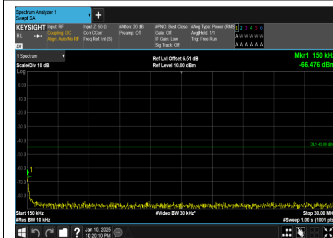
Band41-20MHz-16QAM-40620-1RB#99-0.15~30-PASS
