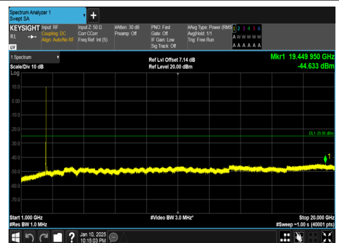
Band41-20MHz-QPSK-39750-100RB#0-1000~20000-PASS
