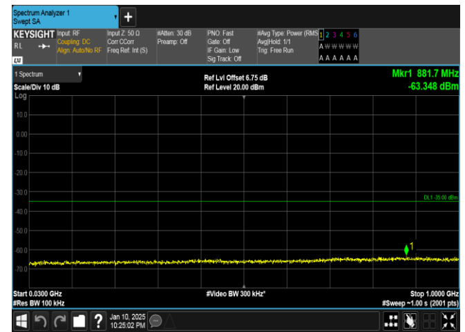
Band41-20MHz-16QAM-41490-1RB#0-30~1000-PASS
