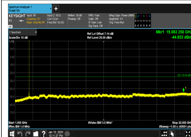
Band41-20MHz-16QAM-39750-1RB#0-1000~20000-PASS
