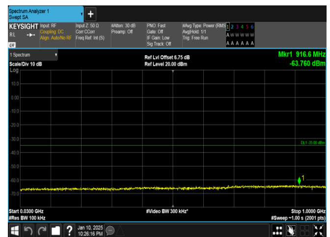
Band41-20MHz-QPSK-41490-1RB#99-30~1000-PASS
