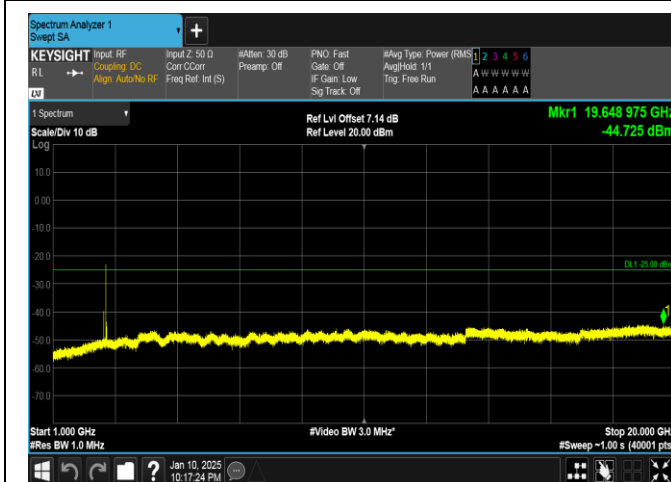
Band41-20MHz-QPSK-40620-1RB#0-1000~20000-PASS
