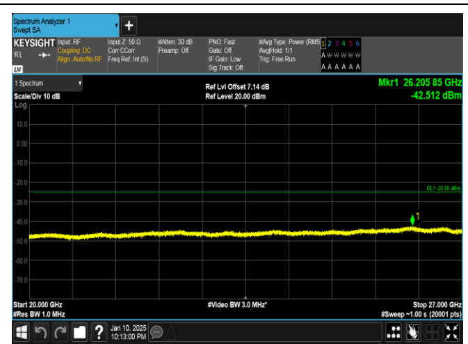
Band41-20MHz-QPSK-39750-1RB#99-20000~27000-PASS
