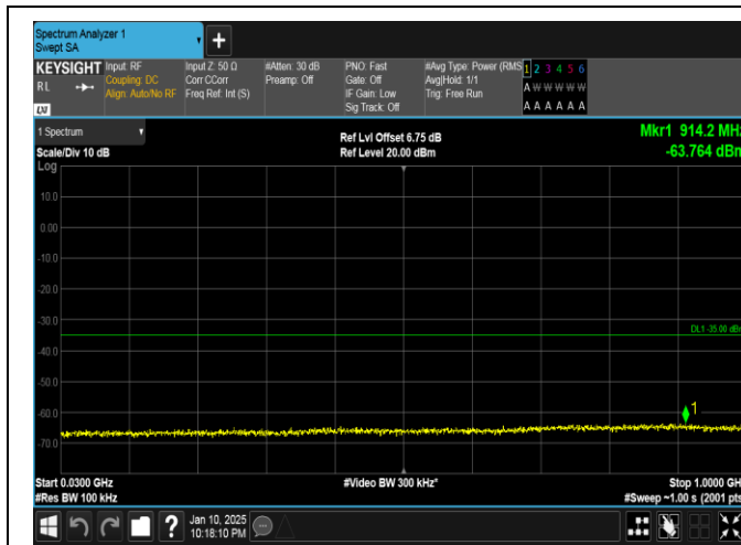
Band41-20MHz-16QAM-40620-1RB#0-30~1000-PASS
