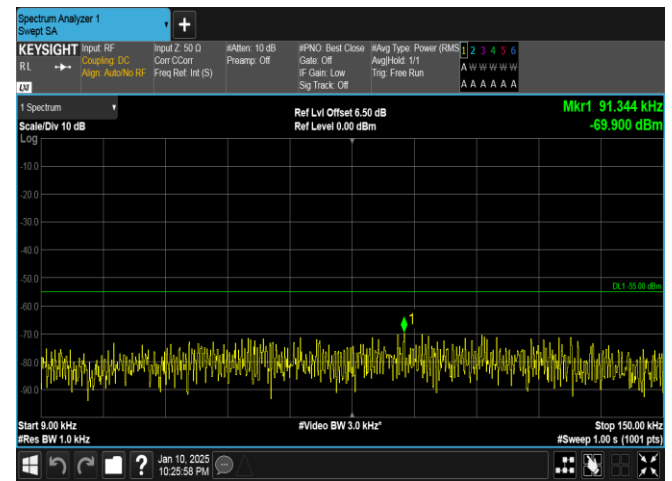
Band41-20MHz-QPSK-41490-1RB#99-0.009~0.15-PASS
