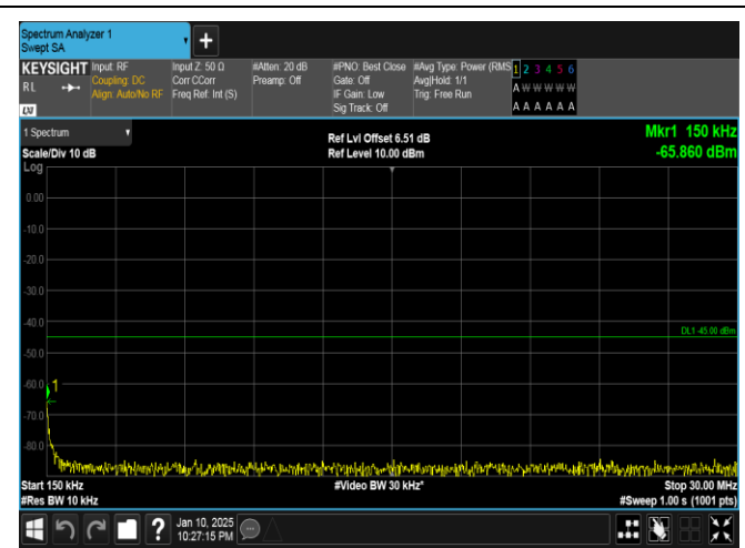
Band41-20MHz-16QAM-41490-1RB#99-0.15~30-PASS
