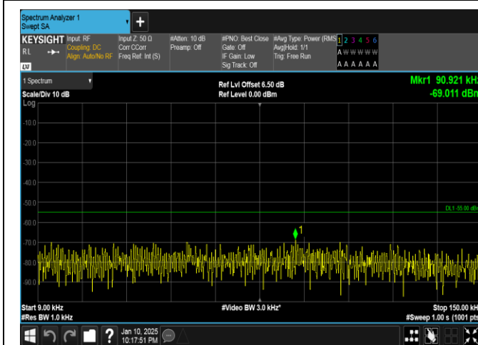
Band41-20MHz-16QAM-40620-1RB#0-0.009~0.15-PASS
