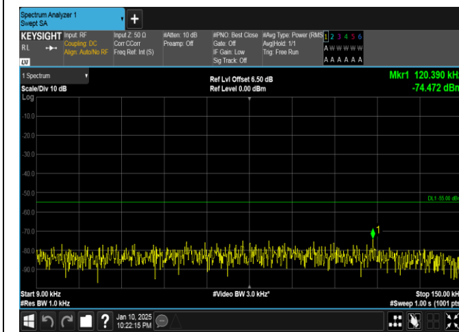
Band41-20MHz-16QAM-40620-100RB#0-0.009~0.15-PASS
