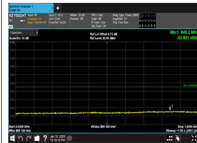
Band41-20MHz-QPSK-40620-1RB#99-30~1000-PASS
