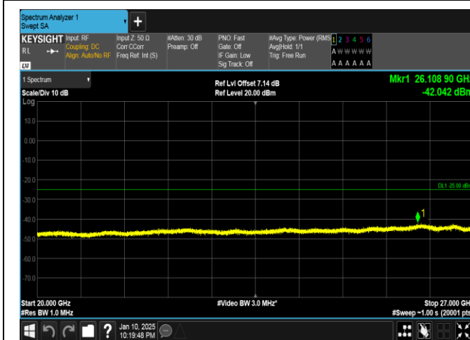
Band41-20MHz-QPSK-40620-1RB#99-20000~27000-PASS
