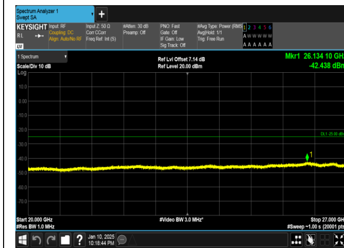
Band41-20MHz-16QAM-40620-1RB#0-20000~27000-PASS
