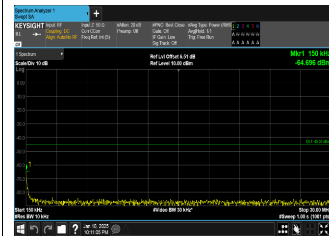
Band41-20MHz-16QAM-39750-1RB#0-0.15~30-PASS
