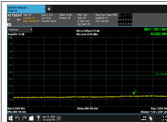
Band41-20MHz-QPSK-39750-1RB#0-30~1000-PASS
