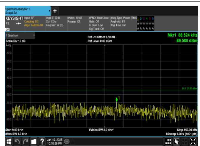
Band41-20MHz-16QAM-39750-1RB#0-0.009~0.15-PASS
