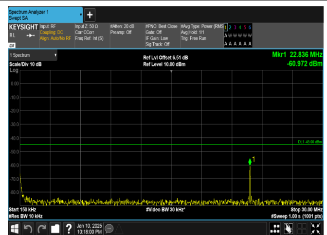
Band41-20MHz-16QAM-40620-1RB#0-0.15~30-PASS
