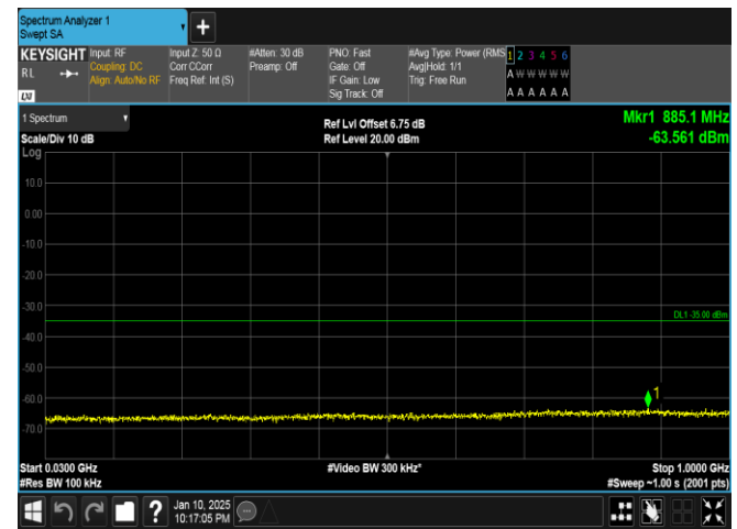
Band41-20MHz-QPSK-40620-1RB#0-30~1000-PASS
