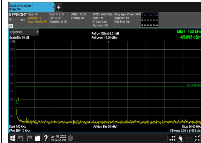
Band41-20MHz-16QAM-41490-1RB#0-0.15~30-PASS
