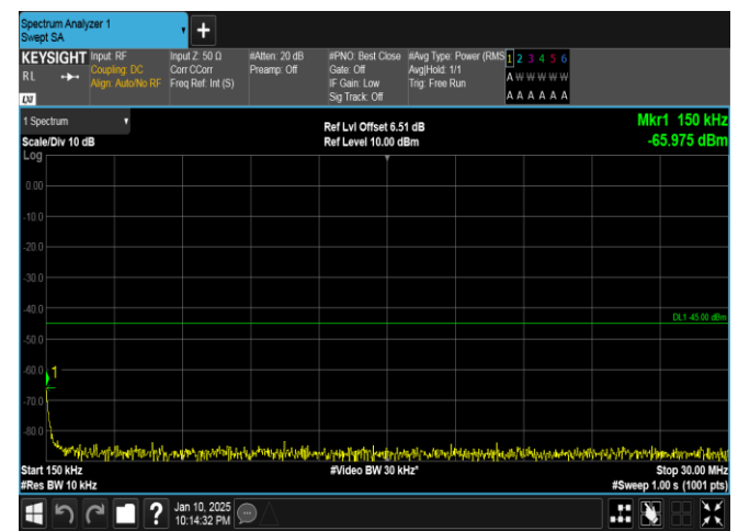
Band41-20MHz-QPSK-39750-100RB#0-0.15~30-PASS
