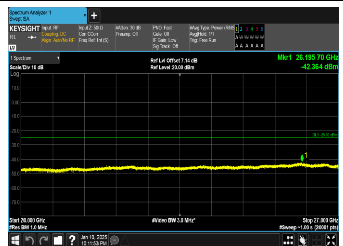
Band41-20MHz-16QAM-39750-1RB#0-20000~27000-PASS
