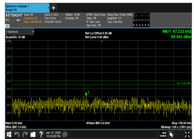
Band41-20MHz-16QAM-40620-1RB#99-0.009~0.15-PASS
