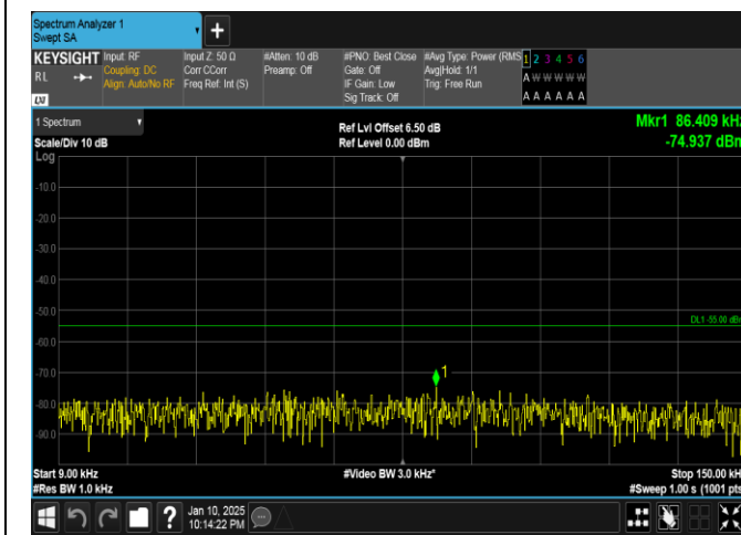
Band41-20MHz-QPSK-39750-100RB#0-0.009~0.15-PASS
