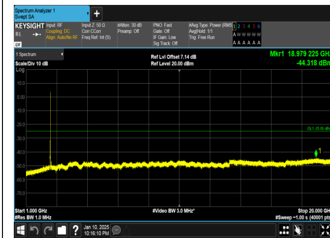
Band41-20MHz-16QAM-39750-100RB#0-1000~20000-PASS
