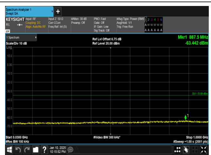
Band41-20MHz-16QAM-39750-100RB#0-30~1000-PASS
