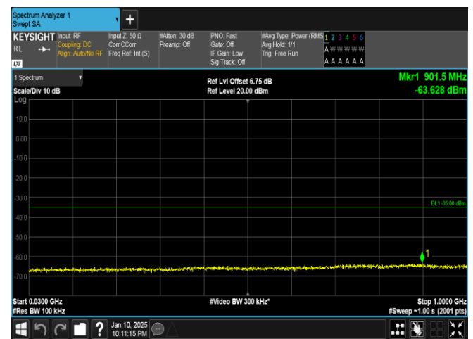
Band41-20MHz-16QAM-39750-1RB#0-30~1000-PASS
