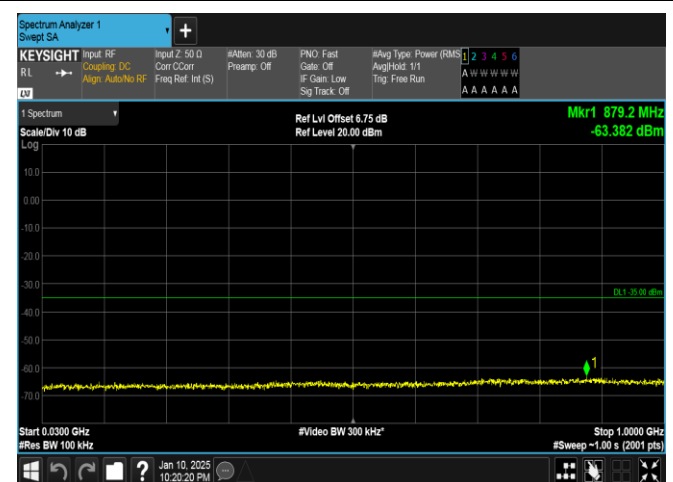
Band41-20MHz-16QAM-40620-1RB#99-30~1000-PASS
