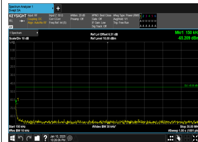
Band41-20MHz-QPSK-41490-1RB#99-0.15~30-PASS
