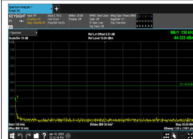
Band41-20MHz-QPSK-39750-1RB#99-0.15~30-PASS
