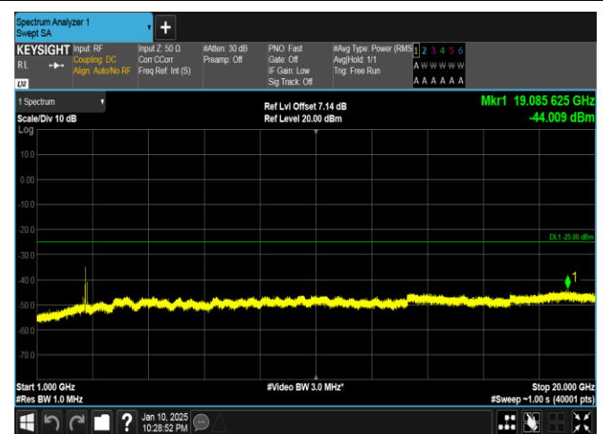
Band41-20MHz-QPSK-41490-100RB#0-1000~20000-PASS
