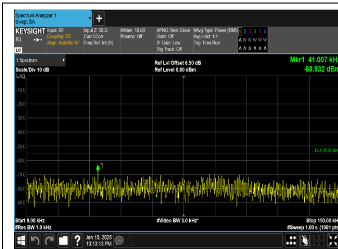
Band41-20MHz-16QAM-39750-1RB#99-0.009~0.15-PASS
