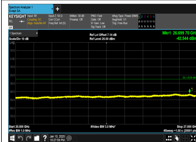
Band41-20MHz-16QAM-41490-1RB#99-20000~27000-PASS
