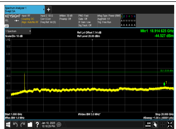
Band41-20MHz-16QAM-40620-1RB#0-1000~20000-PASS
