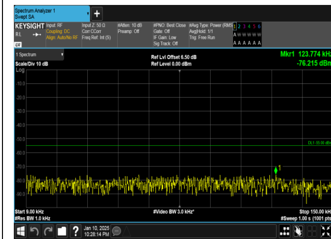
Band41-20MHz-QPSK-41490-100RB#0-0.009~0.15-PASS
