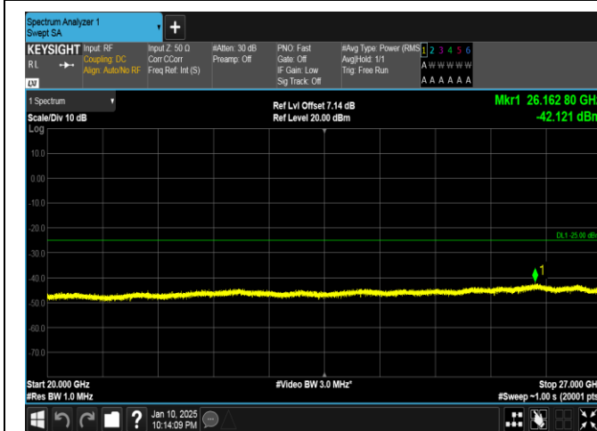
Band41-20MHz-16QAM-39750-1RB#99-20000~27000-PASS
