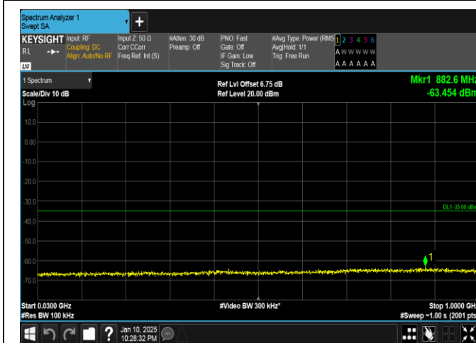
Band41-20MHz-QPSK-41490-100RB#0-30~1000-PASS
