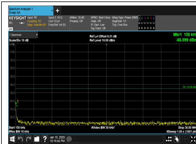
Band41-20MHz-16QAM-39750-100RB#0-0.15~30-PASS
