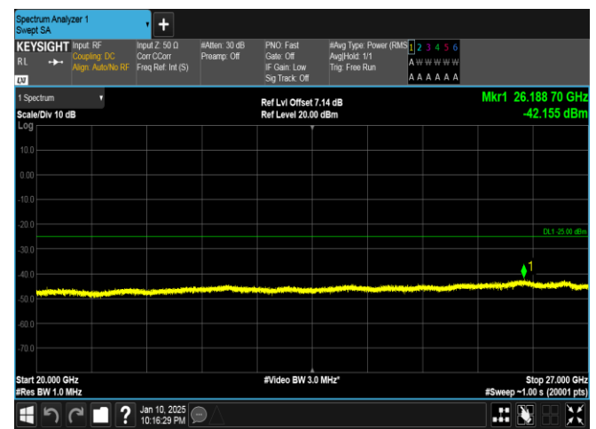
Band41-20MHz-16QAM-39750-100RB#0-20000~27000-PASS
