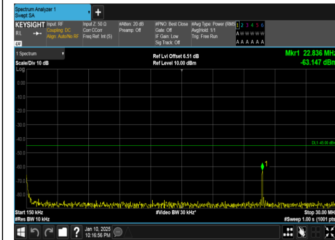
Band41-20MHz-QPSK-40620-1RB#0-0.15~30-PASS
