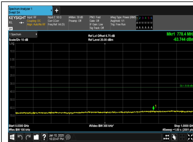
Band41-20MHz-QPSK-41490-1RB#0-30~1000-PASS
