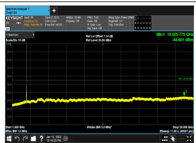
Band41-20MHz-QPSK-39750-1RB#0-1000~20000-PASS
