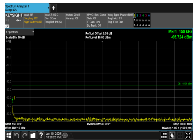
Band41-20MHz-QPSK-41490-100RB#0-0.15~30-PASS
