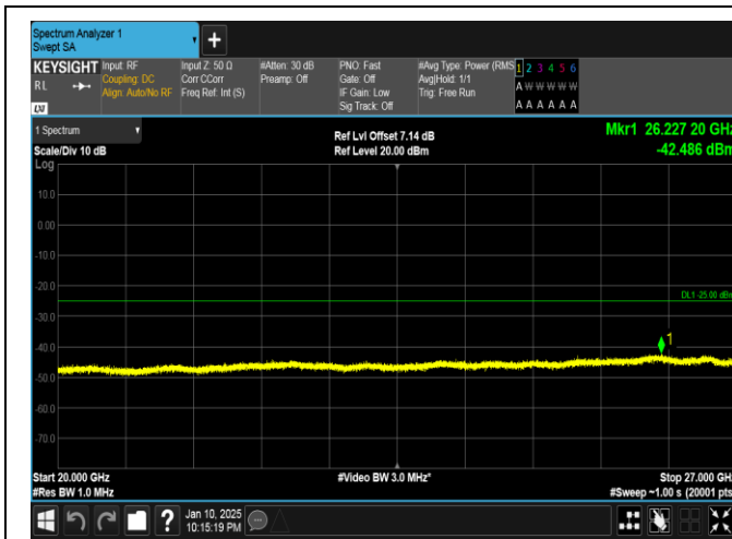
Band41-20MHz-QPSK-39750-100RB#0-20000~27000-PASS
