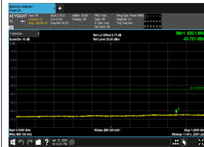
Band41-20MHz-16QAM-39750-1RB#99-30~1000-PASS
