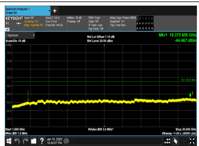
Band41-20MHz-QPSK-41490-1RB#0-1000~20000-PASS
