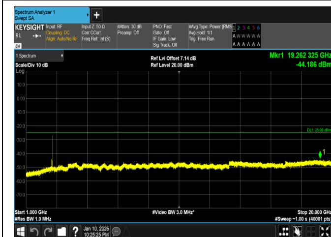
Band41-20MHz-16QAM-41490-1RB#0-1000~20000-PASS
