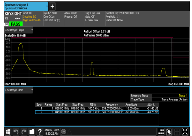
Band5-10MHz-QPSK-20600-1RB#0-PASS
