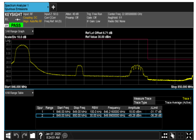
Band5-3MHz-QPSK-20635-1RB#0-PASS
