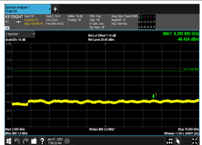
Band5-1.4MHz-QPSK-20525-1RB#0-3000~10000-PASS
