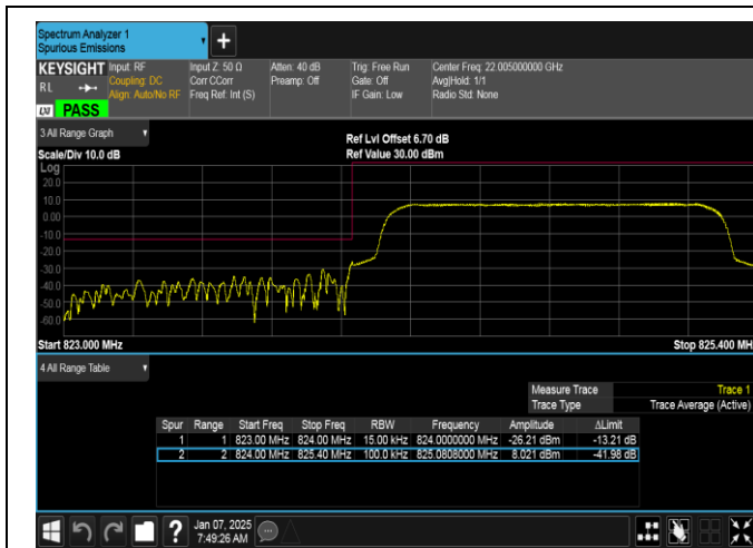
Band5-1.4MHz-16QAM-20407-6RB#0-PASS
