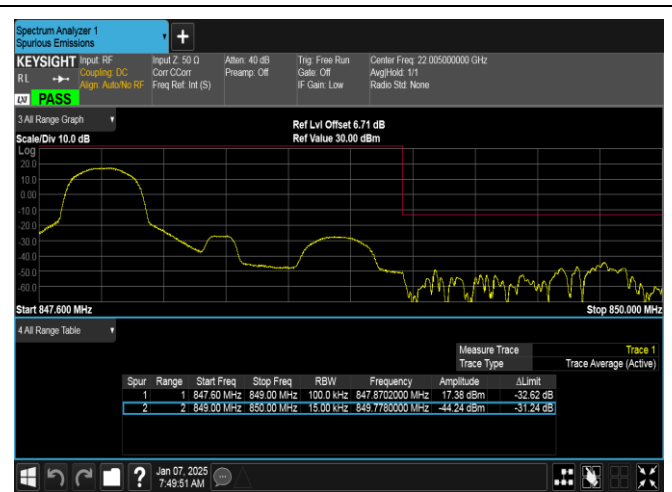
Band5-1.4MHz-16QAM-20643-1RB#0-PASS
