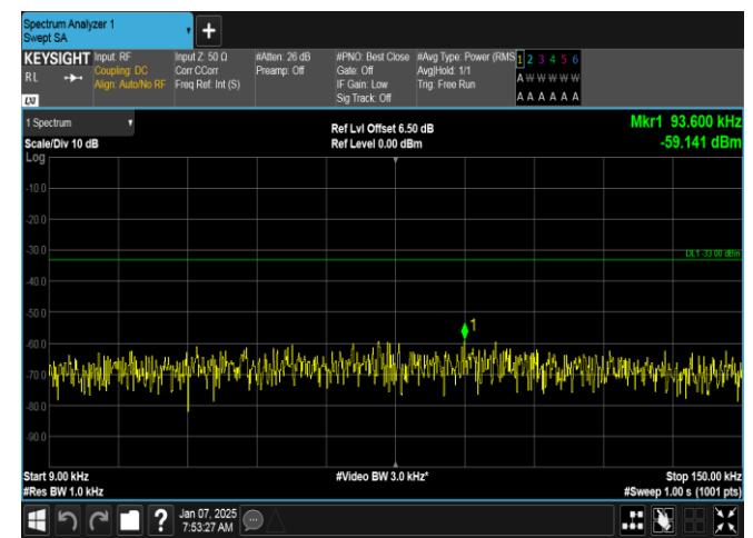
Band5-1.4MHz-QPSK-20407-1RB#5-0.009~0.15-PASS
