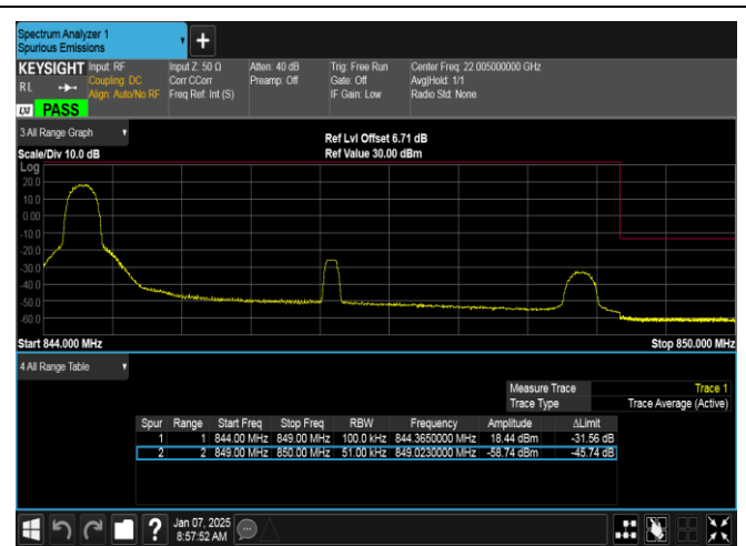
Band5-5MHz-QPSK-20625-1RB#0-PASS
