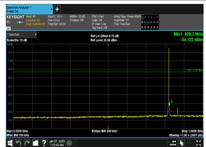
Band5-1.4MHz-QPSK-20407-1RB#5-30~1000-PASS
