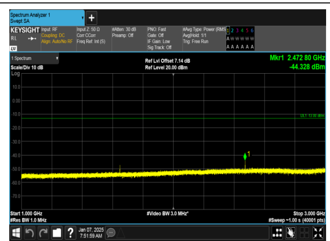
Band5-1.4MHz-QPSK-20407-1RB#0-1000~3000-PASS
