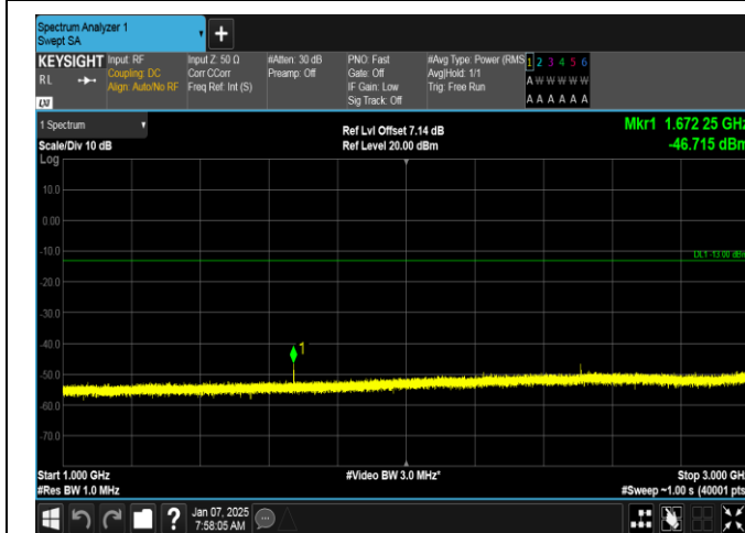
Band5-1.4MHz-QPSK-20525-1RB#0-1000~3000-PASS
