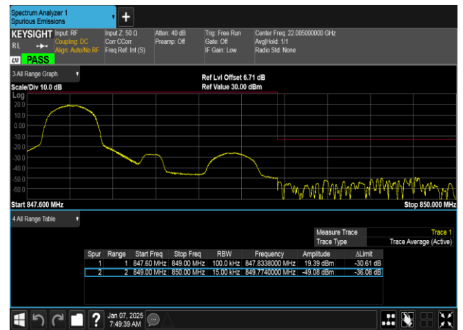
Band5-1.4MHz-QPSK-20643-1RB#0-PASS
