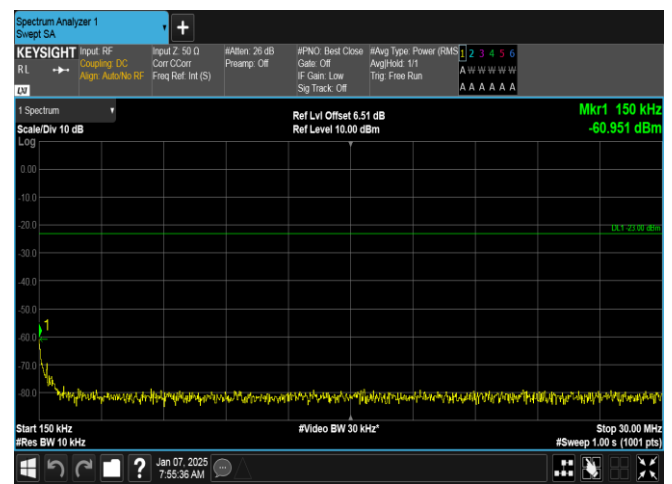
Band5-1.4MHz-QPSK-20407-6RB#0-0.15~30-PASS
