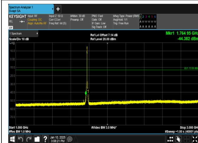
Band66-5MHz-16QAM-132647-25RB#0-1000~3000-PASS
