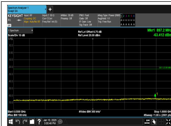
Band66-5MHz-16QAM-132322-25RB#0-30~1000-PASS
