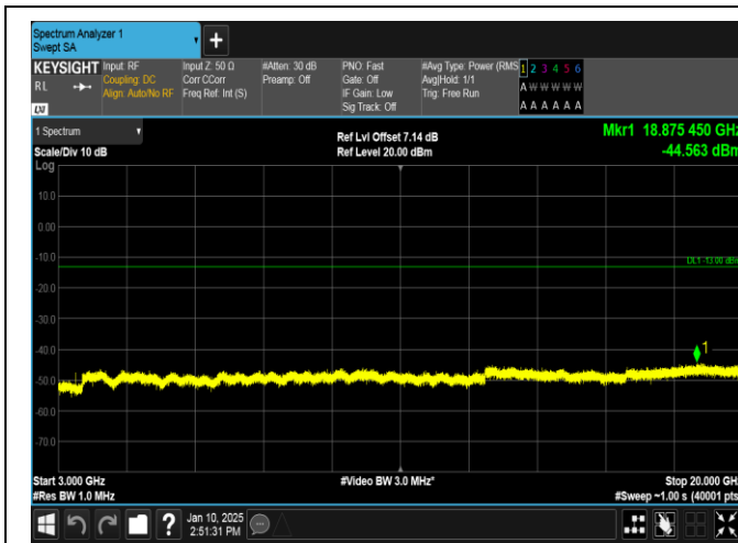
Band66-5MHz-16QAM-131997-1RB#24-3000~20000-PASS
