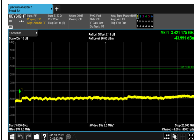
Band66-10MHz-QPSK-132022-1RB#0-3000~20000-PASS
