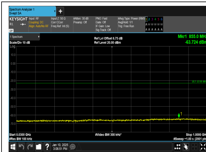
Band66-5MHz-QPSK-132647-25RB#0-30~1000-PASS
