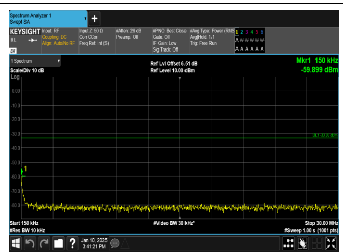
Band66-10MHz-QPSK-132022-1RB#0-0.15~30-PASS
