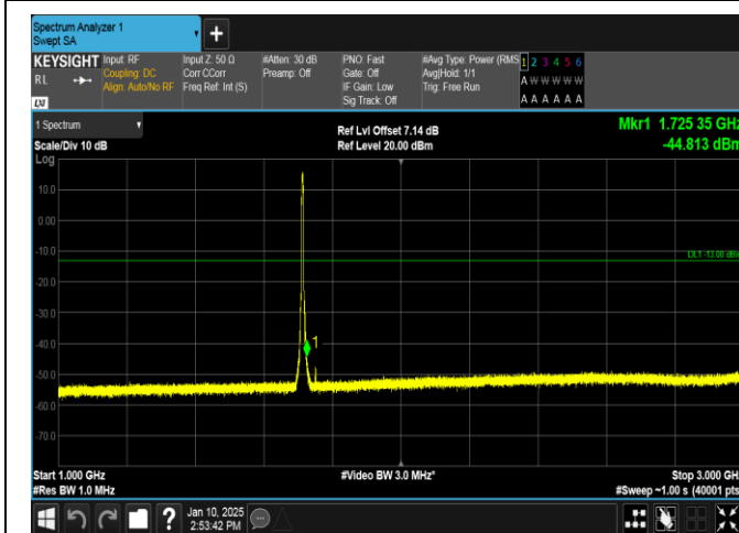
Band66-5MHz-16QAM-131997-25RB#0-1000~3000-PASS
