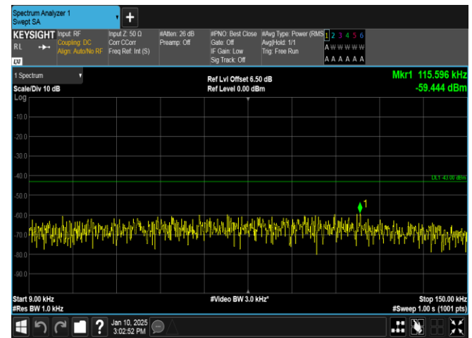
Band66-5MHz-16QAM-132647-1RB#0-0.009~0.15-PASS
