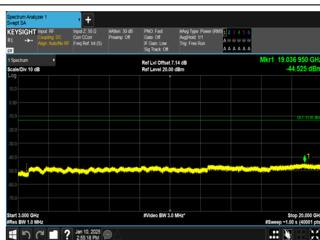
Band66-5MHz-OPSK-132322-1RB#0-3000~20000-PASS
