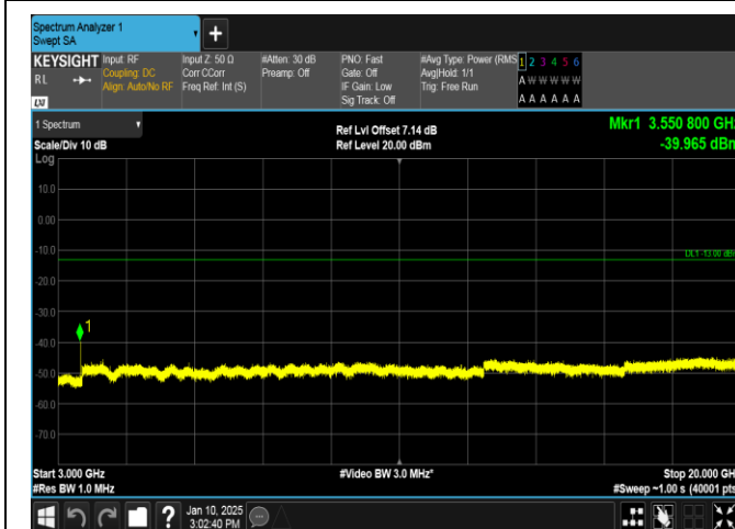
Band66-5MHz-QPSK-132647-1RB#0-3000~20000-PASS
