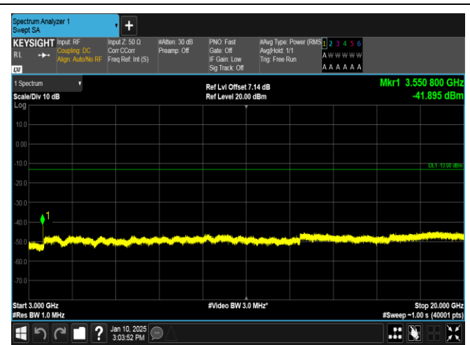
Band66-5MHz-16QAM-132647-1RB#0-3000~20000-PASS
