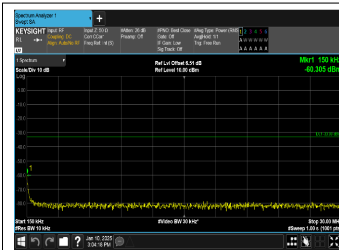
Band66-5MHz-QPSK-132647-1RB#24-0.15~30-PASS
