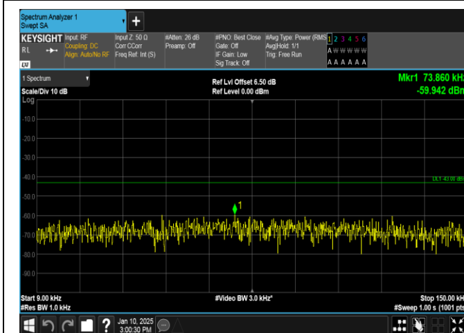
Band66-5MHz-16QAM-132322-25RB#0-0.009~0.15-PASS
