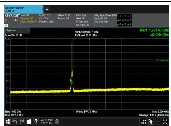
Band66-5MHz-QPSK-132647-25RB#0-1000~3000-PASS
