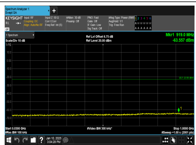
Band66-5MHz-QPSK-132647-1RB#24-30~1000-PASS
