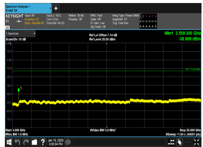
Band66-5MHz-QPSK-132647-1RB#24-3000~20000-PASS
