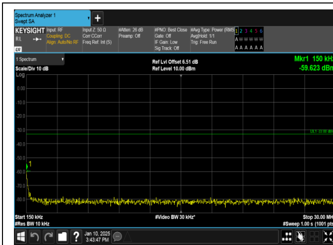
Band66-10MHz-QPSK-132022-1RB#49-0.15~30-PASS
