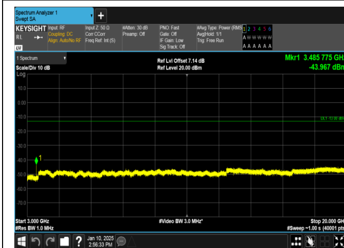
Band66-5MHz-16QAM-132322-1RB#0-3000~20000-PASS
