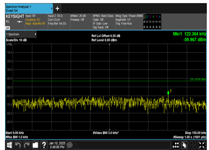
Band66-5MHz-16QAM-131997-1RB#0-0.009~0.15-PASS
