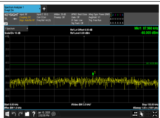
Band66-5MHz-16QAM-131997-25RB#0-0.009~0.15-PASS
