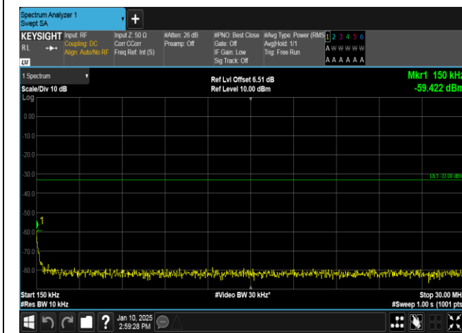
Band66-5MHz-QPSK-132322-25RB#0-0.15~30-PASS
