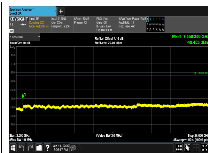
Band66-5MHz-16QAM-132647-1RB#24-3000~20000-PASS
