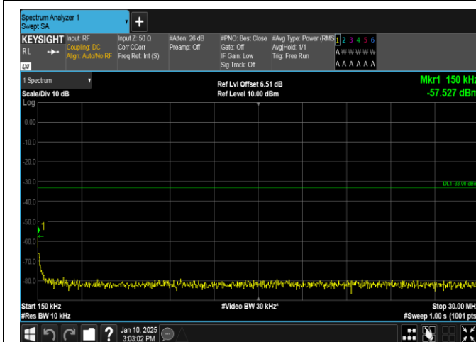
Band66-5MHz-16QAM-132647-1RB#0-0.15~30-PASS
