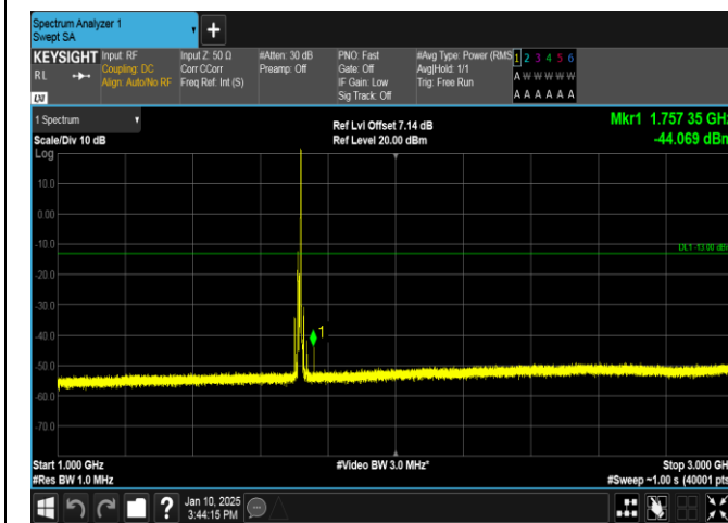
Band66-10MHz-QPSK-132022-1RB#49-1000~3000-PASS
