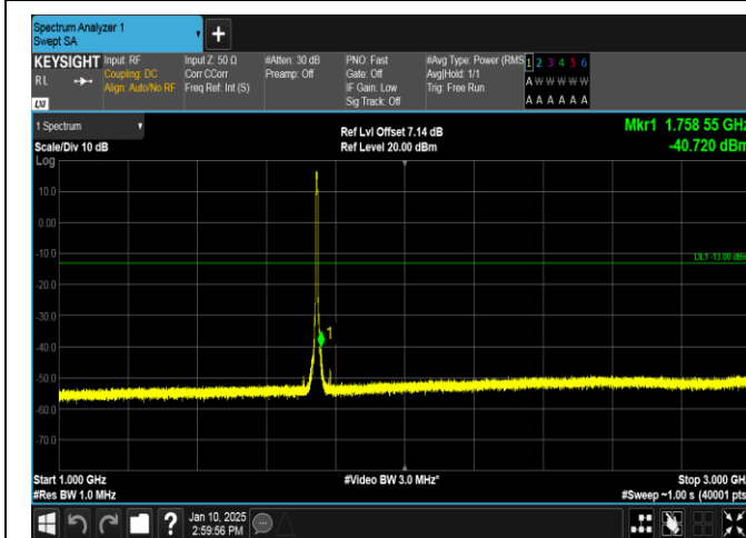
Band66-5MHz-QPSK-132322-25RB#0-1000~3000-PASS
