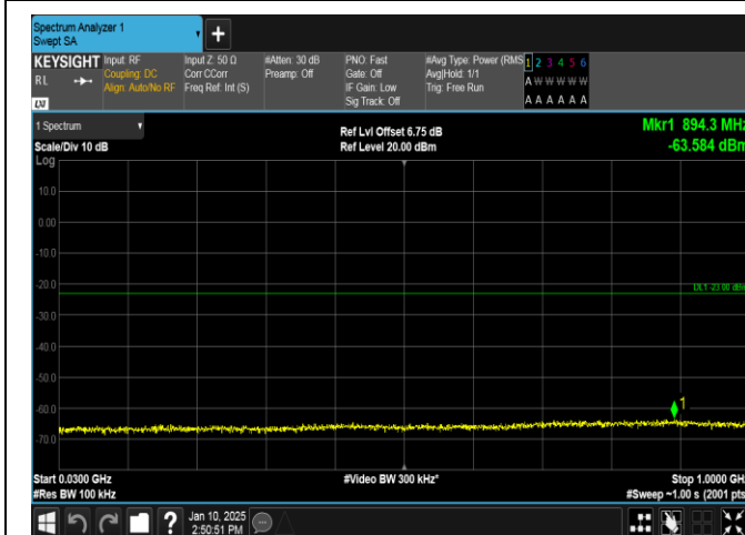
Band66-5MHz-16QAM-131997-1RB#24-30~1000-PASS
