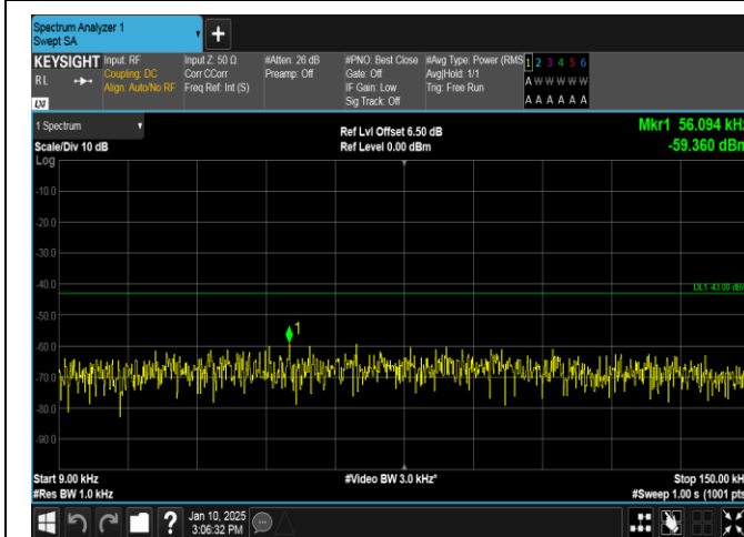
Band66-5MHz-QPSK-132647-25RB#0-0.009~0.15-PASS
