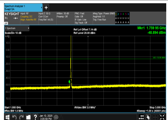
Band66-5MHz-16QAM-132647-1RB#24-1000~3000-PASS
