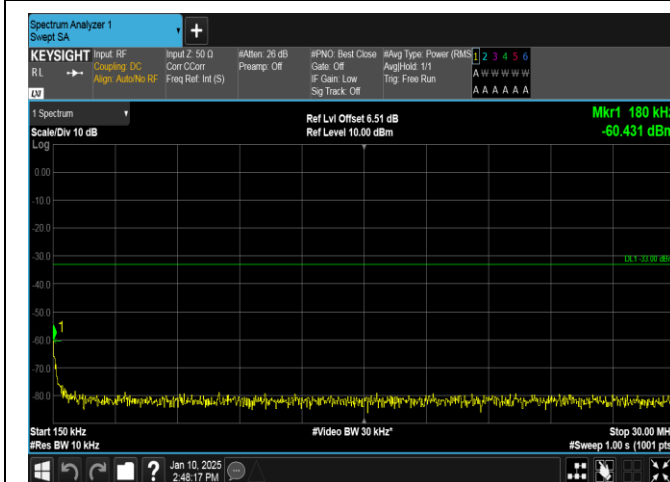
Band66-5MHz-16QAM-131997-1RB#0-0.15~30-PASS
