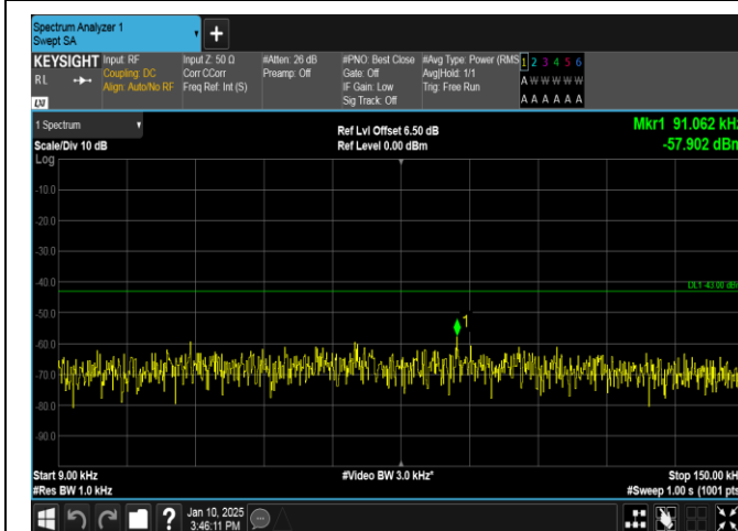
Band66-10MHz-QPSK-132022-50RB#0-0.009~0.15-PASS
