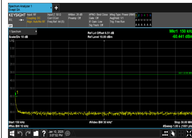
Band66-5MHz-16QAM-132647-25RB#0-0.15~30-PASS
