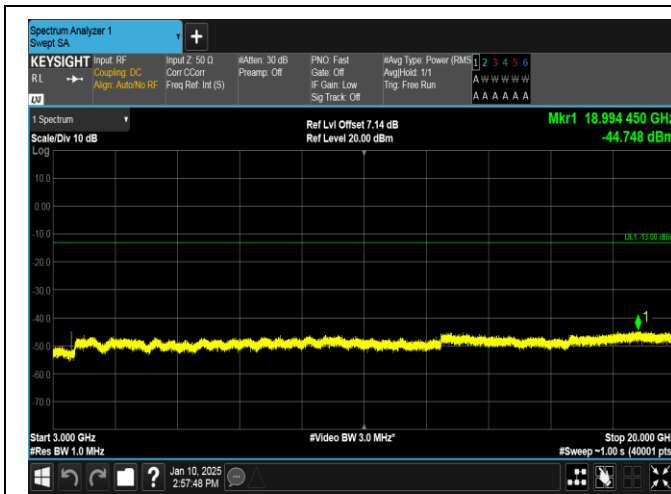
Band66-5MHz-QPSK-132322-1RB#24-3000~20000-PASS
