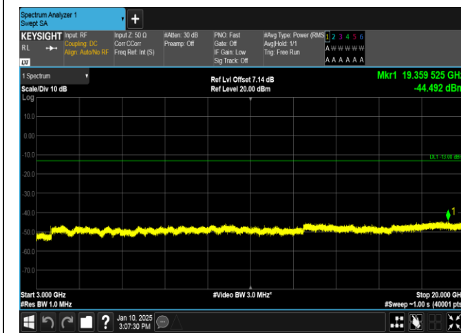
Band66-5MHz-QPSK-132647-25RB#0-3000~20000-PASS
