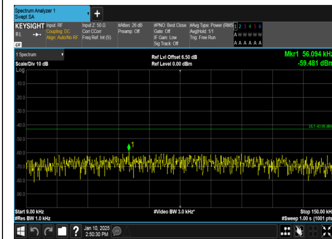
Band66-5MHz-16QAM-131997-1RB#24-0.009~0.15-PASS
