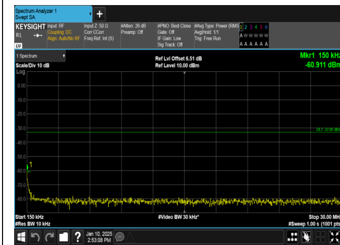
Band66-5MHz-16QAM-131997-25RB#0-0.15~30-PASS
