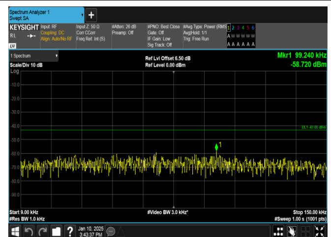
Band66-10MHz-QPSK-132022-1RB#49-0.009~0.15-PASS
