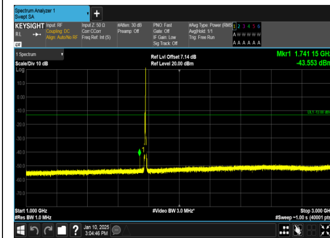
Band66-5MHz-QPSK-132647-1RB#24-1000~3000-PASS
