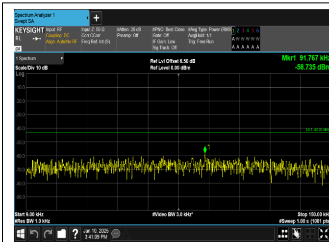
Band66-10MHz-QPSK-132022-1RB#0-0.009~0.15-PASS
