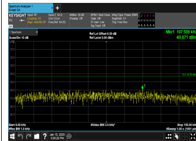
Band66-5MHz-16QAM-132647-1RB#24-0.009~0.15-PASS
