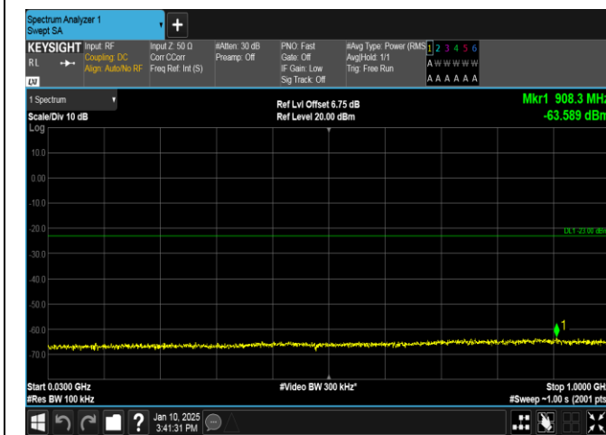
Band66-10MHz-QPSK-132022-1RB#0-30~1000-PASS
