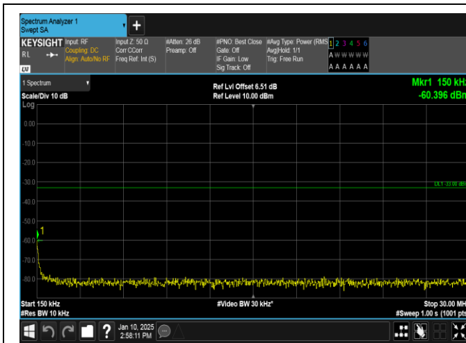
Band66-5MHz-16QAM-132322-1RB#24-0.15~30-PASS
