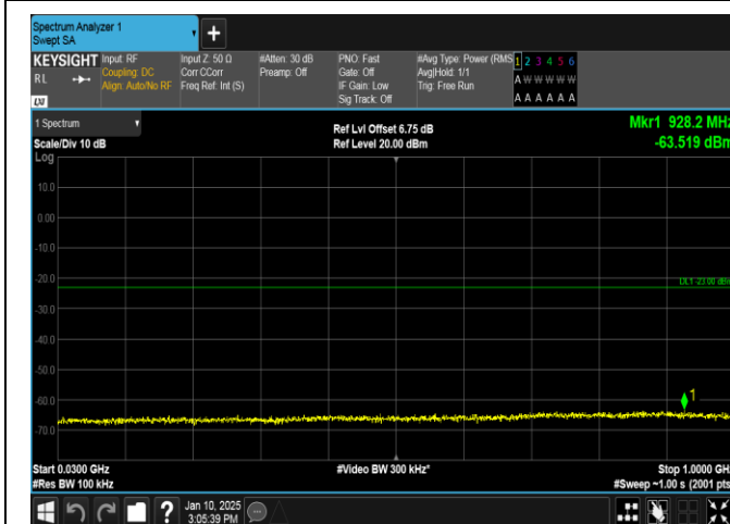
Band66-5MHz-16QAM-132647-1RB#24-30~1000-PASS
