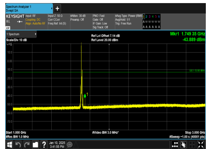
Band66-10MHz-QPSK-132022-1RB#0-1000~3000-PASS
