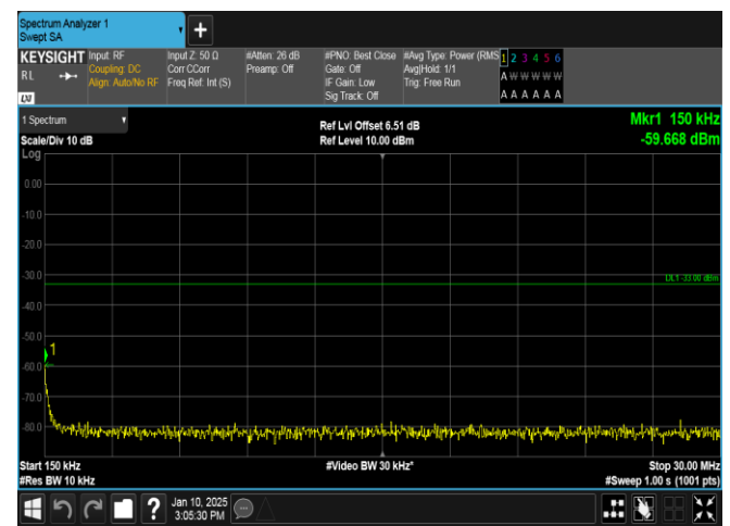
Band66-5MHz-16QAM-132647-1RB#24-0.15~30-PASS
