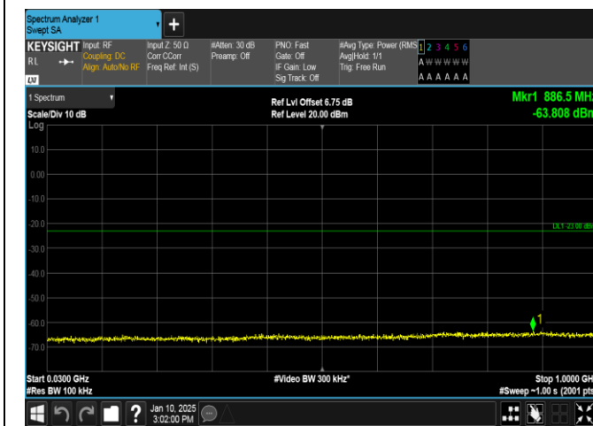
Band66-5MHz-QPSK-132647-1RB#0-30~1000-PASS
