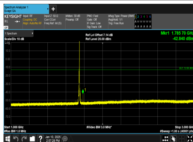
Band66-5MHz-QPSK-132322-1RB#24-1000~3000-PASS
