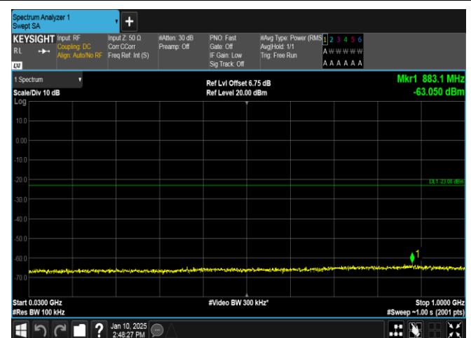
Band66-5MHz-16QAM-131997-1RB#0-30~1000-PASS
