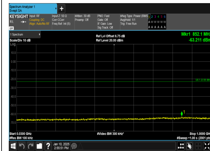
Band66-5MHz-16QAM-132322-1RB#0-30~1000-PASS
