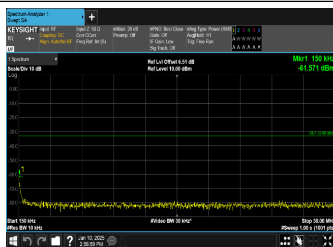
Band66-5MHz-QPSK-132322-1RB#24-0.15~30-PASS
