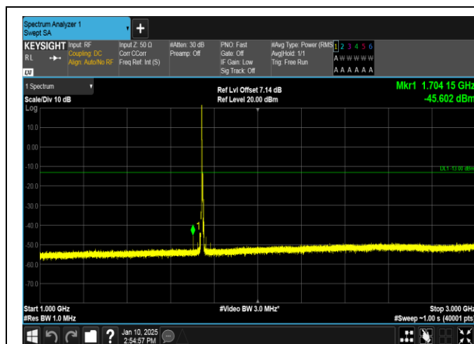
Band66-5MHz-OPSK-132322-1RB#0-1000~3000-PASS
