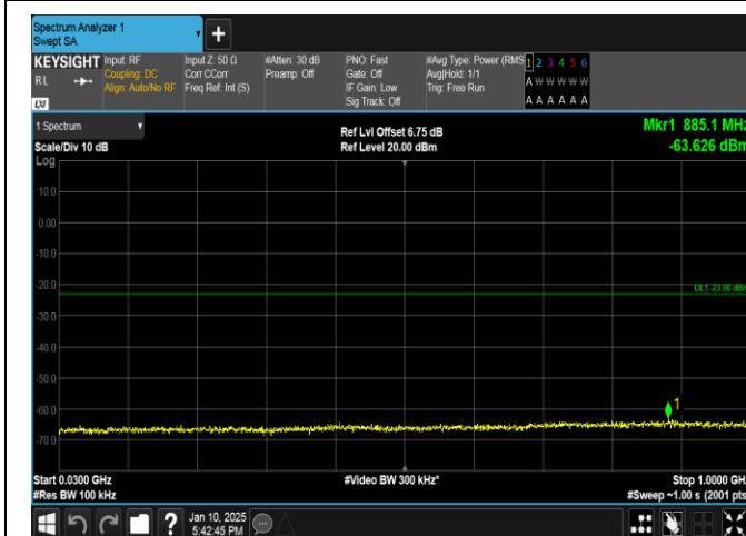
Band66-20MHz-QPSK-132322-1RB#99-30~1000-PASS
