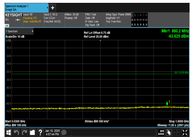
Band66-15MHz-16QAM-132597-75RB#0-30~1000-PASS
