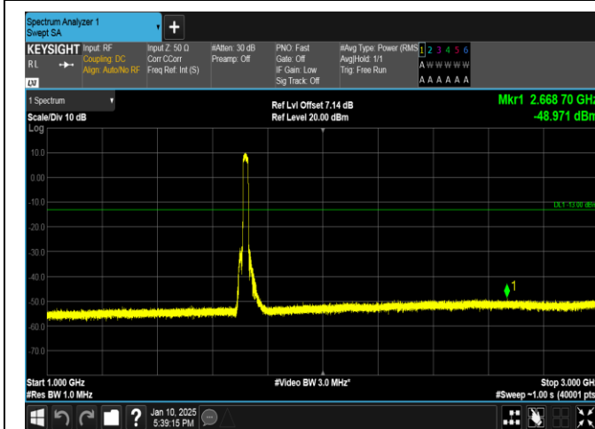
Band66-20MHz-16QAM-132072-100RB#0-1000~3000-PASS
