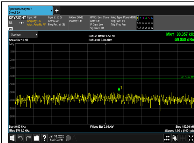
Band66-20MHz-QPSK-132072-1RB#0-0.009~0.15-PASS
