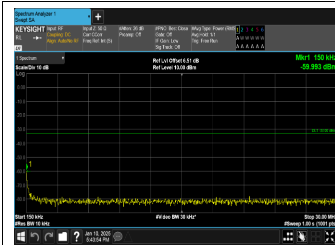
Band66-20MHz-16QAM-132322-1RB#99-0.15~30-PASS
