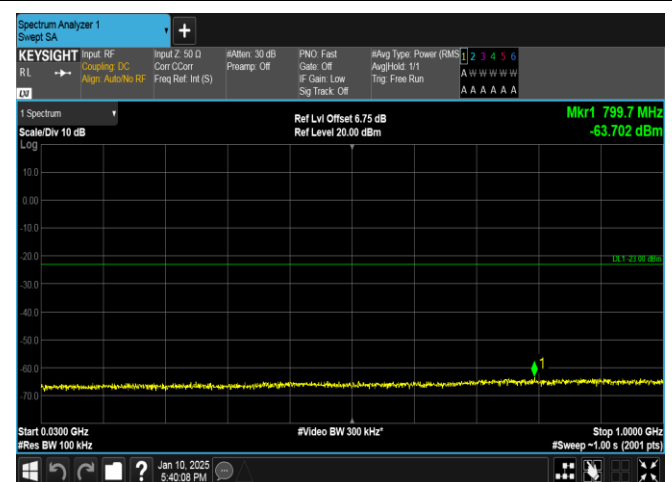
Band66-20MHz-QPSK-132322-1RB#0-30~1000-PASS
