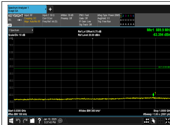
Band66-20MHz-QPSK-132072-100RB#0-30~1000-PASS
