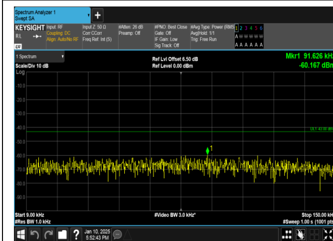
Band66-20MHz-QPSK-132572-100RB#0-0.009~0.15-PASS
