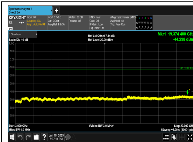
Band66-20MHz-16QAM-132072-1RB#99-3000~20000-PASS
