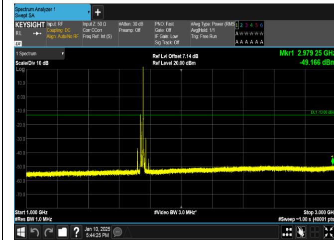
Band66-20MHz-16QAM-132322-1RB#99-1000~3000-PASS
