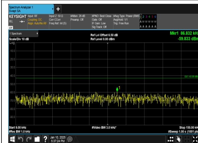
Band66-20MHz-QPSK-132072-100RB#0-0.009~0.15-PASS
