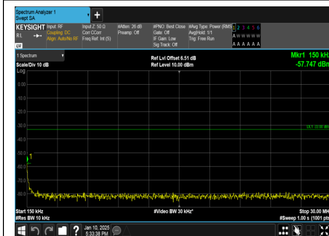
Band66-20MHz-16QAM-132072-1RB#0-0.15~30-PASS
