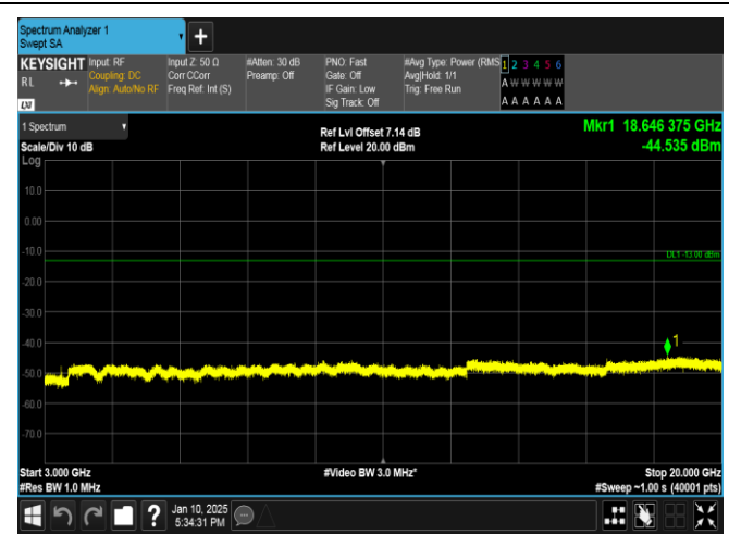
Band66-20MHz-16QAM-132072-1RB#0-3000~20000-PASS
