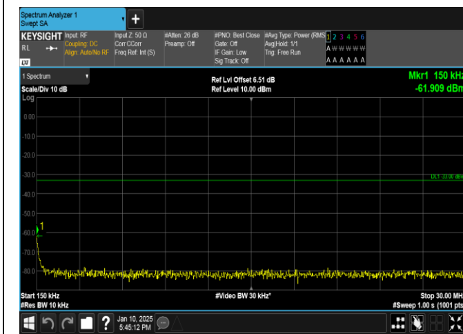
Band66-20MHz-QPSK-132322-100RB#0-0.15~30-PASS
