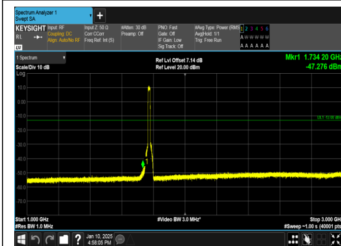
Band66-15MHz-16QAM-132597-75RB#0-1000~3000-PASS
