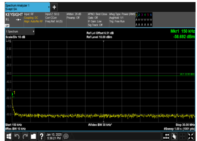
Band66-20MHz-16QAM-132072-1RB#99-0.15~30-PASS
