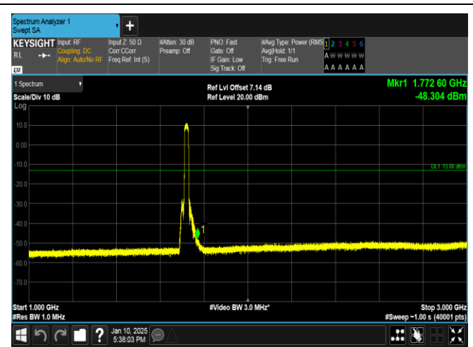
Band66-20MHz-QPSK-132072-100RB#0-1000~3000-PASS
