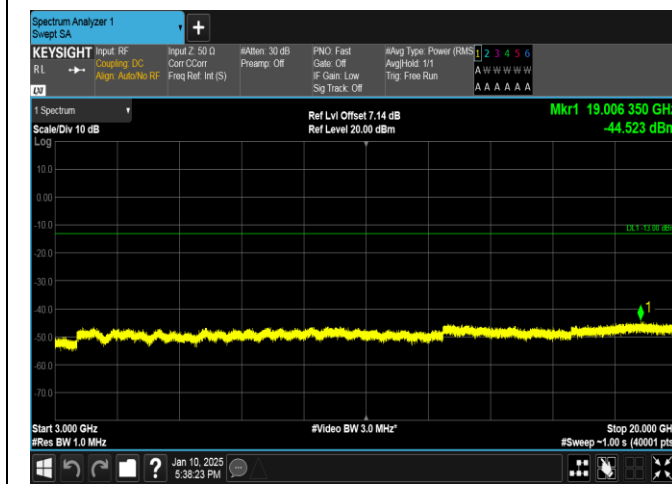
Band66-20MHz-QPSK-132072-100RB#0-3000~20000-PASS
