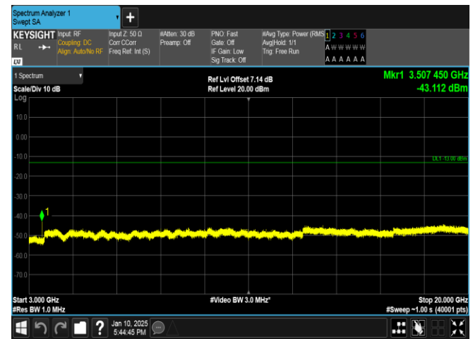
Band66-20MHz-16QAM-132322-1RB#99-3000~20000-PASS
