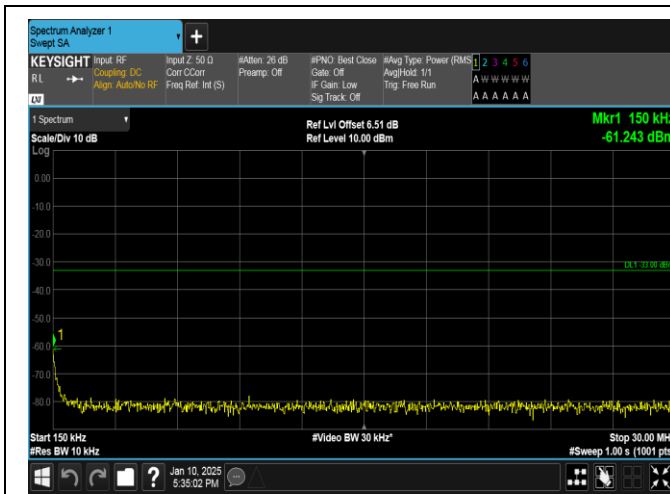
Band66-20MHz-QPSK-132072-1RB#99-0.15~30-PASS
