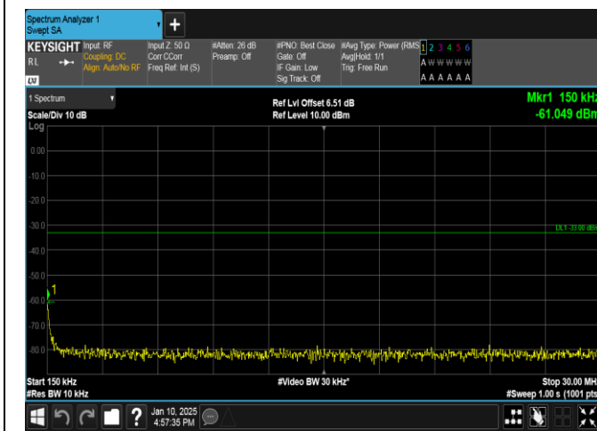
Band66-15MHz-16QAM-132597-75RB#0-0.15~30-PASS
