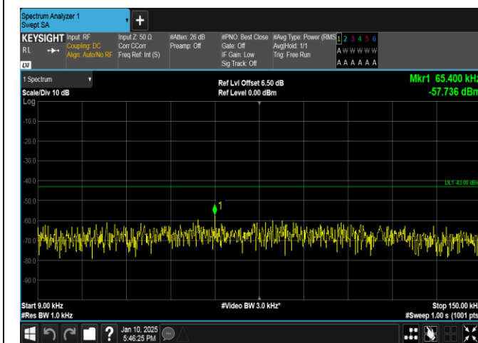
Band66-20MHz-16QAM-132322-100RB#0-0.009~0.15-PASS
