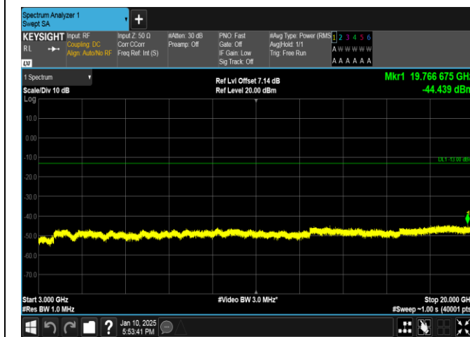
Band66-20MHz-QPSK-132572-100RB#0-3000~20000-PASS
