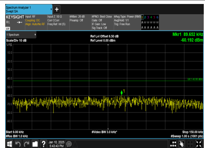
Band66-20MHz-16QAM-132322-1RB#99-0.009~0.15-PASS
