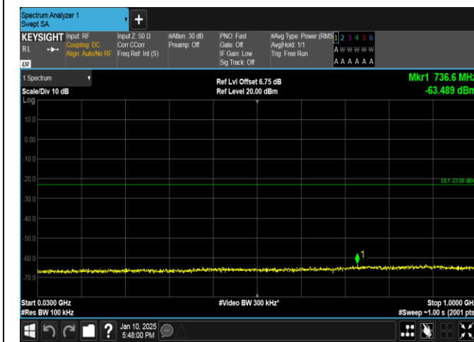
Band66-20MHz-QPSK-132572-1RB#0-30~1000-PASS
