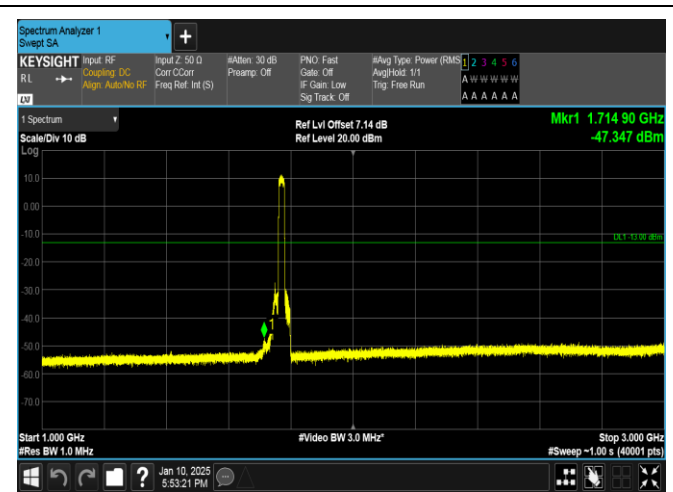
Band66-20MHz-QPSK-132572-100RB#0-1000~3000-PASS
