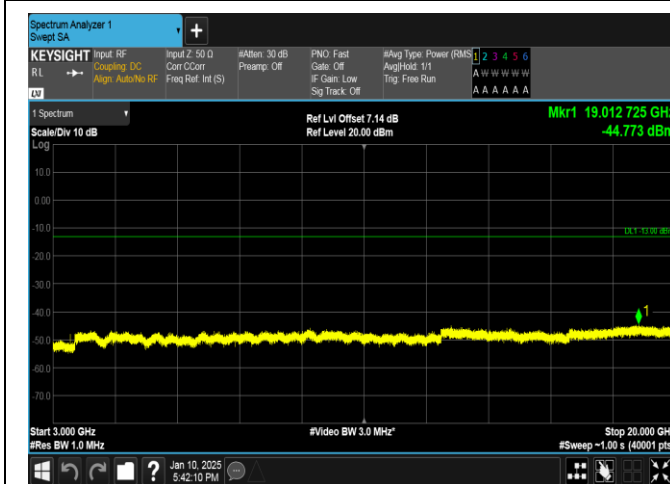
Band66-20MHz-16QAM-132322-1RB#0-3000~20000-PASS
