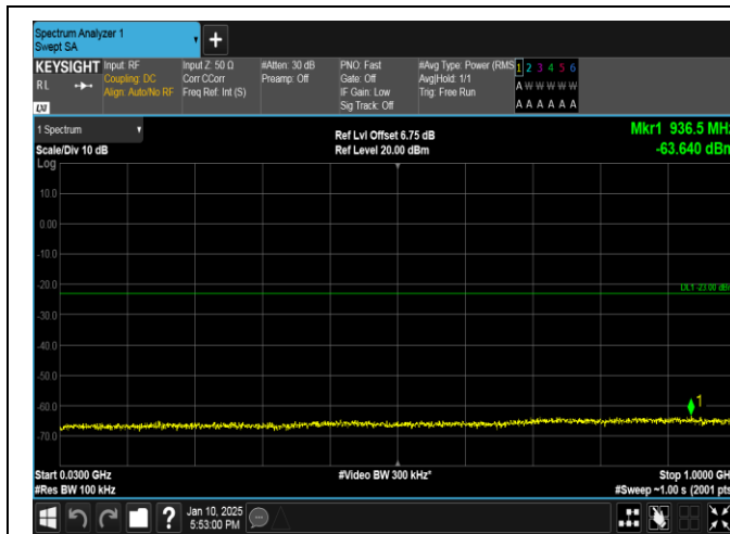
Band66-20MHz-QPSK-132572-100RB#0-30~1000-PASS
