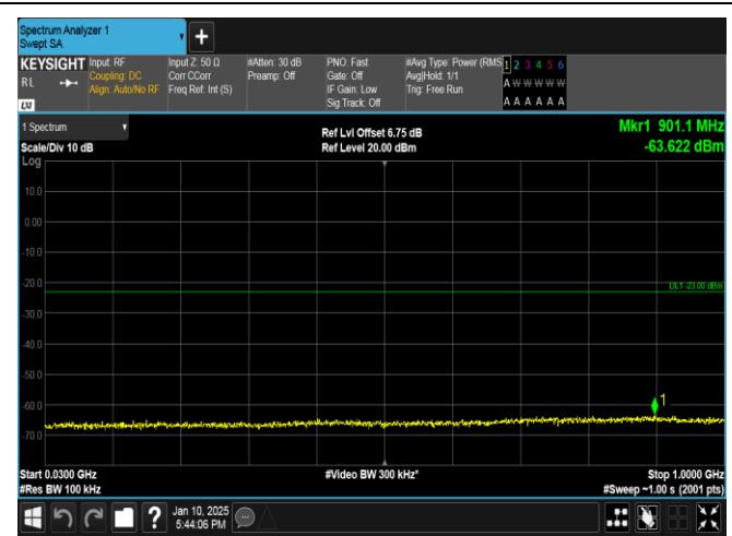
Band66-20MHz-16QAM-132322-1RB#99-30~1000-PASS
