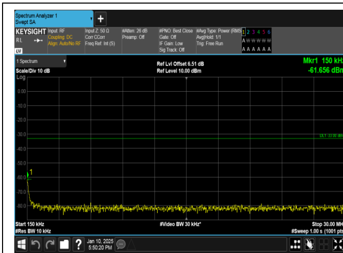
Band66-20MHz-QPSK-132572-1RB#99-0.15~30-PASS
