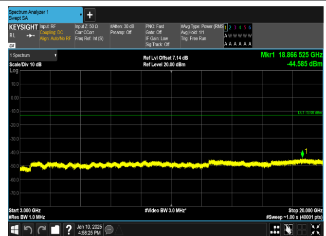
Band66-15MHz-16QAM-132597-75RB#0-3000~20000-PASS
