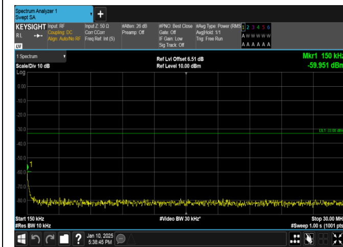
Band66-20MHz-16QAM-132072-100RB#0-0.15~30-PASS
