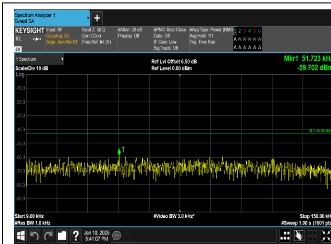
Band66-20MHz-16QAM-132322-1RB#0-0.009~0.15-PASS
