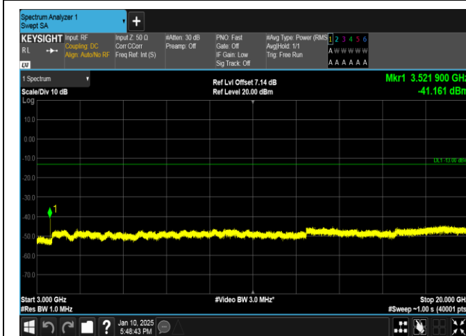
Band66-20MHz-QPSK-132572-1RB#0-3000~20000-PASS
