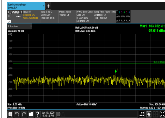
Band66-20MHz-16QAM-132072-1RB#99-0.009~0.15-PASS
