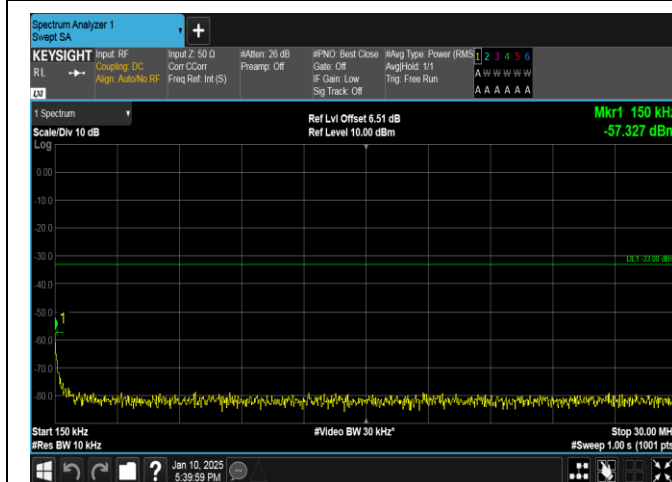
Band66-20MHz-QPSK-132322-1RB#0-0.15~30-PASS
