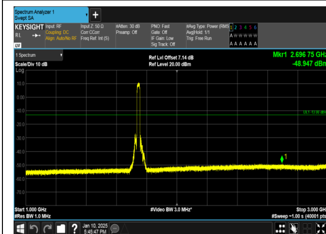
Band66-20MHz-QPSK-132322-100RB#0-1000~3000-PASS
