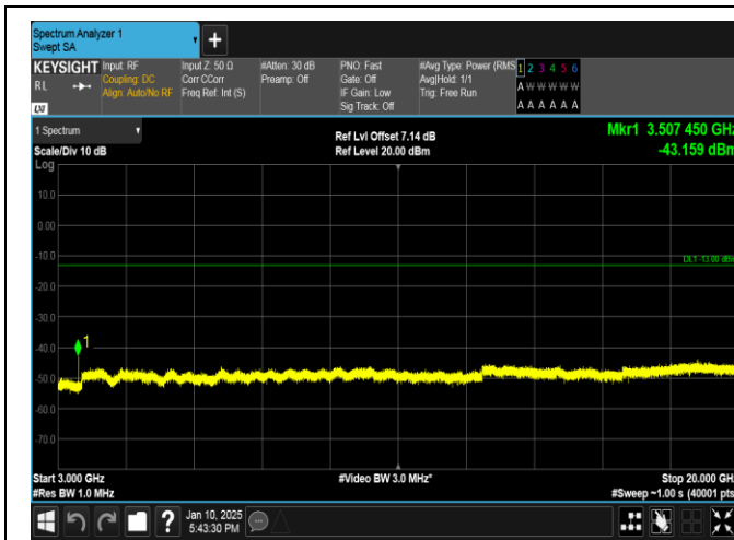
Band66-20MHz-QPSK-132322-1RB#99-3000~20000-PASS
