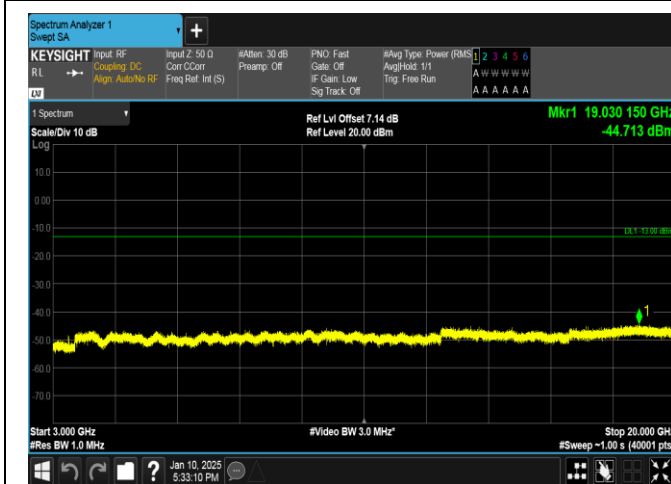
Band66-20MHz-QPSK-132072-1RB#0-3000~20000-PASS
