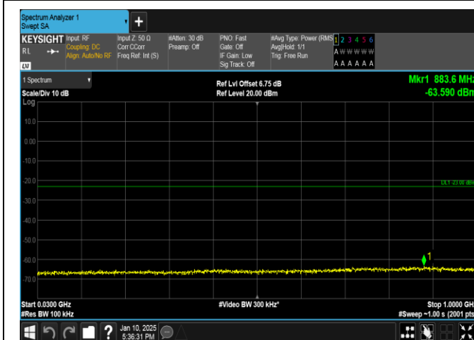
Band66-20MHz-16QAM-132072-1RB#99-30~1000-PASS
