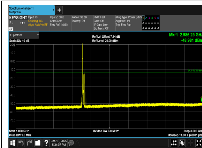
Band66-20MHz-16QAM-132072-1RB#0-1000~3000-PASS
