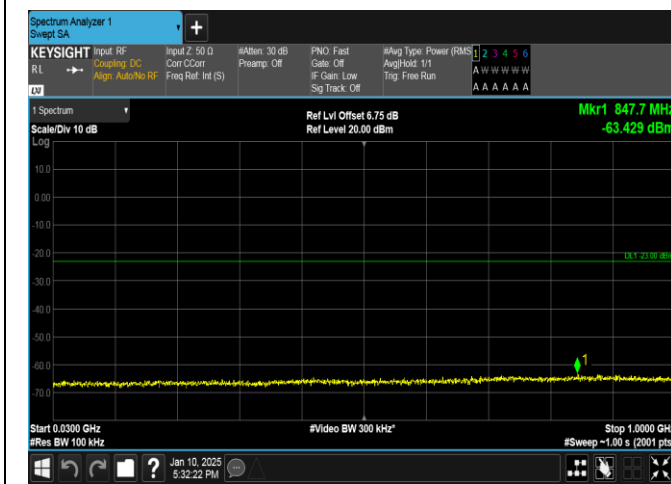
Band66-20MHz-QPSK-132072-1RB#0-30~1000-PASS
