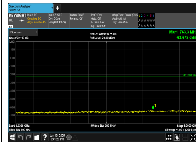
Band66-20MHz-16QAM-132322-1RB#0-30~1000-PASS
