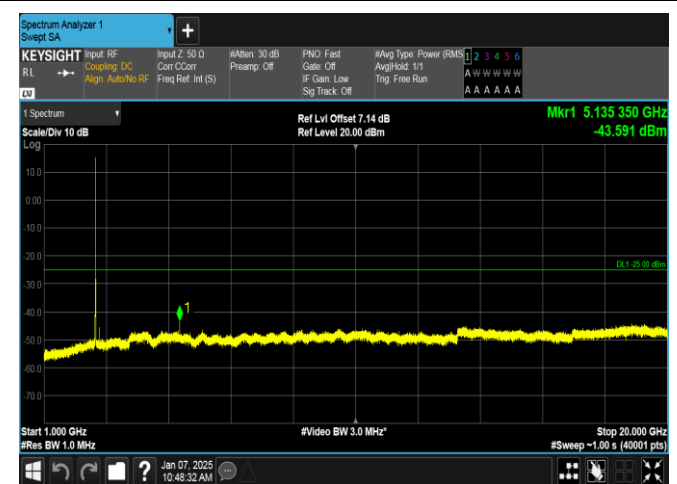
Band7-5MHz-QPSK-21425-25RB#0-1000~20000-PASS
