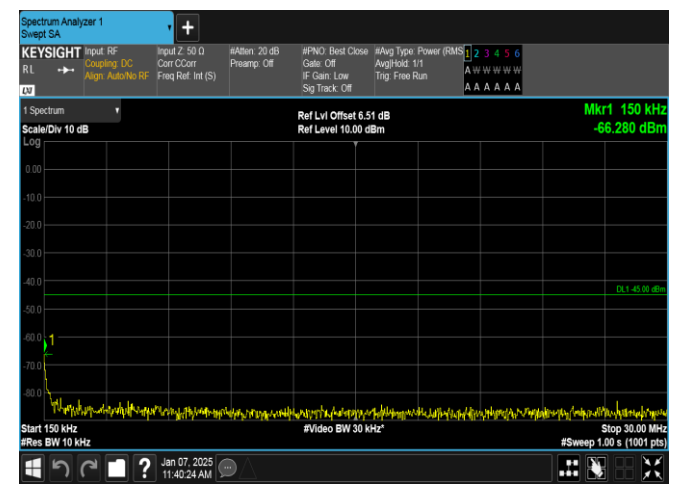
Band7-10MHz-QPSK-20800-50RB#0-0.15~30-PASS
