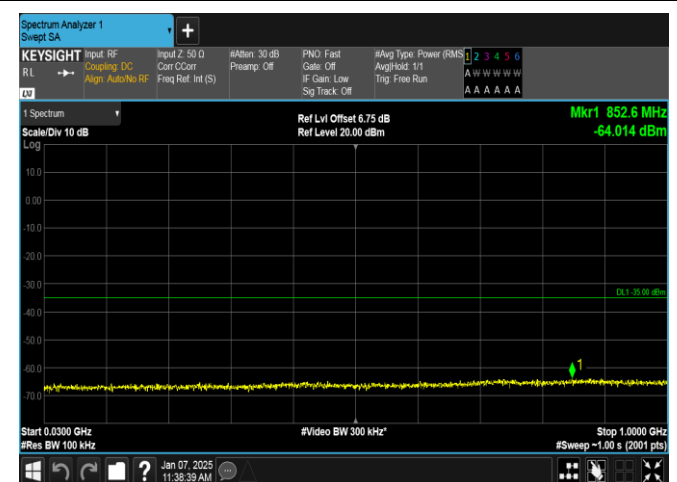
Band7-10MHz-QPSK-20800-1RB#49-30~1000-PASS
