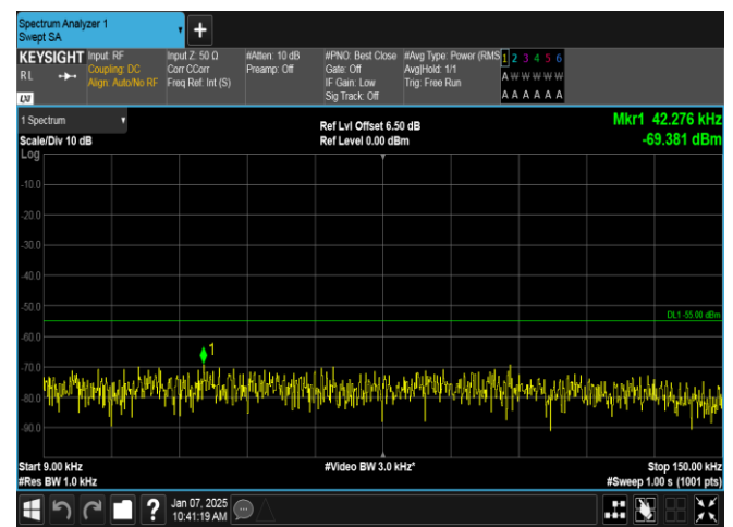
Band7-5MHz-16QAM-21100-1RB#24-0.009~0.15-PASS
