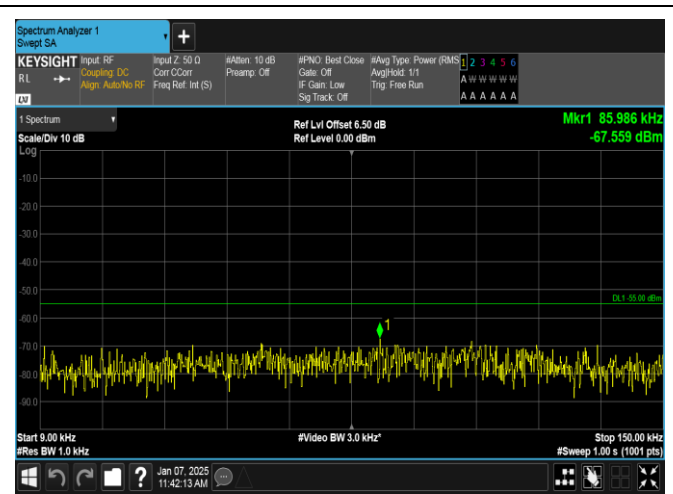
Band7-10MHz-QPSK-21100-1RB#0-0.009~0.15-PASS
