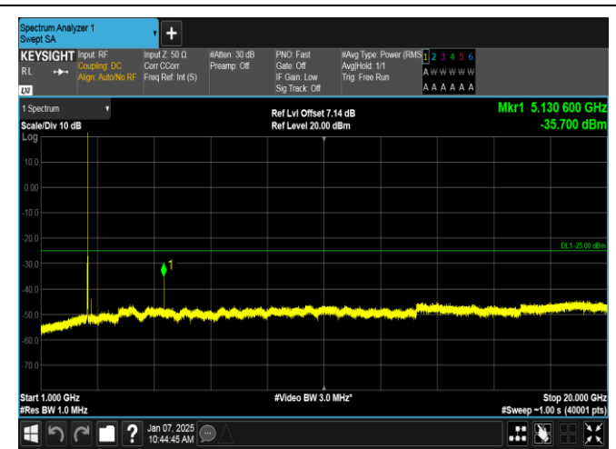
Band7-5MHz-QPSK-21425-1RB#0-1000~20000-PASS
