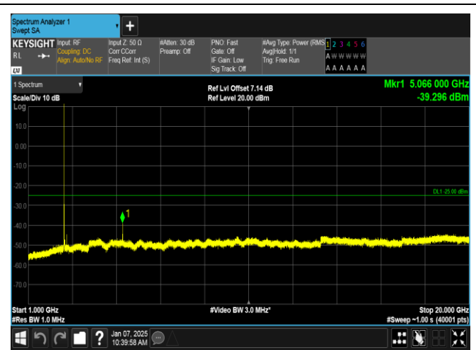
Band7-5MHz-16QAM-21100-1RB#0-1000~20000-PASS
