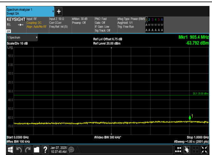
Band7-5MHz-16QAM-20775-25RB#0-30~1000-PASS
