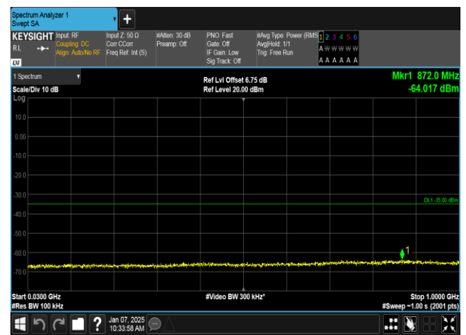
Band7-5MHz-16QAM-20775-1RB#0-30~1000-PASS
