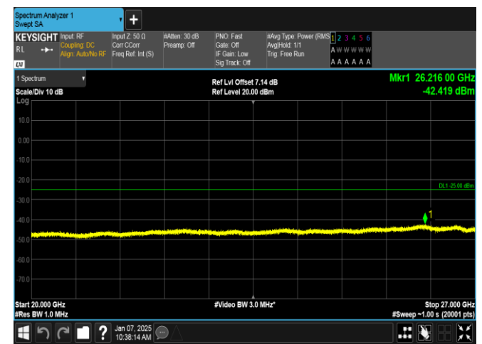
Band7-5MHz-16QAM-20775-25RB#0-20000~27000-PASS
