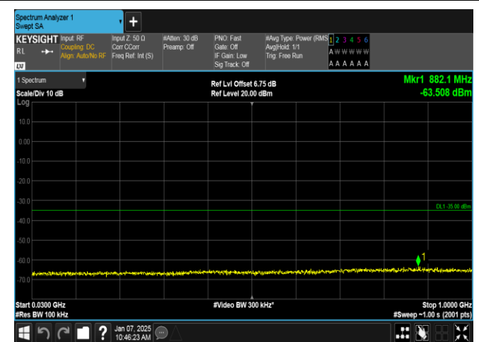
Band7-5MHz-QPSK-21425-1RB#24-30~1000-PASS
