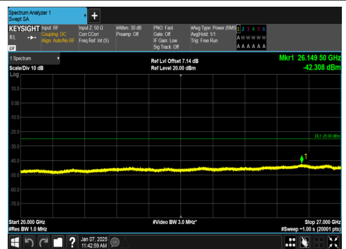
Band7-10MHz-QPSK-21100-1RB#0-20000~27000-PASS
