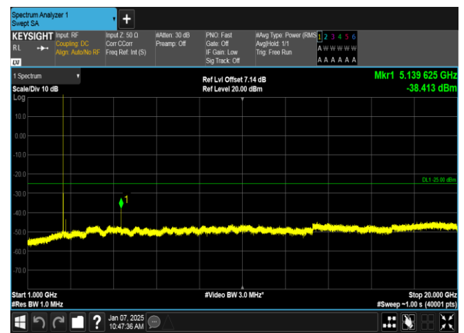
Band7-5MHz-16QAM-21425-1RB#24-1000~20000-PASS
