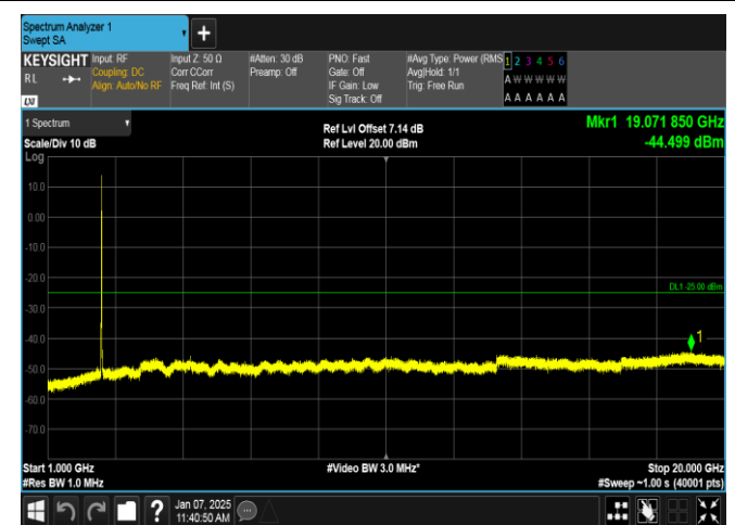
Band7-10MHz-QPSK-20800-50RB#0-1000~20000-PASS
