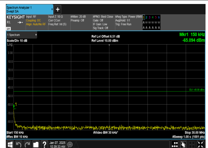
Band7-5MHz-16QAM-21100-1RB#0-0.15~30-PASS
