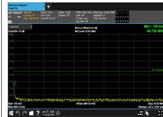
Band7-10MHz-QPSK-21100-1RB#0-0.15~30-PASS
