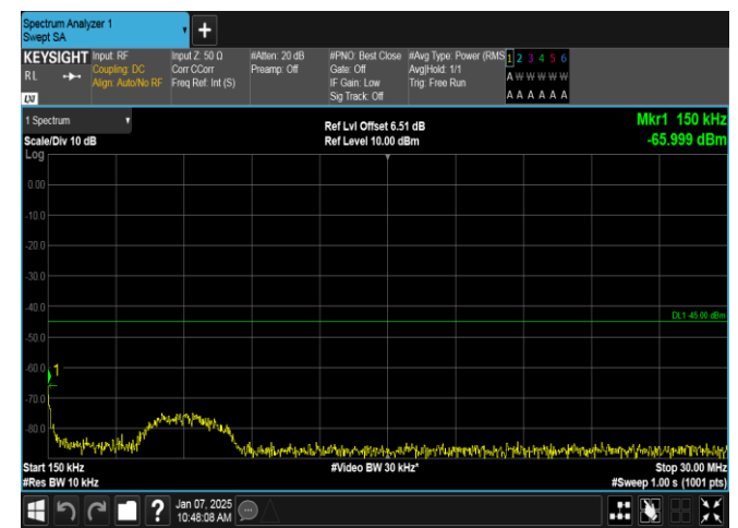
Band7-5MHz-QPSK-21425-25RB#0-0.15~30-PASS
