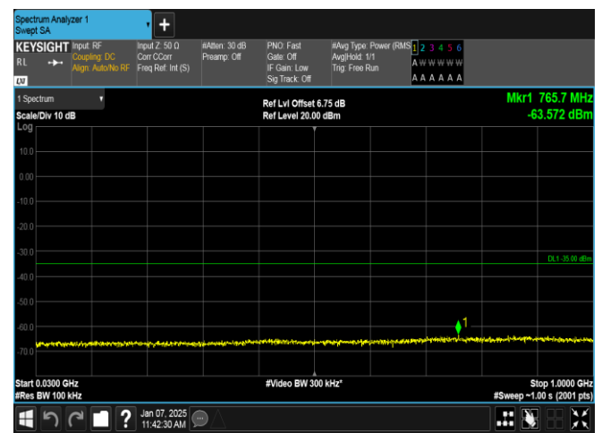
Band7-10MHz-QPSK-21100-1RB#0-30~1000-PASS
