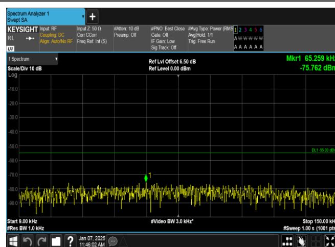
Band7-10MHz-QPSK-21100-50RB#0-0.009~0.15-PASS
