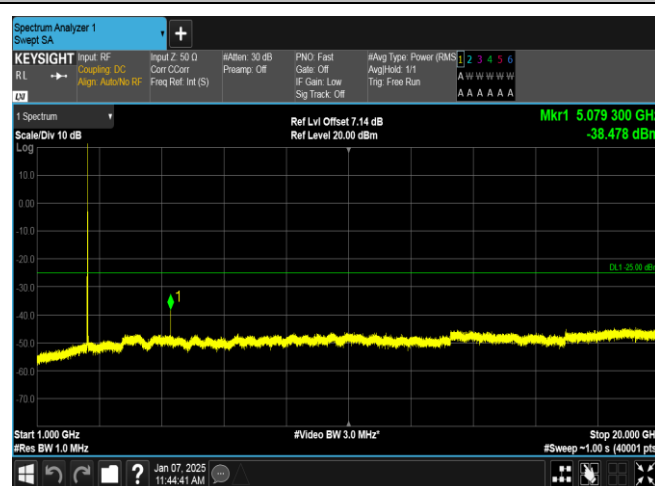
Band7-10MHz-QPSK-21100-1RB#49-1000~20000-PASS
