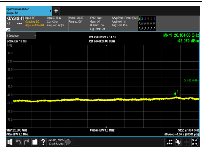
Band7-5MHz-QPSK-21425-1RB#24-20000~27000-PASS
