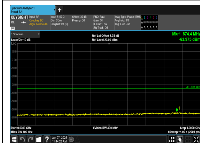
Band7-10MHz-QPSK-21100-1RB#49-30~1000-PASS
