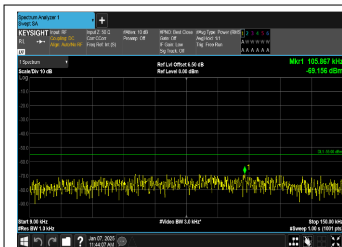
Band7-10MHz-QPSK-21100-1RB#49-0.009~0.15-PASS
