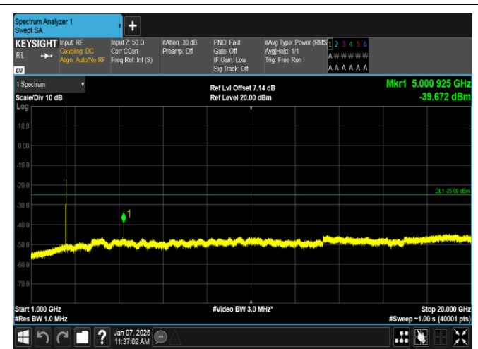
Band7-10MHz-QPSK-20800-1RB#0-1000~20000-PASS
