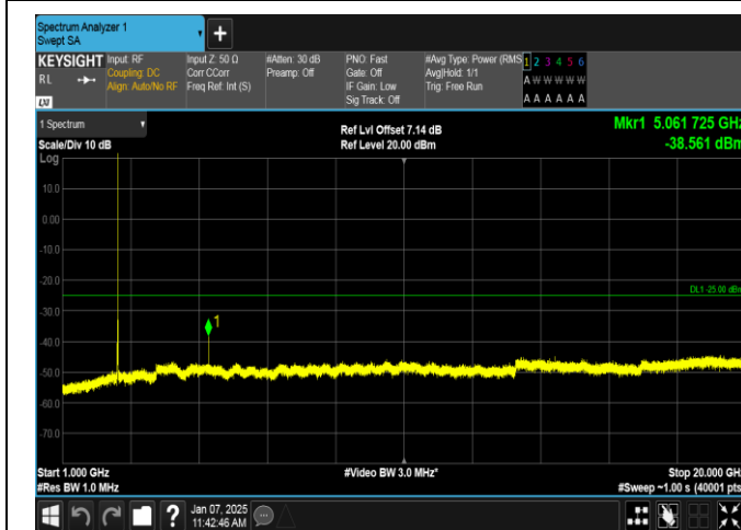
Band7-10MHz-QPSK-21100-1RB#0-1000~20000-PASS
