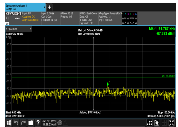
Band7-10MHz-QPSK-20800-1RB#49-0.009~0.15-PASS
