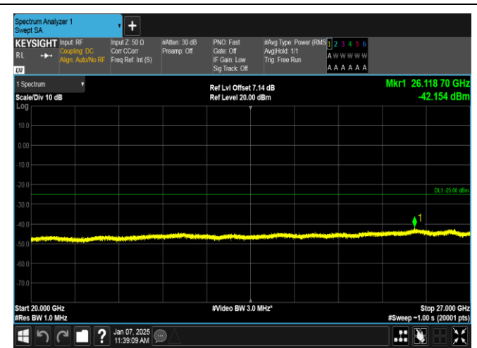
Band7-10MHz-QPSK-20800-1RB#49-20000~27000-PASS
