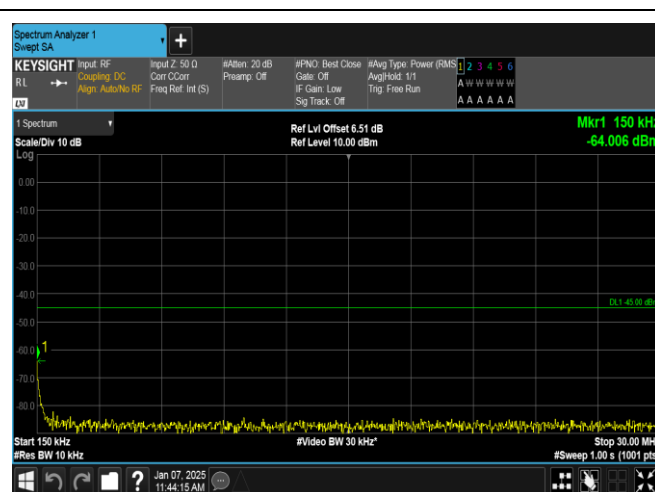
Band7-10MHz-QPSK-21100-1RB#49-0.15~30-PASS
