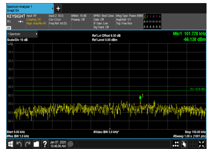
Band7-5MHz-QPSK-21425-1RB#24-0.009~0.15-PASS
