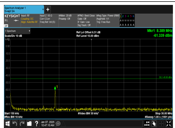
Band7-5MHz-16QAM-21425-1RB#24-0.15~30-PASS
