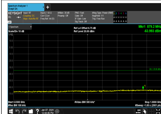
Band7-15MHz-QPSK-20825-75RB#0-30~1000-PASS
