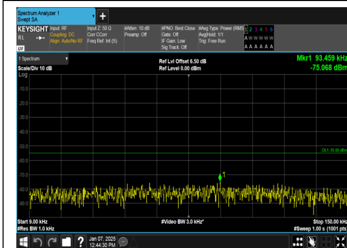
Band7-15MHz-QPSK-20825-75RB#0-0.009~0.15-PASS
