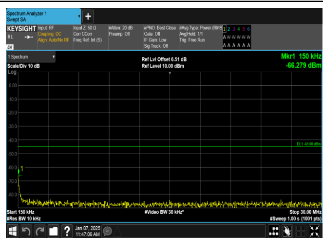
Band7-10MHz-16OAM-21100-50RB#0-0.15~30-PASS
