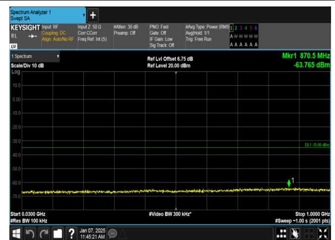
Band7-10MHz-16QAM-21100-1RB#49-30~1000-PASS
