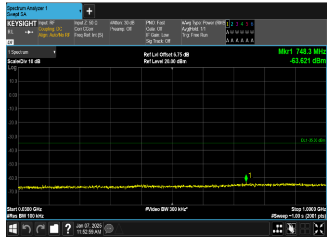
Band7-10MHz-16QAM-21400-50RB#0-30~1000-PASS
