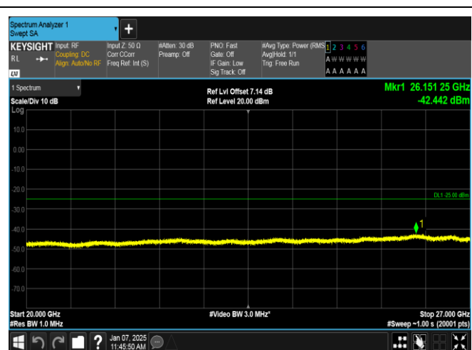
Band7-10MHz-16OAM-21100-1RB#49-20000~27000-PASS
