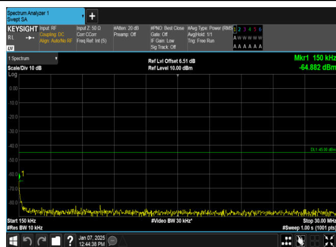
Band7-15MHz-QPSK-20825-75RB#0-0.15~30-PASS
