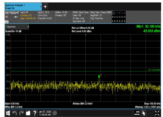
Band7-10MHz-16QAM-21100-1RB#49-0.009~0.15-PASS
