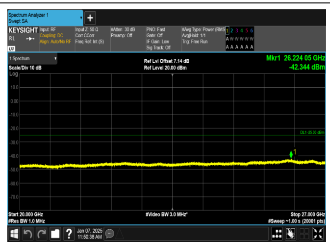
Band7-10MHz-QPSK-21400-1RB#49-20000~27000-PASS
