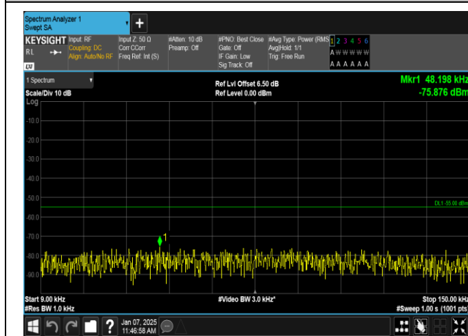
Band7-10MHz-16OAM-21100-50RB#0-0.009~0.15-PASS
