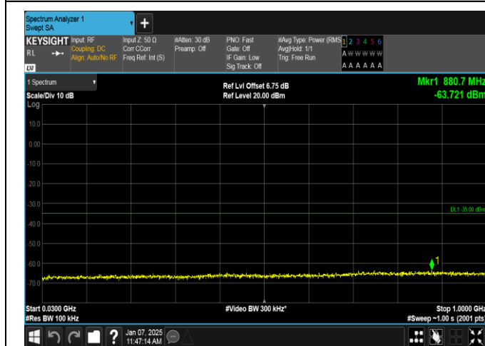
Band7-10MHz-16QAM-21100-50RB#0-30~1000-PASS
