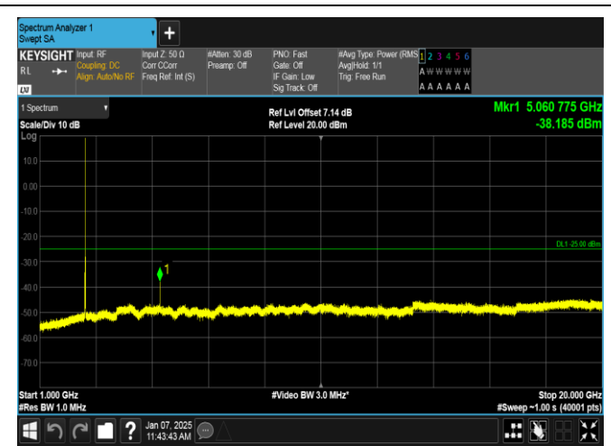
Band7-10MHz-16QAM-21100-1RB#0-1000~20000-PASS
