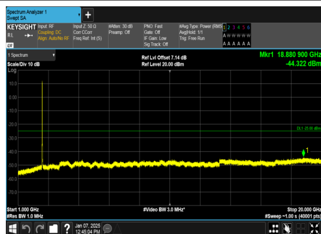
Band7-15MHz-QPSK-20825-75RB#0-1000~20000-PASS
