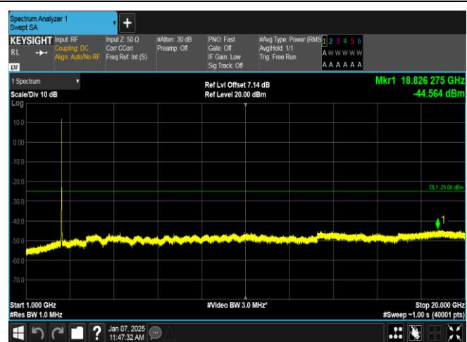
Band7-10MHz-16QAM-21100-50RB#0-1000~20000-PASS
