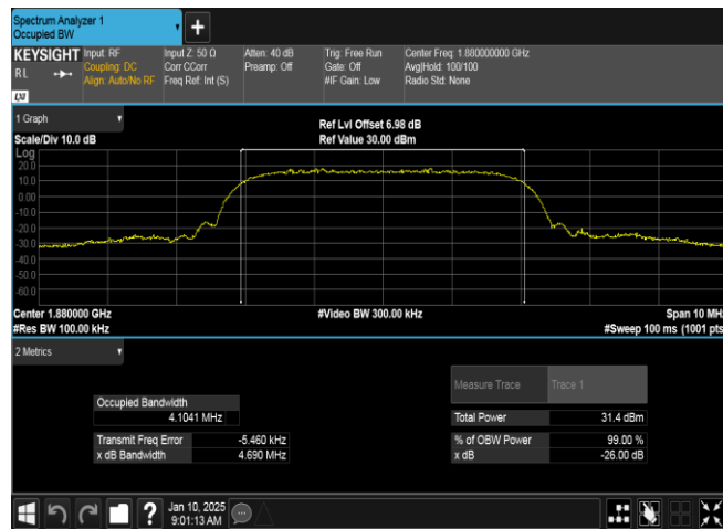
Band2-9400-1-PASS
