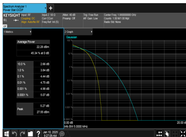
Band2-9400-1-PASS
