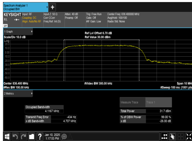
Band5-4182-5-PASS
