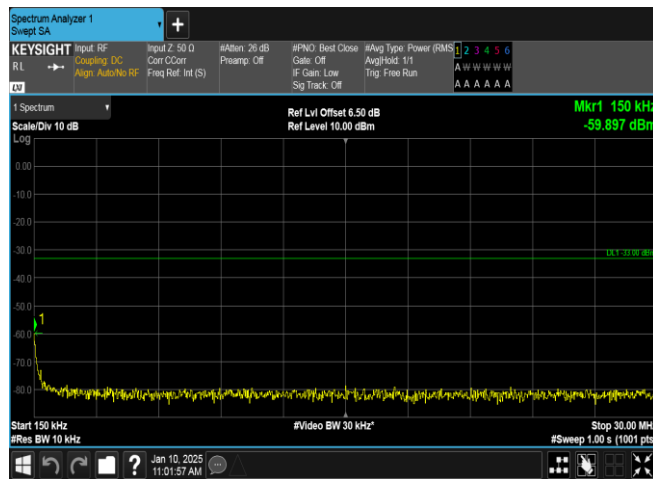
Band2-9400-5-0.15~30MHz-PASS
