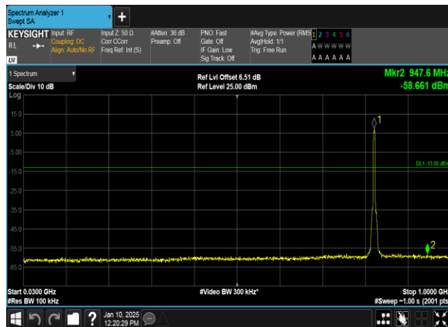
Band5-4132-3-30~1000MHz-PASS
