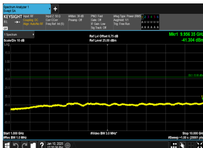
Band5-4132-3-1000~10000MHz-PASS
