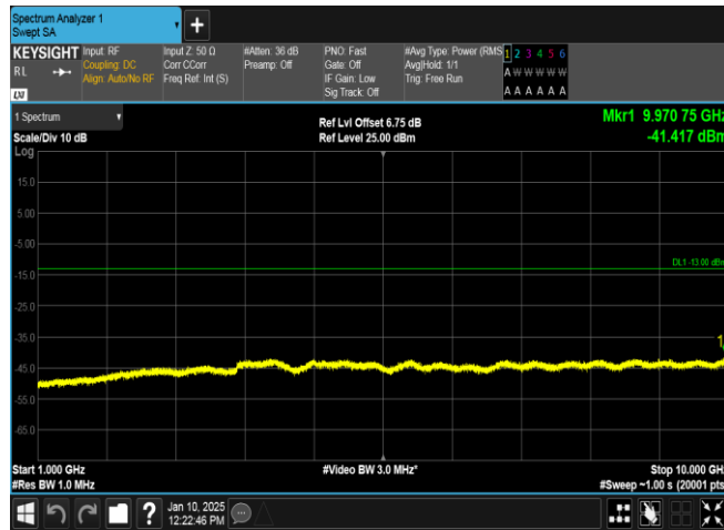
Band5-4132-4-1000~10000MHz-PASS
