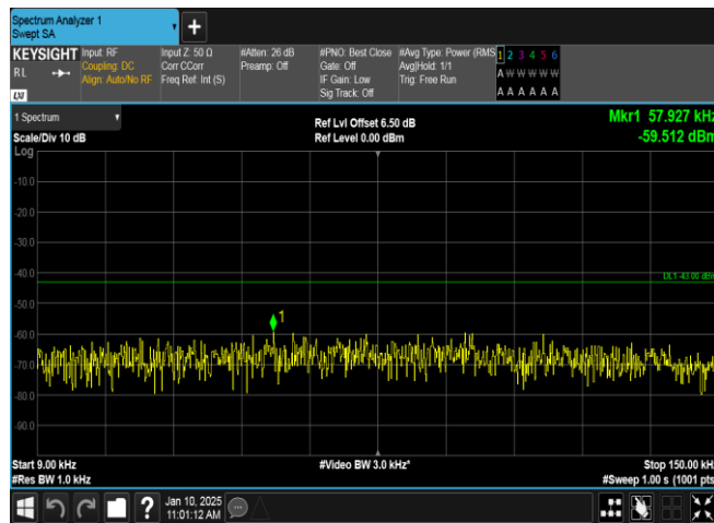
Band2-9262-5-0.009~0.15MHz-PASS
