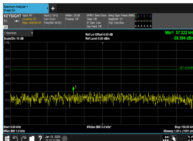
Band5-4233-1-0.009~0.15MHz-PASS
