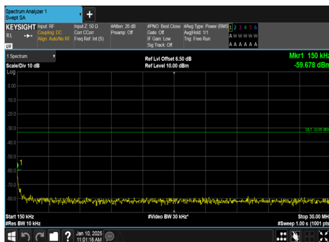
Band2-9262-5-0.15~30MHz-PASS
