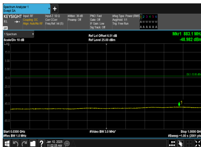
Band2-9400-5-30~1000MHz-PASS
