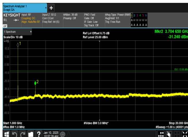
Band2-9400-3-1000~20000MHz-PASS
