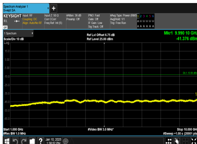
Band5-4182-5-1000~10000MHz-PASS
