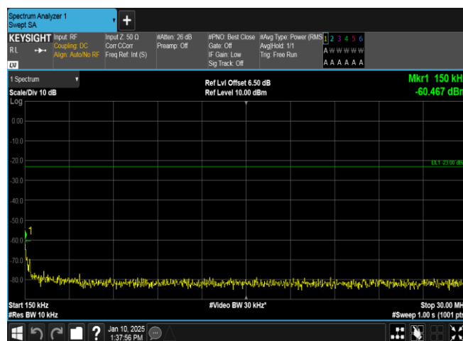
Band5-4132-5-0.15~30MHz-PASS
