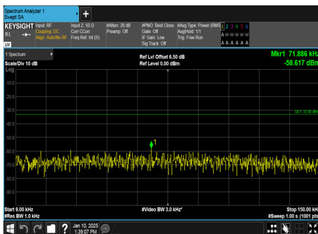
Band5-4233-5-0.009~0.15MHz-PASS
