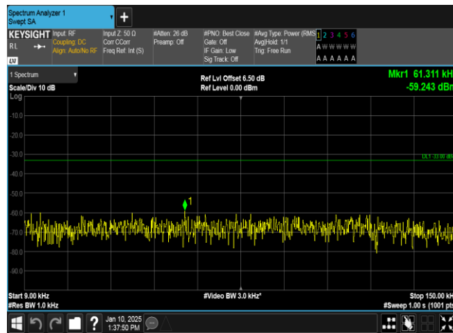
Band5-4132-5-0.009~0.15MHz-PASS
