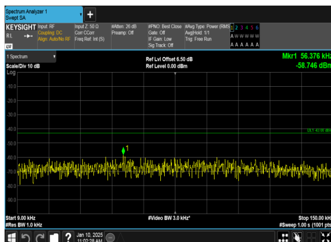
Band2-9538-5-0.009~0.15MHz-PASS
