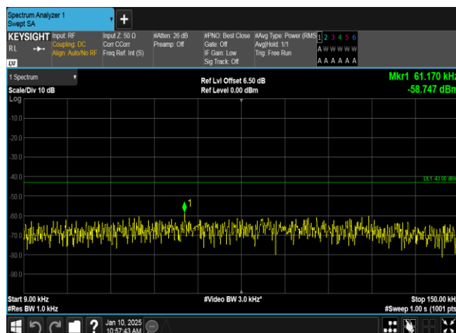
Band2-9538-3-0.009~0.15MHz-PASS
