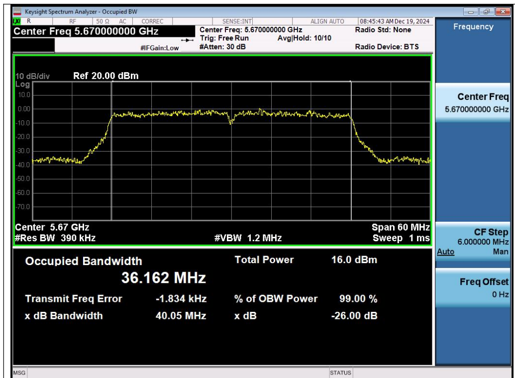
Test_Graph_802.11ac40_ANT1_5670_MCS0_OBW
