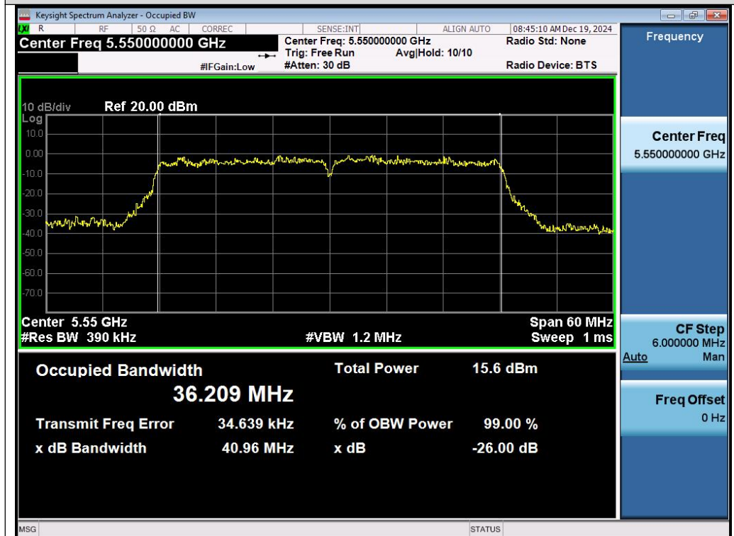
Test_Graph_802.11ac40_ANT1_5550_MCS0_OBW
