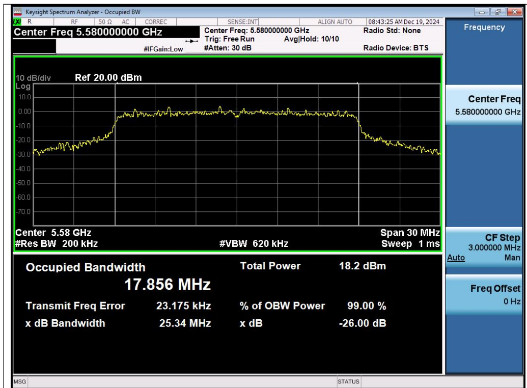
Test_Graph_802.11ac20_ANT1_5580_MCS0_OBW
