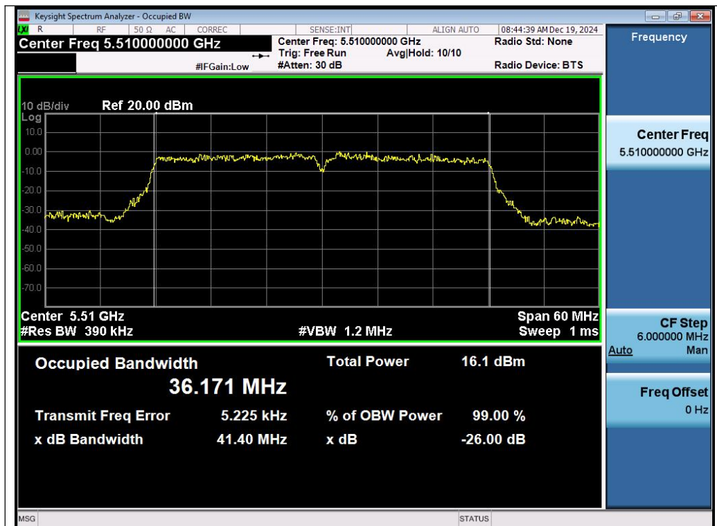
Test_Graph_802.11ac40_ANT1_5510_MCS0_OBW
