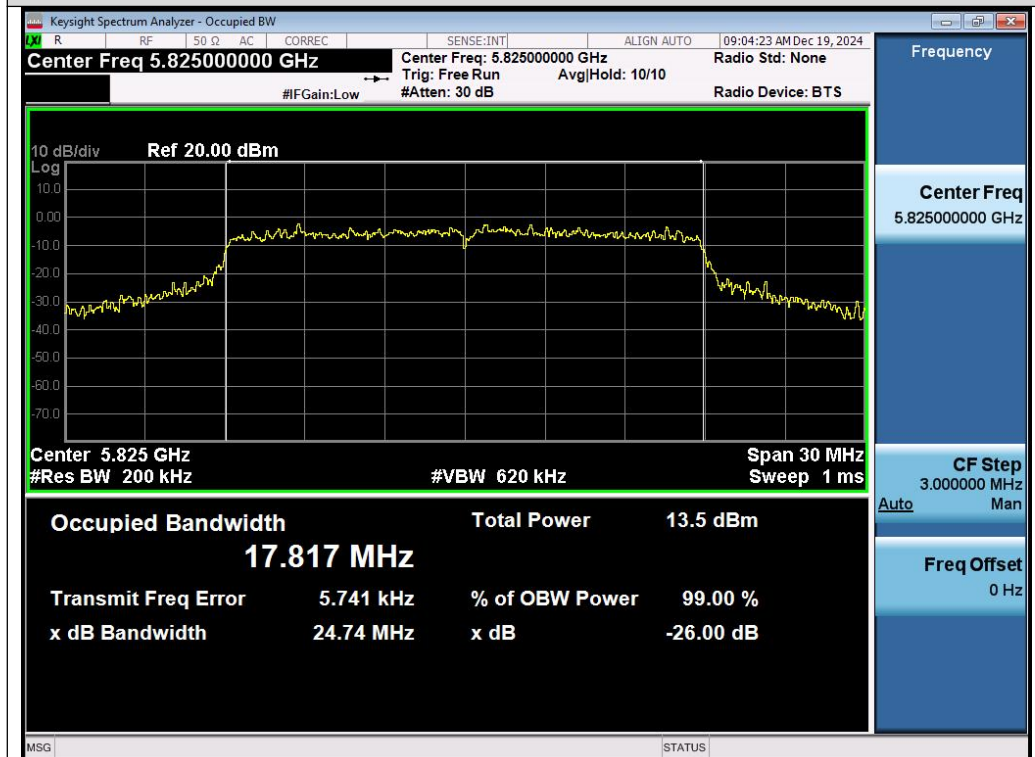
Test_Graph_802.11ac20_ANT1_5825_MCS0_OBW
