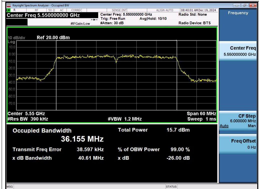
Test_Graph_802.11n40_ANT1_5550_MCS0_OBW
