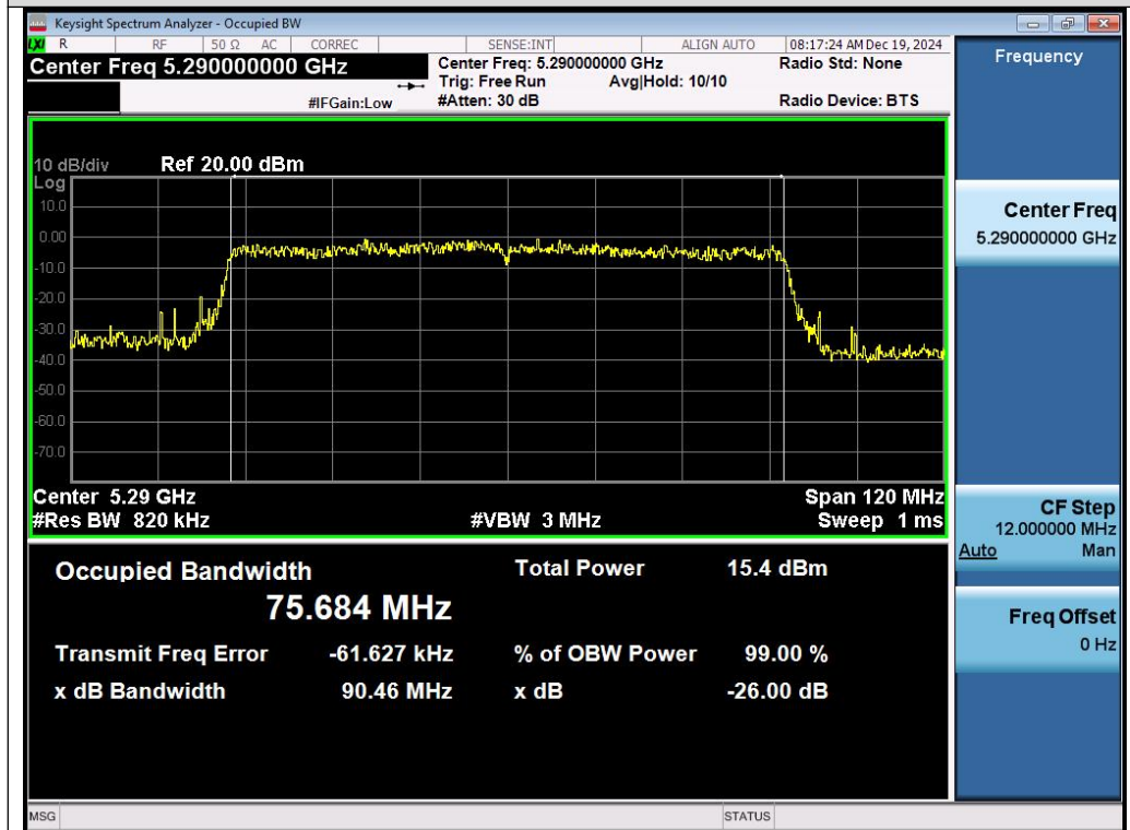
Test_Graph_802.11ac80_ANT1_5290_MCS0_OBW
