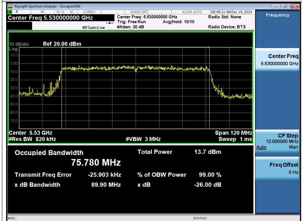
Test_Graph_802.11ac80_ANT1_5530_MCS0_OBW
