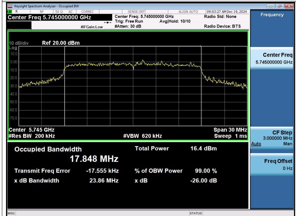
Test_Graph_802.11ac20_ANT1_5745_MCS0_OBW
