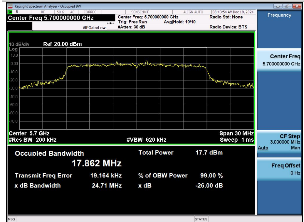
Test_Graph_802.11ac20_ANT1_5700_MCS0_OBW
