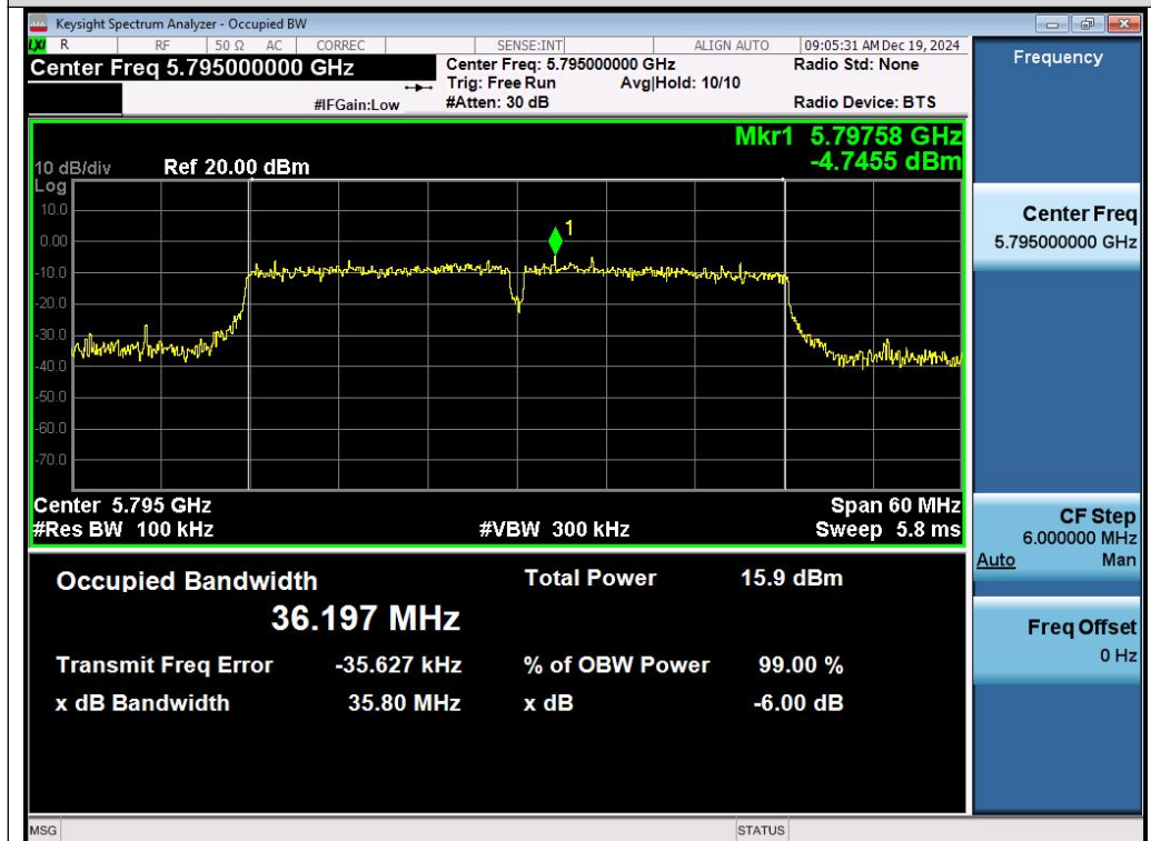
Test_Graph_802.11ac40_ANT1_5795_MCS0_DTSBW
