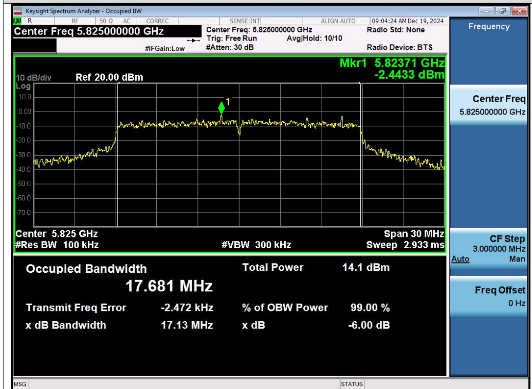
Test_Graph_802.11ac20_ANT1_5825_MCS0_DTSBW
