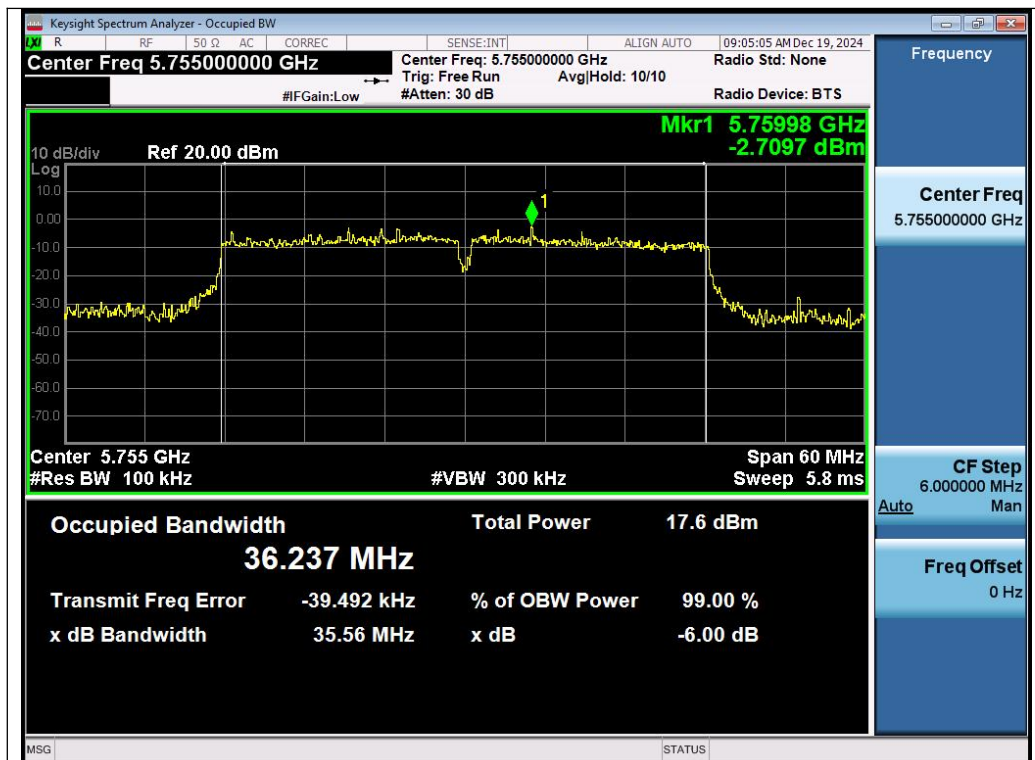
Test_Graph_802.11ac40_ANT1_5755_MCS0_DTSBW
