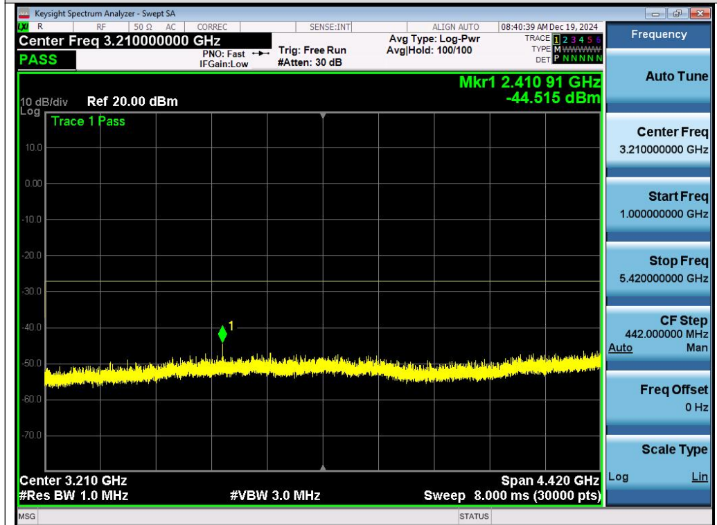
Test_Graph_802.11n40_ANT1_5550_MCS0_Frequency Band 2
