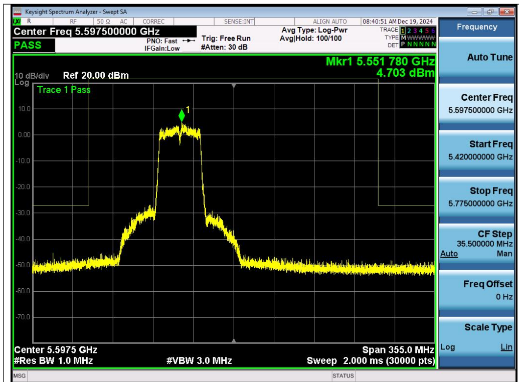
Test_Graph_802.11n40_ANT1_5550_MCS0_Frequency Band 3
