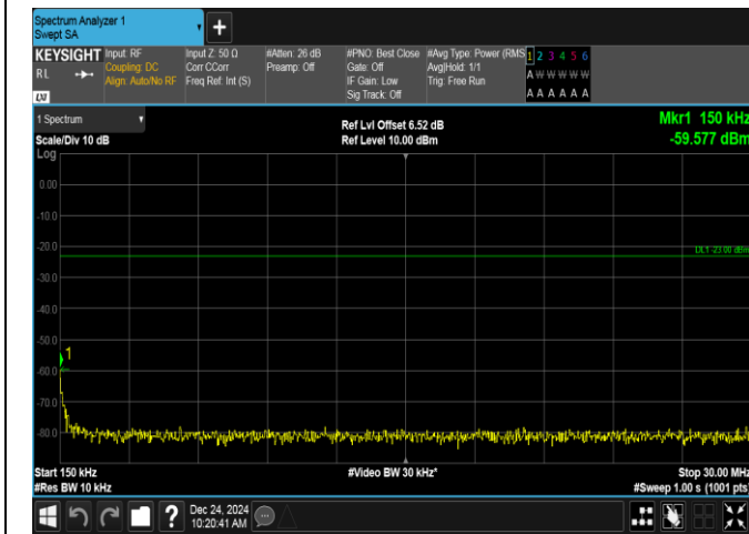
Band12-1.4MHz-16QAM-23017-1RB#0-0.15~30-PASS
