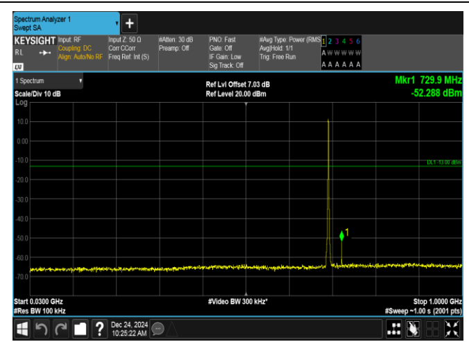
Band12-1.4MHz-16QAM-23017-6RB#0-30~1000-PASS
