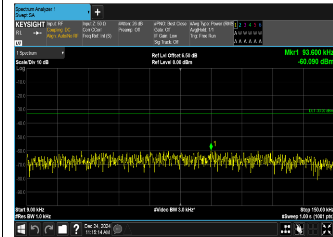
Band12-3MHz-QPSK-23025-15RB#0-0.009~0.15-PASS
