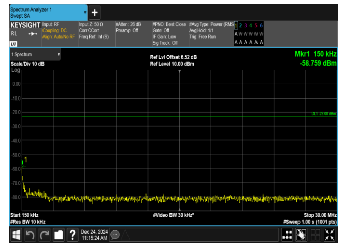
Band12-3MHz-QPSK-23025-15RB#0-0.15~30-PASS
