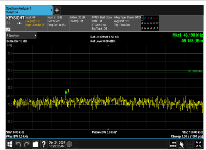
Band12-1.4MHz-16QAM-23017-1RB#0-0.009~0.15-PASS
