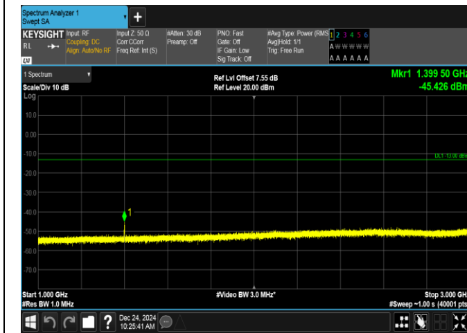
Band12-1.4MHz-16QAM-23017-6RB#0-1000~3000-PASS
