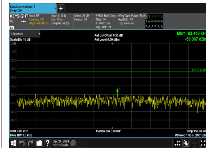
Band12-1.4MHz-16QAM-23095-6RB#0-0.009~0.15-PASS
