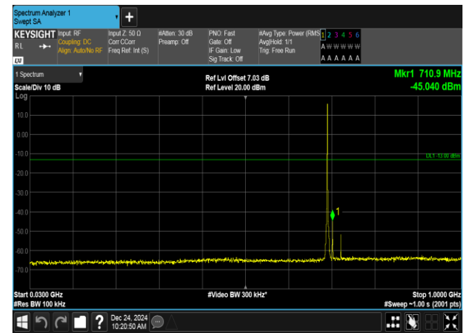
Band12-1.4MHz-16QAM-23017-1RB#0-30~1000-PASS
