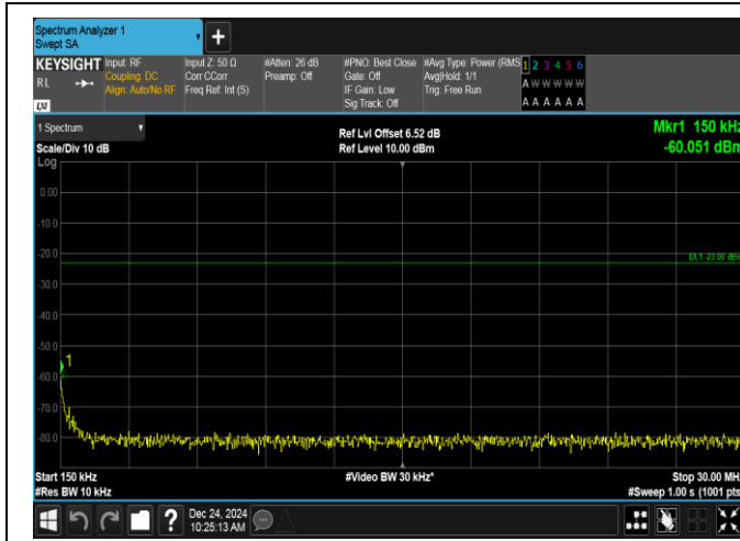
Band12-1.4MHz-16QAM-23017-6RB#0-0.15~30-PASS
