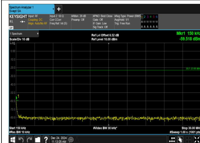
Band12-3MHz-QPSK-23025-1RB#14-0.15~30-PASS
