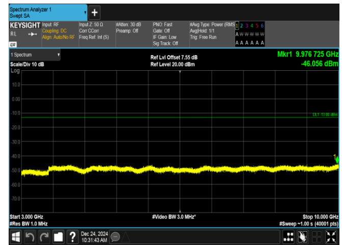
Band12-1.4MHz-QPSK-23095-6RB#0-3000~10000-PASS
