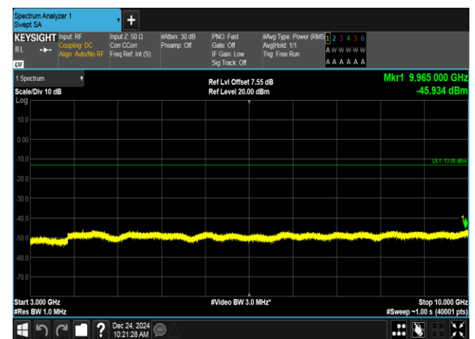
Band12-1.4MHz-16QAM-23017-1RB#0-3000~10000-PASS
