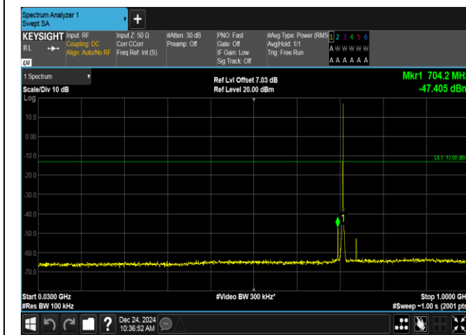
Band12-1.4MHz-16QAM-23173-1RB#5-30~1000-PASS
