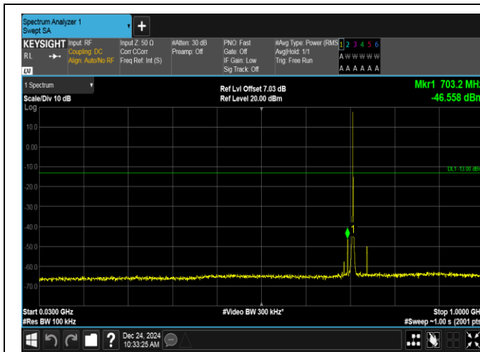
Band12-1.4MHz-QPSK-23173-1RB#0-30~1000-PASS
