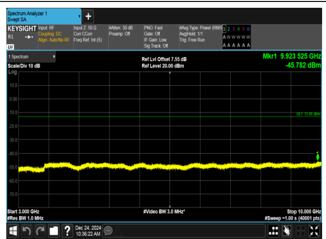
Band12-1.4MHz-QPSK-23173-1RB#5-3000~10000-PASS
