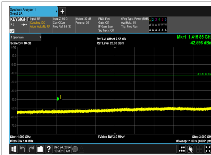
Band12-1.4MHz-16QAM-23095-1RB#5-1000~3000-PASS
