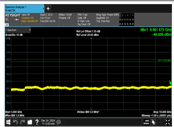
Band12-3MHz-QPSK-23025-1RB#14-3000~10000-PASS
