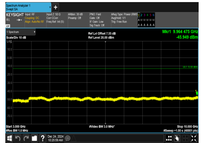
Band12-1.4MHz-16QAM-23017-6RB#0-3000~10000-PASS
