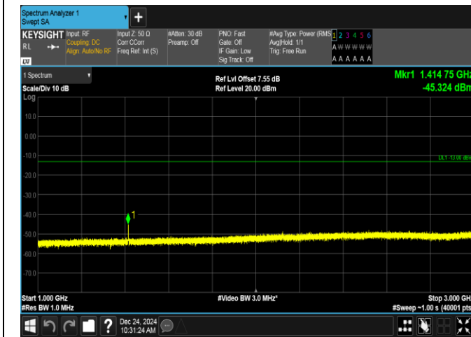
Band12-1.4MHz-QPSK-23095-6RB#0-1000~3000-PASS
