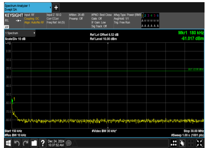
Band12-1.4MHz-QPSK-23173-6RB#0-0.15~30-PASS
