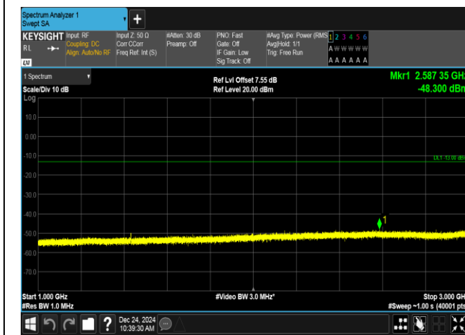
Band12-1.4MHz-16QAM-23173-6RB#0-1000~3000-PASS
