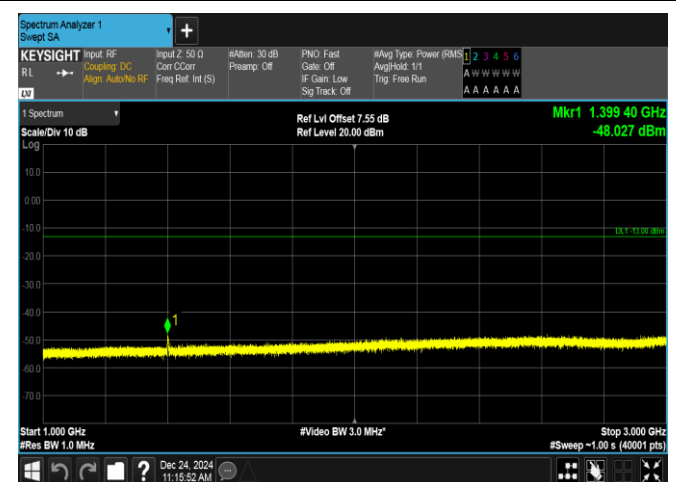
Band12-3MHz-QPSK-23025-15RB#0-1000~3000-PASS
