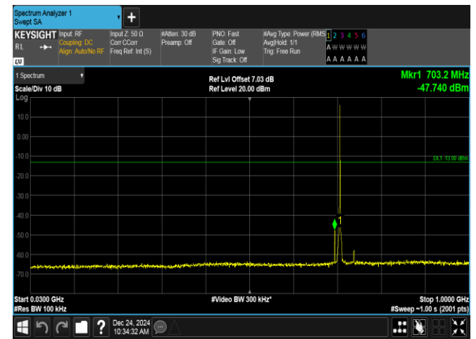
Band12-1.4MHz-16QAM-23173-1RB#0-30~1000-PASS
