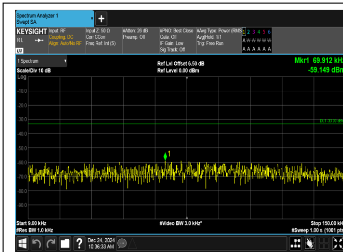
Band12-1.4MHz-16QAM-23173-1RB#5-0.009~0.15-PASS
