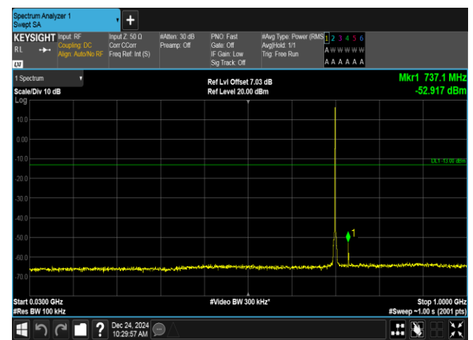
Band12-1.4MHz-16QAM-23095-1RB#5-30~1000-PASS
