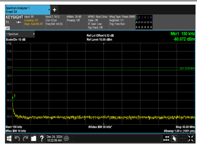
Band12-1.4MHz-16QAM-23017-1RB#5-0.15~30-PASS
