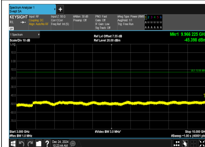
Band12-1.4MHz-16QAM-23017-1RB#5-3000~10000-PAS
