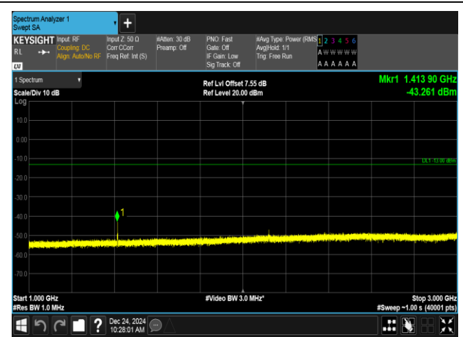
Band12-1.4MHz-16QAM-23095-1RB#0-1000~3000-PASS
