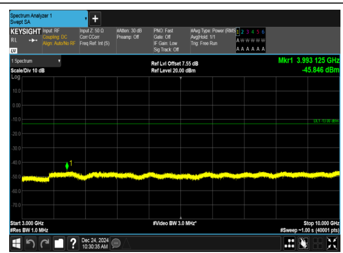
Band12-1.4MHz-16QAM-23095-1RB#5-3000~10000-PASS
