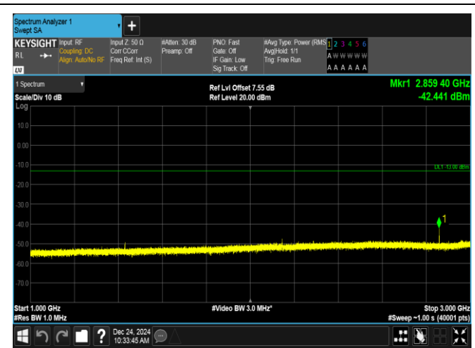
Band12-1.4MHz-QPSK-23173-1RB#0-1000~3000-PASS
