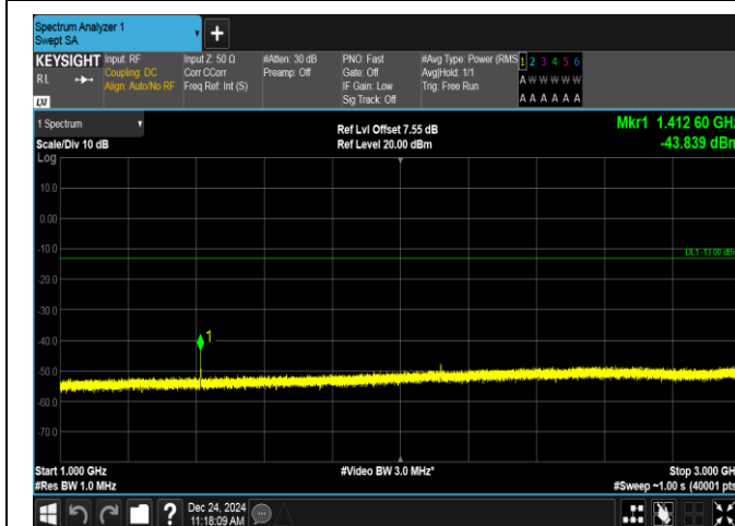
Band12-3MHz-QPSK-23095-1RB#0-1000~3000-PASS
