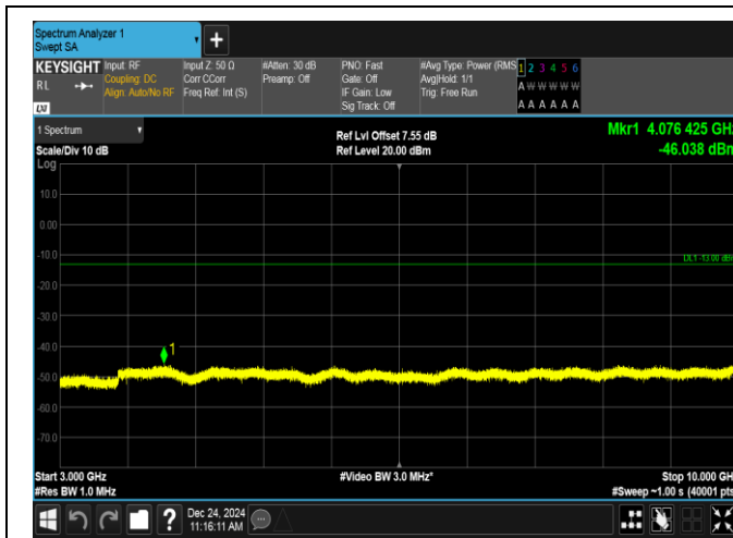
Band12-3MHz-QPSK-23025-15RB#0-3000~10000-PASS
