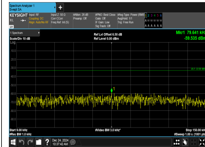
Band12-1.4MHz-QPSK-23173-6RB#0-0.009~0.15-PASS
