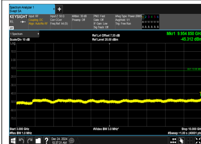
Band12-1.4MHz-16QAM-23173-1RB#5-3000~10000-PAS
