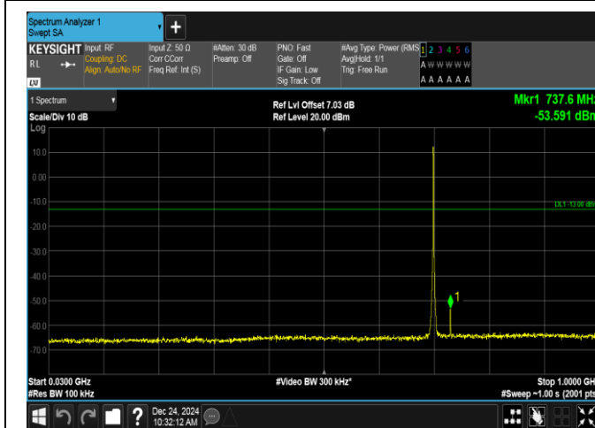
Band12-1.4MHz-16QAM-23095-6RB#0-30~1000-PASS
