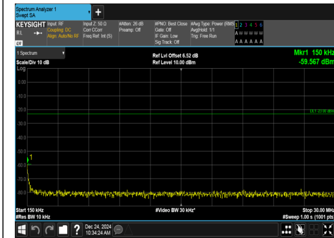
Band12-1.4MHz-16QAM-23173-1RB#0-0.15~30-PASS
