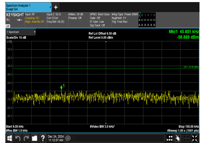
Band12-3MHz-QPSK-23025-1RB#14-0.009~0.15-PASS
