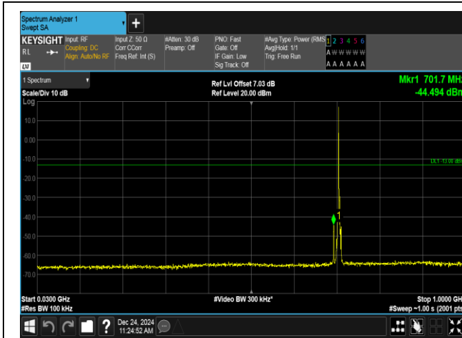
Band12-3MHz-QPSK-23165-1RB#0-30~1000-PASS
