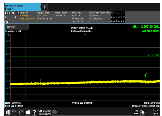
Band12-3MHz-16QAM-23025-1RB#14-1000~3000-PASS
