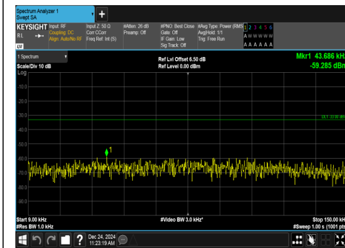
Band12-3MHz-16QAM-23095-15RB#0-0.009~0.15-PASS
