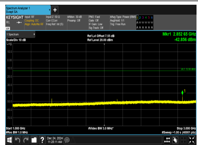
Band12-3MHz-QPSK-23165-1RB#0-1000~3000-PASS
