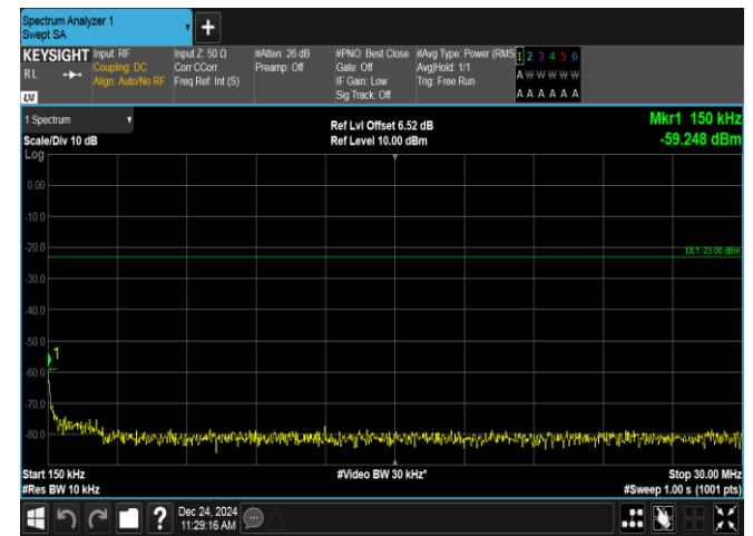
Band12-3MHz-QPSK-23165-15RB#0-0.15~30-PASS
