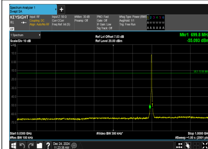
Band12-3MHz-16QAM-23095-15RB#0-30~1000-PASS
