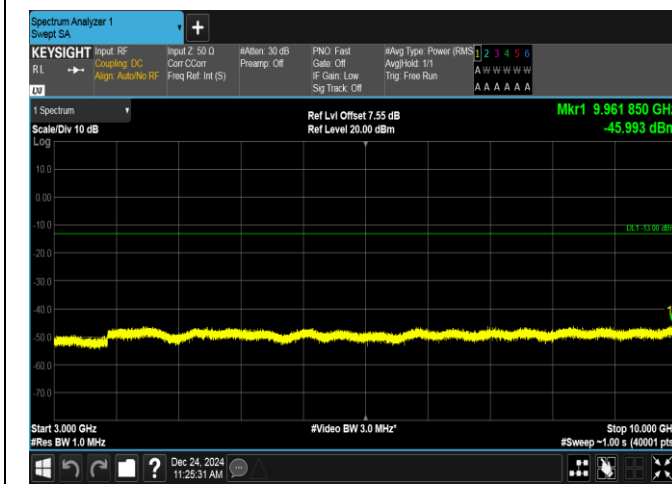
Band12-3MHz-QPSK-23165-1RB#0-3000~10000-PASS
