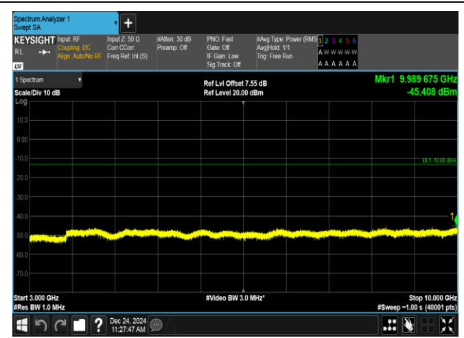
Band12-3MHz-QPSK-23165-1RB#14-3000~10000-PASS
