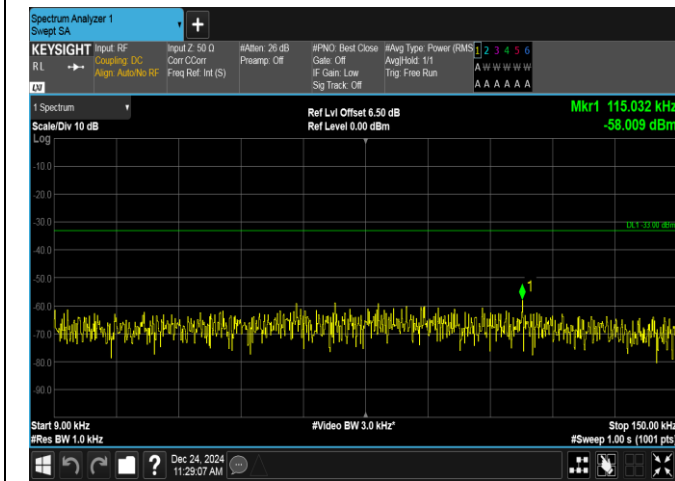
Band12-3MHz-QPSK-23165-15RB#0-0.009~0.15-PASS
