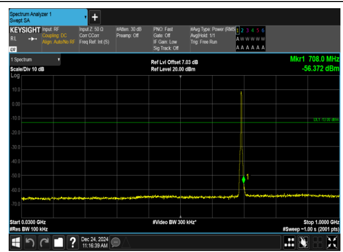
Band12-3MHz-16QAM-23025-15RB#0-30~1000-PASS
