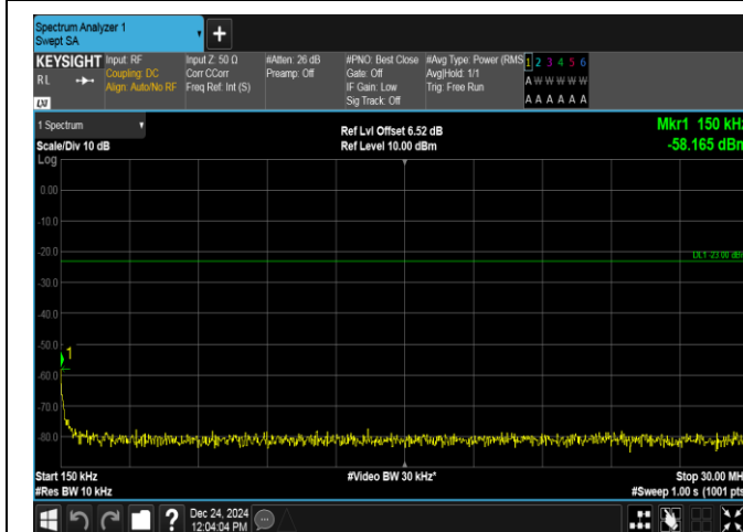
Band12-5MHz-QPSK-23035-1RB#24-0.15~30-PASS
