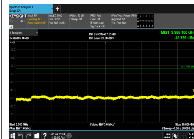
Band12-3MHz-QPSK-23095-1RB#14-3000~10000-PASS
