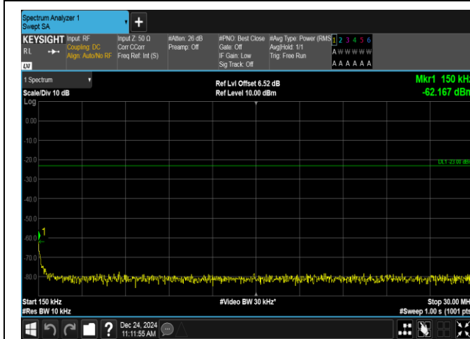
Band12-3MHz-16QAM-23025-1RB#0-0.15~30-PASS
