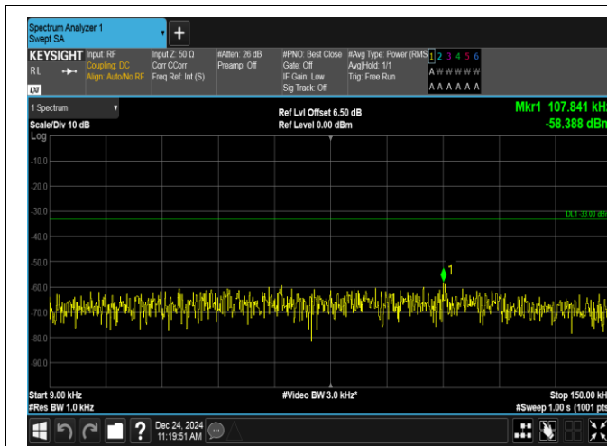
Band12-3MHz-QPSK-23095-1RB#14-0.009~0.15-PASS
