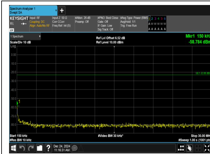
Band12-3MHz-16QAM-23025-15RB#0-0.15~30-PASS
