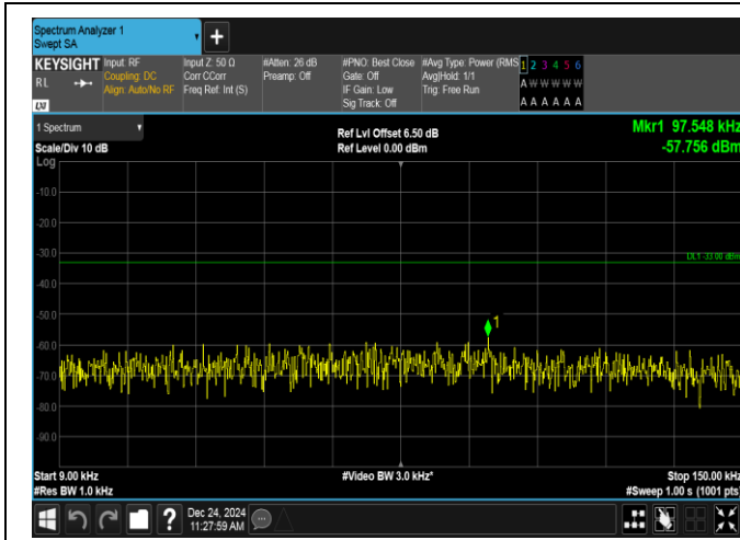
Band12-3MHz-16QAM-23165-1RB#14-0.009~0.15-PASS
