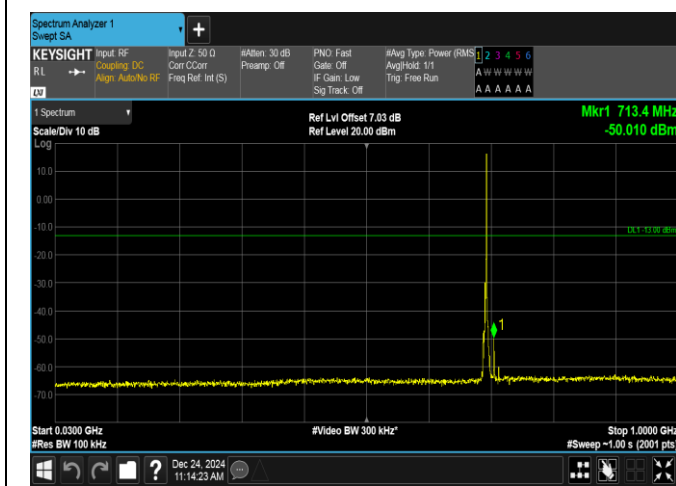
Band12-3MHz-16QAM-23025-1RB#14-30~1000-PASS
