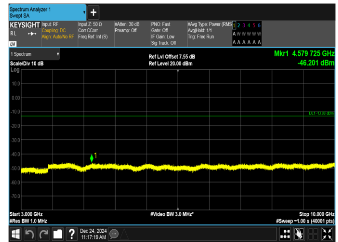
Band12-3MHz-16QAM-23025-15RB#0-3000~10000-PASS
