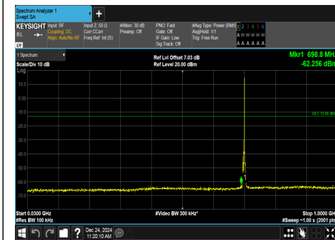
Band12-3MHz-QPSK-23095-1RB#14-30~1000-PASS
