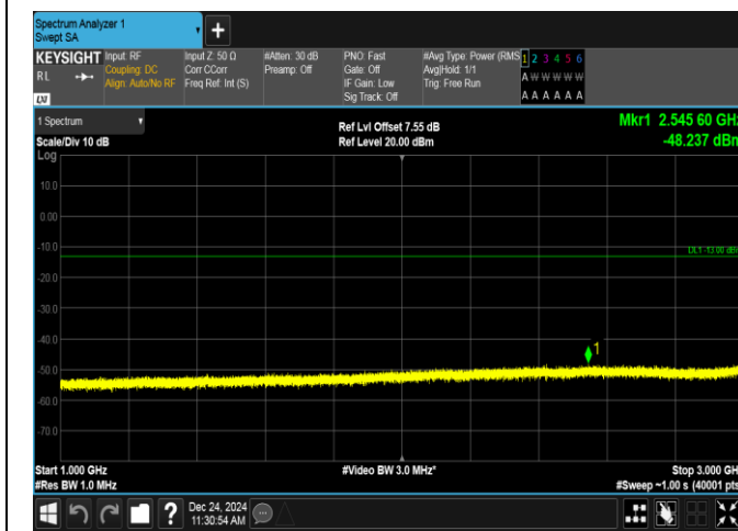
Band12-3MHz-16QAM-23165-15RB#0-1000~3000-PASS
