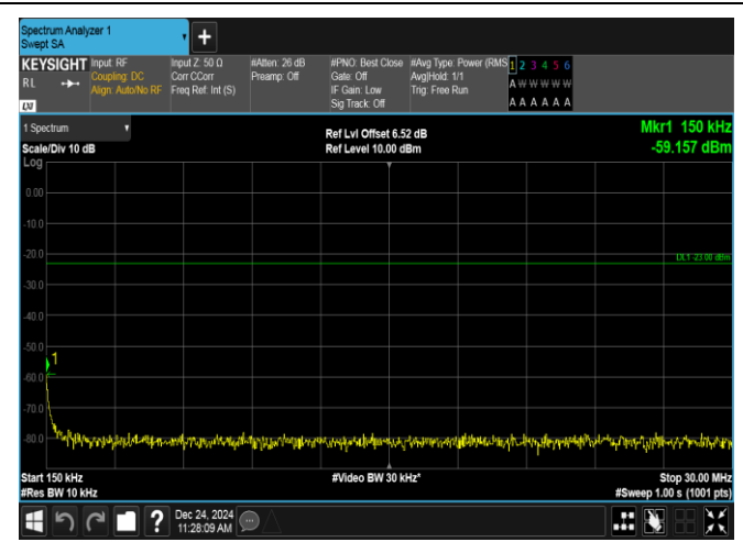
Band12-3MHz-16QAM-23165-1RB#14-0.15~30-PASS
