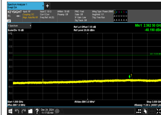
Band12-3MHz-16QAM-23025-15RB#0-1000~3000-PASS
