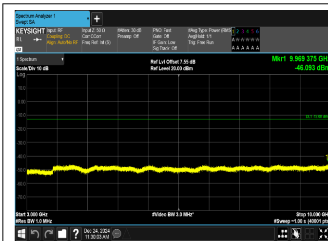
Band12-3MHz-QPSK-23165-15RB#0-3000~10000-PASS
