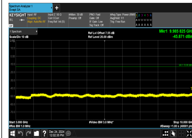
Band12-5MHz-QPSK-23035-1RB#0-3000~10000-PASS
