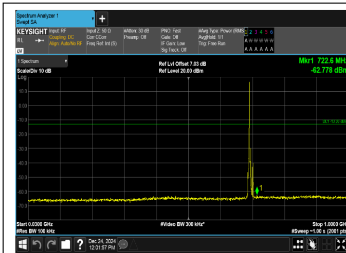
Band12-5MHz-QPSK-23035-1RB#0-30~1000-PASS
