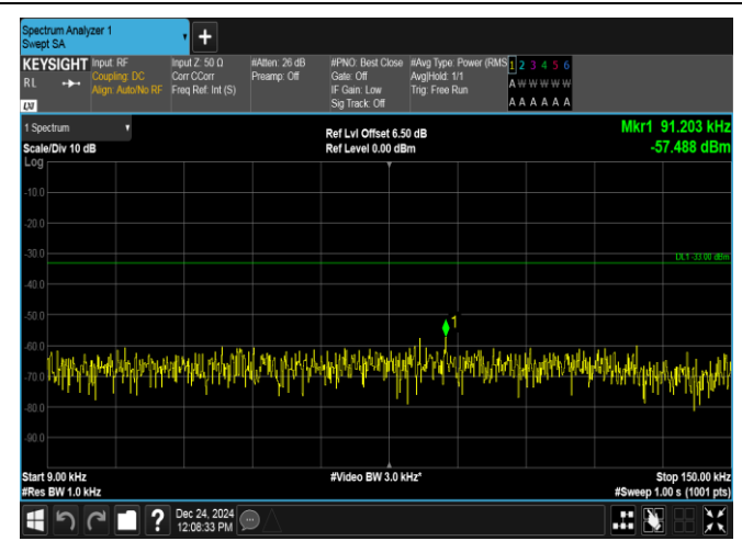
Band12-5MHz-QPSK-23095-1RB#0-0.009~0.15-PASS
