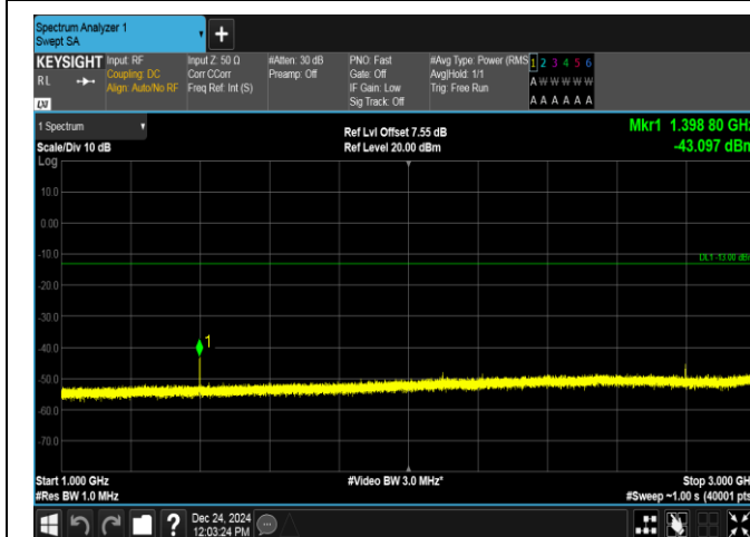
Band12-5MHz-16QAM-23035-1RB#0-1000~3000-PASS
