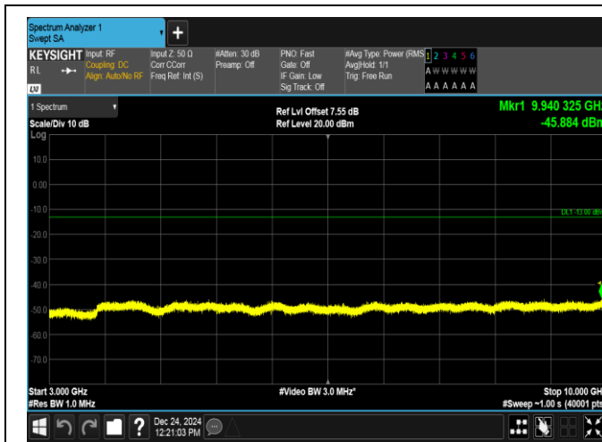
Band12-5MHz-QPSK-23155-25RB#0-3000~10000-PASS
