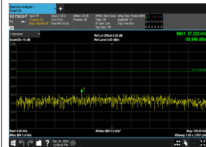
Band12-5MHz-16QAM-23095-1RB#0-0.009~0.15-PASS
