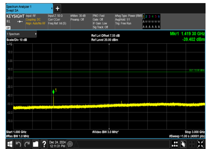
Band12-5MHz-QPSK-23095-1RB#24-1000~3000-PASS
