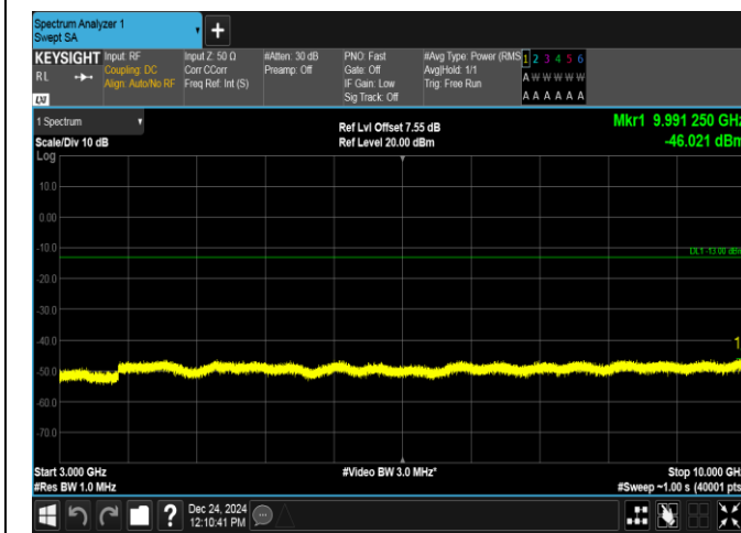
Band12-5MHz-16QAM-23095-1RB#0-3000~10000-PASS
