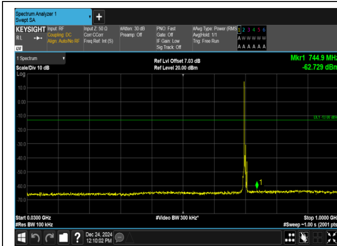
Band12-5MHz-16QAM-23095-1RB#0-30~1000-PASS
