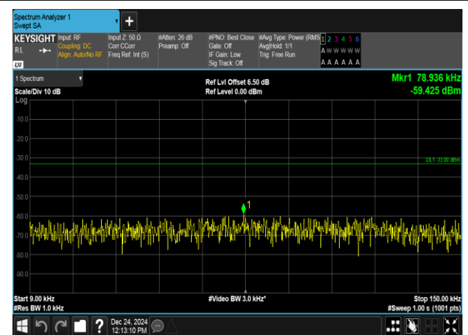
Band12-5MHz-QPSK-23095-25RB#0-0.009~0.15-PASS
