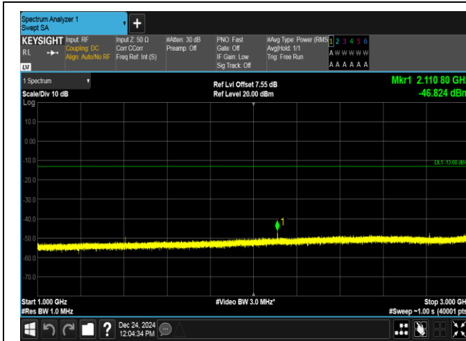
Band12-5MHz-QPSK-23035-1RB#24-1000~3000-PASS
