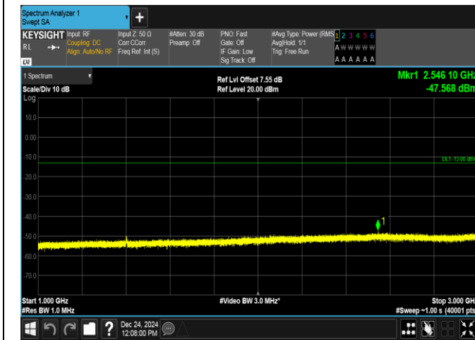
Band12-5MHz-16QAM-23035-25RB#0-1000~3000-PASS
