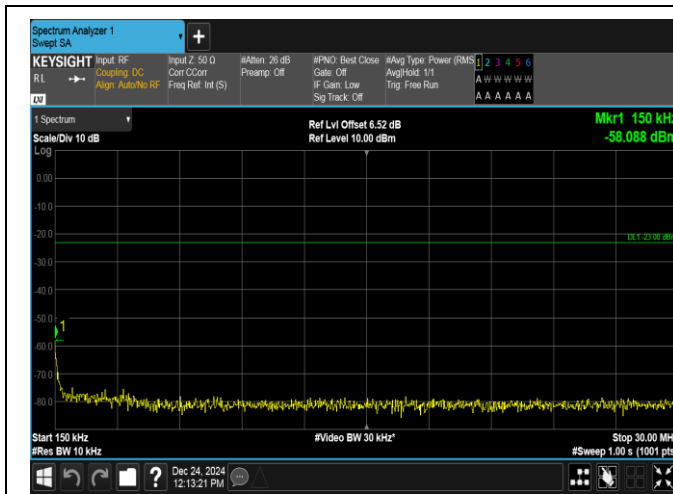
Band12-5MHz-QPSK-23095-25RB#0-0.15~30-PASS
