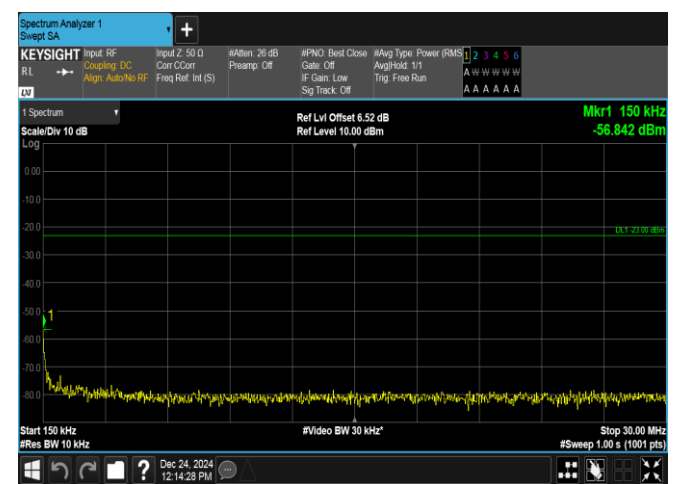
Band12-5MHz-16QAM-23095-25RB#0-0.15~30-PASS
