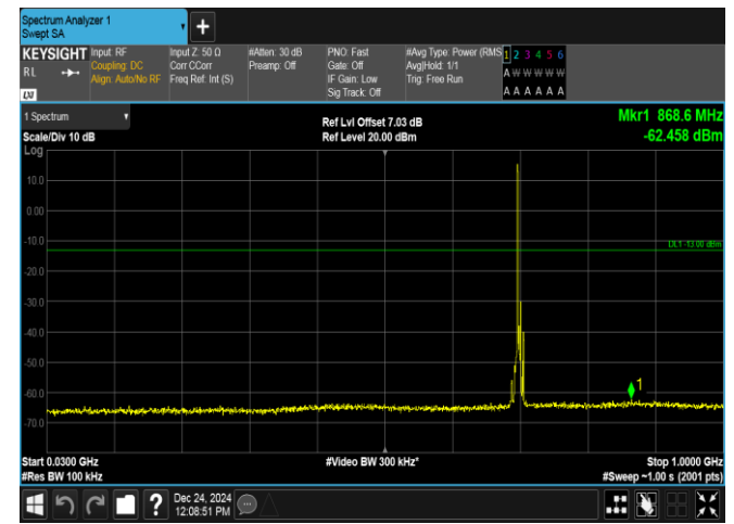
Band12-5MHz-QPSK-23095-1RB#0-30~1000-PASS
