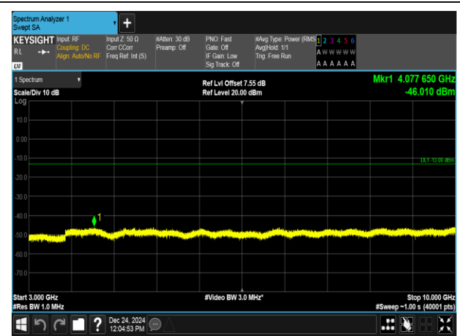
Band12-5MHz-QPSK-23035-1RB#24-3000~10000-PASS
