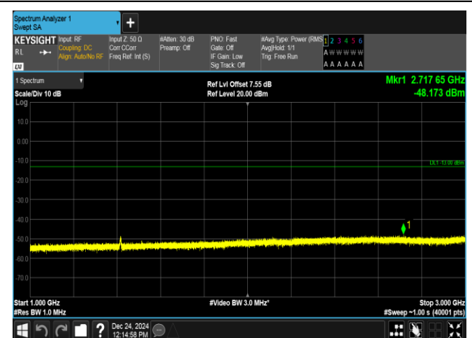
Band12-5MHz-16QAM-23095-25RB#0-1000~3000-PASS
