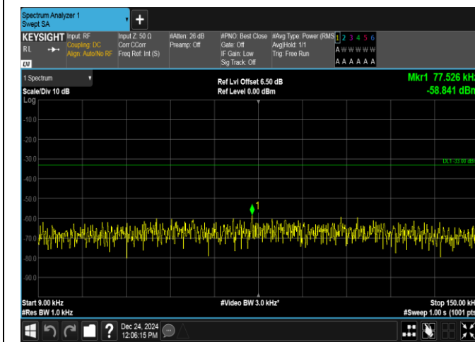
Band12-5MHz-QPSK-23035-25RB#0-0.009~0.15-PASS
