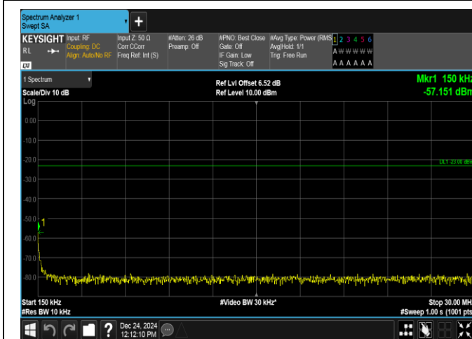
Band12-5MHz-16QAM-23095-1RB#24-0.15~30-PASS
