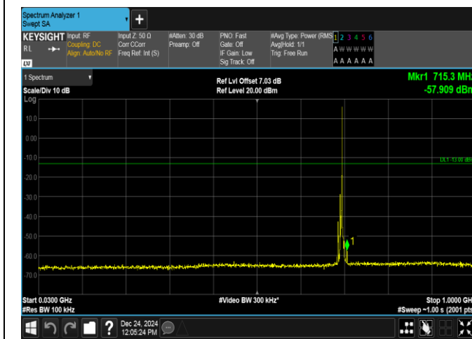
Band12-5MHz-16QAM-23035-1RB#24-30~1000-PASS
