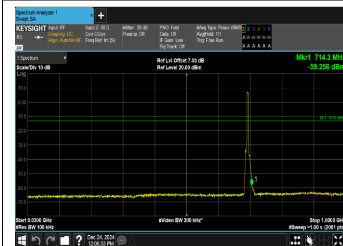
Band12-5MHz-QPSK-23035-25RB#0-30~1000-PASS
