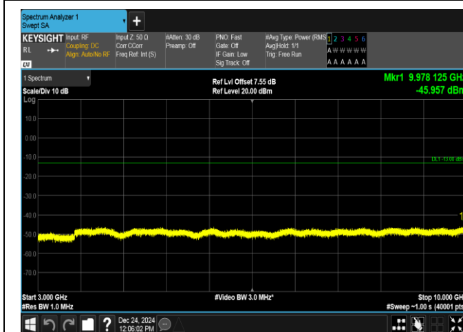
Band12-5MHz-16QAM-23035-1RB#24-3000~10000-PASS
