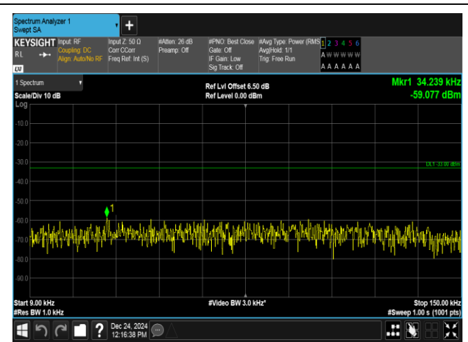
Band12-5MHz-16QAM-23155-1RB#0-0.009~0.15-PASS
