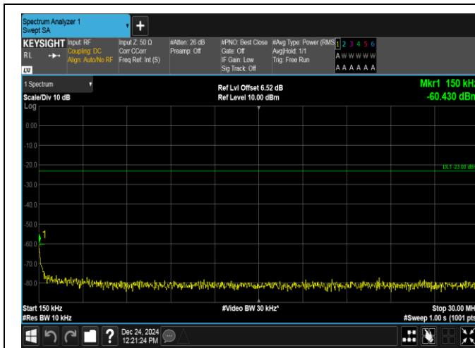
Band12-5MHz-16QAM-23155-25RB#0-0.15~30-PASS
