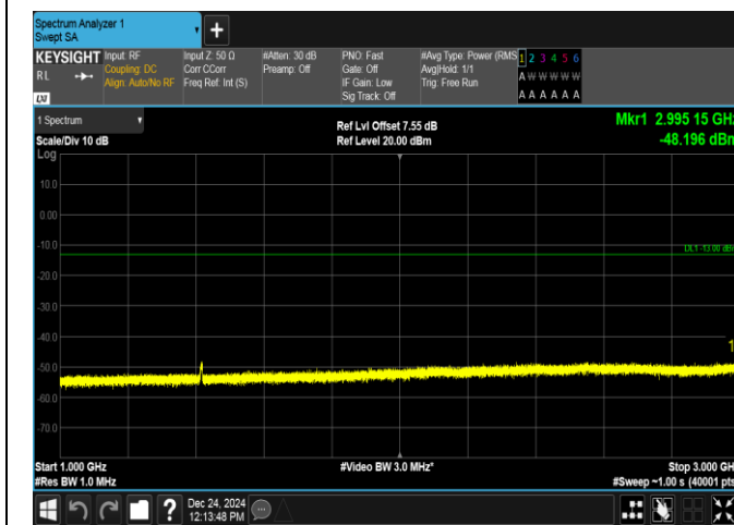
Band12-5MHz-QPSK-23095-25RB#0-1000~3000-PASS
