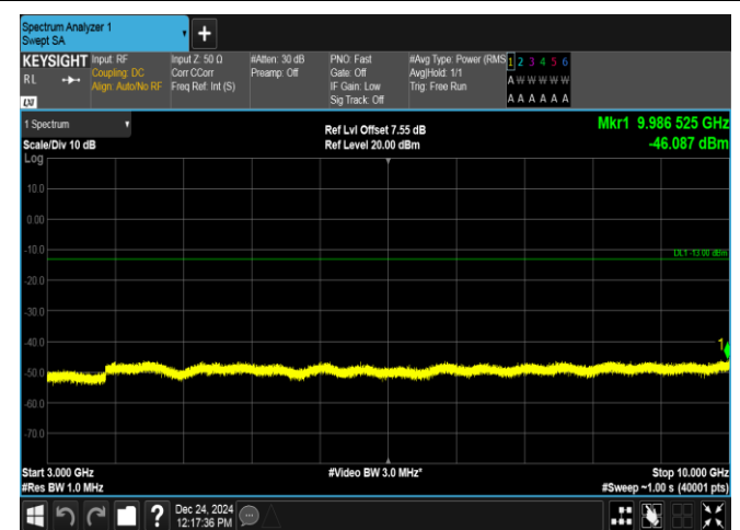
Band12-5MHz-16QAM-23155-1RB#0-3000~10000-PASS
