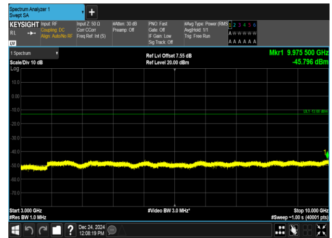
Band12-5MHz-16QAM-23035-25RB#0-3000~10000-PASS
