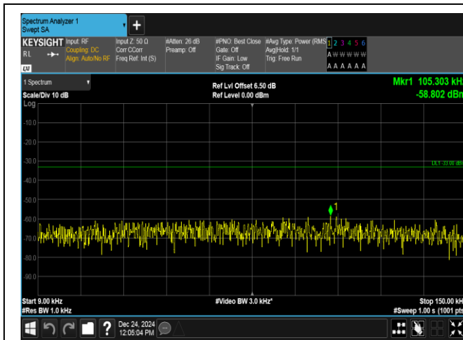
Band12-5MHz-16QAM-23035-1RB#24-0.009~0.15-PASS
