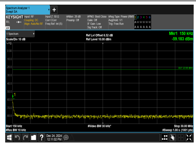
Band12-5MHz-QPSK-23095-1RB#24-0.15~30-PASS
