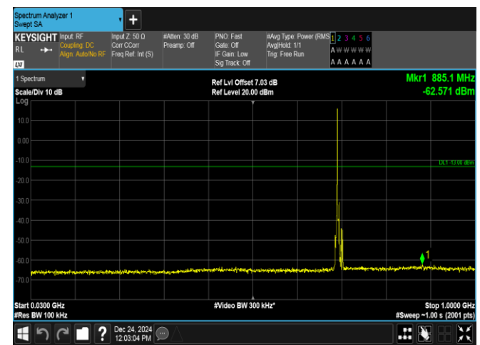
Band12-5MHz-16QAM-23035-1RB#0-30~1000-PASS
