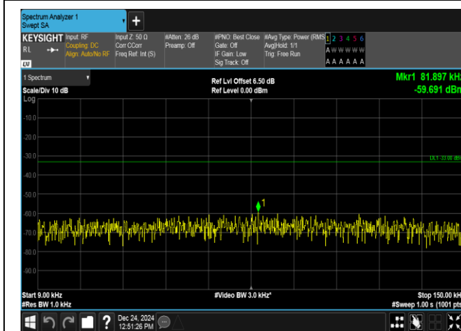
Band12-10MHz-QPSK-23060-1RB#0-0.009~0.15-PASS
