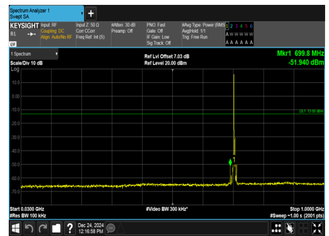
Band12-5MHz-16QAM-23155-1RB#0-30~1000-PASS
