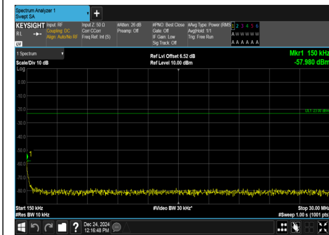
Band12-5MHz-16QAM-23155-1RB#0-0.15~30-PASS
