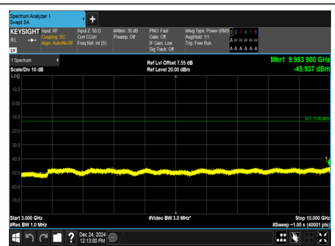
Band12-5MHz-16QAM-23095-1RB#24-3000~10000-PASS
