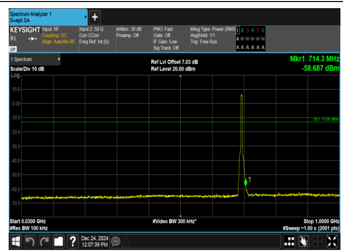
Band12-5MHz-16QAM-23035-25RB#0-30~1000-PASS
