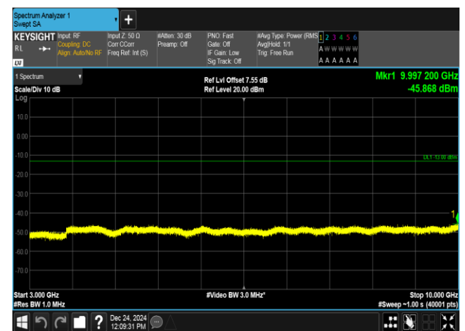
Band12-5MHz-QPSK-23095-1RB#0-3000~10000-PASS
