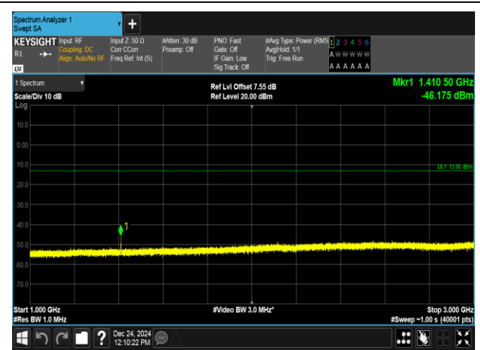
Band12-5MHz-16QAM-23095-1RB#0-1000~3000-PASS
