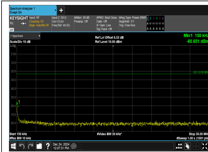
Band12-5MHz-16QAM-23035-25RB#0-0.15~30-PASS
