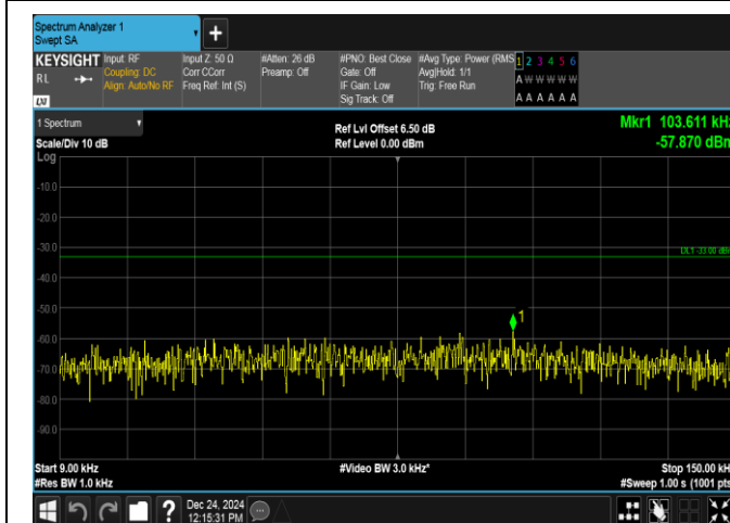
Band12-5MHz-QPSK-23155-1RB#0-0.009~0.15-PASS
