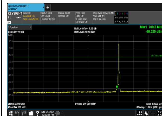
Band12-5MHz-QPSK-23155-25RB#0-30~1000-PASS
