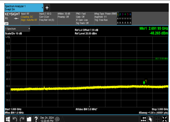
Band12-5MHz-QPSK-23155-25RB#0-1000~3000-PASS
