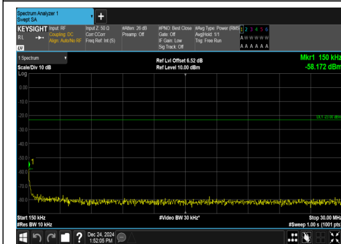
Band13-5MHz-16QAM-23205-25RB#0-0.15~30-PASS
