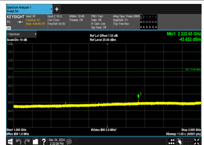
Band13-10MHz-QPSK-23230-1RB#0-1000~3000-PASS
