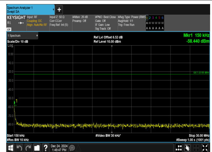
Band13-5MHz-16QAM-23205-1RB#24-0.15~30-PASS
