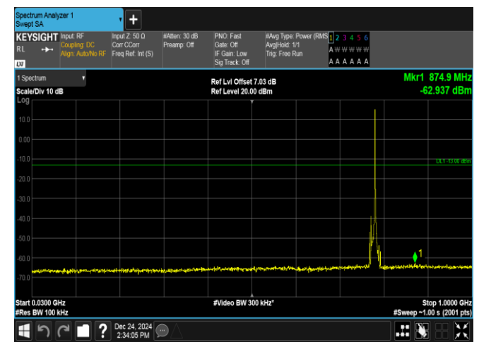
Band13-10MHz-QPSK-23230-1RB#49-30~1000-PASS
