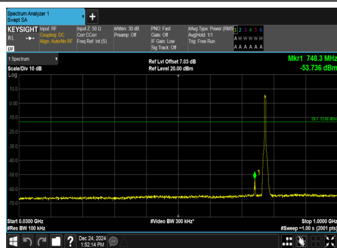
Band13-5MHz-16QAM-23205-25RB#0-30~1000-PASS
