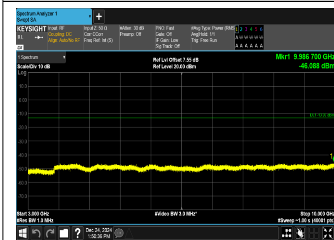
Band13-5MHz-16QAM-23205-1RB#24-3000~10000-PASS
