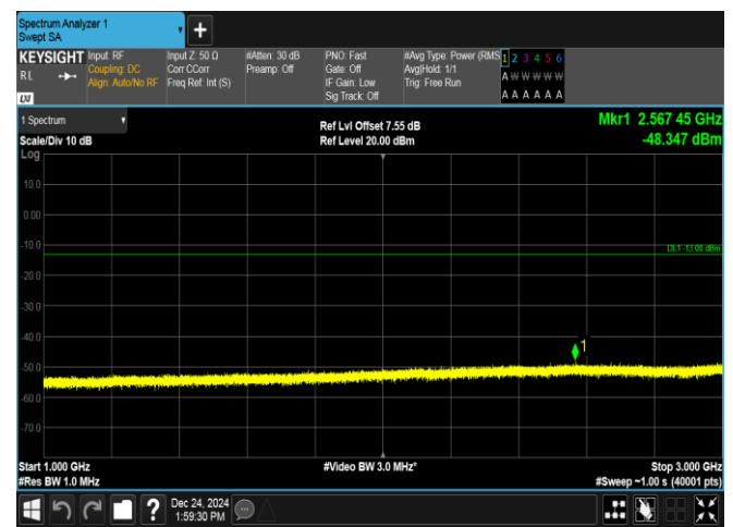
Band13-5MHz-16QAM-23230-25RB#0-1000~3000-PASS
