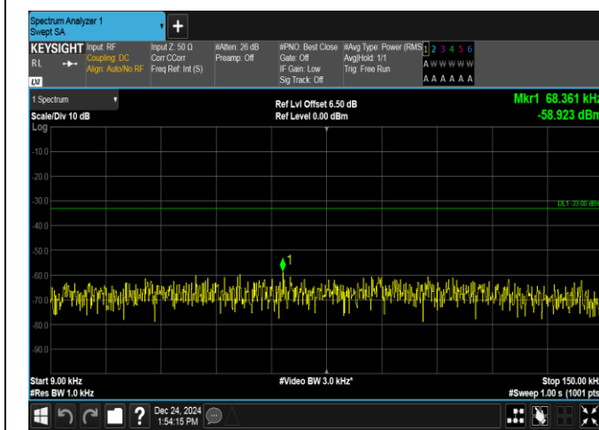
Band13-5MHz-16QAM-23230-1RB#0-0.009~0.15-PASS
