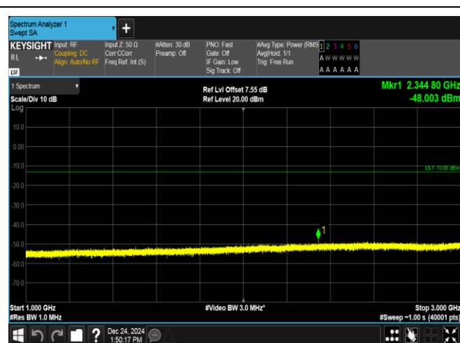
Band13-5MHz-16QAM-23205-1RB#24-1000~3000-PASS
