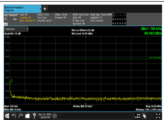
Band13-5MHz-16QAM-23230-25RB#0-0.15~30-PASS
