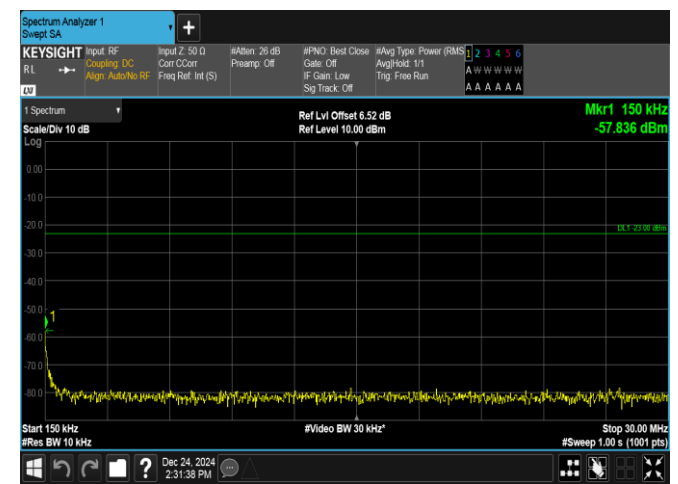
Band13-10MHz-QPSK-23230-1RB#0-0.15~30-PASS
