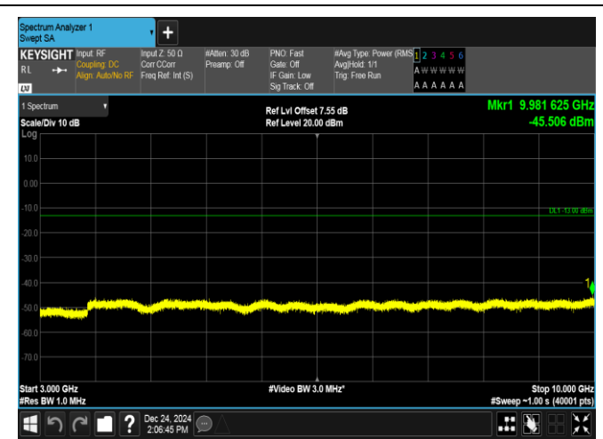
Band13-5MHz-16QAM-23255-25RB#0-3000~10000-PASS
