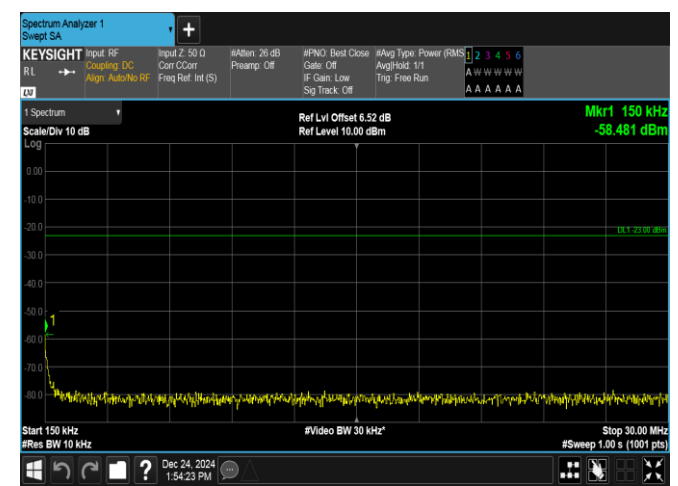
Band13-5MHz-16QAM-23230-1RB#0-0.15~30-PASS
