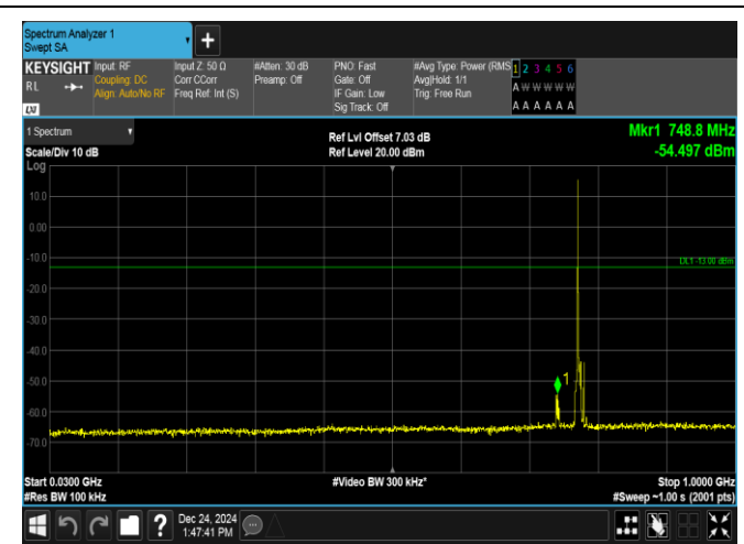
Band13-5MHz-16QAM-23205-1RB#0-30~1000-PASS
