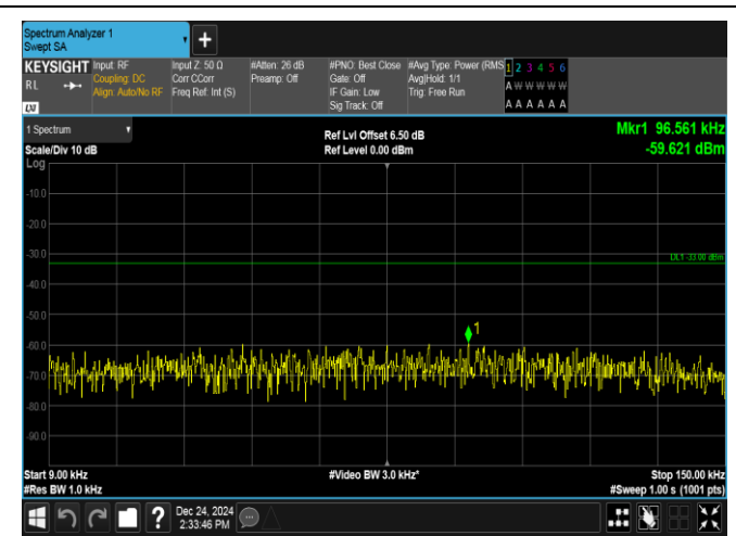
Band13-10MHz-QPSK-23230-1RB#49-0.009~0.15-PASS
