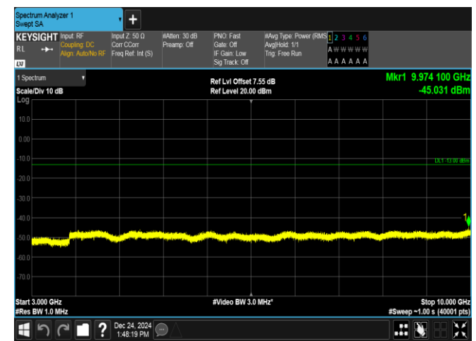
Band13-5MHz-16QAM-23205-1RB#0-3000~10000-PASS
