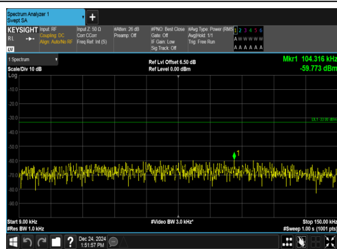
Band13-5MHz-16QAM-23205-25RB#0-0.009~0.15-PASS
