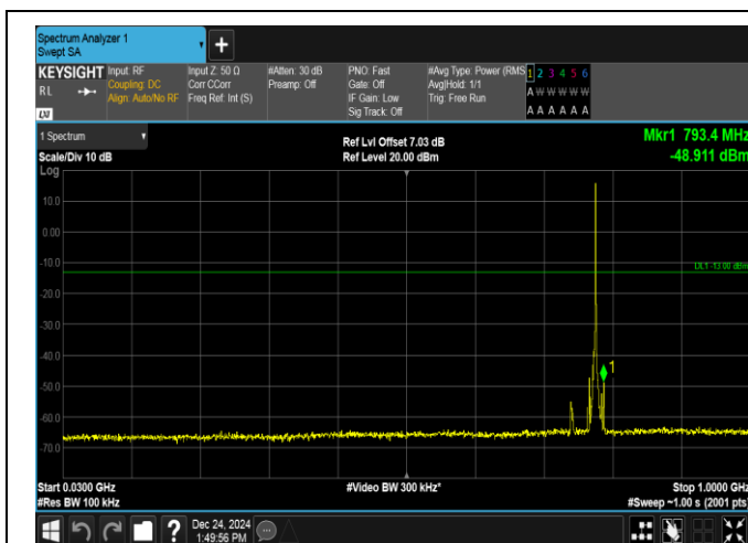
Band13-5MHz-16QAM-23205-1RB#24-30~1000-PASS
