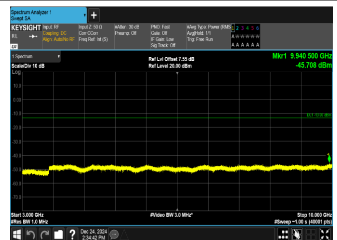
Band13-10MHz-QPSK-23230-1RB#49-3000~10000-PASS
