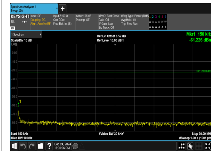
Band17-10MHz-QPSK-23790-50RB#0-0.15~30-PASS
