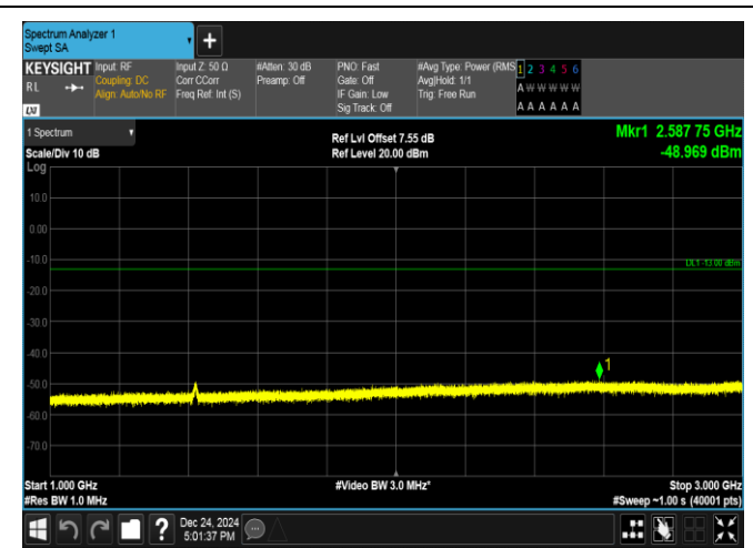
Band17-10MHz-16QAM-23790-50RB#0-1000~3000-PASS
