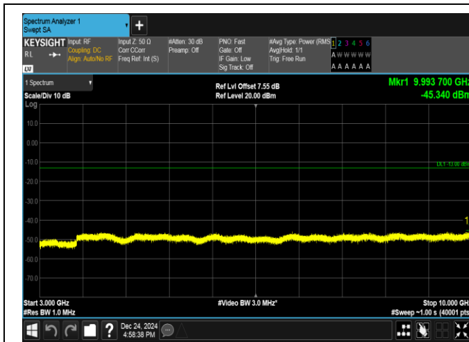
Band17-10MHz-QPSK-23790-1RB#49-3000~10000-PASS
