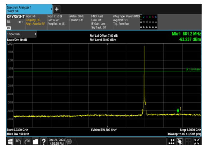
Band17-10MHz-QPSK-23790-1RB#0-30~1000-PASS
