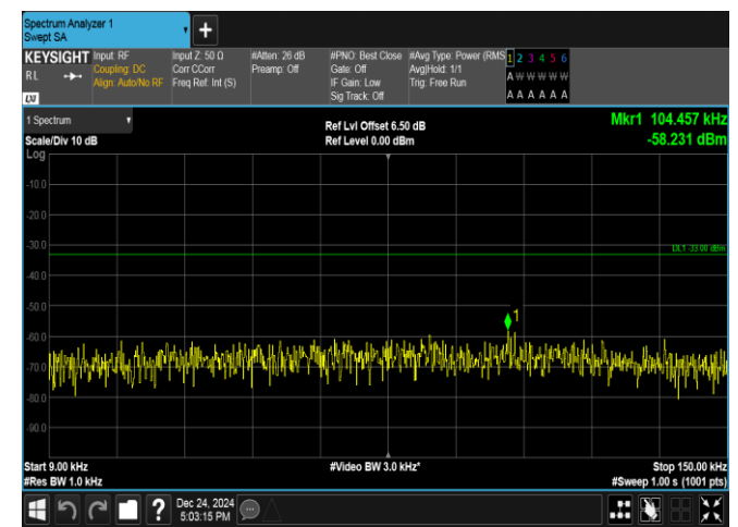
Band17-10MHz-16QAM-23800-1RB#0-0.009~0.15-PASS
