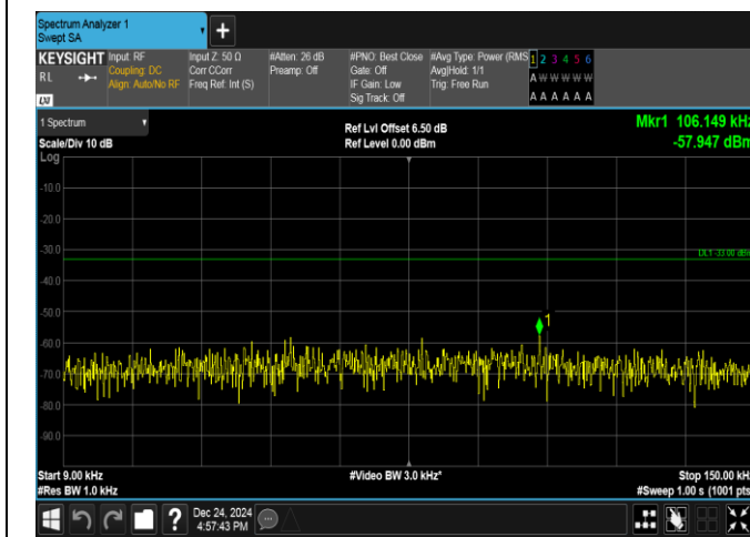
Band17-10MHz-QPSK-23790-1RB#49-0.009~0.15-PASS
