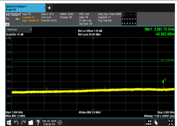
Band17-10MHz-16QAM-23800-1RB#49-1000~3000-PASS
