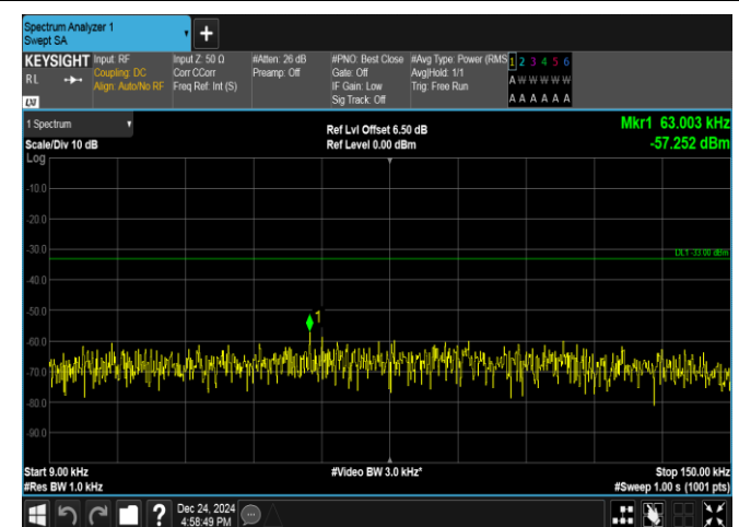
Band17-10MHz-16QAM-23790-1RB#49-0.009~0.15-PASS
