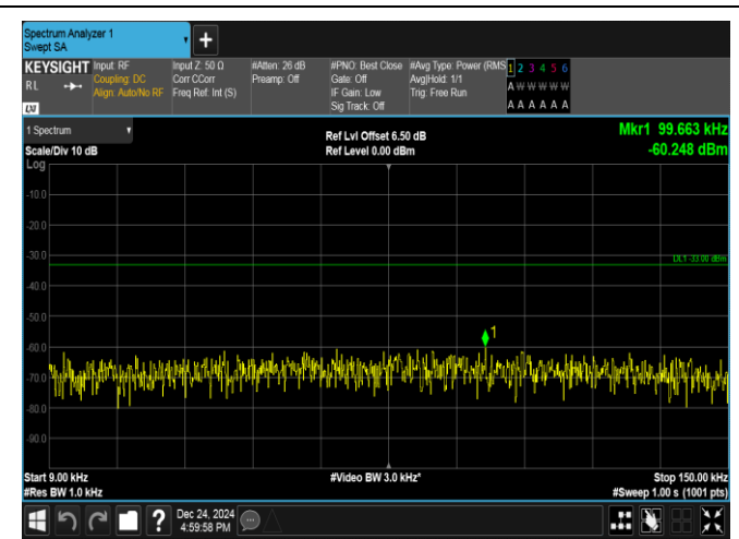
Band17-10MHz-QPSK-23790-50RB#0-0.009~0.15-PASS
