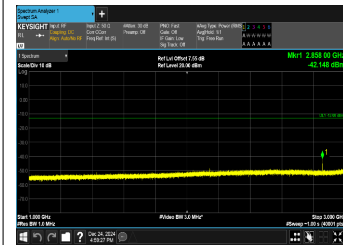
Band17-10MHz-16QAM-23790-1RB#49-1000~3000-PASS
