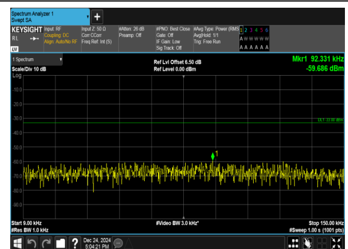
Band17-10MHz-QPSK-23800-1RB#49-0.009~0.15-PASS
