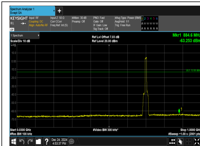
Band17-10MHz-QPSK-23780-50RB#0-30~1000-PASS
