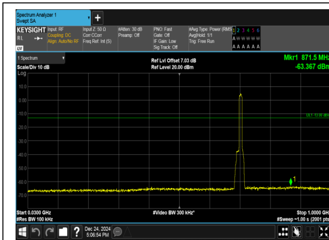
Band17-10MHz-QPSK-23800-50RB#0-30~1000-PASS
