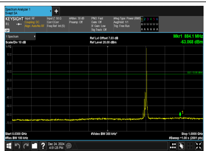
Band17-10MHz-QPSK-23780-1RB#49-30~1000-PASS
