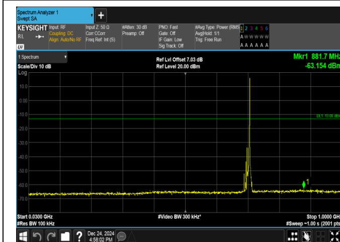
Band17-10MHz-QPSK-23790-1RB#49-30~1000-PASS
