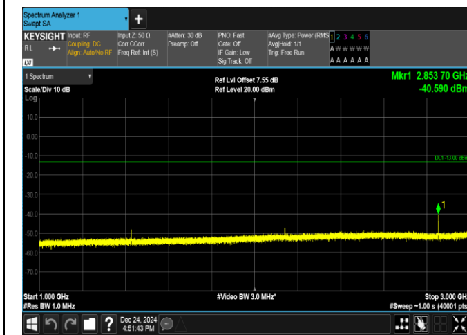
Band17-10MHz-QPSK-23780-1RB#49-1000~3000-PASS
