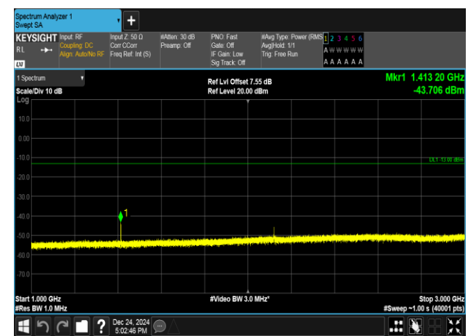
Band17-10MHz-QPSK-23800-1RB#0-1000~3000-PASS
