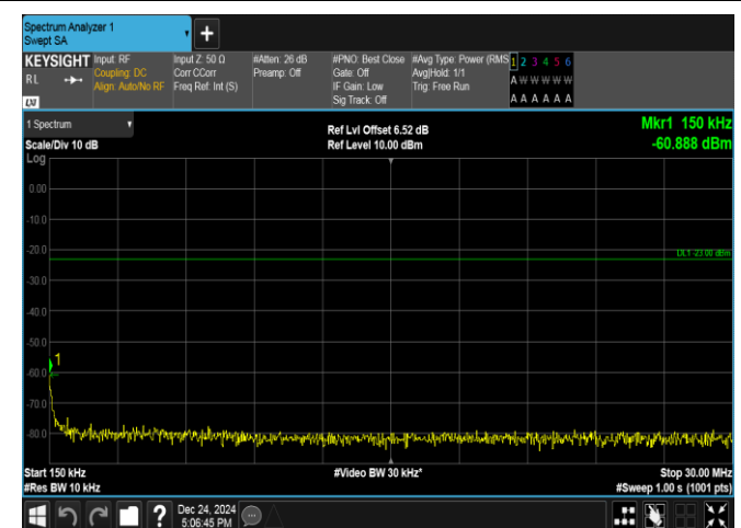
Band17-10MHz-QPSK-23800-50RB#0-0.15~30-PASS
