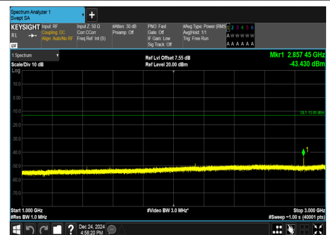
Band17-10MHz-QPSK-23790-1RB#49-1000~3000-PASS
