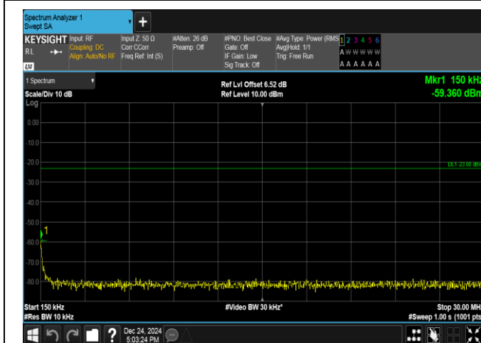
Band17-10MHz-16QAM-23800-1RB#0-0.15~30-PASS
