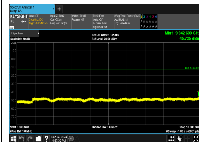
Band17-10MHz-16QAM-23790-1RB#0-3000~10000-PASS
