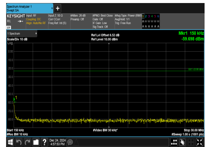
Band17-10MHz-QPSK-23790-1RB#49-0.15~30-PASS
