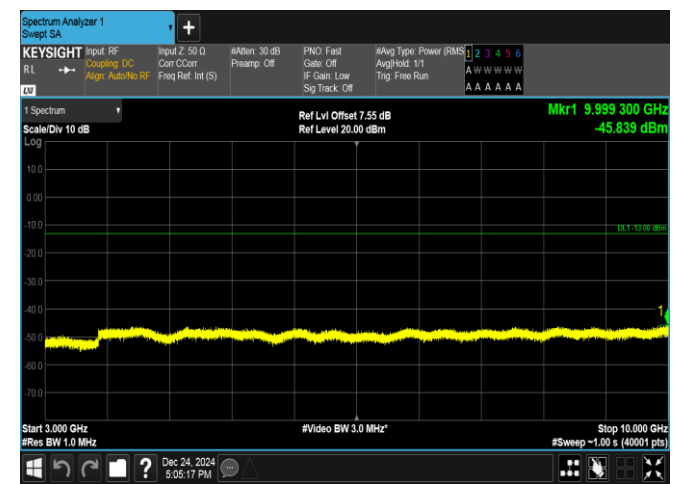
Band17-10MHz-QPSK-23800-1RB#49-3000~10000-PASS
