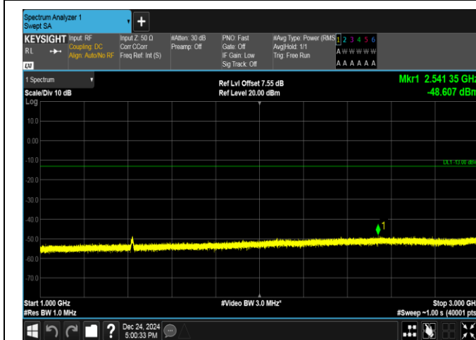
Band17-10MHz-QPSK-23790-50RB#0-1000~3000-PASS
