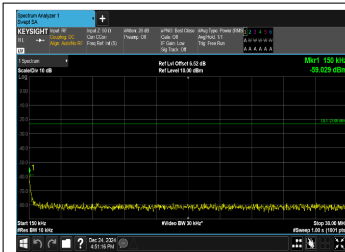
Band17-10MHz-QPSK-23780-1RB#49-0.15~30-PASS
