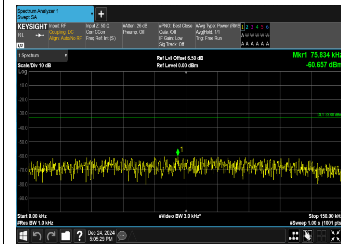
Band17-10MHz-16QAM-23800-1RB#49-0.009~0.15-PASS
