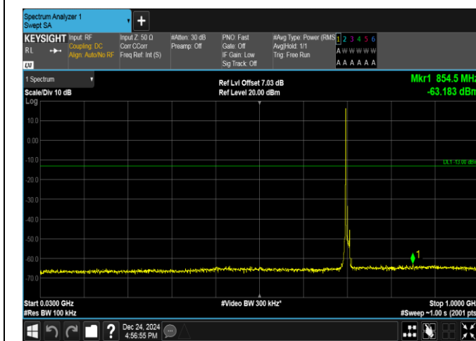
Band17-10MHz-16QAM-23790-1RB#0-30~1000-PASS
