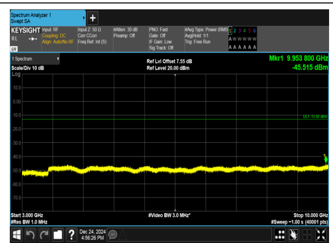
Band17-10MHz-QPSK-23790-1RB#0-3000~10000-PASS
