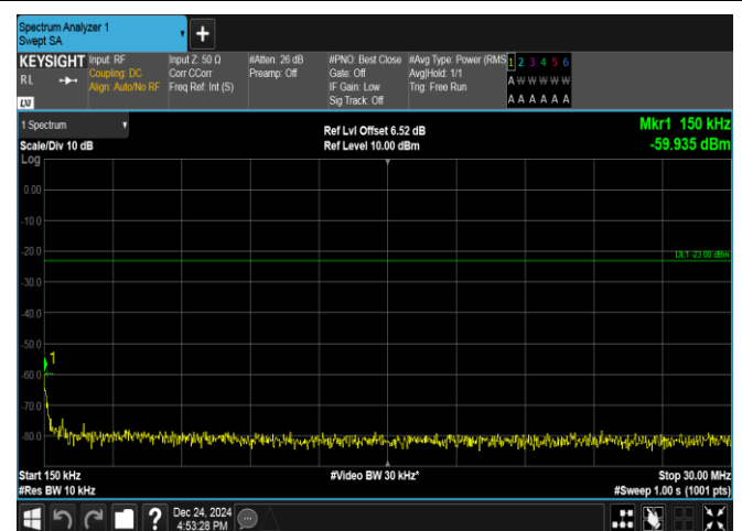
Band17-10MHz-QPSK-23780-50RB#0-0.15~30-PASS
