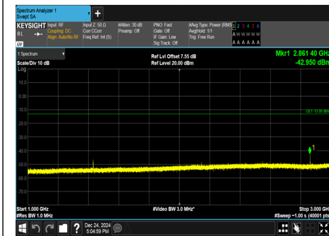
Band17-10MHz-QPSK-23800-1RB#49-1000~3000-PASS
