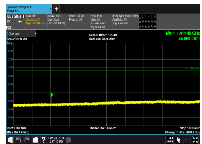
Band17-10MHz-16QAM-23790-1RB#0-1000~3000-PASS
