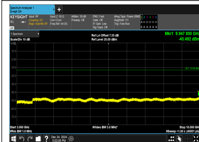
Band17-10MHz-QPSK-23800-1RB#0-3000~10000-PASS
