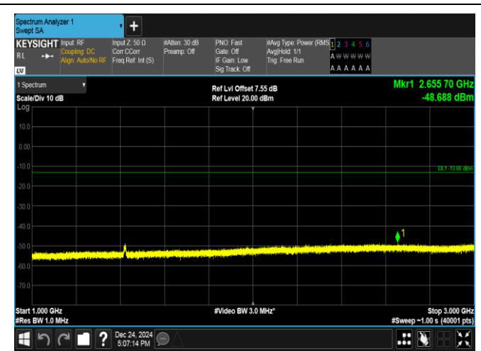
Band17-10MHz-QPSK-23800-50RB#0-1000~3000-PASS
