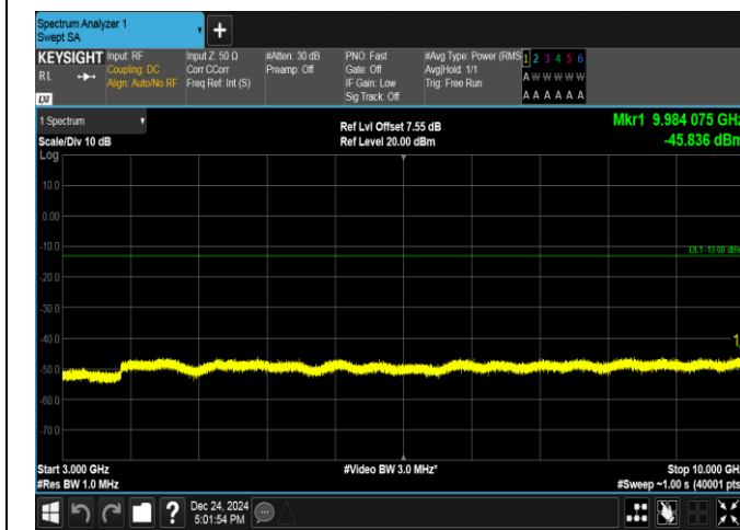
Band17-10MHz-16QAM-23790-50RB#0-3000~10000-PASS
