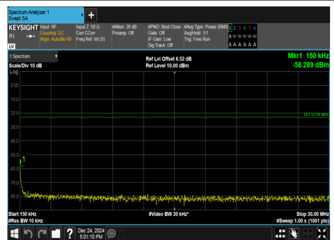
Band17-10MHz-16QAM-23790-50RB#0-0.15~30-PASS
