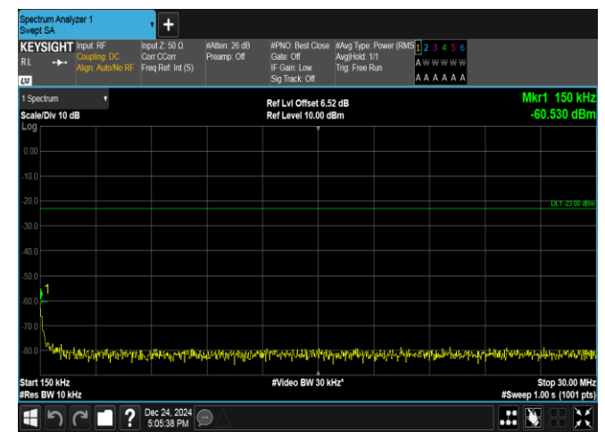
Band17-10MHz-16QAM-23800-1RB#49-0.15~30-PASS
