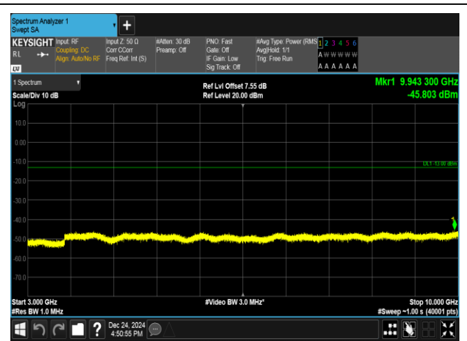
Band17-10MHz-16QAM-23780-1RB#0-3000~10000-PASS
