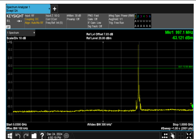
Band17-10MHz-16QAM-23780-1RB#0-30~1000-PASS
