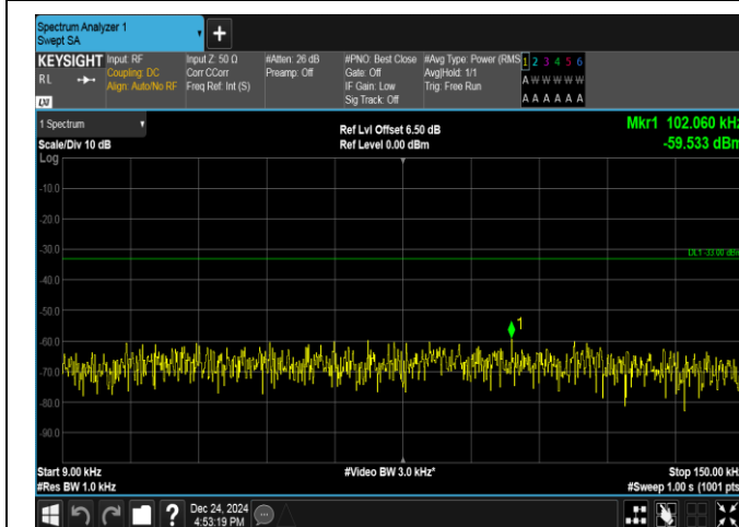
Band17-10MHz-QPSK-23780-50RB#0-0.009~0.15-PASS
