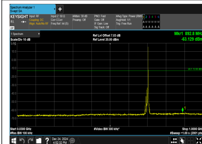
Band17-10MHz-16QAM-23780-1RB#49-30~1000-PASS
