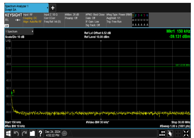
Band17-10MHz-16QAM-23780-1RB#49-0.15~30-PASS
