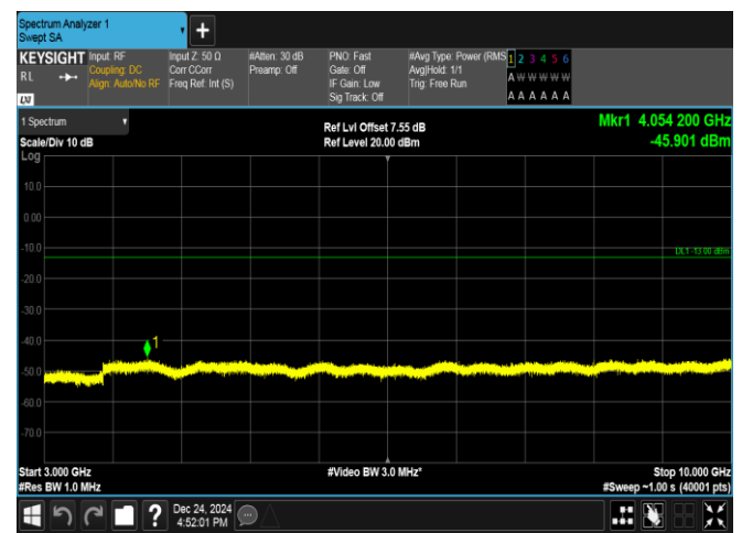
Band17-10MHz-QPSK-23780-1RB#49-3000~10000-PASS
