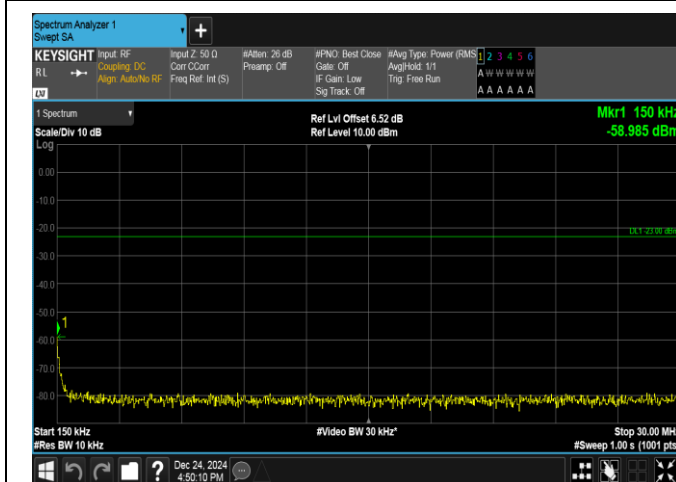
Band17-10MHz-16QAM-23780-1RB#0-0.15~30-PASS
