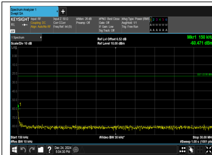
Band17-10MHz-QPSK-23800-1RB#49-0.15~30-PASS
