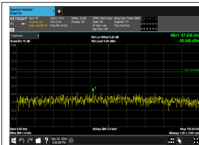
Band17-10MHz-QPSK-23800-1RB#0-0.009~0.15-PASS
