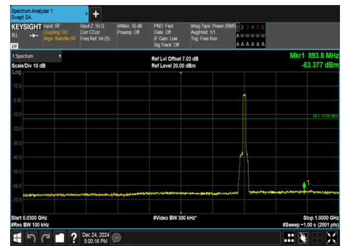
Band17-10MHz-QPSK-23790-50RB#0-30~1000-PASS
