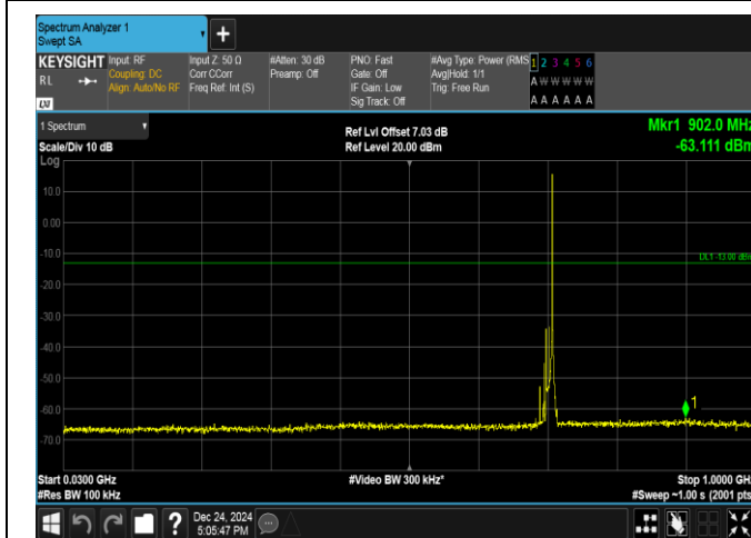
Band17-10MHz-16QAM-23800-1RB#49-30~1000-PASS
