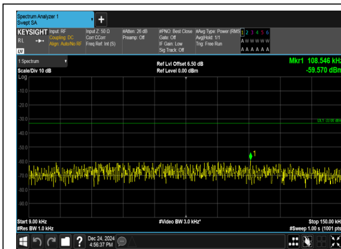
Band17-10MHz-16QAM-23790-1RB#0-0.009~0.15-PASS
