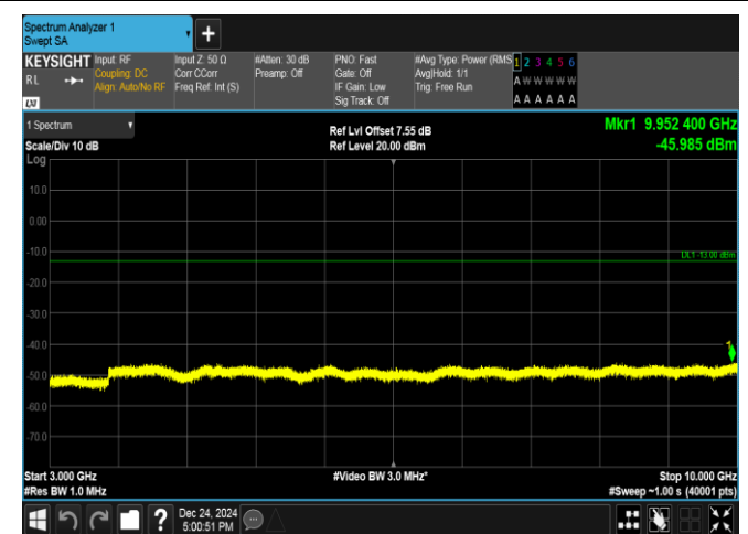
Band17-10MHz-QPSK-23790-50RB#0-3000~10000-PASS
