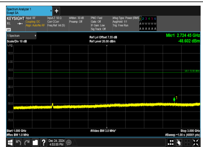
Band17-10MHz-QPSK-23780-50RB#0-1000~3000-PASS
