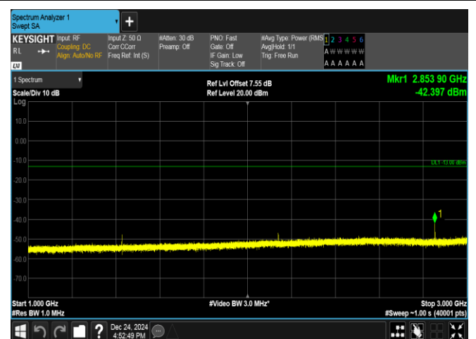
Band17-10MHz-16QAM-23780-1RB#49-1000~3000-PASS
