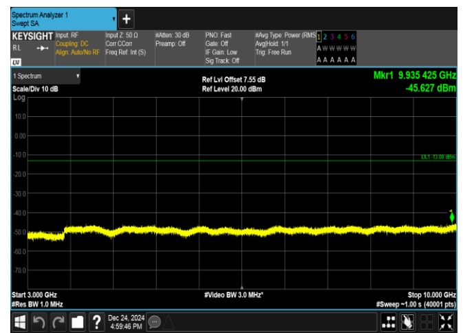
Band17-10MHz-16QAM-23790-1RB#49-3000~10000-PASS
