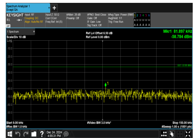
Band17-10MHz-QPSK-23790-1RB#0-0.009~0.15-PASS
