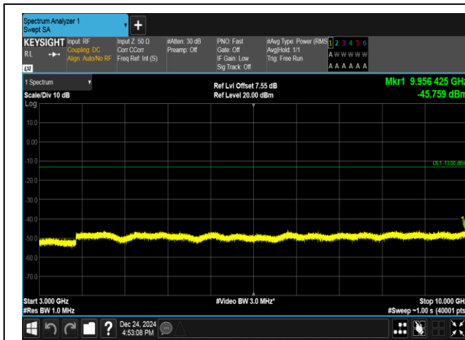
Band17-10MHz-16QAM-23780-1RB#49-3000~10000-PASS
