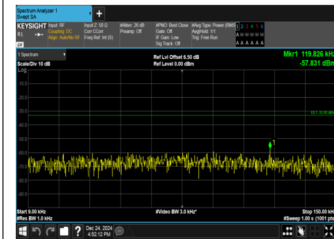
Band17-10MHz-16QAM-23780-1RB#49-0.009~0.15-PASS
