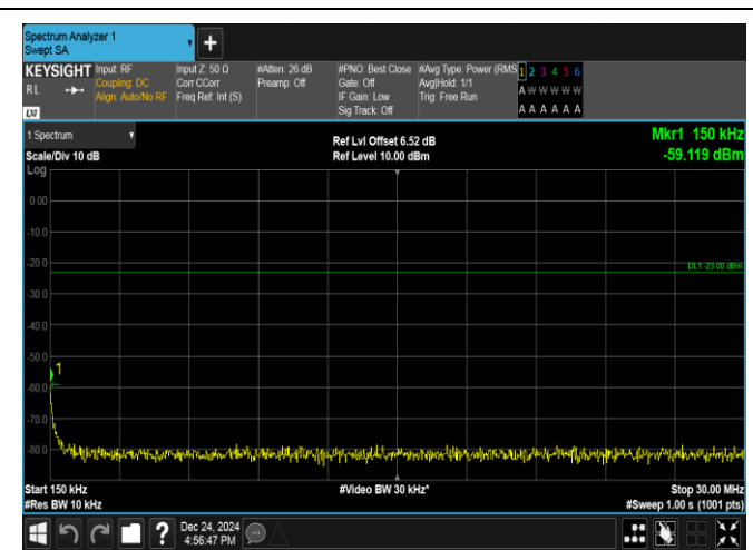
Band17-10MHz-16QAM-23790-1RB#0-0.15~30-PASS
