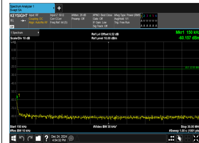
Band17-10MHz-16QAM-23780-50RB#0-0.15~30-PASS
