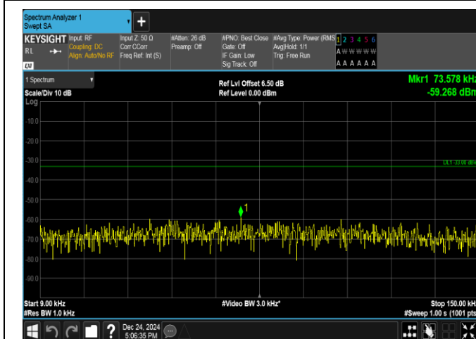
Band17-10MHz-QPSK-23800-50RB#0-0.009~0.15-PASS
