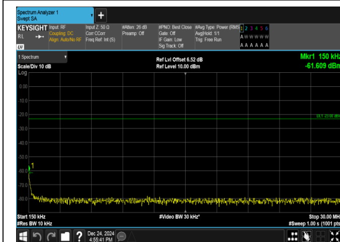
Band17-10MHz-QPSK-23790-1RB#0-0.15~30-PASS
