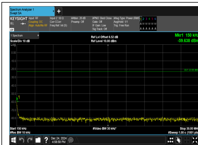
Band17-10MHz-16QAM-23790-1RB#49-0.15~30-PASS
