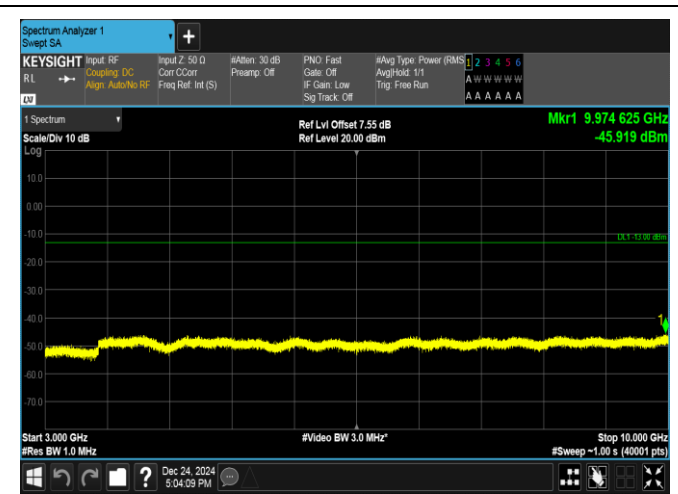
Band17-10MHz-16QAM-23800-1RB#0-3000~10000-PASS
