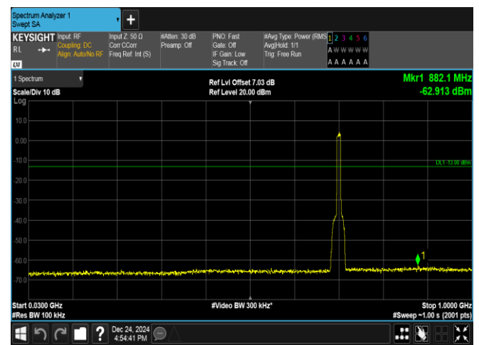
Band17-10MHz-16QAM-23780-50RB#0-30~1000-PASS
