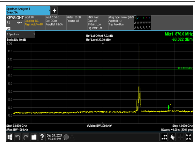
Band17-10MHz-QPSK-23800-1RB#49-30~1000-PASS
