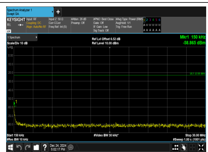
Band17-10MHz-QPSK-23800-1RB#0-0.15~30-PASS
