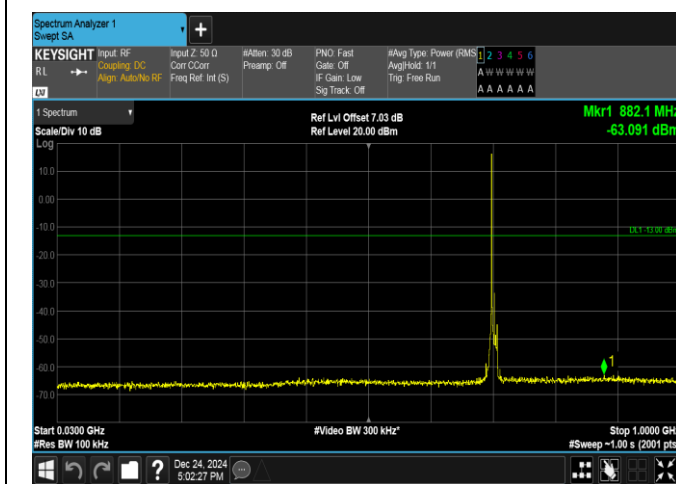
Band17-10MHz-QPSK-23800-1RB#0-30~1000-PASS
