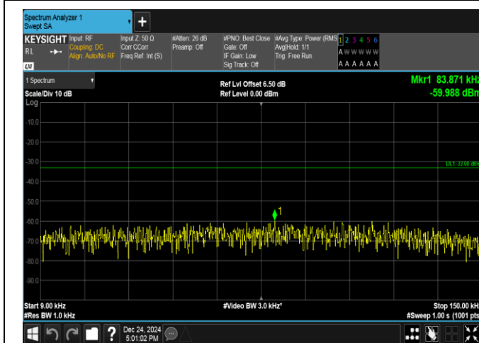
Band17-10MHz-16QAM-23790-50RB#0-0.009~0.15-PASS
