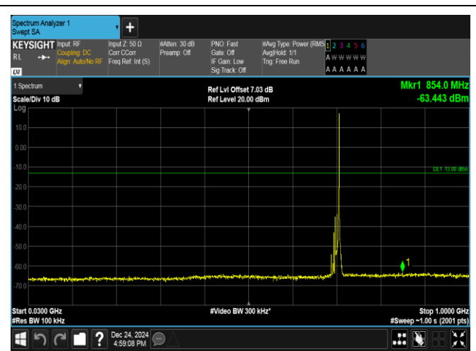
Band17-10MHz-16QAM-23790-1RB#49-30~1000-PASS
