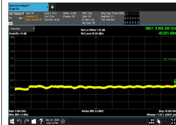
Band17-10MHz-QPSK-23780-50RB#0-3000~10000-PASS
