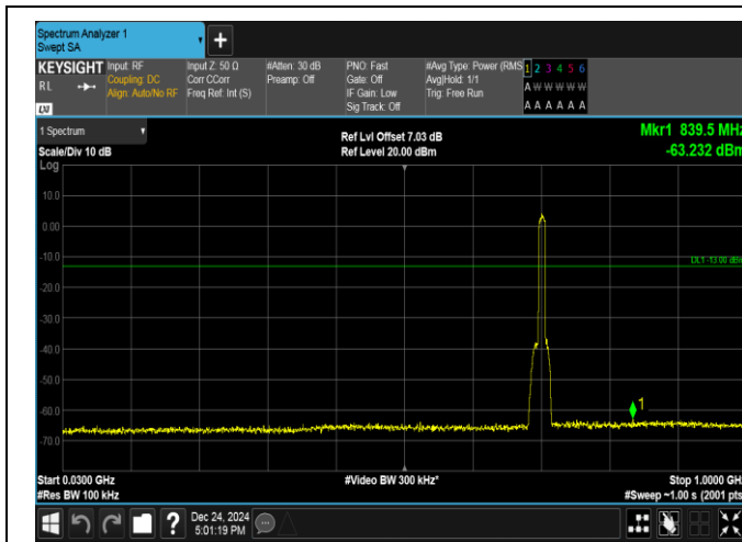
Band17-10MHz-16QAM-23790-50RB#0-30~1000-PASS
