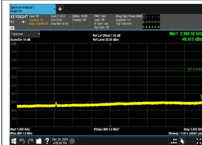
Band17-10MHz-16QAM-23780-50RB#0-1000~3000-PASS
