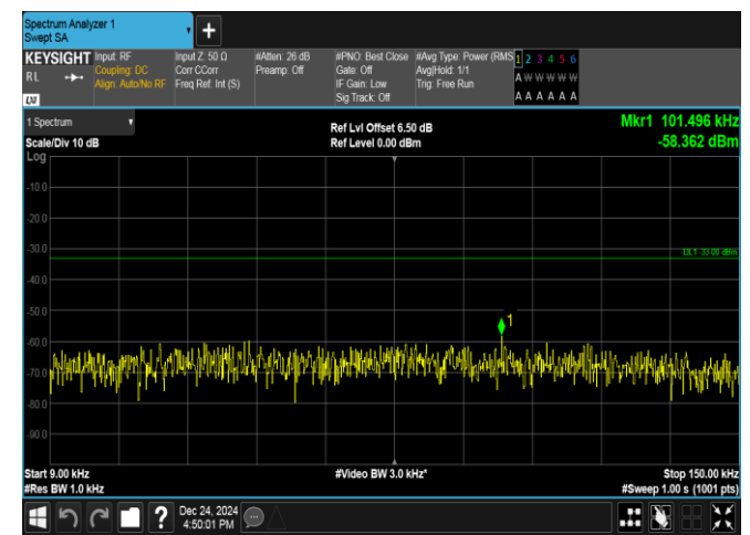
Band17-10MHz-16QAM-23780-1RB#0-0.009~0.15-PASS
