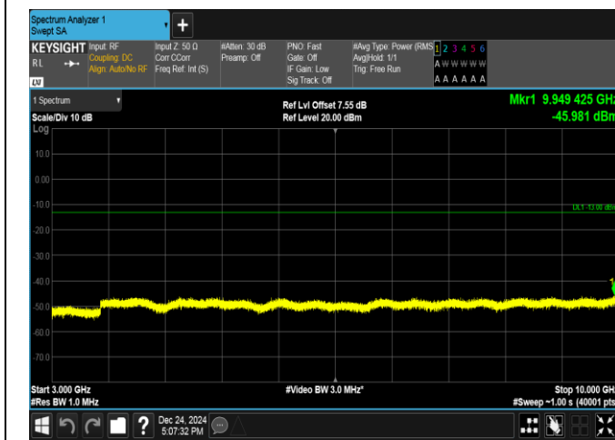
Band17-10MHz-QPSK-23800-50RB#0-3000~10000-PASS
