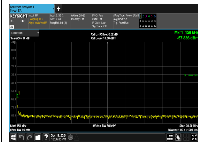
Band2-20MHz-16QAM-19100-100RB#0-0.15~30-PASS
