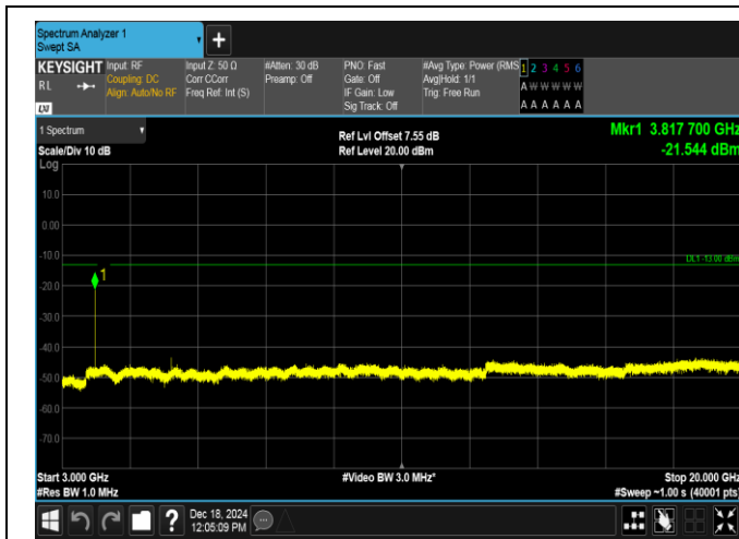
Band2-20MHz-16QAM-19100-1RB#99-3000~20000-PASS
