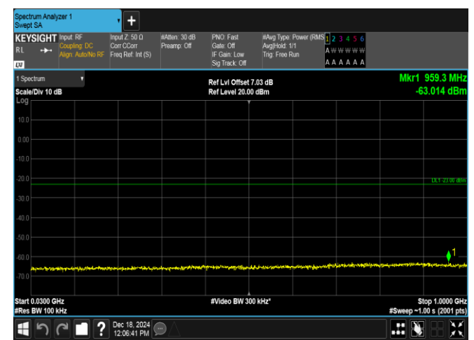
Band2-20MHz-16QAM-19100-100RB#0-30~1000-PASS
