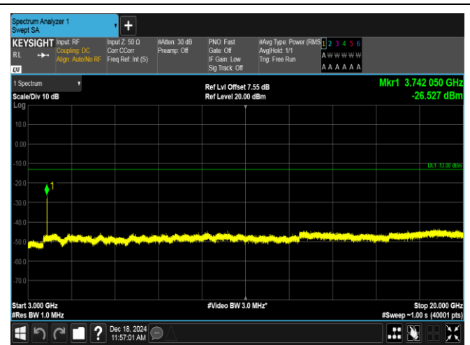
Band2-20MHz-QPSK-18900-1RB#0-3000~20000-PASS
