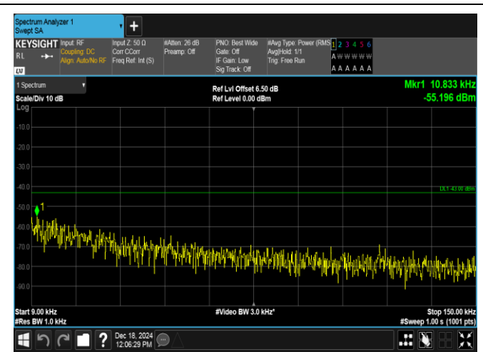
Band2-20MHz-16QAM-19100-100RB#0-0.009~0.15-PASS
