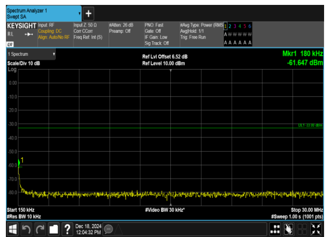
Band2-20MHz-16QAM-19100-1RB#99-0.15~30-PASS
