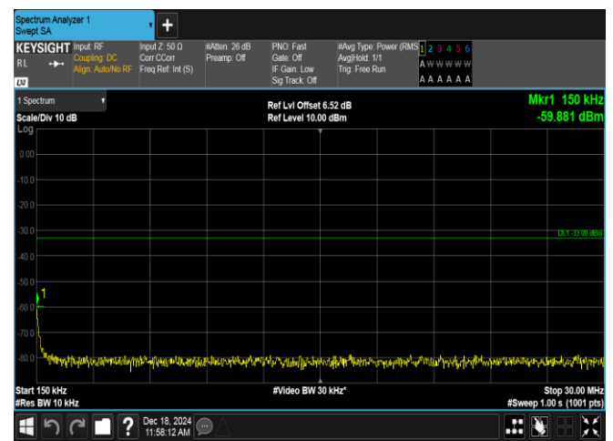
Band2-20MHz-QPSK-18900-1RB#99-0.15~30-PASS
