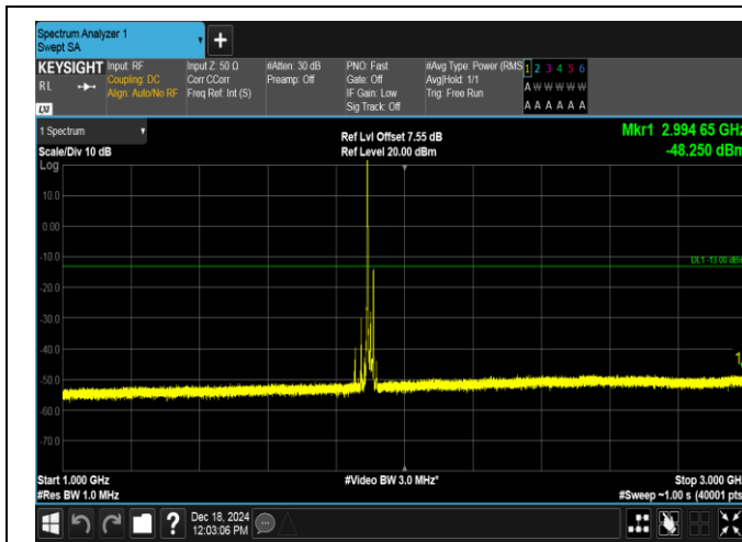
Band2-20MHz-16QAM-19100-1RB#0-1000~3000-PASS
