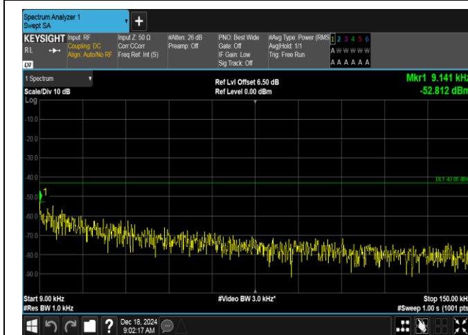
Band2-3MHz-QPSK-18615-15RB#0-0.009~0.15-PASS
