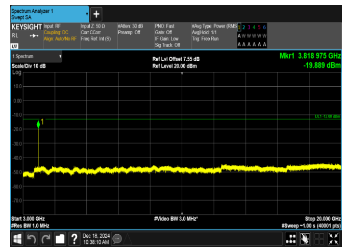
Band2-10MHz-QPSK-19150-1RB#49-3000~20000-PASS
