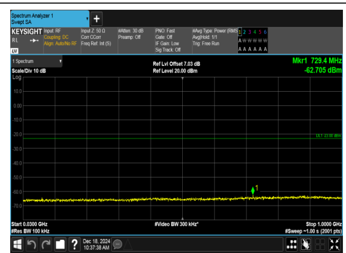
Band2-10MHz-QPSK-19150-1RB#49-30~1000-PASS
