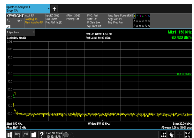
Band2-10MHz-QPSK-19150-50RB#0-0.15~30-PASS
