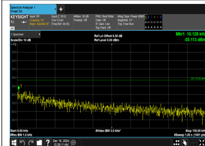
Band2-10MHz-QPSK-19150-50RB#0-0.009~0.15-PASS
