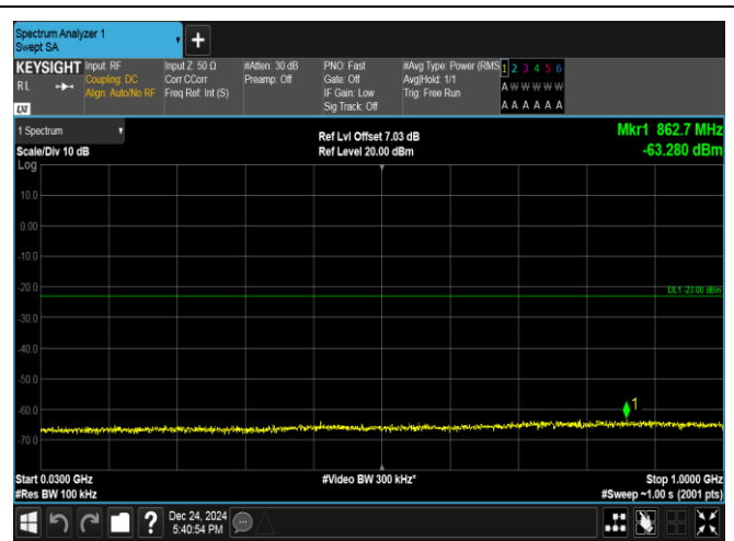
Band25-1.4MHz-QPSK-26047-1RB#5-30~1000-PASS
