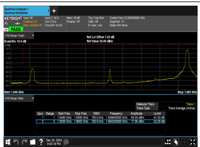
Band25-15MHz-16QAM-26115-1RB#74-PASS
