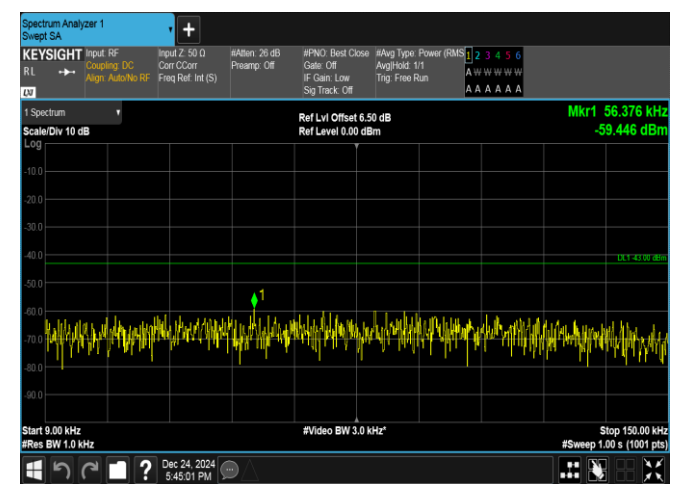
Band25-1.4MHz-QPSK-26365-1RB#0-0.009~0.15-PASS
