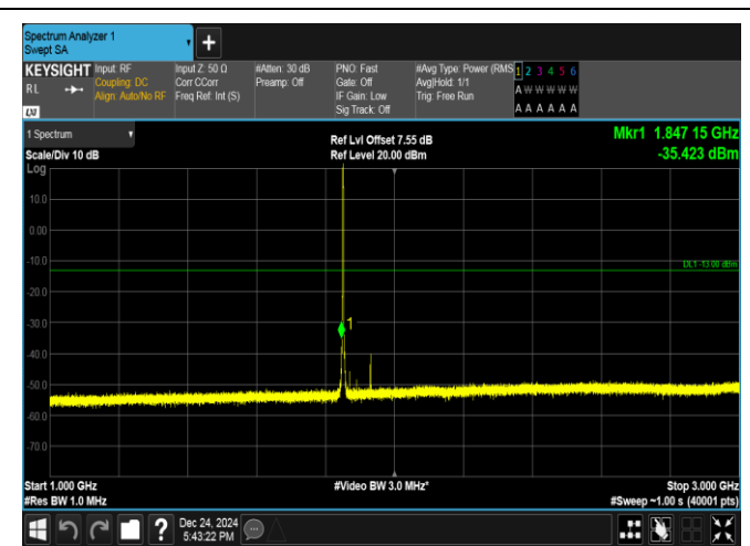
Band25-1.4MHz-QPSK-26047-6RB#0-1000~3000-PASS
