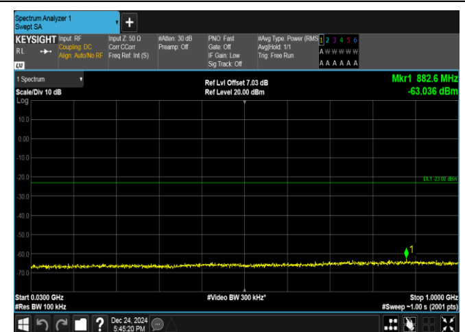
Band25-1.4MHz-QPSK-26365-1RB#0-30~1000-PASS
