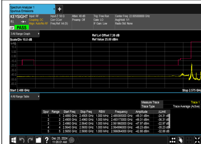
Band38-5MHz-16QAM-37775-1RB#0-PASS
