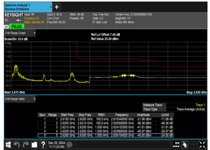
Band38-5MHz-16QAM-38225-1RB#0-PASS
