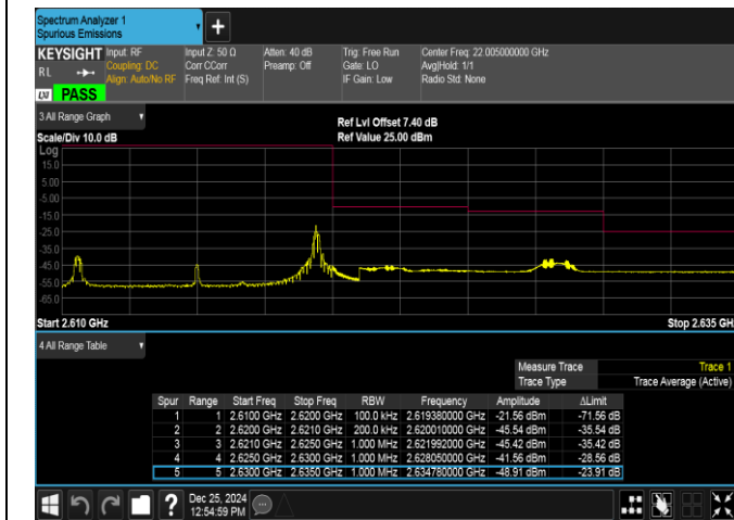
Band38-10MHz-QPSK-38200-1RB#49-PASS
