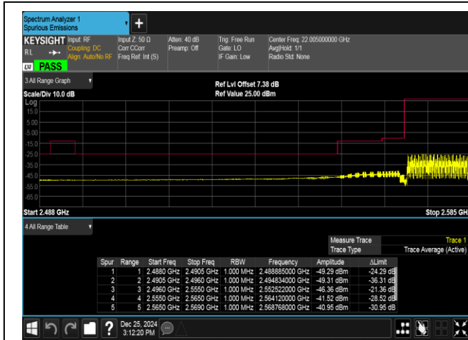
Band38-15MHz-QPSK-37825-75RB#0-PASS
