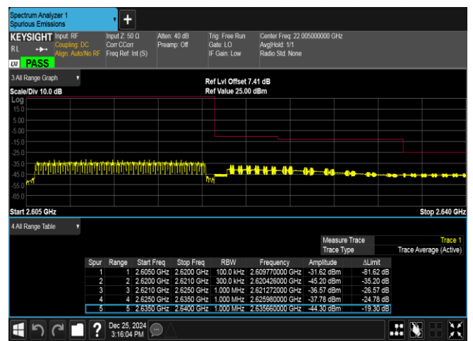
Band38-15MHz-QPSK-38175-75RB#0-PASS
