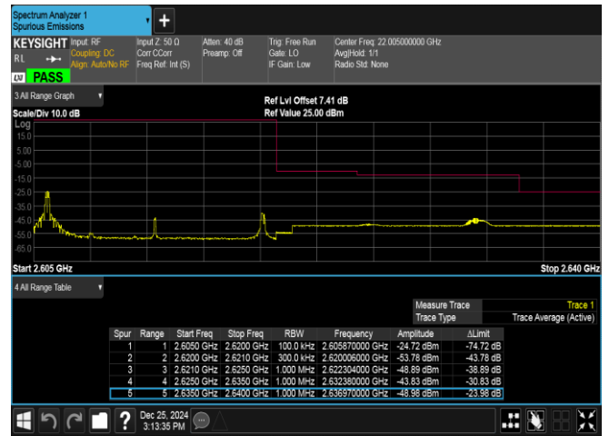
Band38-15MHz-QPSK-38175-1RB#0-PASS
