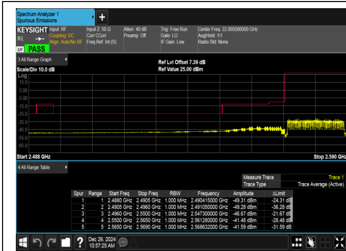
Band38-20MHz-QPSK-37850-100RB#0-PASS
