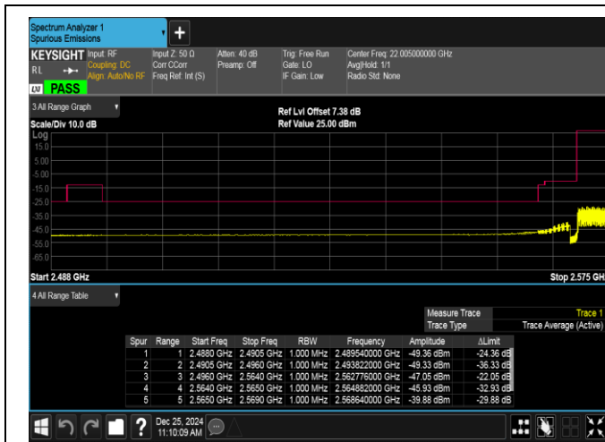
Band38-5MHz-16QAM-37775-25RB#0-PASS
