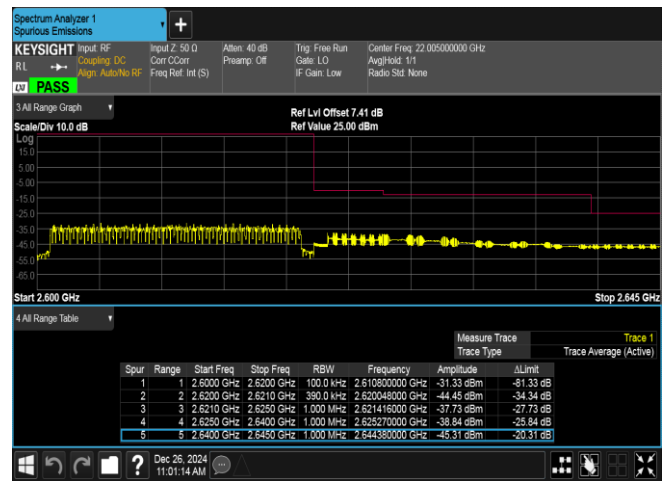
Band38-20MHz-QPSK-38150-100RB#0-PASS
