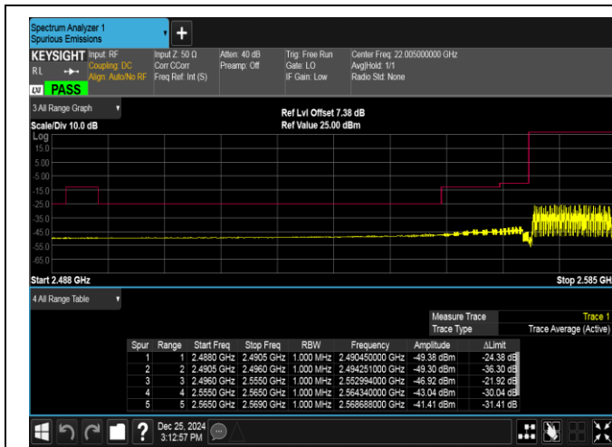
Band38-15MHz-16QAM-37825-75RB#0-PASS
