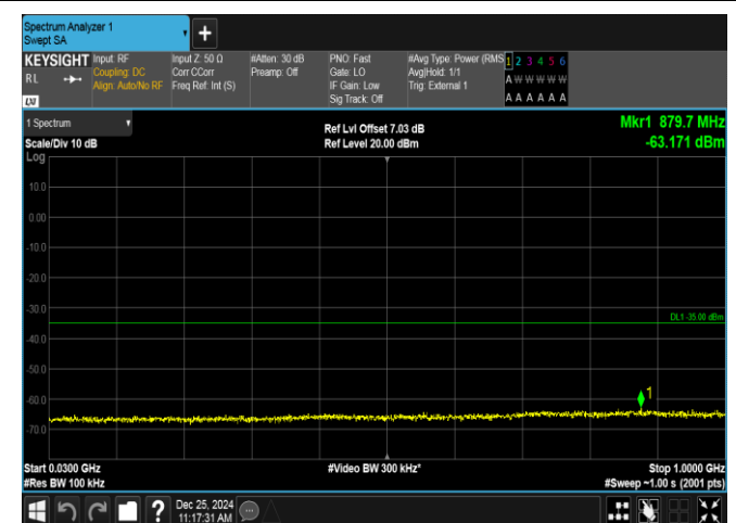
Band38-5MHz-QPSK-37775-1RB#24-30~1000-PASS
