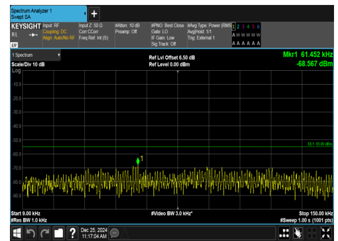
Band38-5MHz-QPSK-37775-1RB#24-0.009~0.15-PASS
