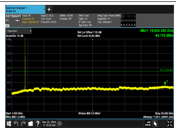
Band38-5MHz-QPSK-37775-1RB#0-1000~20000-PASS
