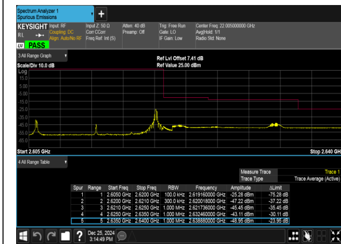
Band38-15MHz-QPSK-38175-1RB#74-PASS
