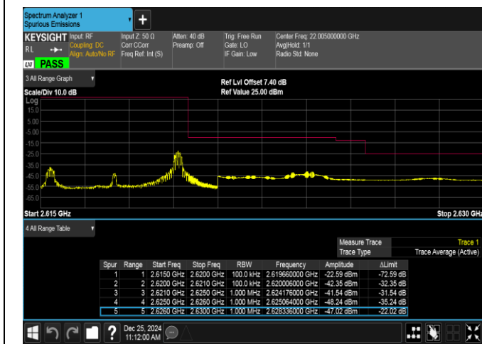
Band38-5MHz-QPSK-38225-1RB#24-PASS
