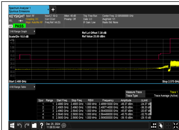
Band38-5MHz-QPSK-37775-25RB#0-PASS
