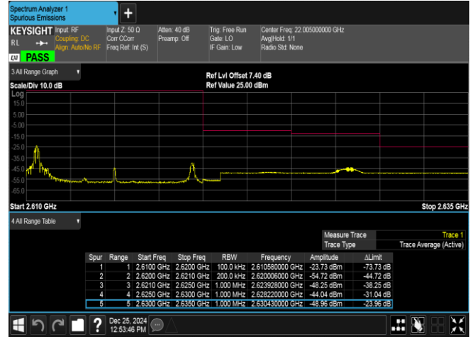
Band38-10MHz-QPSK-38200-1RB#0-PASS
