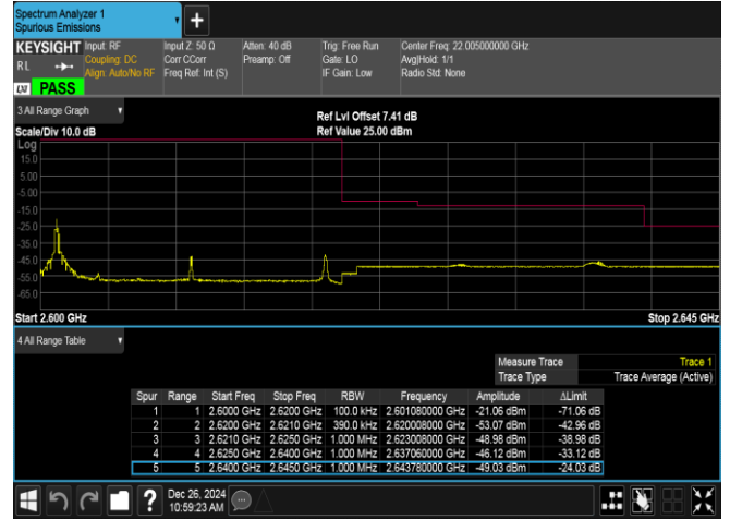
Band38-20MHz-16QAM-38150-1RB#0-PASS
