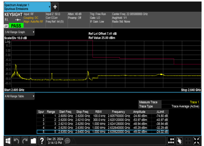
Band38-15MHz-16QAM-38175-1RB#0-PASS
