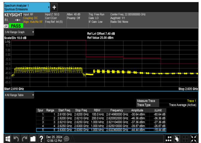
Band38-10MHz-QPSK-38200-50RB#0-PASS
