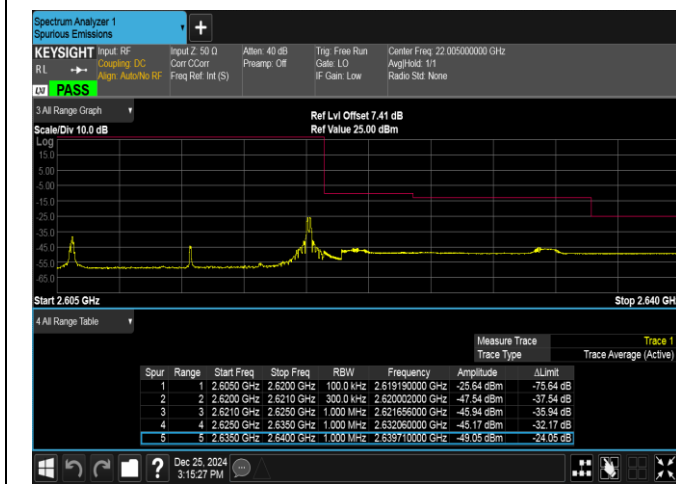
Band38-15MHz-16QAM-38175-1RB#74-PASS
