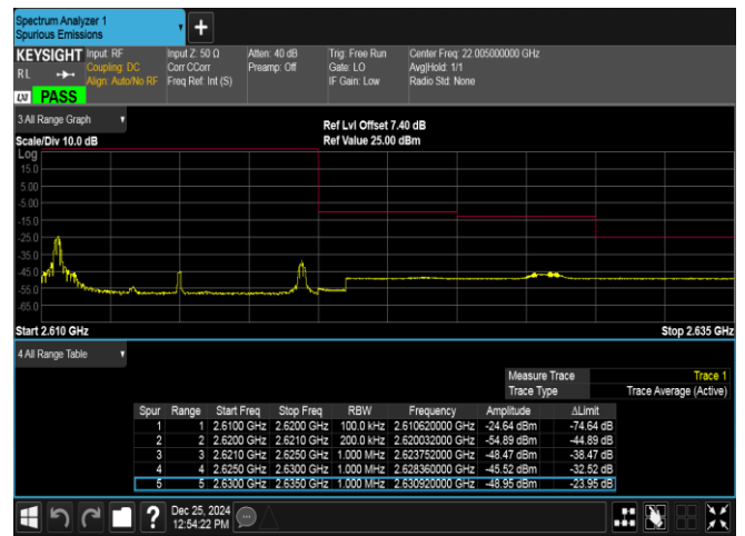
Band38-10MHz-16QAM-38200-1RB#0-PASS
