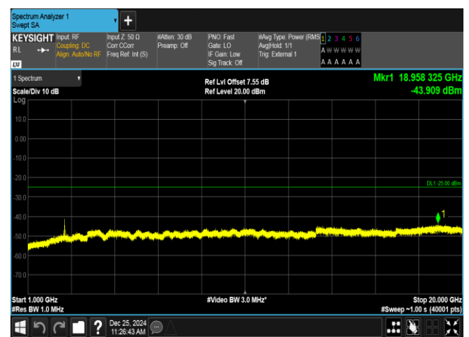
Band38-5MHz-QPSK-38000-1RB#24-1000~20000-PASS
