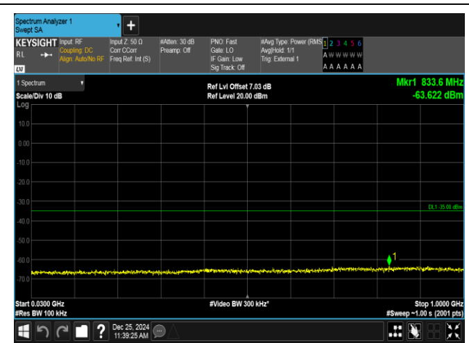
Band38-5MHz-16QAM-38225-25RB#0-30~1000-PASS
