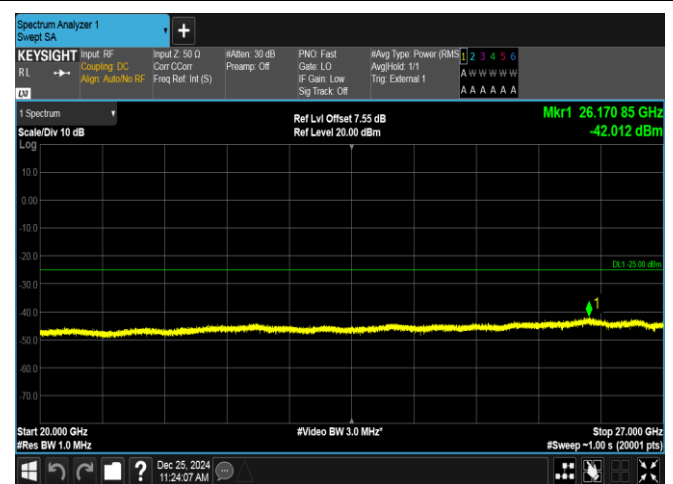
Band38-5MHz-QPSK-38000-1RB#0-20000~27000-PASS
