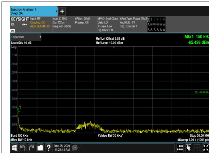
Band38-5MHz-16QAM-37775-25RB#0-0.15~30-PASS
