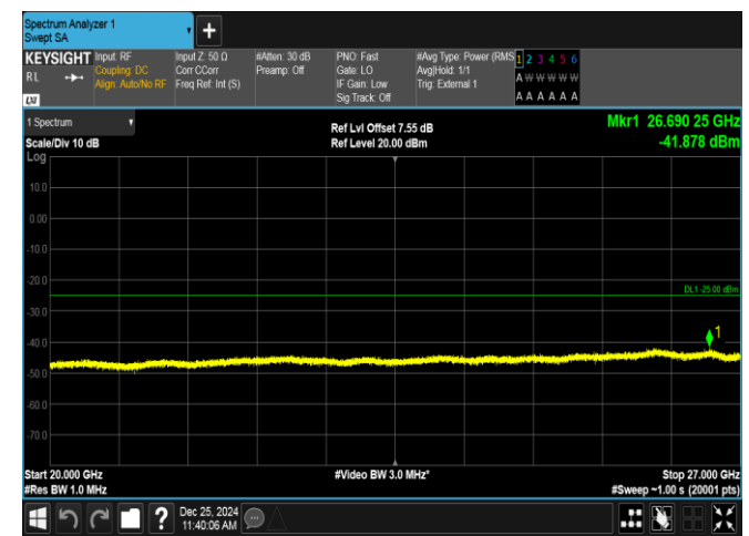
Band38-5MHz-16QAM-38225-25RB#0-20000~27000-PASS
