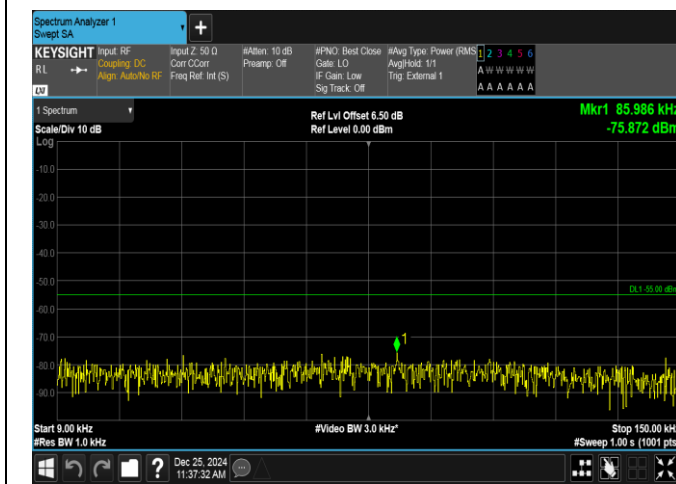
Band38-5MHz-QPSK-38225-25RB#0-0.009~0.15-PASS
