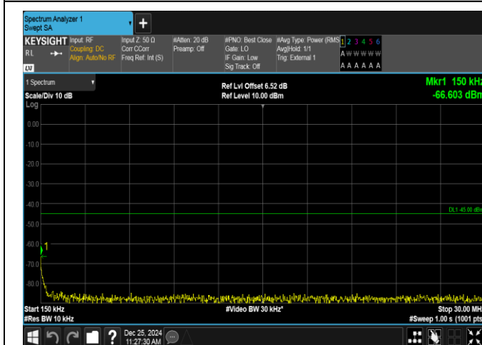
Band38-5MHz-16QAM-38000-1RB#24-0.15~30-PASS
