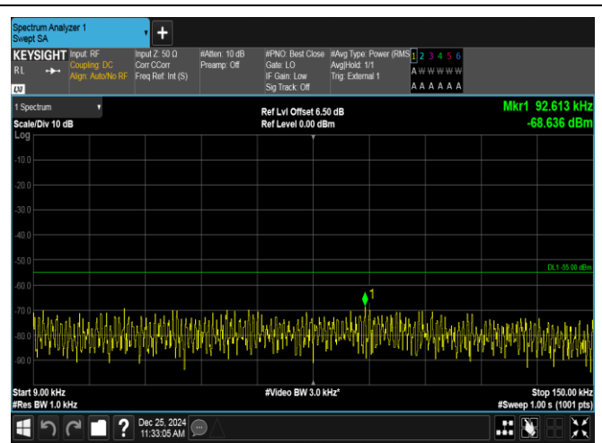
Band38-5MHz-16QAM-38225-1RB#0-0.009~0.15-PASS
