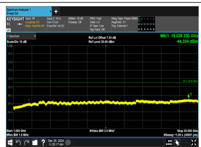
Band38-5MHz-16QAM-38000-1RB#0-1000~20000-PASS
