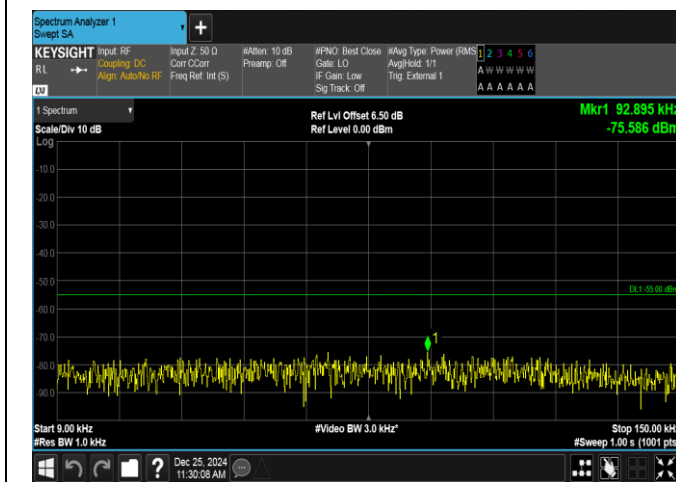
Band38-5MHz-16QAM-38000-25RB#0-0.009~0.15-PASS
