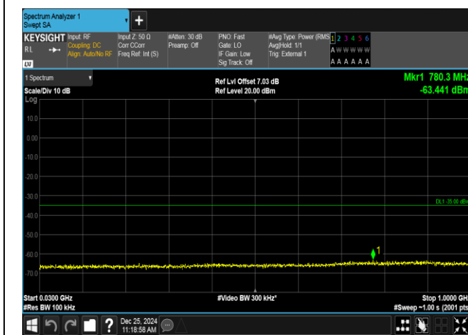
Band38-5MHz-16QAM-37775-1RB#24-30~1000-PASS
