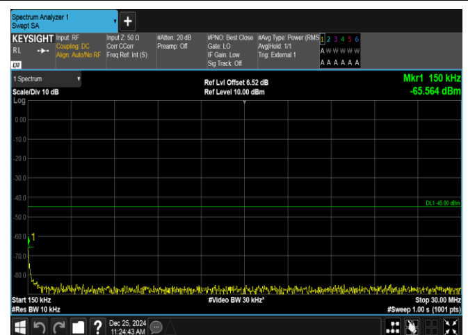
Band38-5MHz-16QAM-38000-1RB#0-0.15~30-PASS
