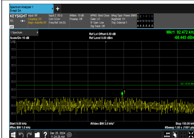
Band38-5MHz-16QAM-38000-1RB#0-0.009~0.15-PASS
