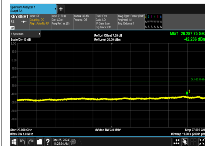
Band38-5MHz-16QAM-38000-1RB#0-20000~27000-PASS
