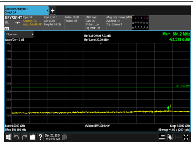
Band38-5MHz-16QAM-37775-25RB#0-30~1000-PASS
