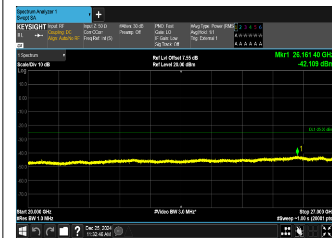
Band38-5MHz-QPSK-38225-1RB#0-20000~27000-PASS
