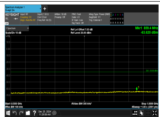
Band38-5MHz-QPSK-38000-25RB#0-30~1000-PASS
