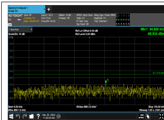
Band38-5MHz-QPSK-38000-1RB#24-0.009~0.15-PASS
