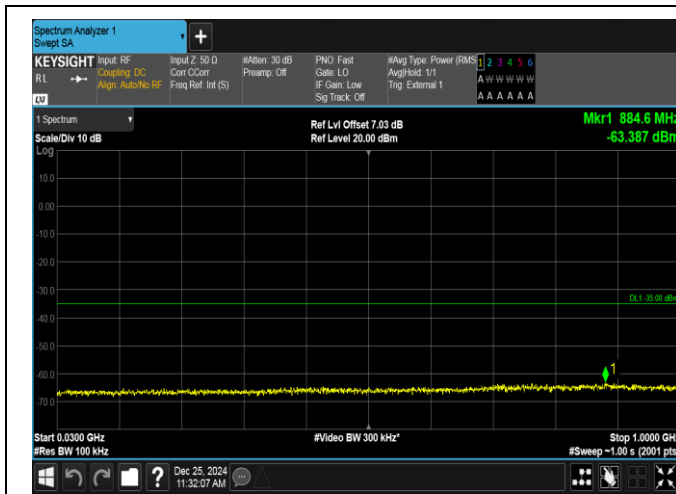
Band38-5MHz-QPSK-38225-1RB#0-30~1000-PASS
