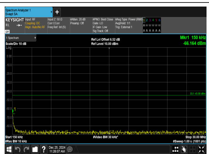
Band38-5MHz-QPSK-38000-1RB#24-0.15~30-PASS
