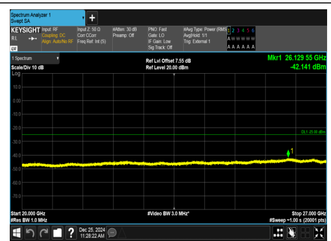
Band38-5MHz-16QAM-38000-1RB#24-20000~27000-PASS
