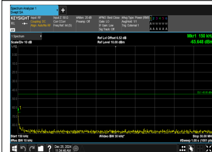
Band38-5MHz-QPSK-38225-1RB#24-0.15~30-PASS
