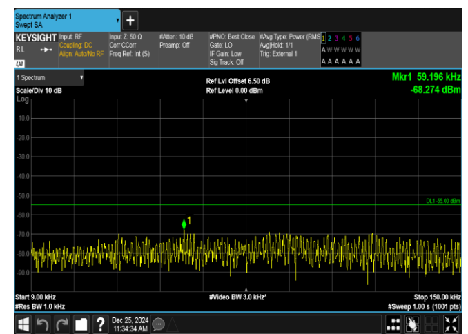
Band38-5MHz-QPSK-38225-1RB#24-0.009~0.15-PASS
