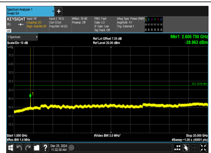
Band38-5MHz-QPSK-38225-1RB#0-1000~20000-PASS
