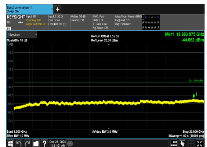
Band38-5MHz-16QAM-38000-25RB#0-1000~20000-PASS
