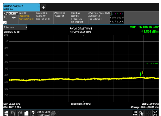
Band38-5MHz-16QAM-38225-1RB#0-20000~27000-PASS
