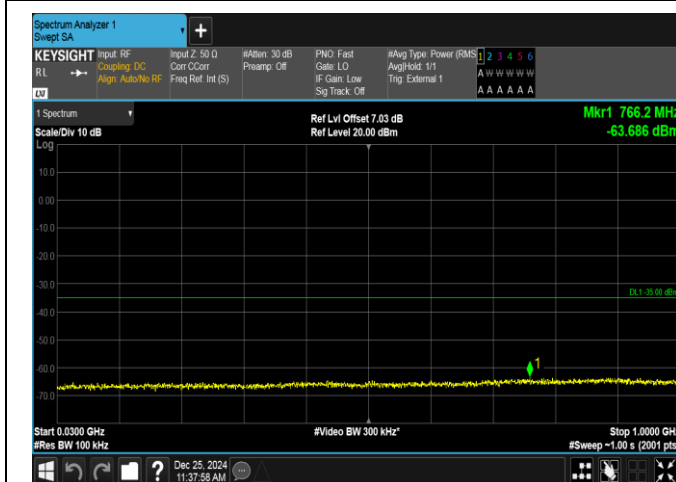
Band38-5MHz-QPSK-38225-25RB#0-30~1000-PASS
