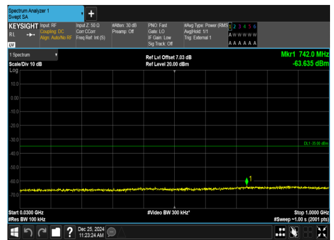
Band38-5MHz-QPSK-38000-1RB#0-30~1000-PASS
