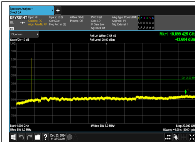
Band38-5MHz-QPSK-38225-1RB#24-1000~20000-PASS
