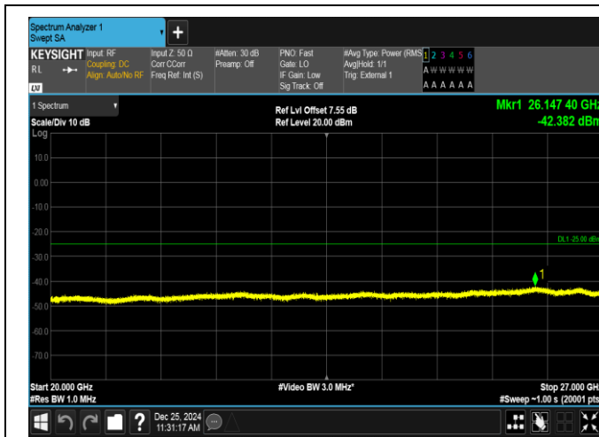
Band38-5MHz-16QAM-38000-25RB#0-20000~27000-PASS
