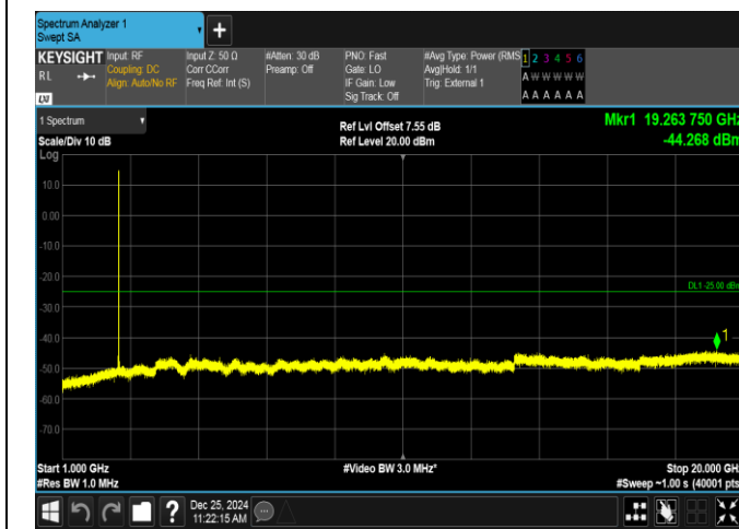
Band38-5MHz-16QAM-37775-25RB#0-1000~20000-PASS
