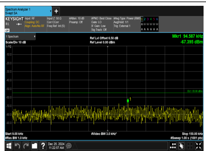
Band38-5MHz-QPSK-38000-1RB#0-0.009~0.15-PASS
