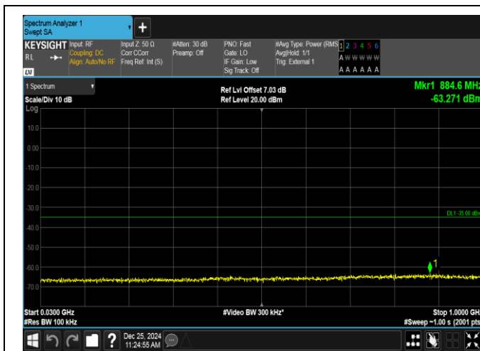
Band38-5MHz-16QAM-38000-1RB#0-30~1000-PASS
