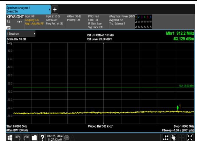
Band38-5MHz-16QAM-38000-1RB#24-30~1000-PASS
