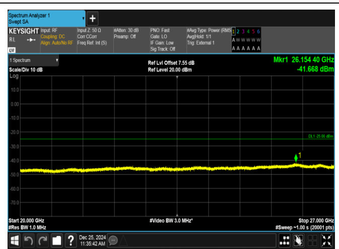
Band38-5MHz-QPSK-38225-1RB#24-20000~27000-PASS
