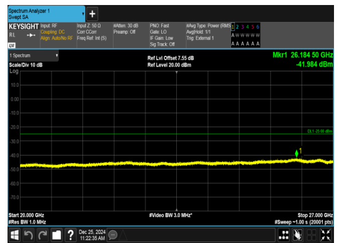
Band38-5MHz-16QAM-37775-25RB#0-20000~27000-PASS
