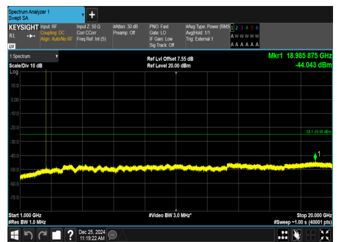
Band38-5MHz-16QAM-37775-1RB#24-1000~20000-PASS
