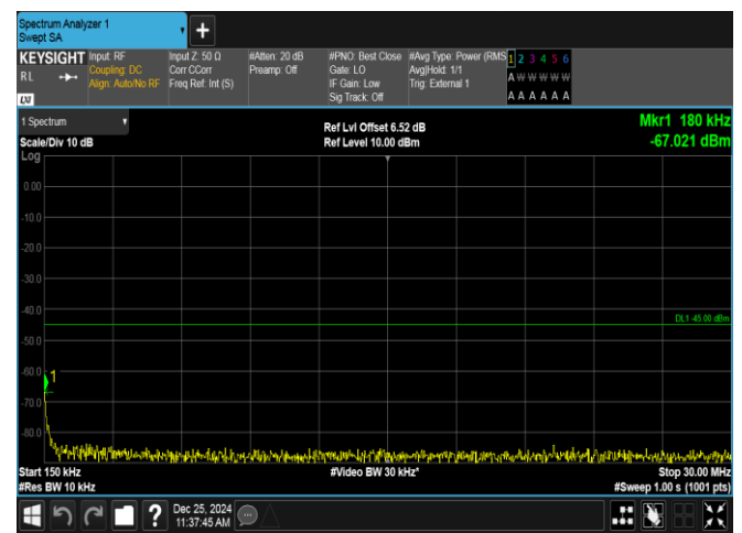
Band38-5MHz-QPSK-38225-25RB#0-0.15~30-PASS
