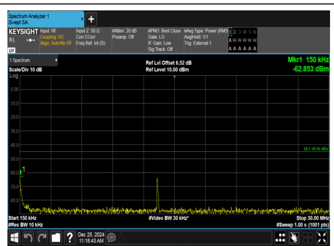
Band38-5MHz-16QAM-37775-1RB#24-0.15~30-PASS
