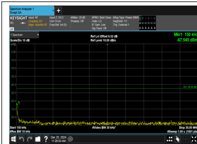
Band38-5MHz-QPSK-38000-25RB#0-0.15~30-PASS
