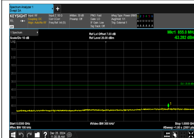
Band38-5MHz-16QAM-38000-25RB#0-30~1000-PASS
