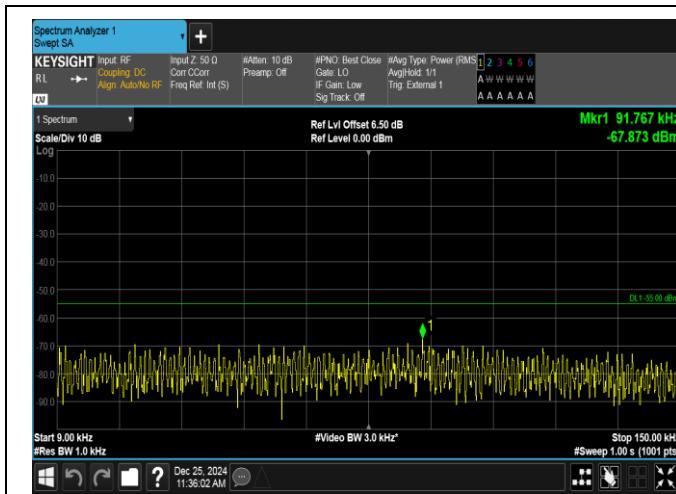
Band38-5MHz-16QAM-38225-1RB#24-0.009~0.15-PASS
