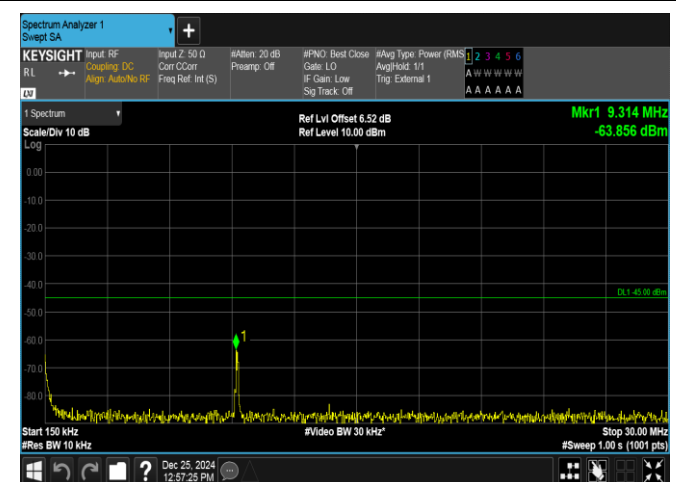
Band38-10MHz-QPSK-37800-1RB#0-0.15~30-PASS
