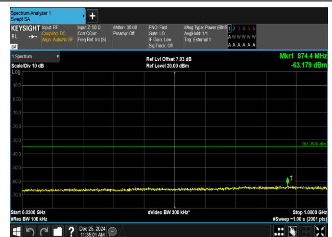
Band38-5MHz-QPSK-38225-1RB#24-30~1000-PASS
