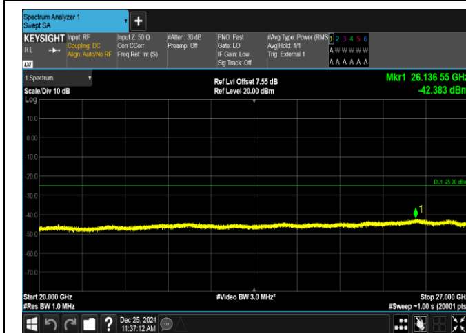
Band38-5MHz-16QAM-38225-1RB#24-20000~27000-PASS
