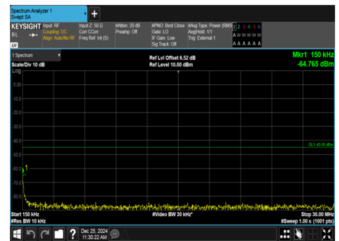
Band38-5MHz-16QAM-38000-25RB#0-0.15~30-PASS
