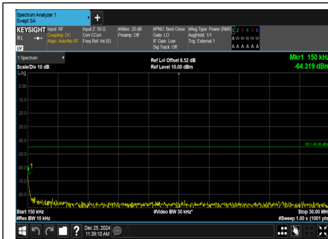
Band38-5MHz-16QAM-38225-25RB#0-0.15~30-PASS
