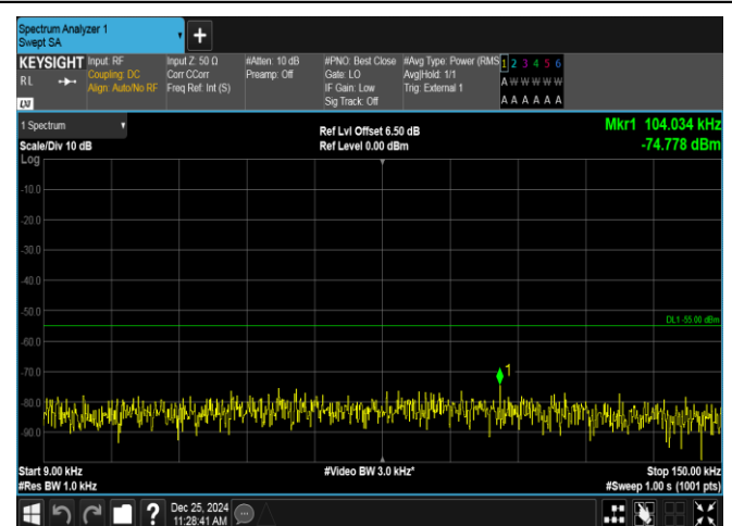
Band38-5MHz-QPSK-38000-25RB#0-0.009~0.15-PASS
