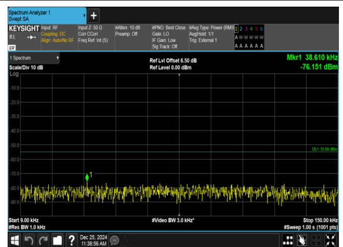
Band38-5MHz-16QAM-38225-25RB#0-0.009~0.15-PASS
