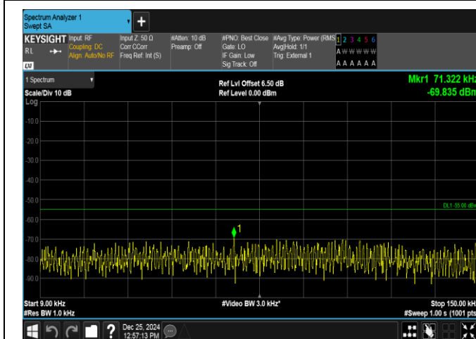
Band38-10MHz-QPSK-37800-1RB#0-0.009~0.15-PASS
