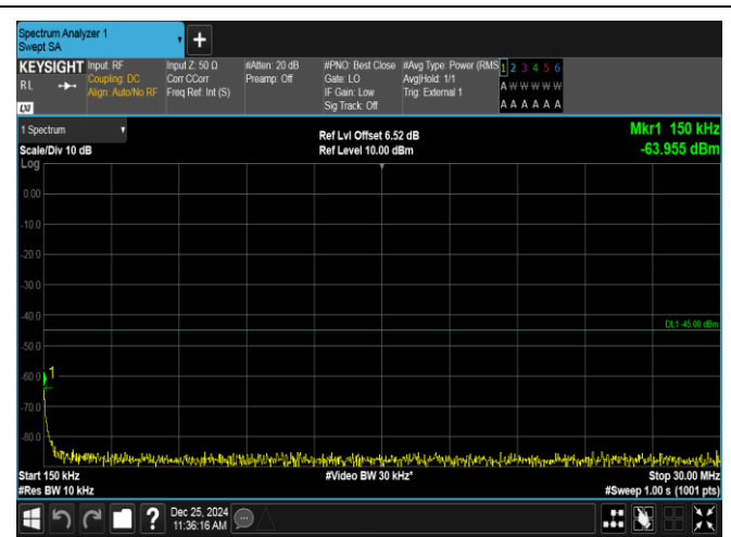
Band38-5MHz-16QAM-38225-1RB#24-0.15~30-PASS
