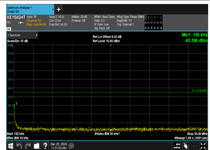
Band38-5MHz-QPSK-38225-1RB#0-0.15~30-PASS
