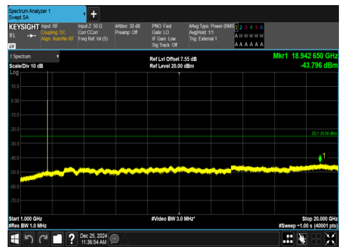
Band38-5MHz-16QAM-38225-1RB#24-1000~20000-PASS
