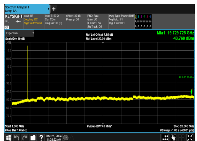
Band38-5MHz-QPSK-38225-25RB#0-1000~20000-PASS
