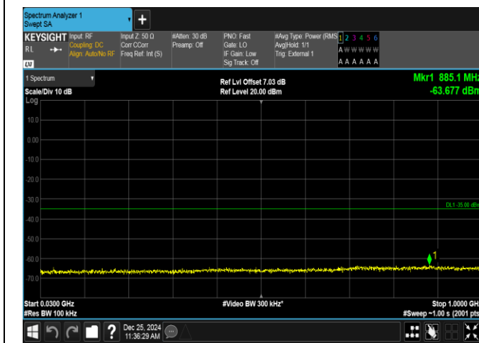
Band38-5MHz-16QAM-38225-1RB#24-30~1000-PASS
