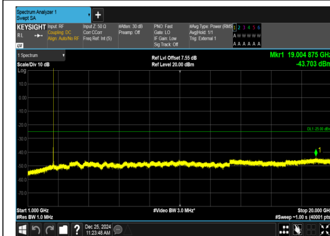
Band38-5MHz-QPSK-38000-1RB#0-1000~20000-PASS
