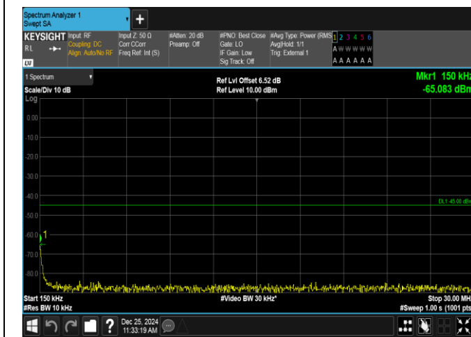
Band38-5MHz-16QAM-38225-1RB#0-0.15~30-PASS
