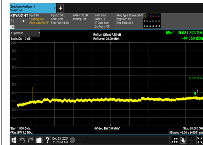
Band38-5MHz-QPSK-38000-25RB#0-1000~20000-PASS
