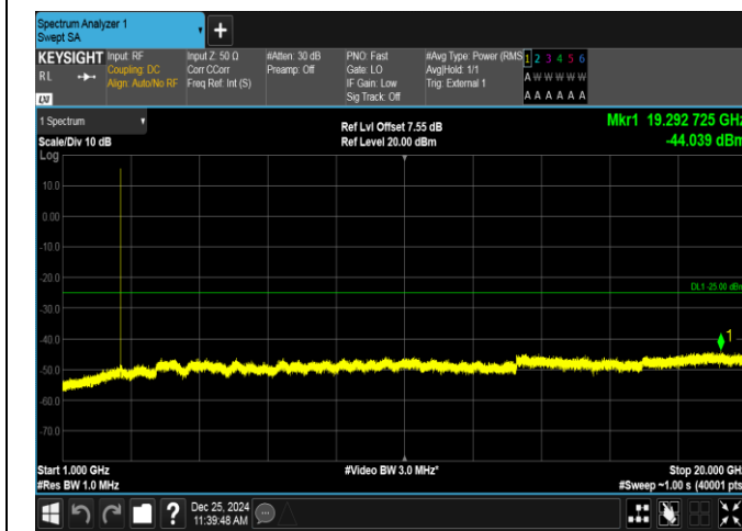
Band38-5MHz-16QAM-38225-25RB#0-1000~20000-PASS
