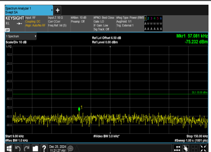
Band38-5MHz-16QAM-37775-25RB#0-0.009~0.15-PASS
