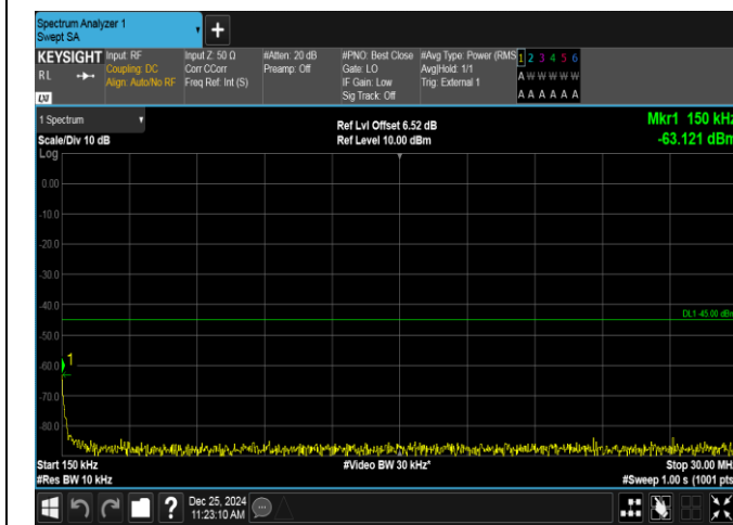
Band38-5MHz-QPSK-38000-1RB#0-0.15~30-PASS
