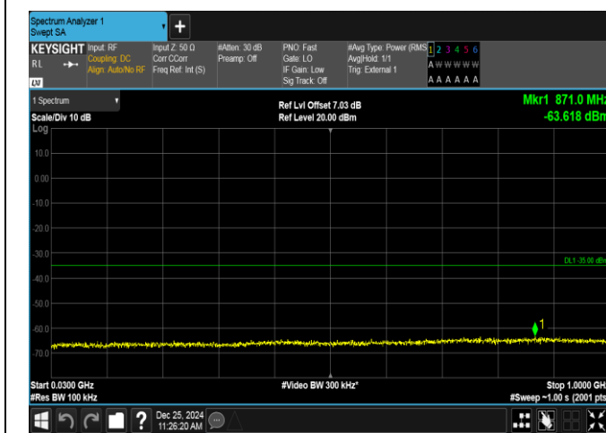
Band38-5MHz-QPSK-38000-1RB#24-30~1000-PASS
