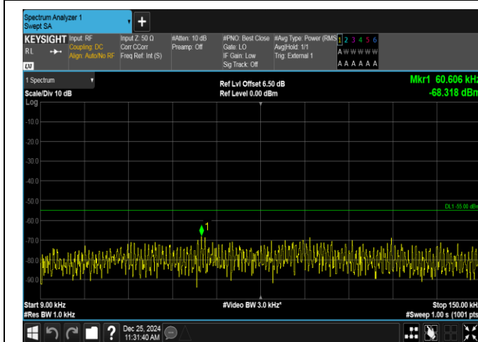
Band38-5MHz-QPSK-38225-1RB#0-0.009~0.15-PASS
