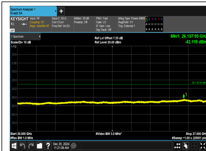
Band38-5MHz-QPSK-37775-25RB#0-20000~27000-PASS
