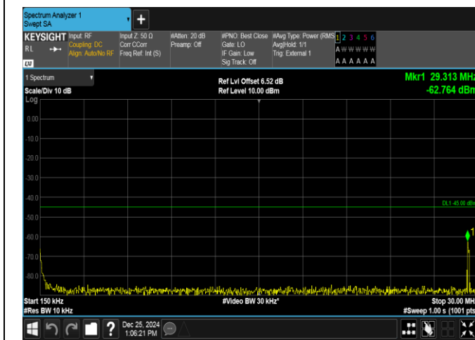
Band38-10MHz-QPSK-38000-1RB#0-0.15~30-PASS
