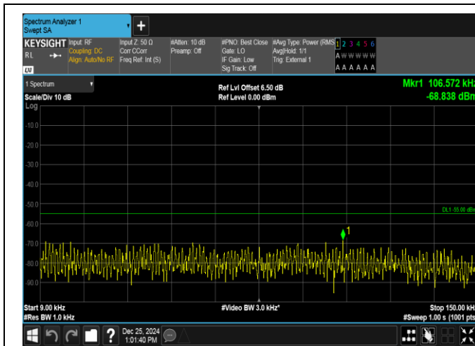
Band38-10MHz-16QAM-37800-1RB#49-0.009~0.15-PASS
