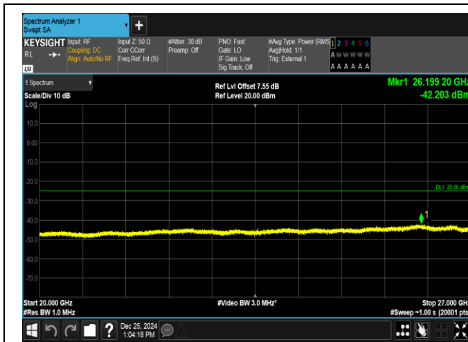
Band38-10MHz-QPSK-37800-50RB#0-20000~27000-PASS
