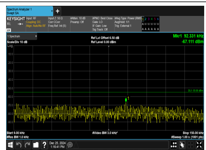
Band38-10MHz-16QAM-38200-1RB#0-0.009~0.15-PASS
