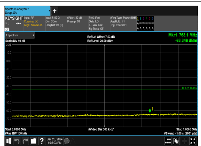
Band38-10MHz-16QAM-37800-50RB#0-30~1000-PASS
