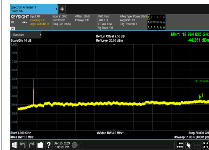
Band38-10MHz-16QAM-37800-50RB#0-1000~20000-PASS
