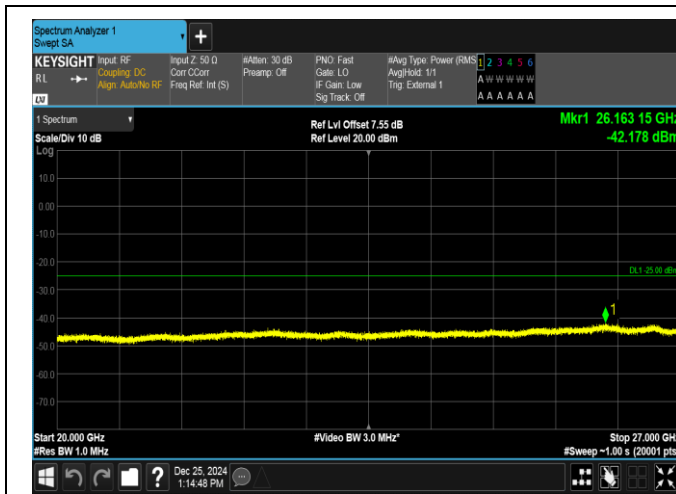
Band38-10MHz-16QAM-38000-50RB#0-20000~27000-PASS
