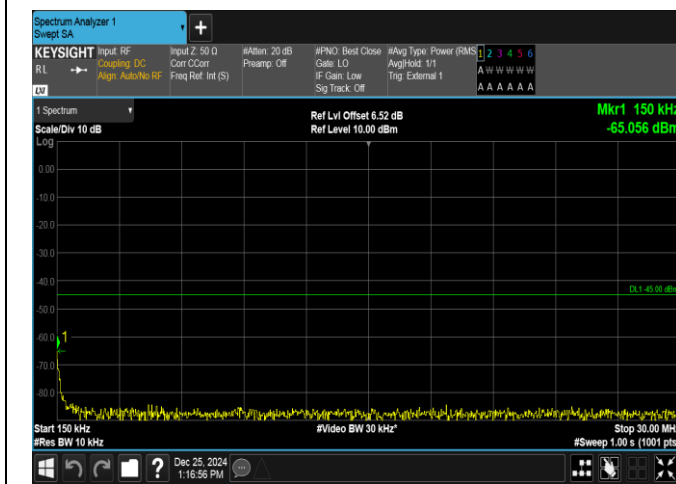
Band38-10MHz-16QAM-38200-1RB#0-0.15~30-PASS
