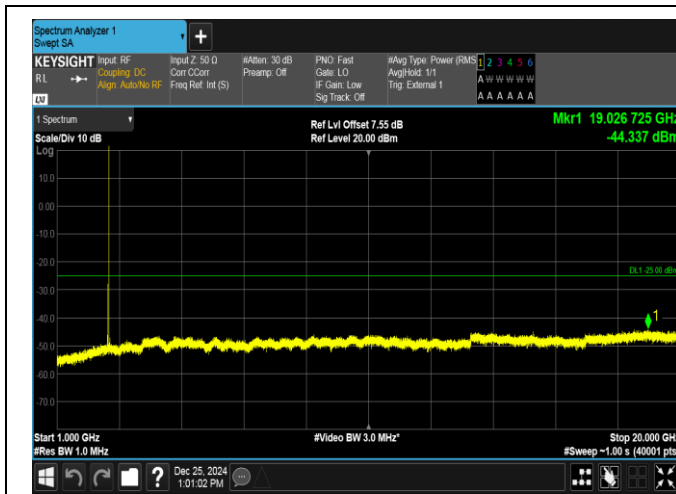
Band38-10MHz-QPSK-37800-1RB#49-1000~20000-PASS
