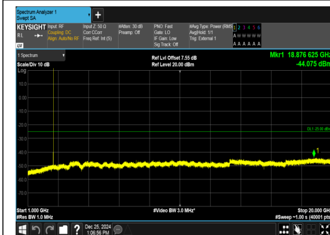
Band38-10MHz-QPSK-38000-1RB#0-1000~20000-PASS
