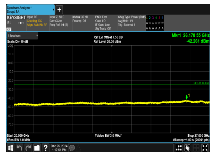
Band38-10MHz-16QAM-38200-1RB#0-20000~27000-PASS
