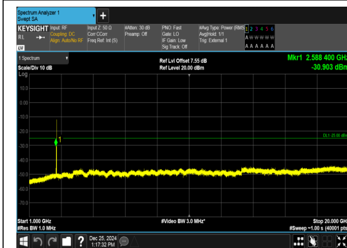
Band38-10MHz-16QAM-38200-1RB#0-1000~20000-PASS
