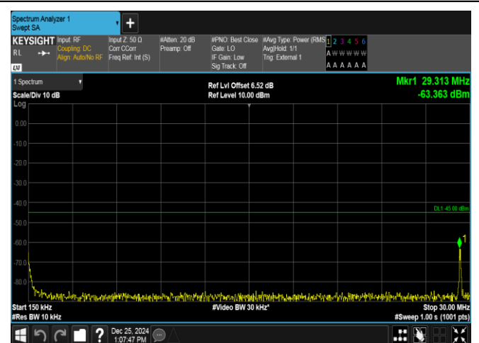
Band38-10MHz-16QAM-38000-1RB#0-0.15~30-PASS
