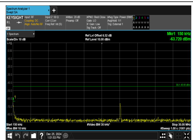
Band38-10MHz-16QAM-37800-1RB#49-0.15~30-PASS
