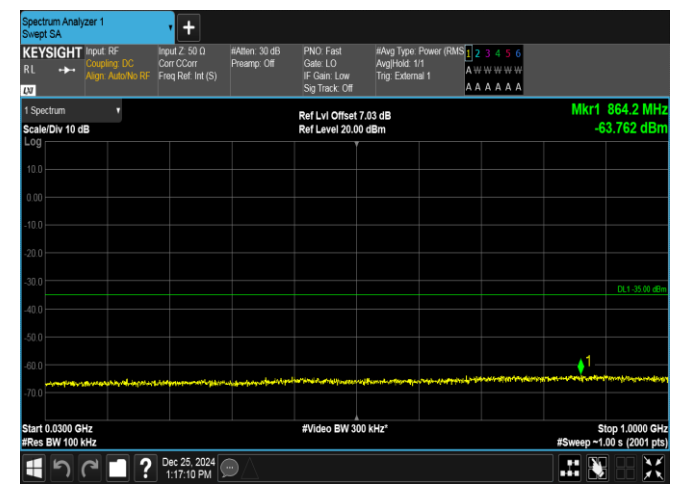
Band38-10MHz-16QAM-38200-1RB#0-30~1000-PASS
