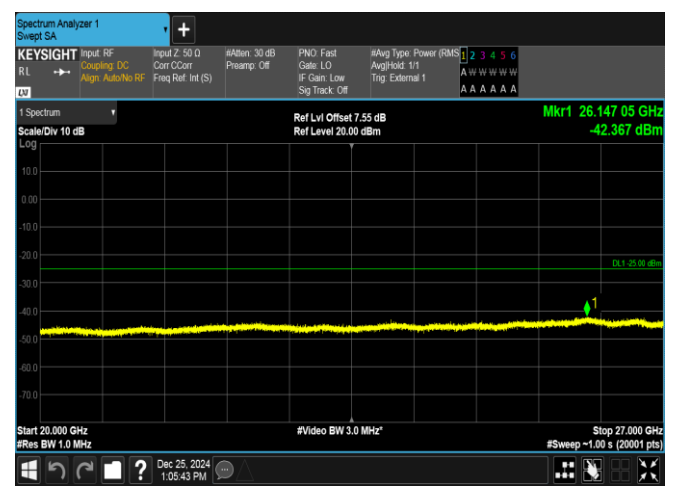
Band38-10MHz-16QAM-37800-50RB#0-20000~27000-PASS
