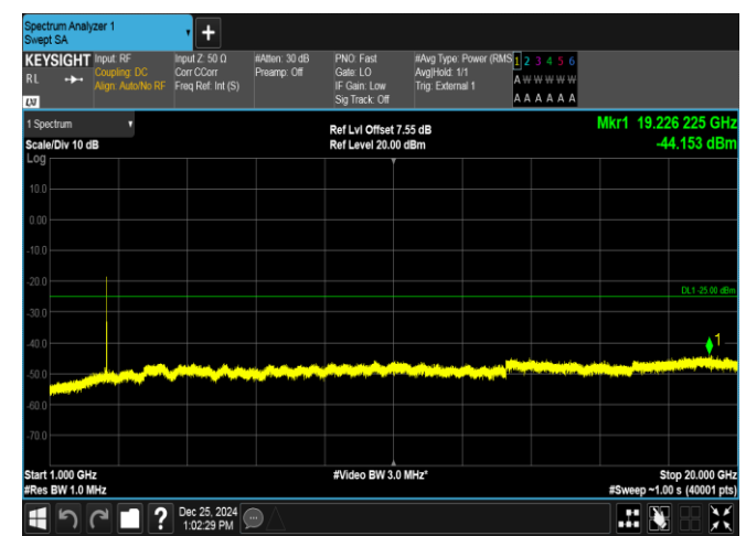
Band38-10MHz-16QAM-37800-1RB#49-1000~20000-PASS
