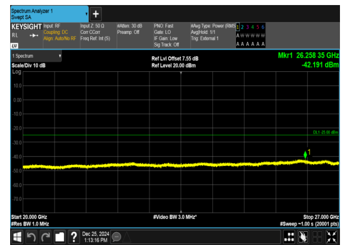
Band38-10MHz-QPSK-38000-50RB#0-20000~27000-PASS
