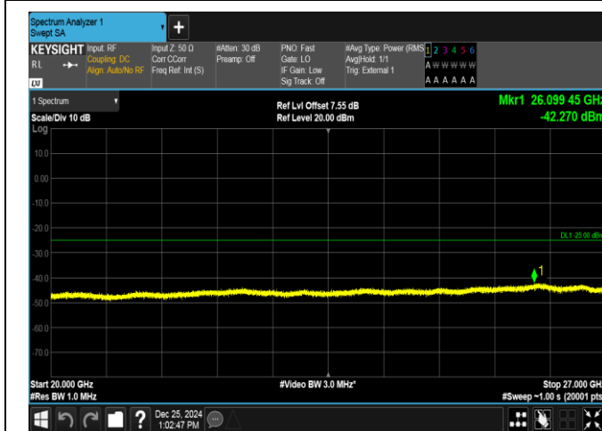
Band38-10MHz-16QAM-37800-1RB#49-20000~27000-PASS
