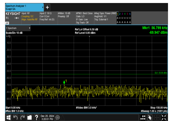
Band38-15MHz-QPSK-37825-1RB#74-0.009~0.15-PASS
