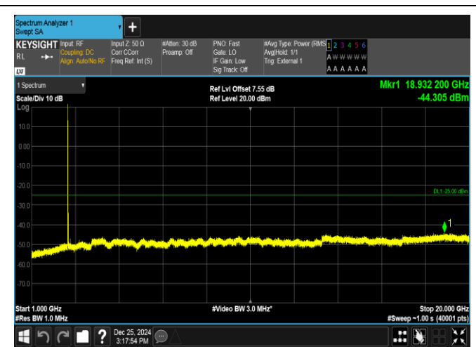
Band38-15MHz-QPSK-37825-1RB#0-1000~20000-PASS
