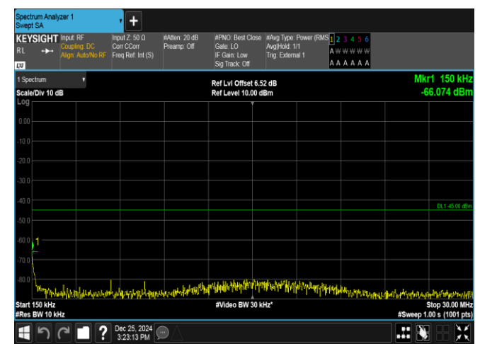
Band38-15MHz-QPSK-37825-75RB#0-0.15~30-PASS
