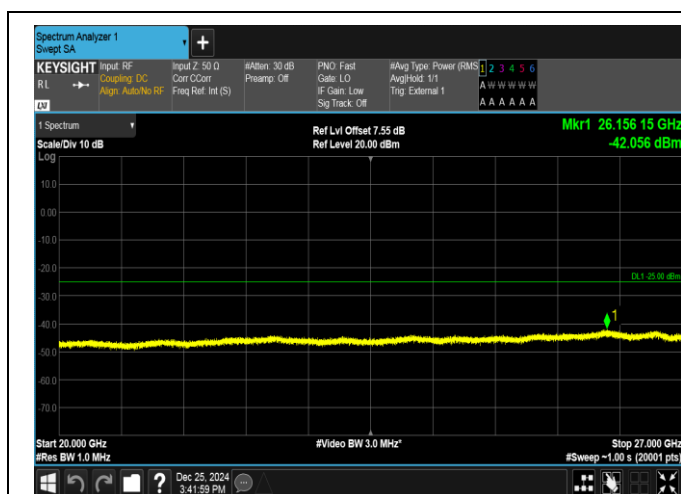
Band38-15MHz-OPSK-38175-75RB#0-20000~27000-PASS
