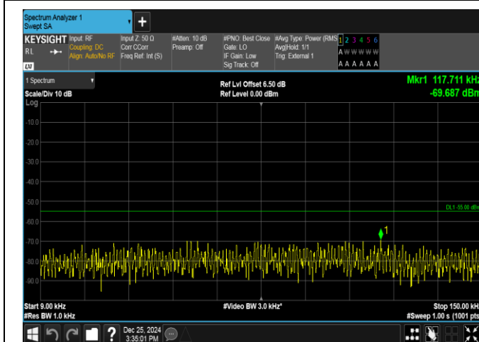
Band38-15MHz-QPSK-38175-1RB#0-0.009~0.15-PASS
