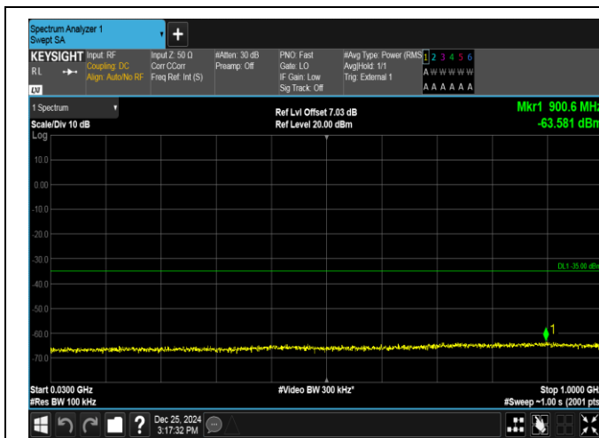
Band38-15MHz-QPSK-37825-1RB#0-30~1000-PASS
