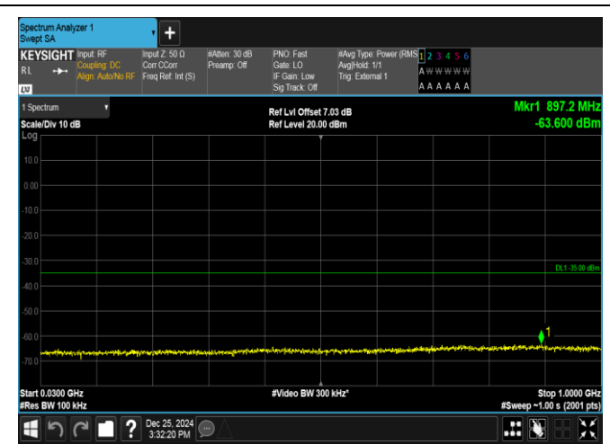
Band38-15MHz-QPSK-38000-75RB#0-30~1000-PASS
