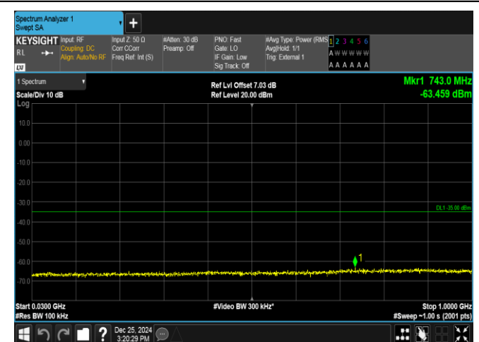
Band38-15MHz-QPSK-37825-1RB#74-30~1000-PASS
