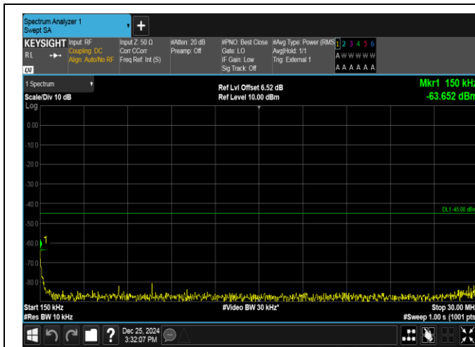
Band38-15MHz-QPSK-38000-75RB#0-0.15~30-PASS
