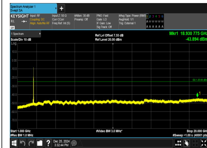
Band38-15MHz-QPSK-38000-75RB#0-1000~20000-PASS
