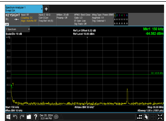
Band38-15MHz-16QAM-37825-1RB#74-0.15~30-PASS
