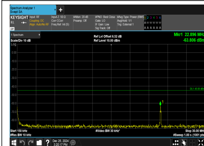
Band38-15MHz-QPSK-37825-1RB#74-0.15~30-PASS
