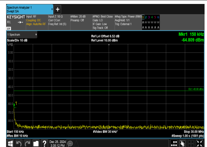
Band38-15MHz-QPSK-38175-1RB#0-0.15~30-PASS
