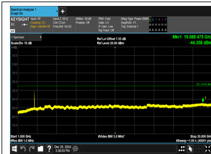
Band38-15MHz-QPSK-38175-1RB#74-1000~20000-PASS
