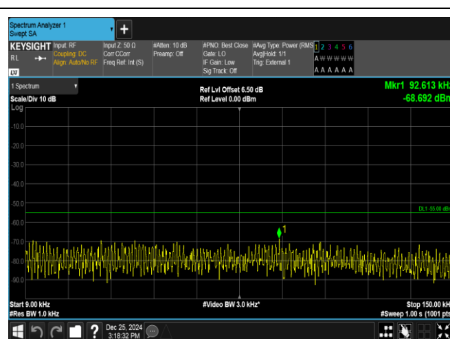
Band38-15MHz-16OAM-37825-1RB#0-0.009~0.15-PASS
