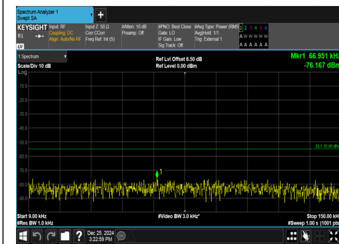
Band38-15MHz-QPSK-37825-75RB#0-0.009~0.15-PASS
