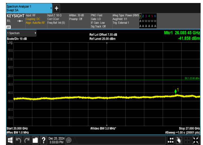
Band38-15MHz-QPSK-38000-75RB#0-20000~27000-PASS
