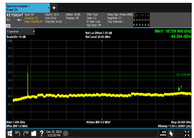
Band38-15MHz-16QAM-37825-1RB#74-1000~20000-PASS
