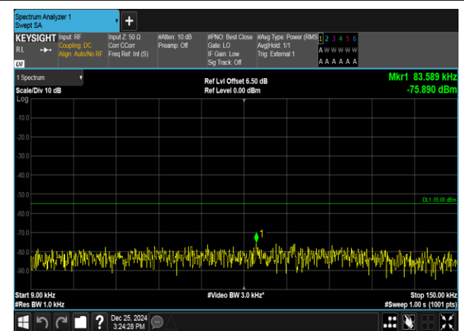
Band38-15MHz-16QAM-37825-75RB#0-0.009~0.15-PASS
