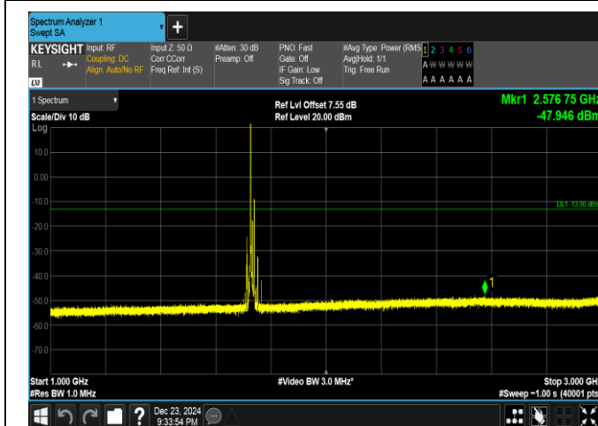
Band4-15MHz-QPSK-20175-1RB#0-1000~3000-PASS
