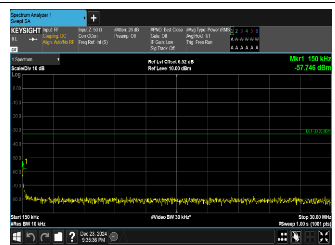
Band4-15MHz-QPSK-20175-1RB#74-0.15~30-PASS
