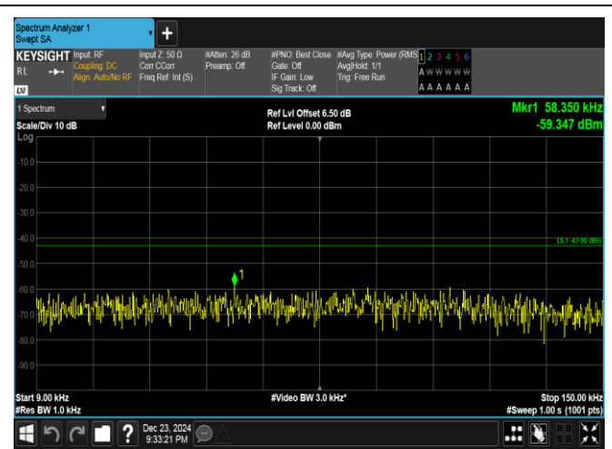
Band4-15MHz-QPSK-20175-1RB#0-0.009~0.15-PASS
