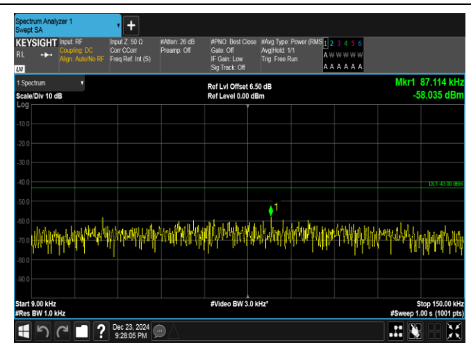
Band4-15MHz-16QAM-20025-1RB#0-0.009~0.15-PASS
