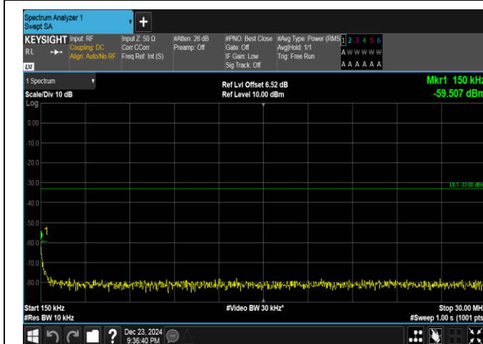
Band4-15MHz-16QAM-20175-1RB#74-0.15~30-PASS
