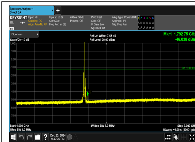
Band4-15MHz-QPSK-20325-1RB#74-1000~3000-PASS
