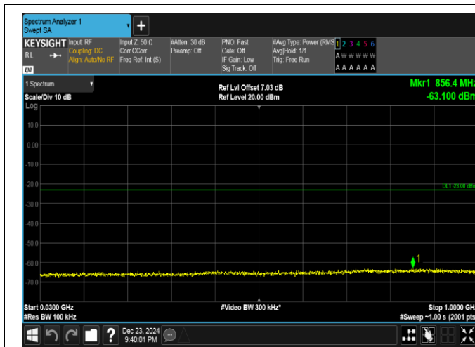
Band4-15MHz-QPSK-20325-1RB#0-30~1000-PASS
