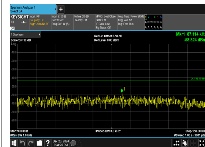
Band4-15MHz-16QAM-20175-1RB#0-0.009~0.15-PASS
