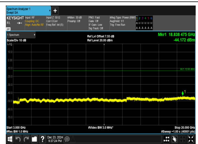
Band4-15MHz-16QAM-20175-1RB#74-3000~20000-PASS
