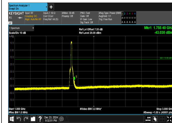
Band4-15MHz-16QAM-20025-75RB#0-1000~3000-PASS
