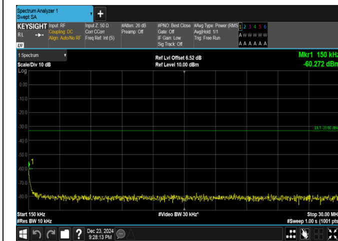
Band4-15MHz-16QAM-20025-1RB#0-0.15~30-PASS
