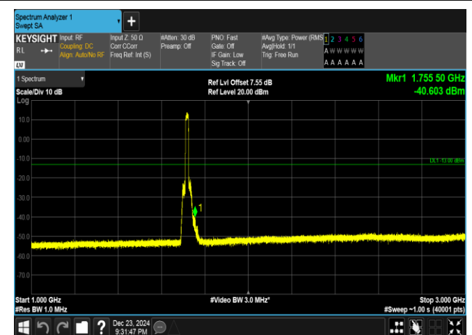
Band4-15MHz-QPSK-2025-75RB#0-1000~3000-PASS
