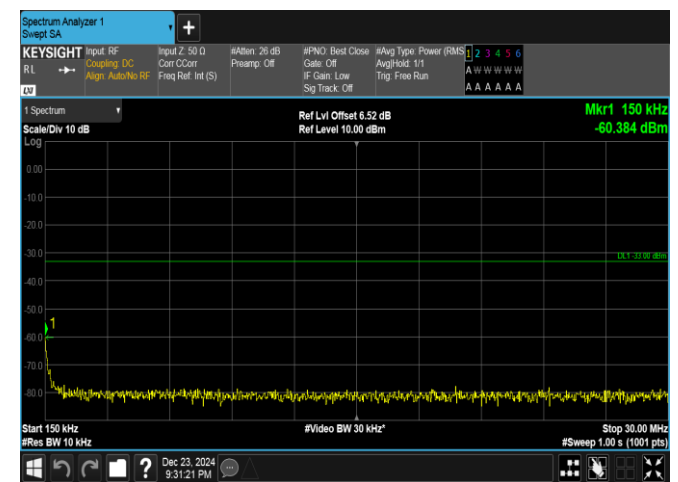
Band4-15MHz-QPSK-2025-75RB#0-0.15~30-PASS
