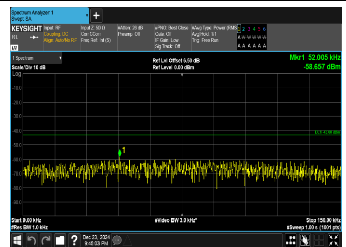
Band4-15MHz-16QAM-20325-75RB#0-0.009~0.15-PASS
