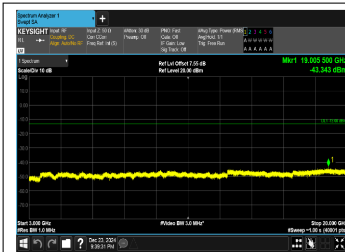
Band4-15MHz-16QAM-20175-75RB#0-3000~20000-PASS
