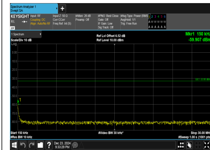
Band4-15MHz-QPSK-20175-1RB#0-0.15~30-PASS
