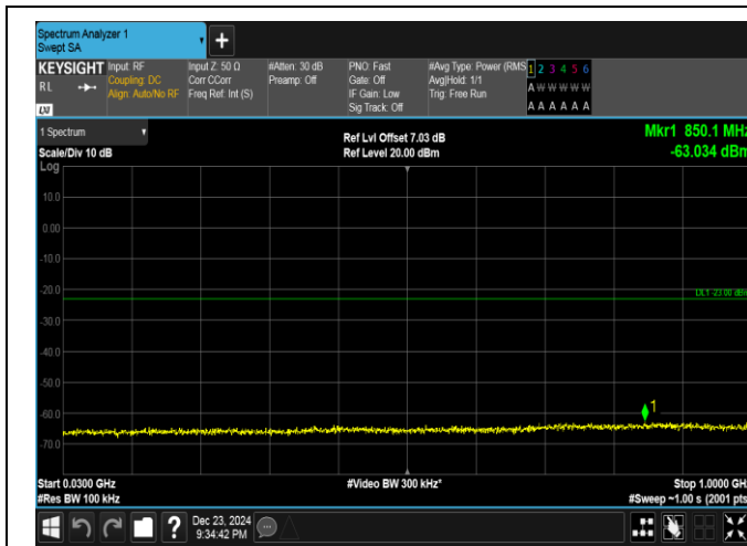
Band4-15MHz-16QAM-20175-1RB#0-30~1000-PASS
