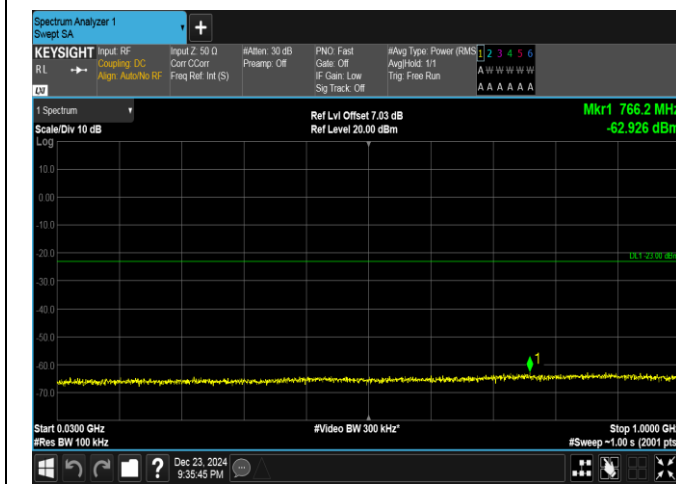
Band4-15MHz-QPSK-20175-1RB#74-30~1000-PASS
