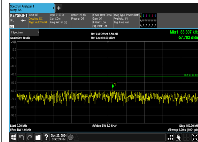
Band4-15MHz-16QAM-20175-75RB#0-0.009~0.15-PASS
