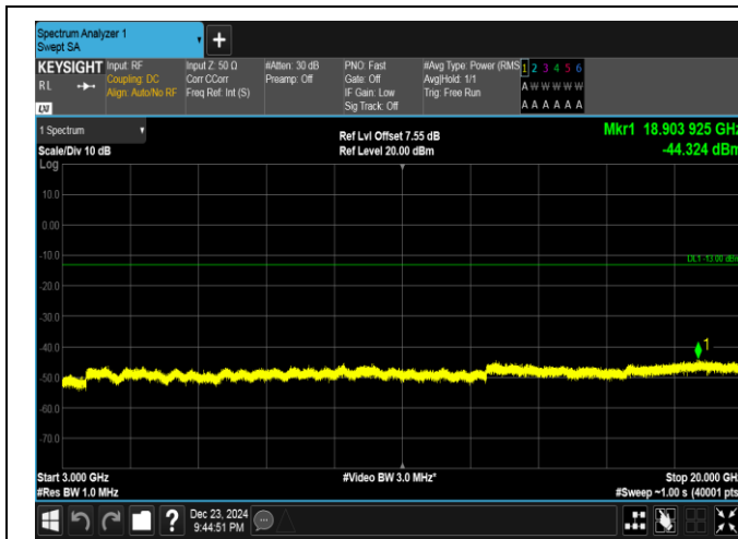
Band4-15MHz-QPSK-20325-75RB#0-3000~20000-PASS
