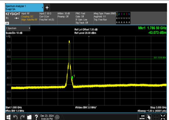
Band4-15MHz-QPSK-20325-75RB#0-1000~3000-PASS
