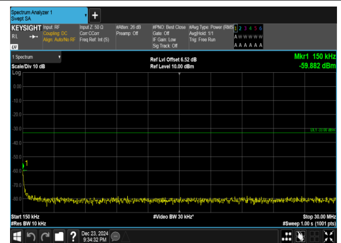
Band4-15MHz-16QAM-20175-1RB#0-0.15~30-PASS
