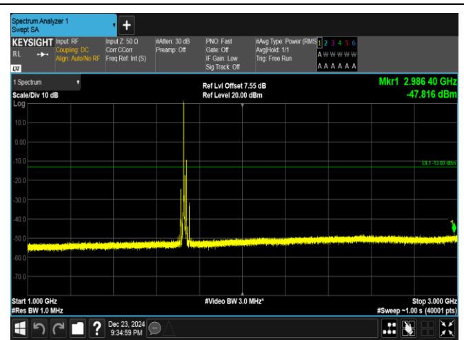
Band4-15MHz-16QAM-20175-1RB#0-1000~3000-PASS
