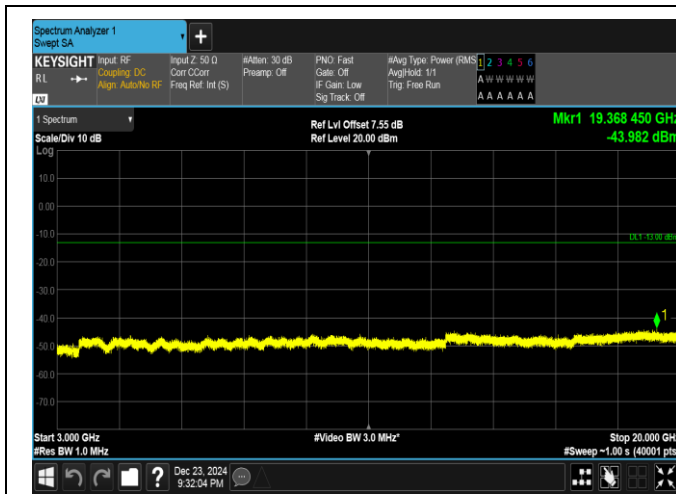
Band4-15MHz-QPSK-20025-75RB#0-3000~20000-PASS
