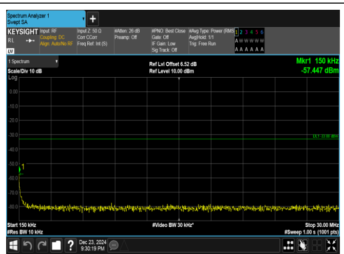
Band4-15MHz-16QAM-2025-1RB#74-0.15~30-PASS
