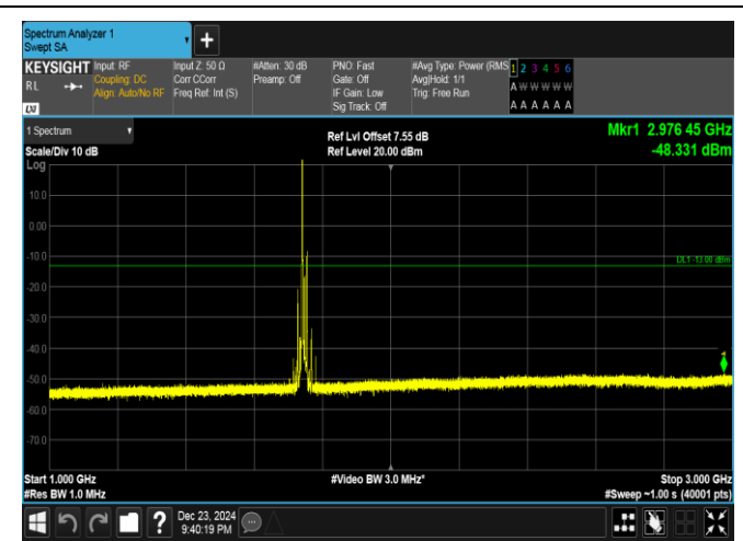
Band4-15MHz-QPSK-20325-1RB#0-1000~3000-PASS
