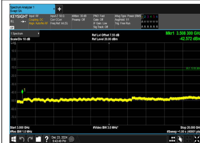
Band4-15MHz-16QAM-20325-1RB#74-3000~20000-PASS
