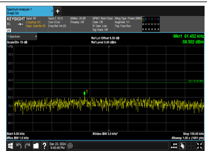
Band4-15MHz-16QAM-20325-1RB#0-0.009~0.15-PASS
