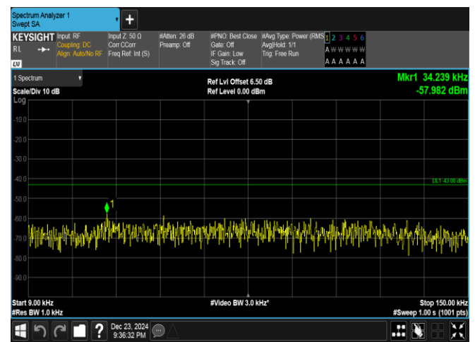
Band4-15MHz-16QAM-20175-1RB#74-0.009~0.15-PASS
