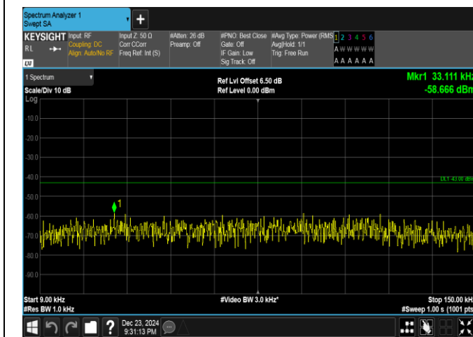
Band4-15MHz-QPSK-2025-75RB#0-0.009~0.15-PASS
