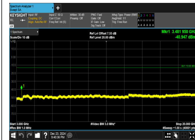
Band4-15MHz-QPSK-20325-1RB#0-3000~20000-PASS
