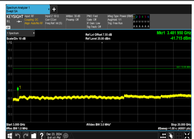
Band4-15MHz-16QAM-20325-1RB#0-3000~20000-PASS
