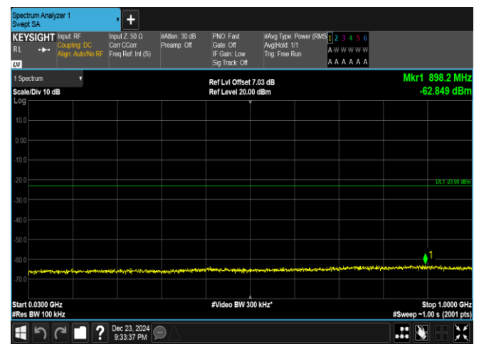
Band4-15MHz-QPSK-20175-1RB#0-30~1000-PASS
