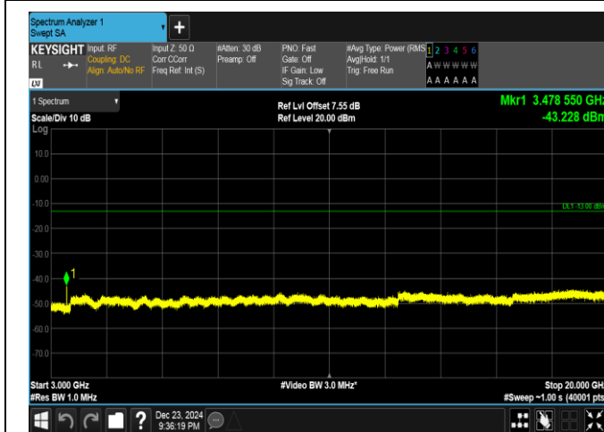
Band4-15MHz-QPSK-20175-1RB#74-3000~20000-PASS
