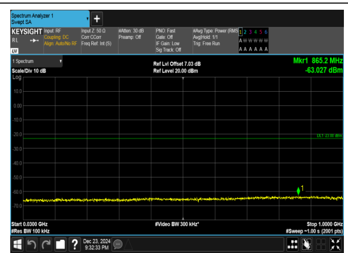
Band4-15MHz-16QAM-20025-75RB#0-30~1000-PASS
