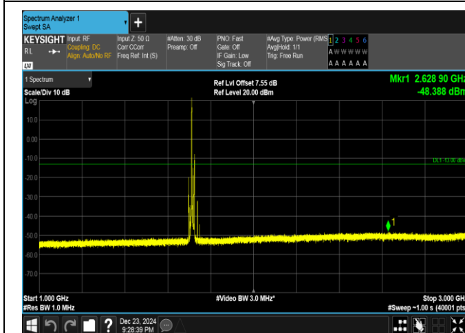
Band4-15MHz-16QAM-20025-1RB#0-1000~3000-PASS
