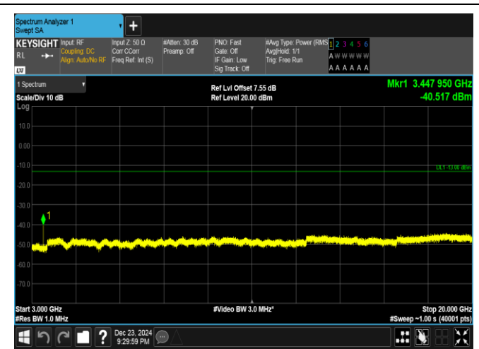
Band4-15MHz-QPSK-2025-1RB#74-3000~20000-PASS
