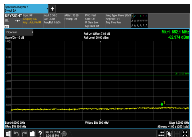
Band4-15MHz-16QAM-20175-1RB#74-30~1000-PASS
