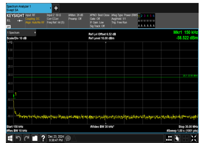
Band4-15MHz-16QAM-20175-75RB#0-0.15~30-PASS
