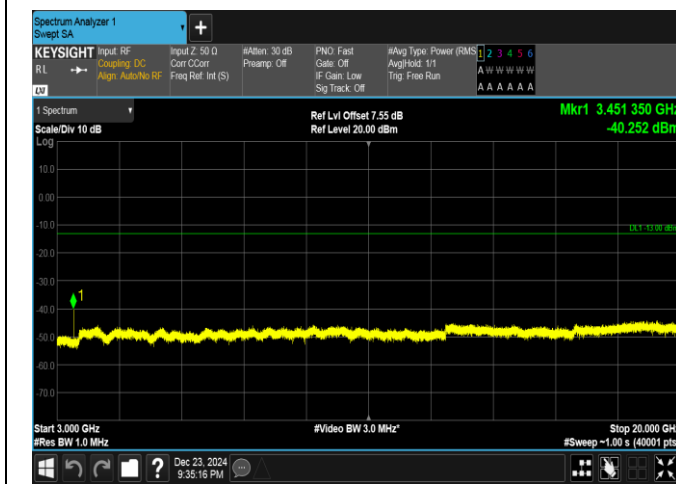
Band4-15MHz-16QAM-20175-1RB#0-3000~20000-PASS
