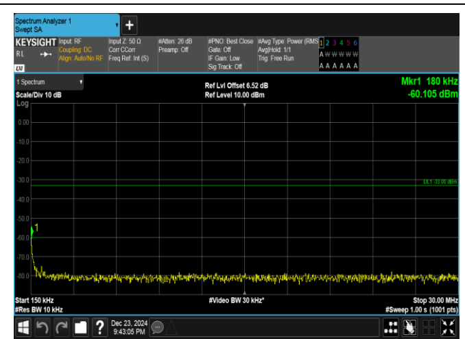
Band4-15MHz-16QAM-20325-1RB#74-0.15~30-PASS
