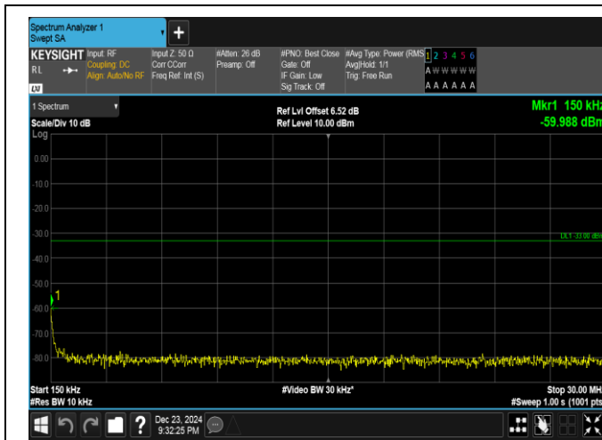
Band4-15MHz-16QAM-20025-75RB#0-0.15~30-PASS
