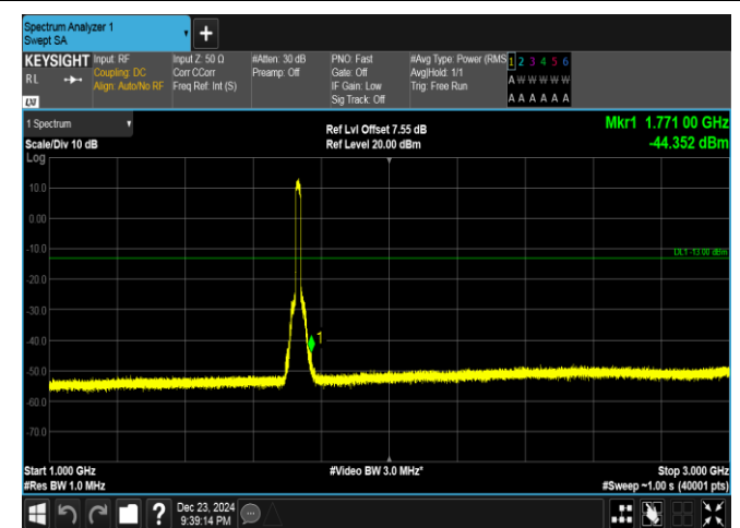
Band4-15MHz-16QAM-20175-75RB#0-1000~3000-PASS
