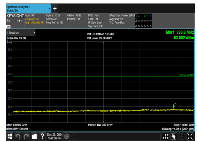
Band4-15MHz-16QAM-20325-1RB#0-30~1000-PASS
