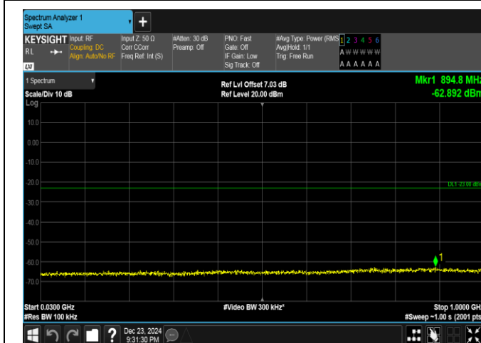
Band4-15MHz-QPSK-2025-75RB#0-30~1000-PASS
