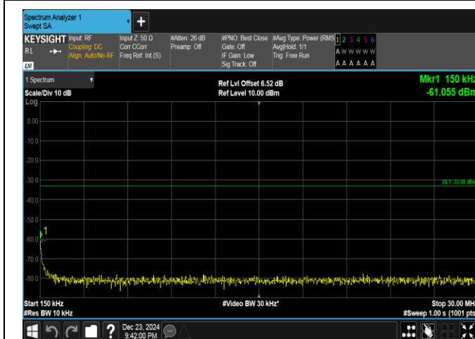
Band4-15MHz-QPSK-20325-1RB#74-0.15~30-PASS
