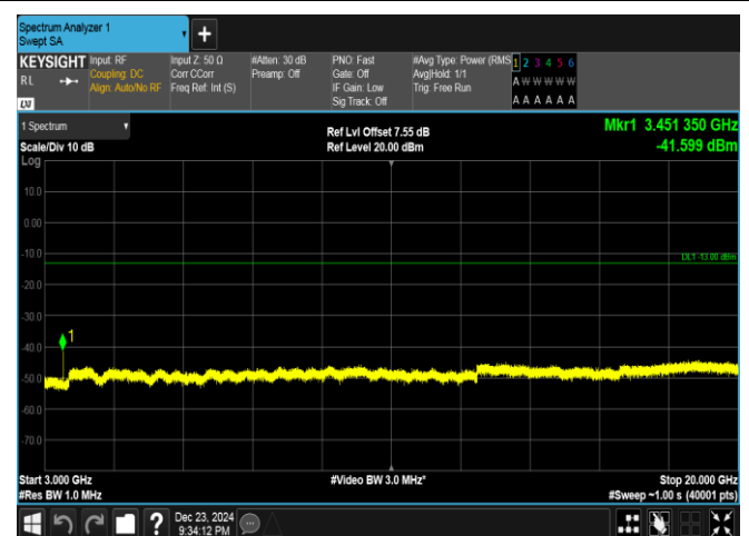
Band4-15MHz-QPSK-20175-1RB#0-3000~20000-PASS
