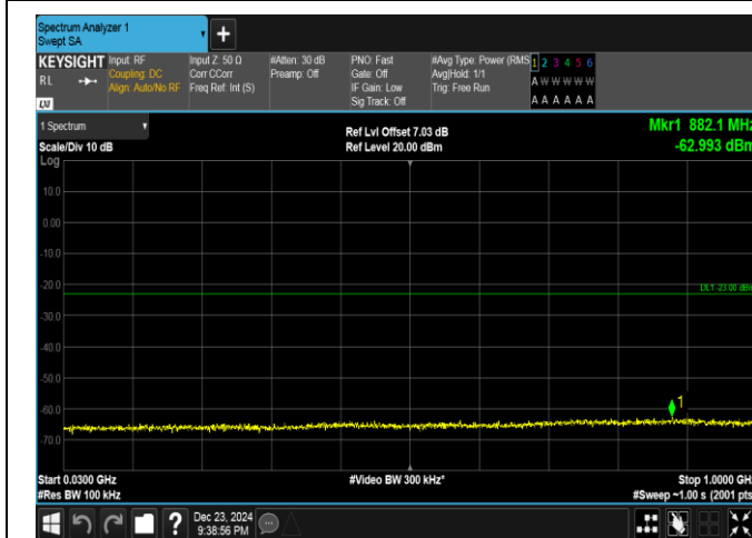
Band4-15MHz-16QAM-20175-75RB#0-30~1000-PASS
