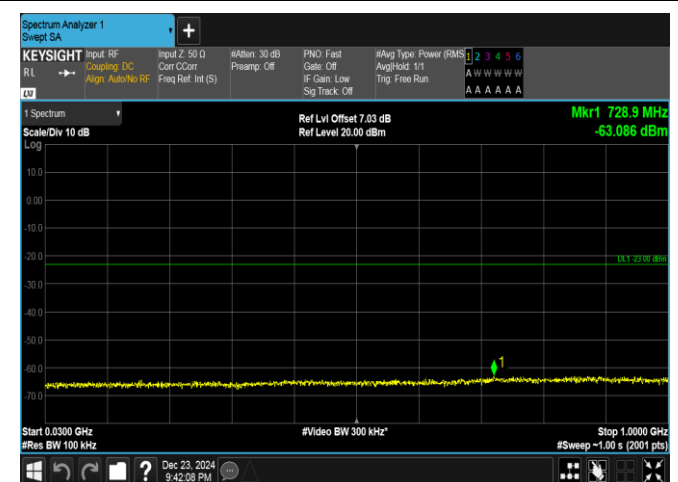
Band4-15MHz-QPSK-20325-1RB#74-30~1000-PASS
