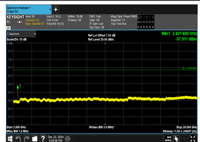
Band4-15MHz-16QAM-20025-1RB#0-3000~20000-PASS
