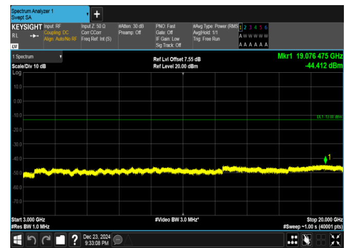
Band4-15MHz-16QAM-20025-75RB#0-3000~20000-PASS
