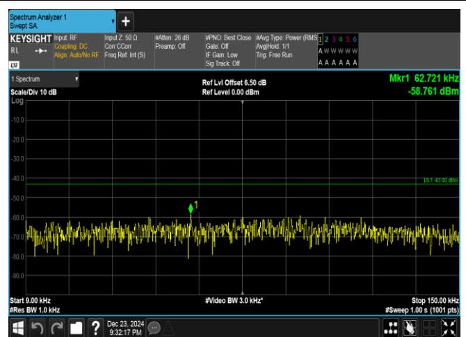
Band4-15MHz-16QAM-2025-75RB#0-0.009~0.15-PASS
