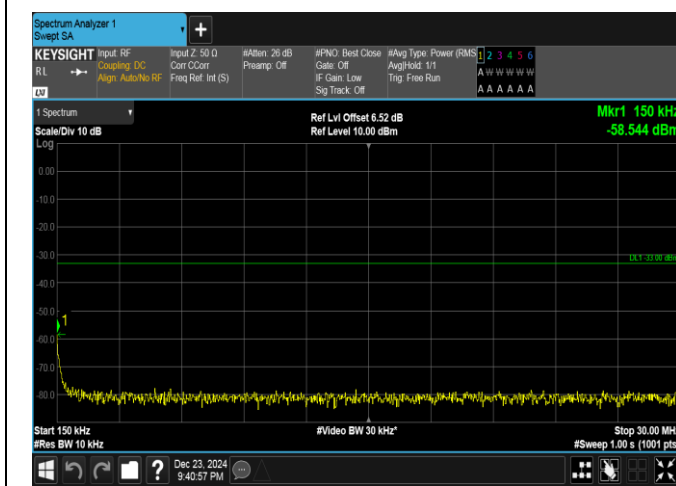
Band4-15MHz-16QAM-20325-1RB#0-0.15~30-PASS
