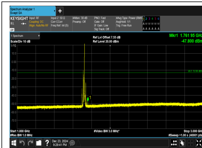
Band4-15MHz-QPSK-2025-1RB#74-1000~3000-PASS
