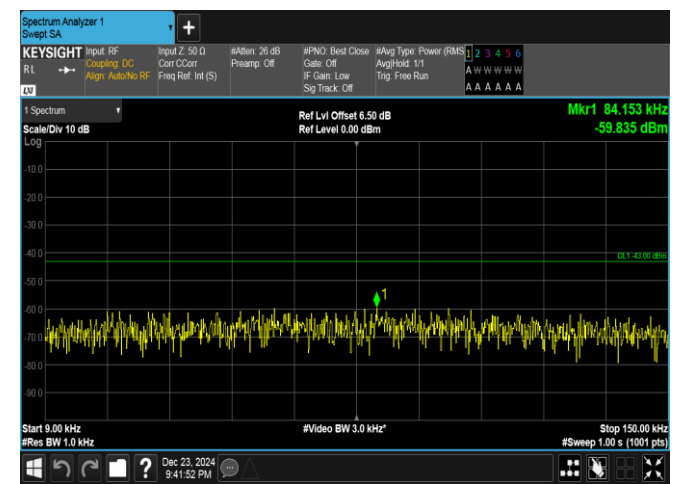
Band4-15MHz-QPSK-20325-1RB#74-0.009~0.15-PASS
