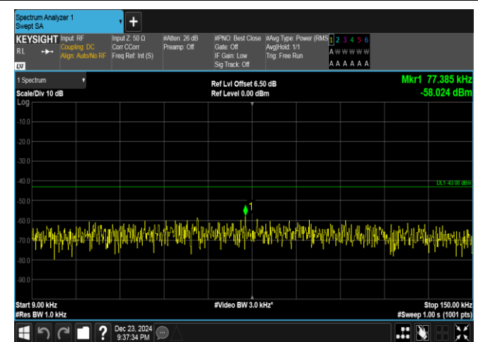
Band4-15MHz-QPSK-20175-75RB#0-0.009~0.15-PASS
