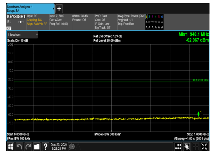
Band4-15MHz-16QAM-20025-1RB#0-30~1000-PASS
