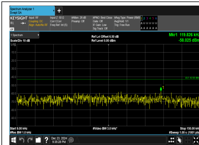
Band4-15MHz-QPSK-20175-1RB#74-0.009~0.15-PASS
