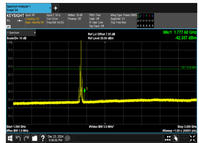
Band4-15MHz-QPSK-20175-1RB#74-1000~3000-PASS
