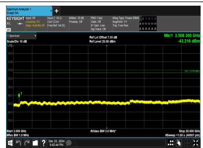
Band4-15MHz-QPSK-20325-1RB#74-3000~20000-PASS
