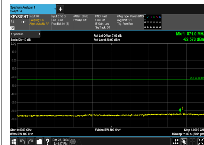
Band4-15MHz-QPSK-20325-75RB#0-30~1000-PASS
