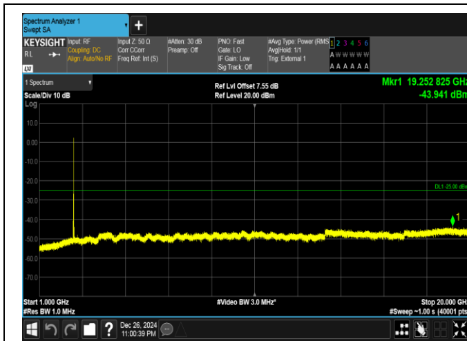
Band41-15MHz-QPSK-39725-1RB#74-1000~20000-PASS
