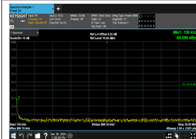
Band41-15MHz-QPSK-39725-1RB#74-0.15~30-PASS
