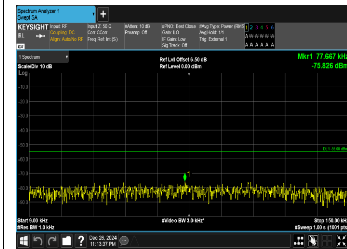
Band41-15MHz-16QAM-40620-75RB#0-0.009~0.15-PASS
