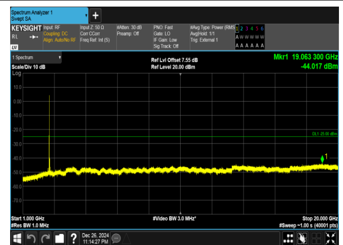
Band41-15MHz-16QAM-40620-75RB#0-1000~20000-PASS
