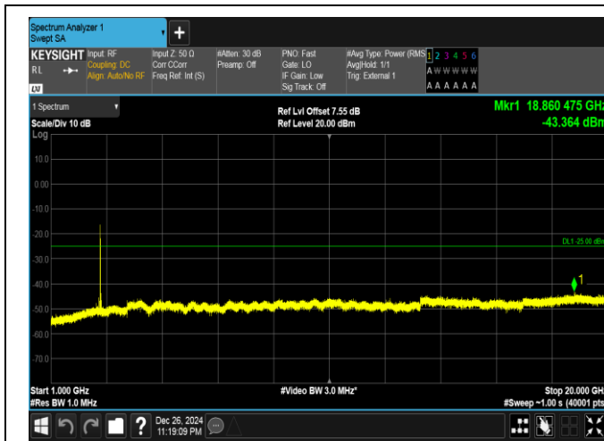
Band41-15MHz-QPSK-41515-1RB#74-1000~20000-PASS
