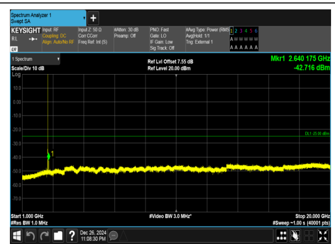
Band41-15MHz-16QAM-40620-1RB#0-1000~20000-PASS
