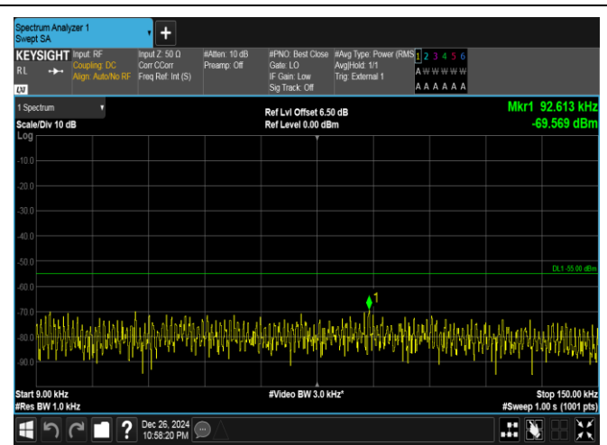
Band41-15MHz-16QAM-39725-1RB#0-0.009~0.15-PASS
