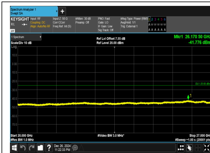
Band41-15MHz-QPSK-41515-75RB#0-20000~27000-PASS
