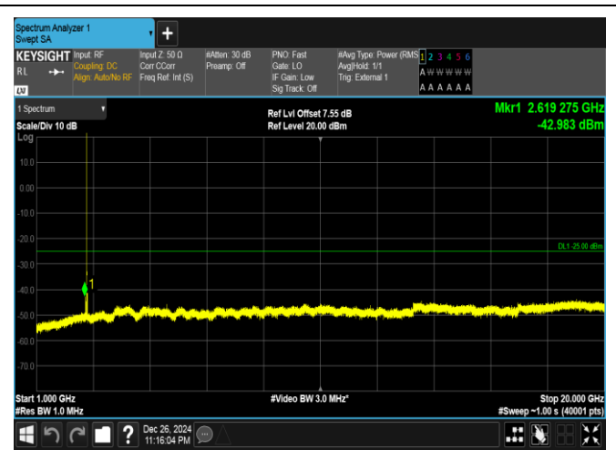
Band41-15MHz-QPSK-41515-1RB#0-1000~20000-PASS
