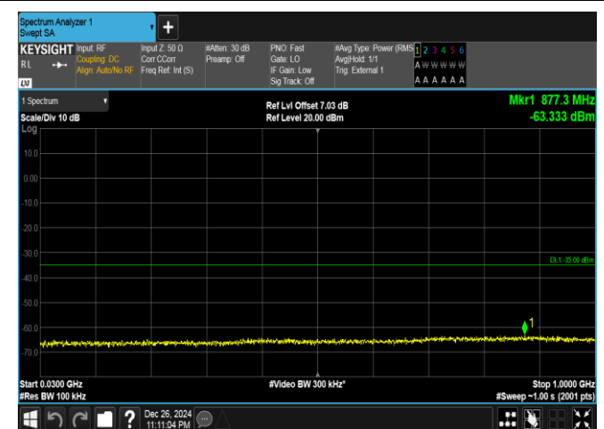
Band41-15MHz-16QAM-40620-1RB#74-30~1000-PASS
