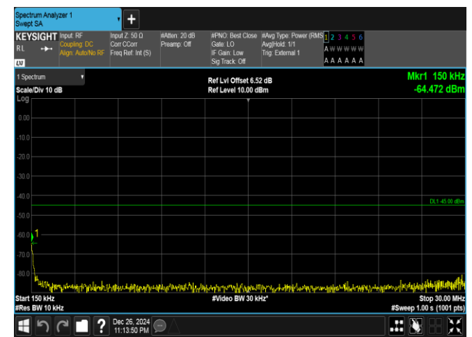
Band41-15MHz-16QAM-40620-75RB#0-0.15~30-PASS
