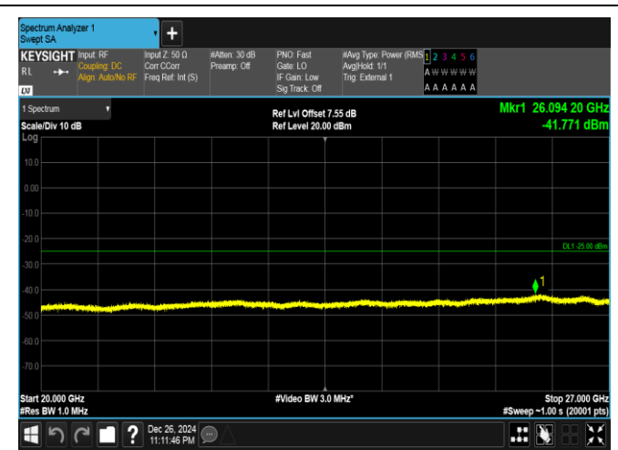
Band41-15MHz-16QAM-40620-1RB#74-20000~27000-PASS
