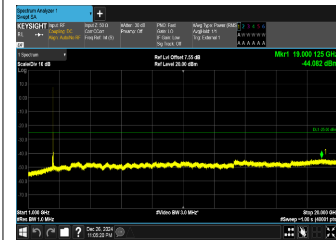
Band41-15MHz-16QAM-39725-75RB#0-1000~20000-PASS
