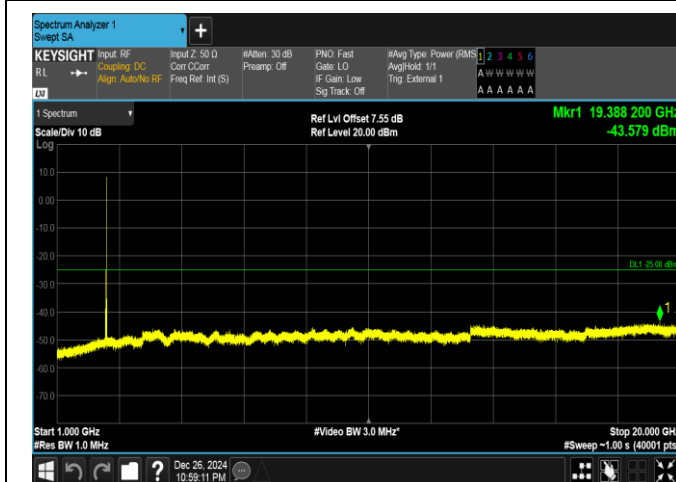
Band41-15MHz-16QAM-39725-1RB#0-1000~20000-PASS
