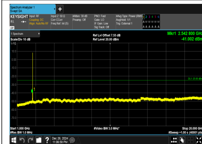
Band41-15MHz-QPSK-40620-1RB#0-1000~20000-PASS
