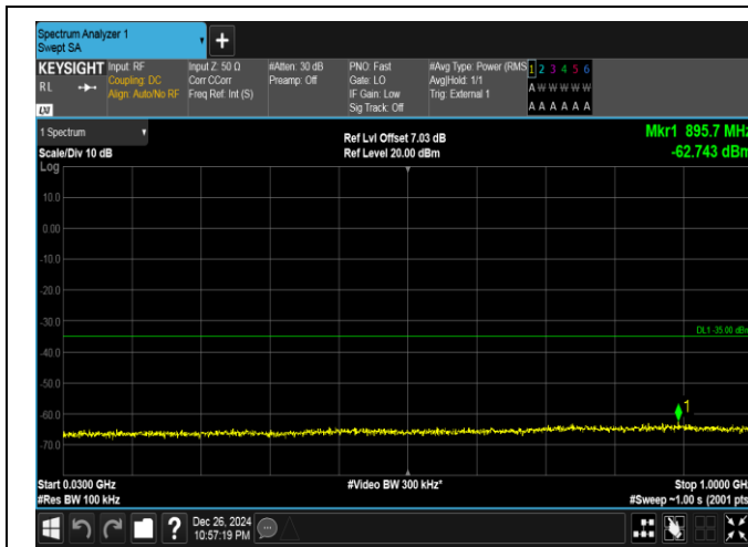
Band41-15MHz-QPSK-39725-1RB#0-30~1000-PASS
