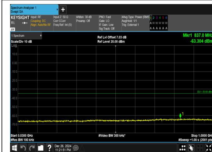
Band41-15MHz-QPSK-41515-75RB#0-30~1000-PASS
