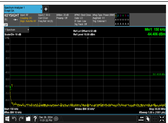
Band41-15MHz-16QAM-39725-1RB#74-0.15~30-PASS
