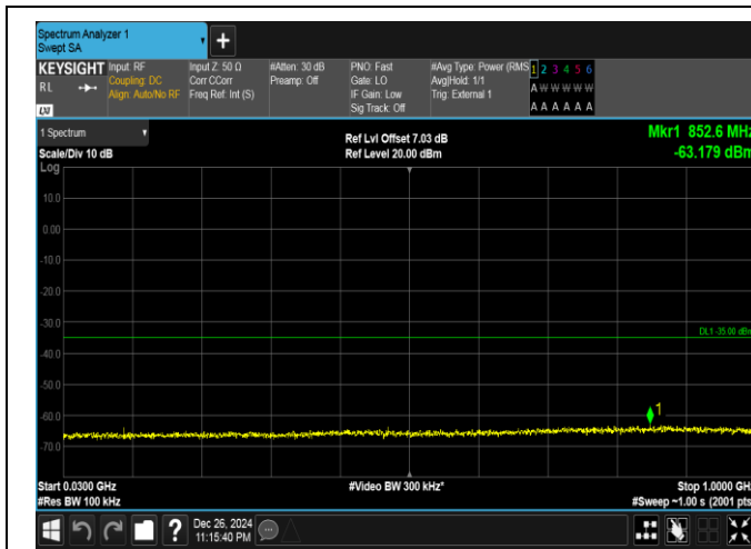
Band41-15MHz-QPSK-41515-1RB#0-30~1000-PASS
