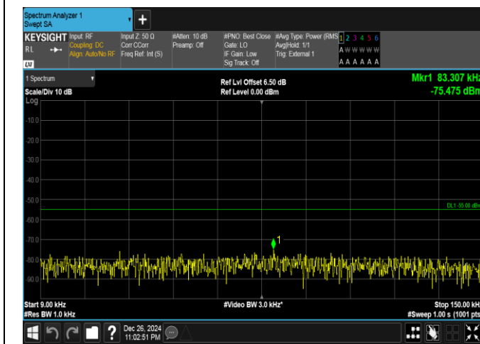
Band41-15MHz-QPSK-39725-75RB#0-0.009~0.15-PASS
