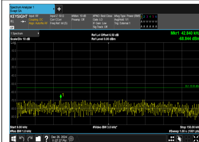
Band41-15MHz-16QAM-40620-1RB#0-0.009~0.15-PASS
