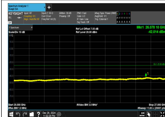
Band41-15MHz-16QAM-39725-1RB#74-20000~27000-PASS
