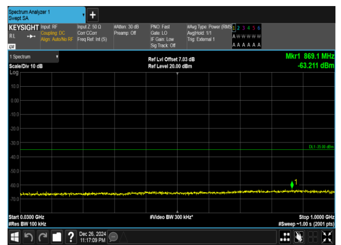
Band41-15MHz-16QAM-41515-1RB#0-30~1000-PASS
