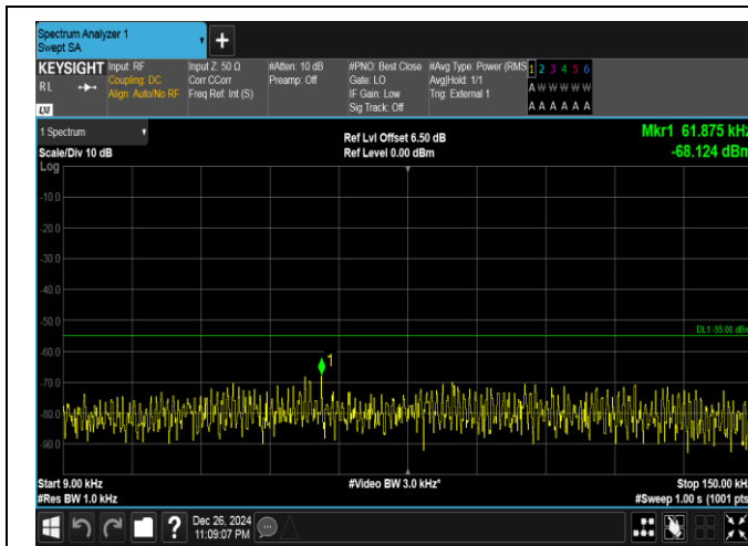
Band41-15MHz-QPSK-40620-1RB#74-0.009~0.15-PASS
