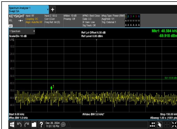
Band41-15MHz-16QAM-39725-1RB#74-0.009~0.15-PASS
