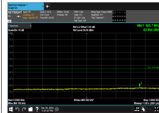
Band41-15MHz-16QAM-39725-1RB#74-30~1000-PASS
