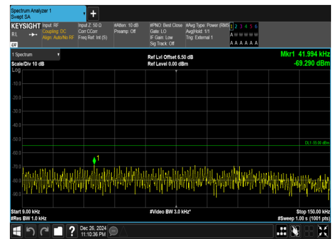
Band41-15MHz-16QAM-40620-1RB#74-0.009~0.15-PASS
