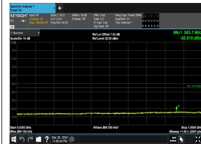
Band41-15MHz-QPSK-40620-1RB#74-30~1000-PASS
