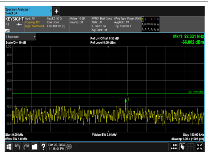
Band41-15MHz-16QAM-41515-1RB#0-0.009~0.15-PASS
