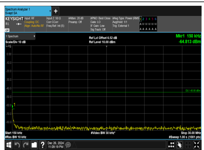
Band41-15MHz-QPSK-40620-1RB#74-0.15~30-PASS
