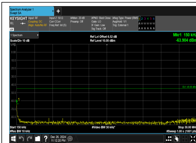
Band41-15MHz-QPSK-40620-75RB#0-0.15~30-PASS
