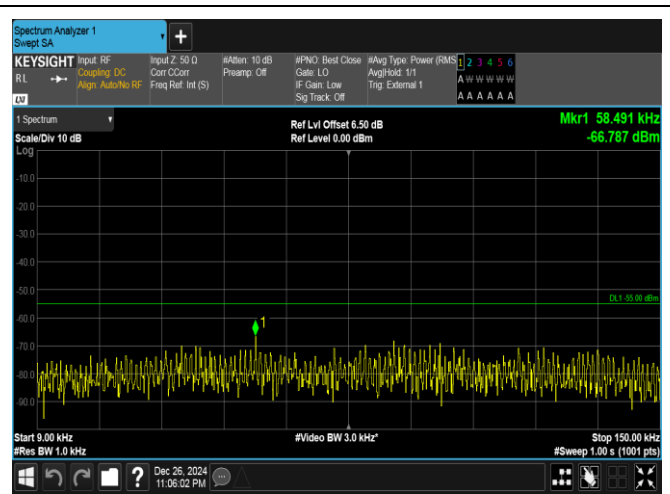
Band41-15MHz-QPSK-40620-1RB#0-0.009~0.15-PASS
