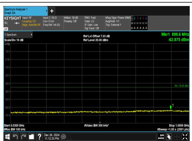
Band41-15MHz-QPSK-40620-75RB#0-30~1000-PASS
