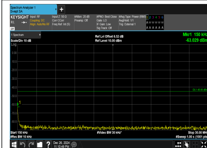
Band41-15MHz-16QAM-40620-1RB#74-0.15~30-PASS
