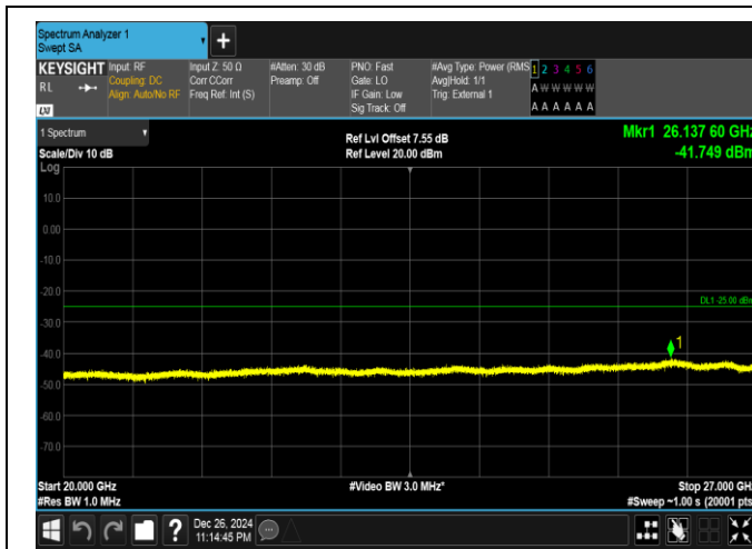
Band41-15MHz-16QAM-40620-75RB#0-20000~27000-PASS
