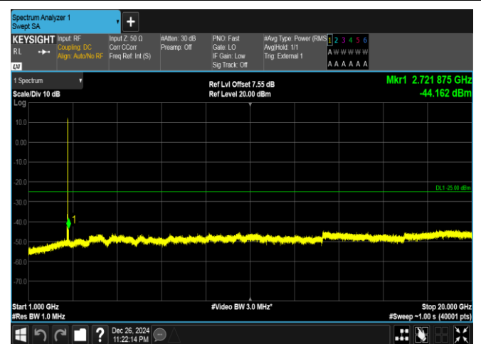
Band41-15MHz-QPSK-41515-75RB#0-1000~20000-PASS
