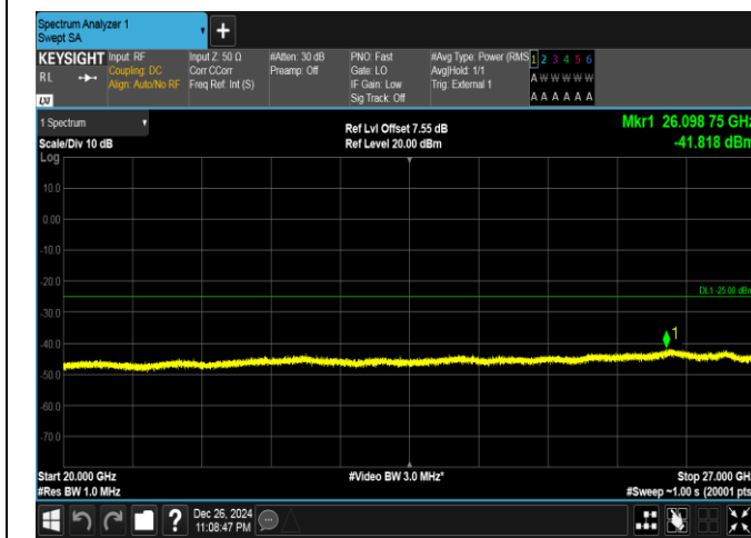
Band41-15MHz-16QAM-40620-1RB#0-20000~27000-PASS
