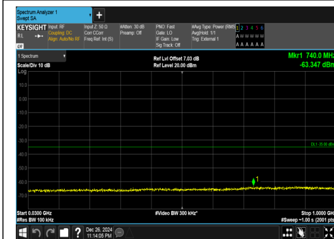
Band41-15MHz-16QAM-40620-75RB#0-30~1000-PASS
