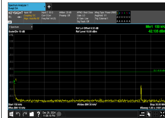
Band41-15MHz-QPSK-40620-1RB#0-0.15~30-PASS
