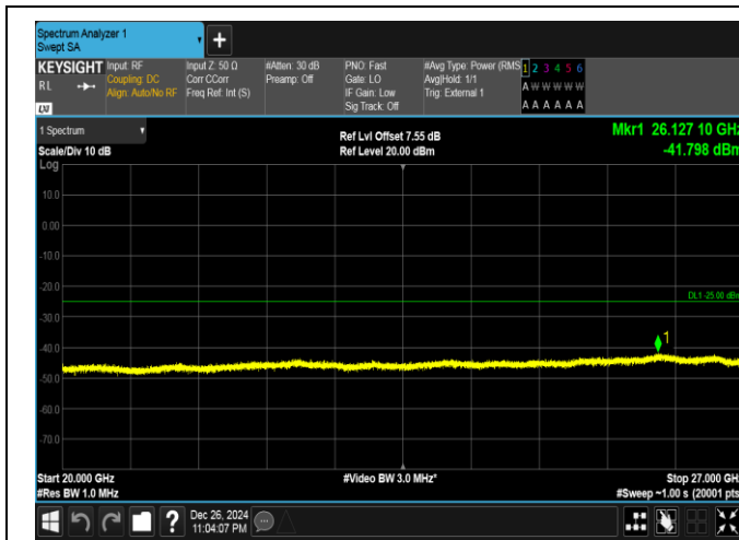
Band41-15MHz-QPSK-39725-75RB#0-20000~27000-PASS
