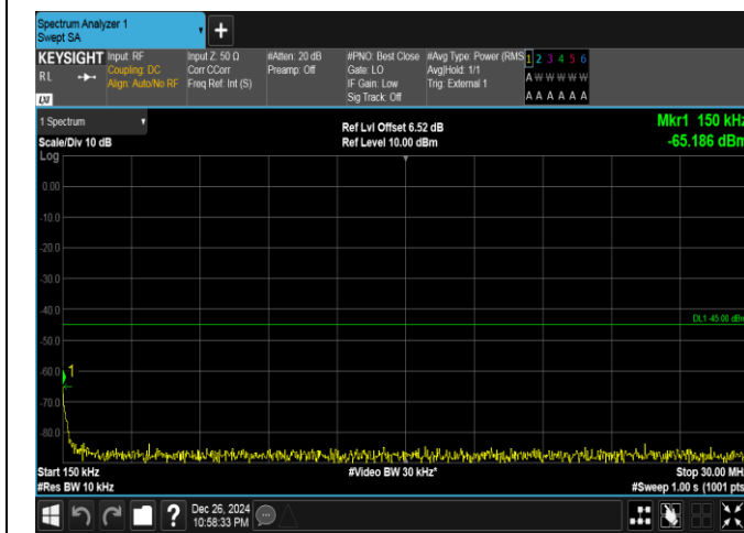
Band41-15MHz-16QAM-39725-1RB#0-0.15~30-PASS
