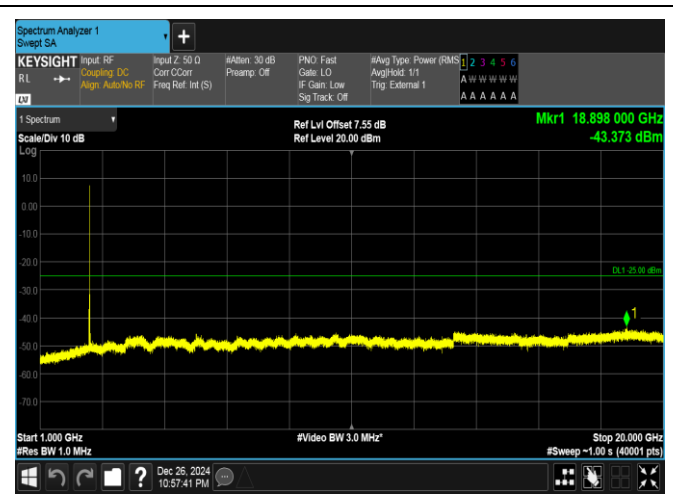
Band41-15MHz-QPSK-39725-1RB#0-1000~20000-PASS
