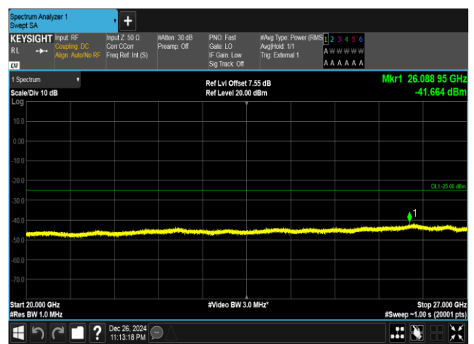
Band41-15MHz-QPSK-40620-75RB#0-20000~27000-PASS
