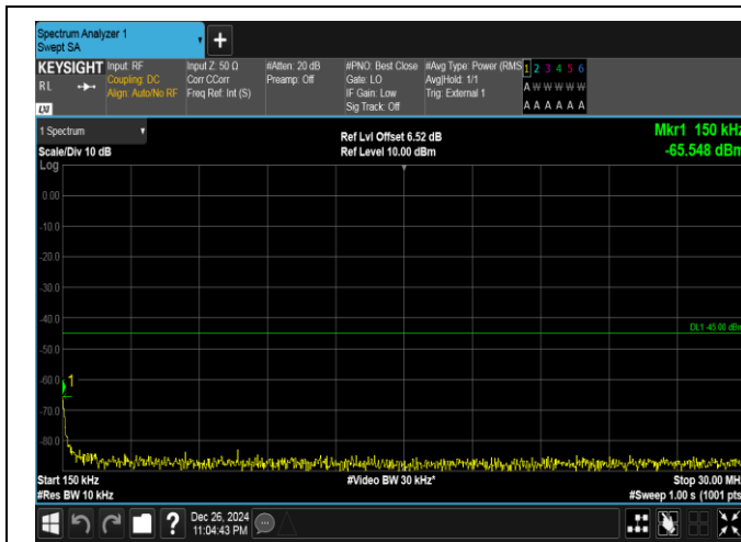
Band41-15MHz-16QAM-39725-75RB#0-0.15~30-PASS
