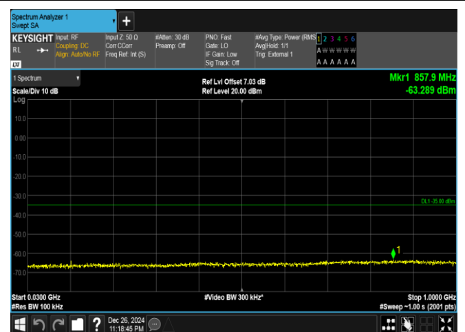
Band41-15MHz-QPSK-41515-1RB#74-30~1000-PASS
