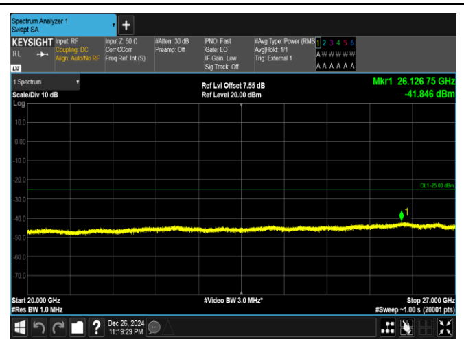
Band41-15MHz-QPSK-41515-1RB#74-20000~27000-PASS
