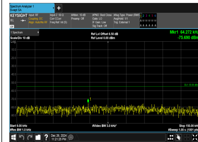
Band41-15MHz-QPSK-41515-75RB#0-0.009~0.15-PASS
