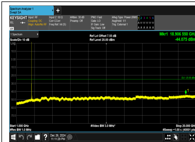
Band41-15MHz-16QAM-40620-1RB#74-1000~20000-PASS
