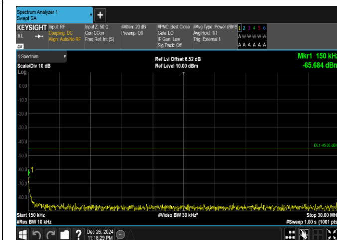
Band41-15MHz-QPSK-41515-1RB#74-0.15~30-PASS
