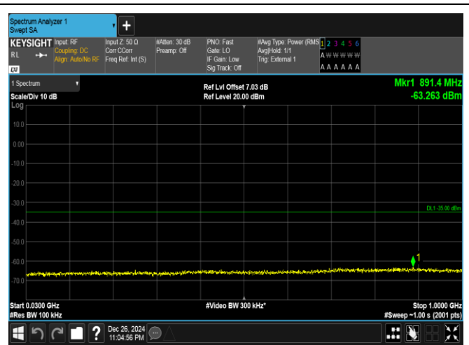
Band41-15MHz-16QAM-39725-75RB#0-30~1000-PASS
