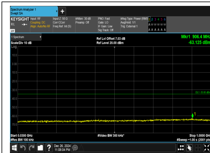
Band41-15MHz-16QAM-40620-1RB#0-30~1000-PASS
