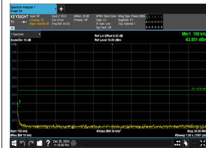
Band41-15MHz-16QAM-41515-1RB#0-0.15~30-PASS
