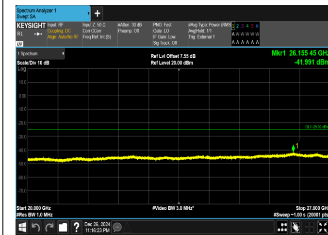
Band41-15MHz-QPSK-41515-1RB#0-20000~27000-PASS
