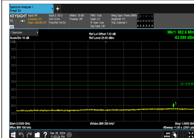
Band41-15MHz-QPSK-39725-75RB#0-30~1000-PASS
