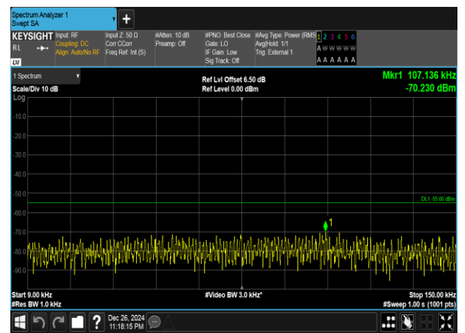
Band41-15MHz-QPSK-41515-1RB#74-0.009~0.15-PASS
