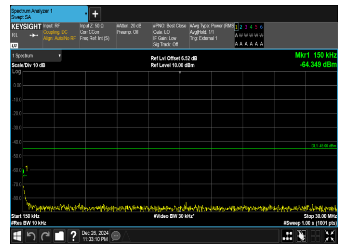
Band41-15MHz-QPSK-39725-75RB#0-0.15~30-PASS
