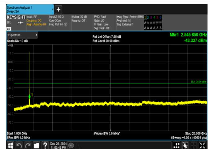
Band41-15MHz-QPSK-39725-75RB#0-1000~20000-PASS
