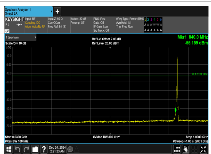
Band5-3MHz-16QAM-20635-15RB#0-30~1000-PASS
