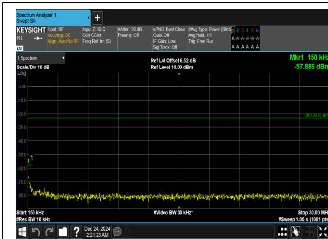
Band5-3MHz-16QAM-20635-15RB#0-0.15~30-PASS
