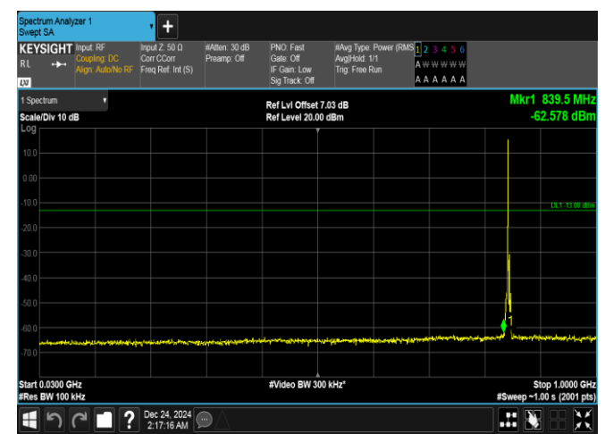
Band5-3MHz-16QAM-20635-1RB#0-30~1000-PASS
