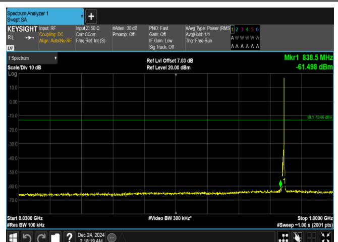
Band5-3MHz-QPSK-20635-1RB#14-30~1000-PASS
