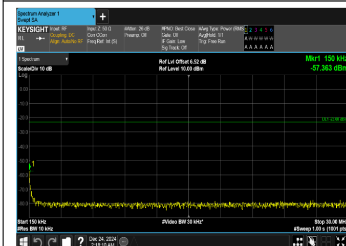
Band5-3MHz-QPSK-20635-1RB#14-0.15~30-PASS
