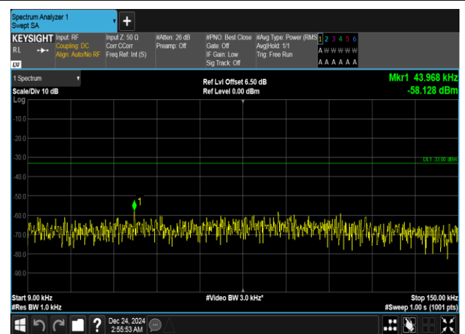
Band5-5MHz-16QAM-20625-25RB#0-0.009~0.15-PASS
