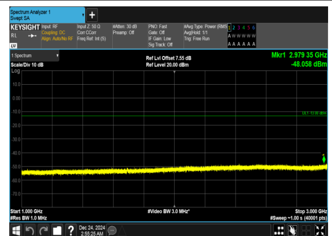
Band5-5MHz-QPSK-20625-25RB#0-1000~3000-PASS
