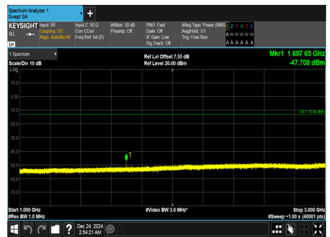
Band5-5MHz-16QAM-20625-1RB#24-1000~3000-PASS
