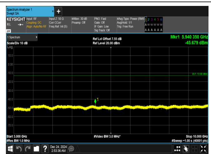
Band5-5MHz-QPSK-20625-1RB#24-3000~10000-PASS
