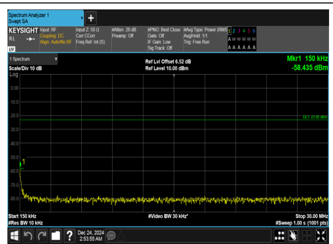
Band5-5MHz-16QAM-20625-1RB#24-0.15~30-PASS
