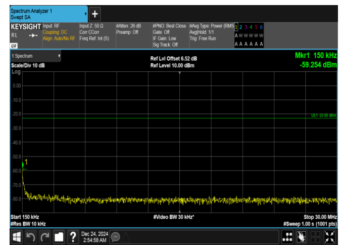
Band5-5MHz-QPSK-20625-25RB#0-0.15~30-PASS
