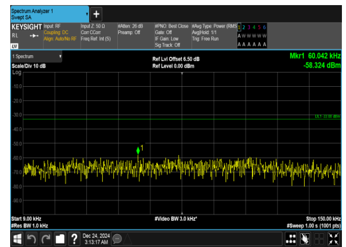
Band5-10MHz-QPSK-20450-1RB#49-0.009~0.15-PASS
