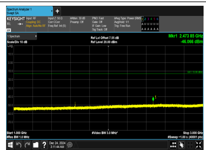
Band5-10MHz-QPSK-20450-1RB#0-1000~3000-PASS
