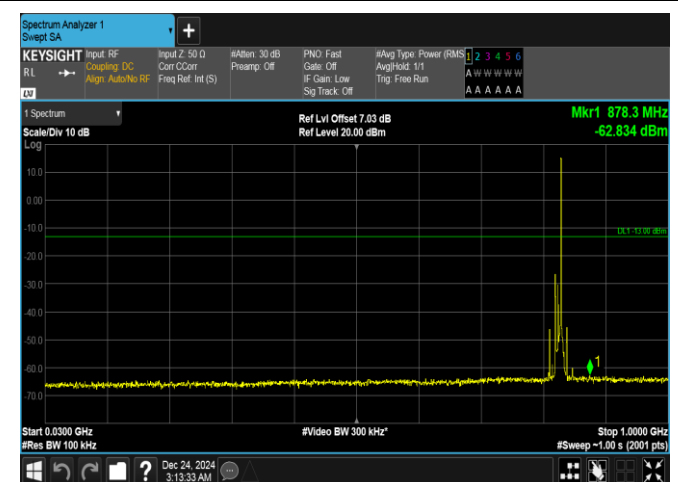
Band5-10MHz-QPSK-20450-1RB#49-30~1000-PASS
