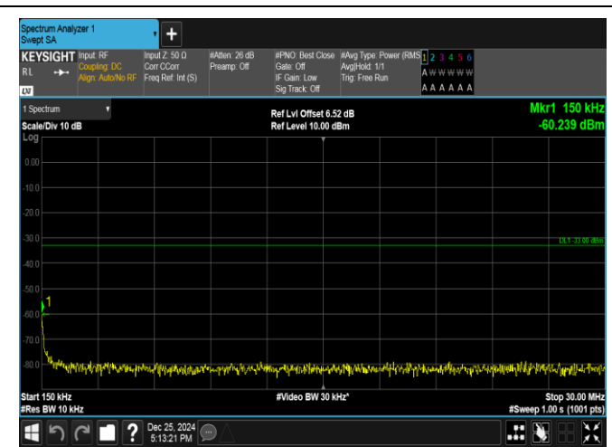
Band66-1.4MHz-16QAM-132665-1RB#5-0.15~30-PASS
