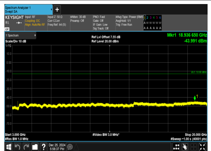
Band66-3MHz-QPSK-132322-1RB#0-3000~20000-PASS
