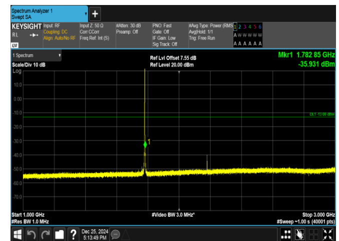
Band66-1.4MHz-16QAM-132665-1RB#5-1000~3000-PASS
