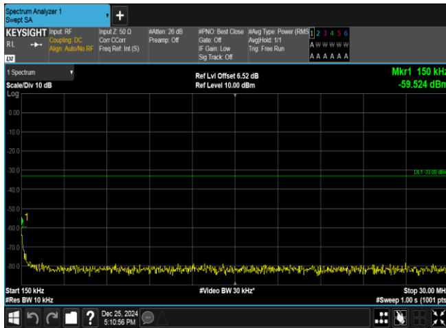
Band66-1.4MHz-16QAM-132665-1RB#0-0.15~30-PASS
