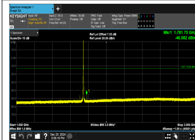
Band66-3MHz-QPSK-132322-1RB#0-1000~3000-PASS
