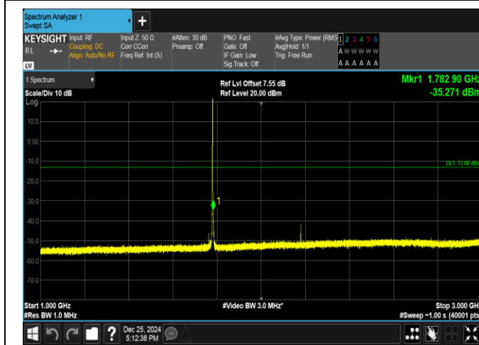
Band66-1.4MHz-QPSK-132665-1RB#5-1000~3000-PASS
