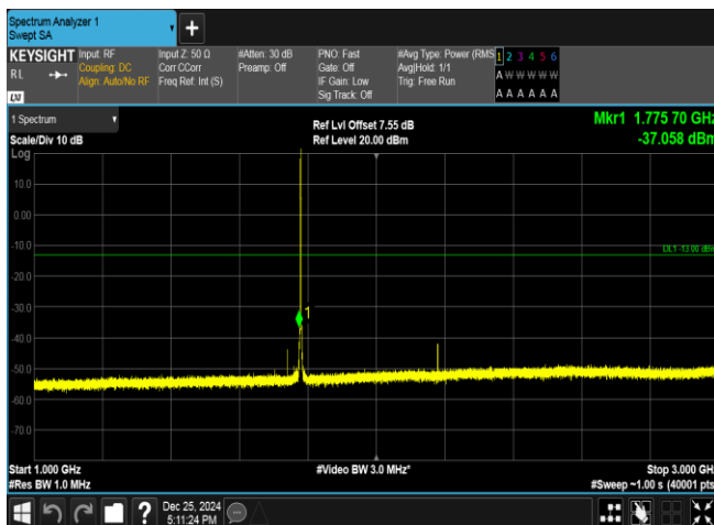
Band66-1.4MHz-16QAM-132665-1RB#0-1000~3000-PAS S
