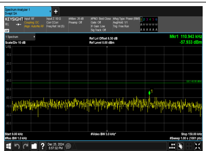
Band66-3MHz-QPSK-132322-1RB#0-0.009~0.15-PASS
