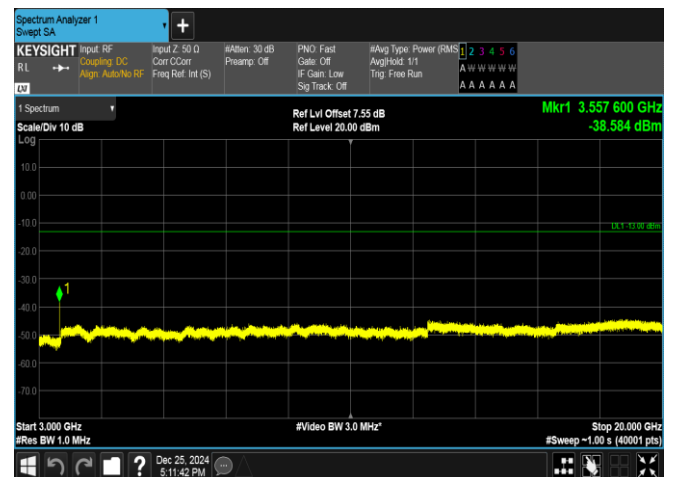
Band66-1.4MHz-16QAM-132665-1RB#0-3000~20000-PA SS
