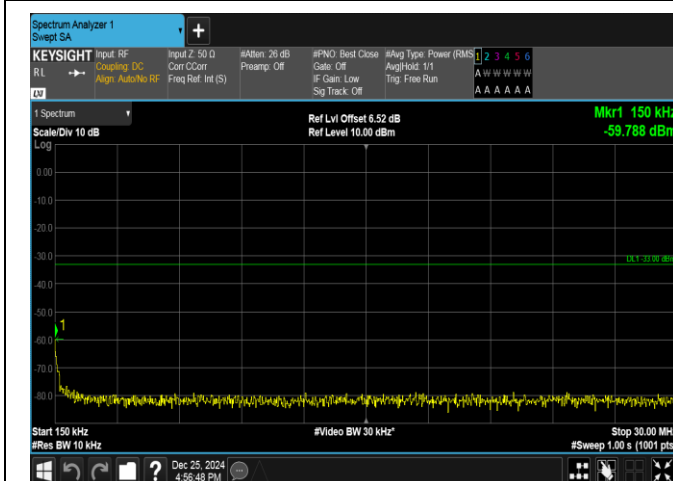
Band66-1.4MHz-16QAM-131979-1RB#0-0.15~30-PASS
