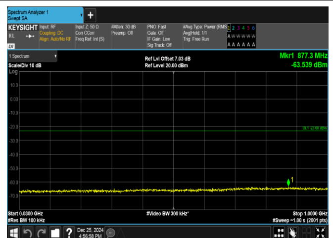
Band66-1.4MHz-16QAM-131979-1RB#0-30~1000-PASS
