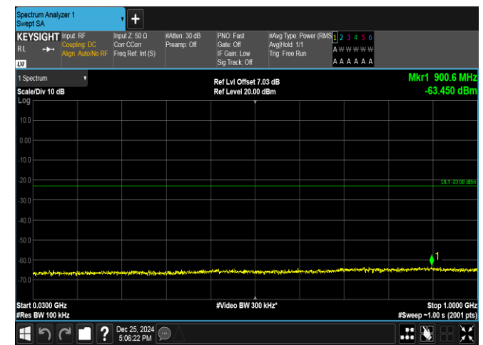
Band66-1.4MHz-16QAM-132322-1RB#5-30~1000-PASS
