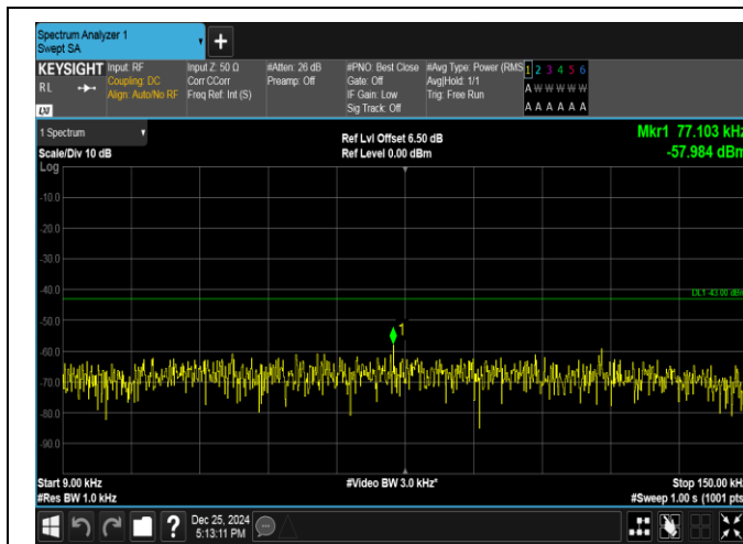
Band66-1.4MHz-16QAM-132665-1RB#5-0.009~0.15-PASS
