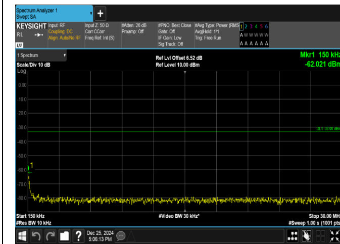
Band66-1.4MHz-16QAM-132322-1RB#5-0.15~30-PASS
