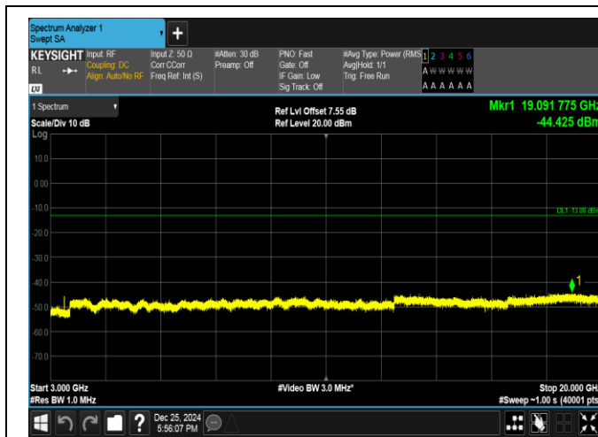
Band66-3MHz-QPSK-131987-15RB#0-3000~20000-PASS
