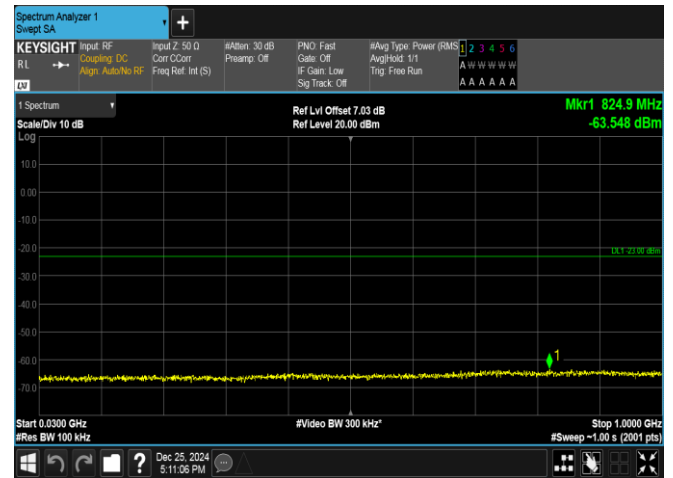
Band66-1.4MHz-16QAM-132665-1RB#0-30~1000-PASS
