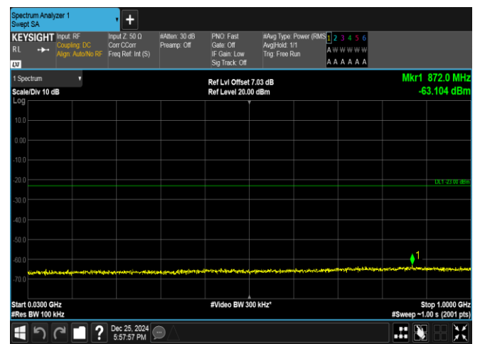
Band66-3MHz-QPSK-132322-1RB#0-30~1000-PASS
