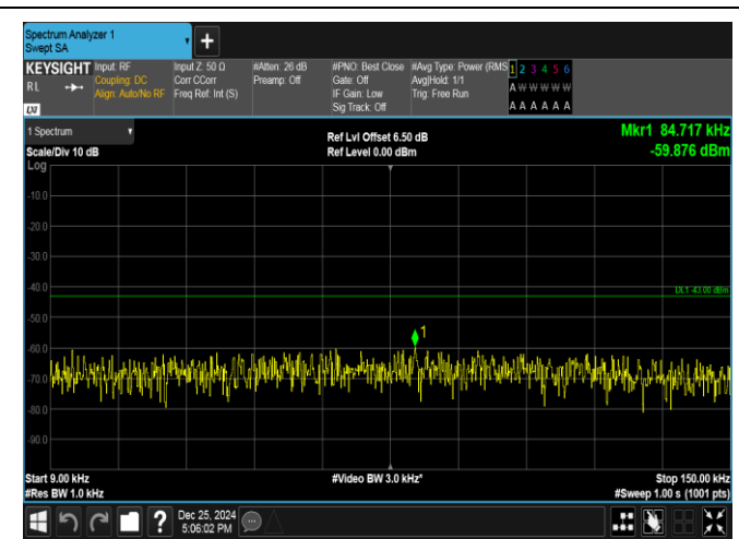
Band66-1.4MHz-16QAM-132322-1RB#5-0.009~0.15-PASS
