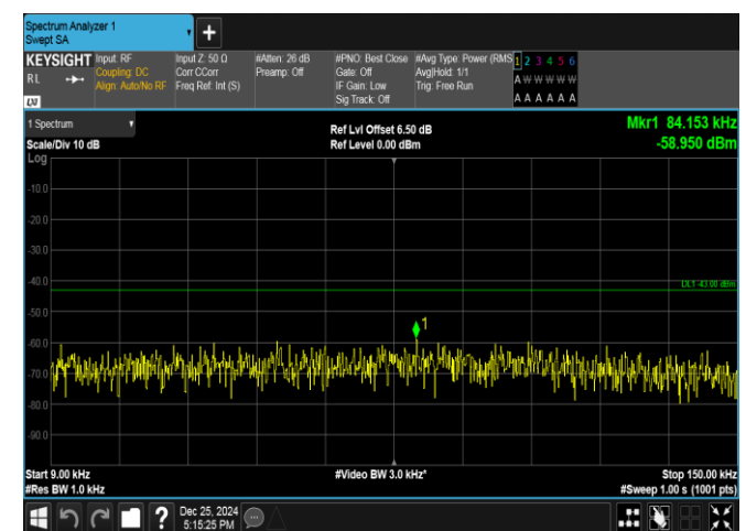
Band66-1.4MHz-16QAM-132665-6RB#0-0.009~0.15-PASS
