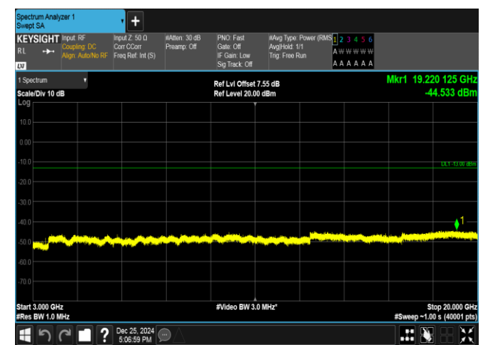
Band66-1.4MHz-16QAM-132322-1RB#5-3000~20000-PASS
