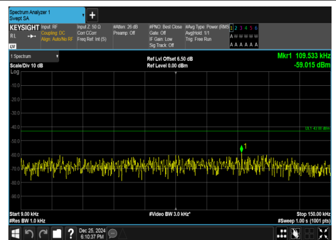
Band66-3MHz-16QAM-132657-15RB#0-0.009~0.15-PASS
