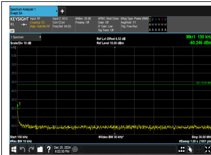
Band66-3MHz-QPSK-132322-15RB#0-0.15~30-PASS
