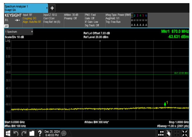
Band66-5MHz-QPSK-131997-1RB#24-30~1000-PASS
