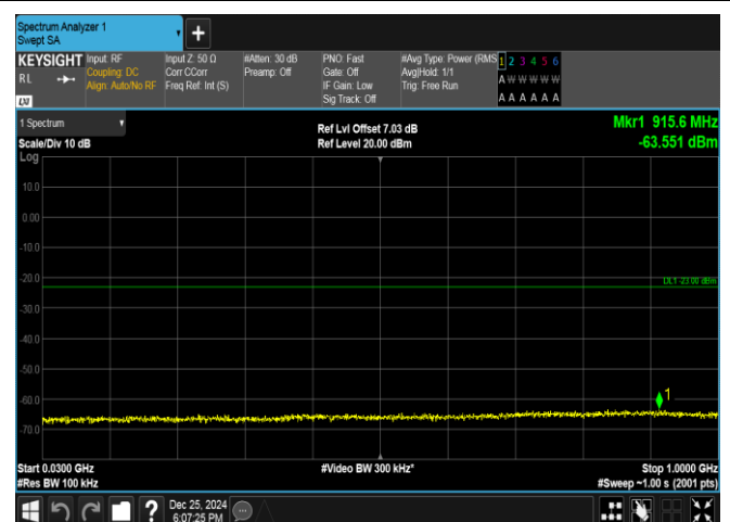
Band66-3MHz-QPSK-132657-1RB#14-30~1000-PASS
