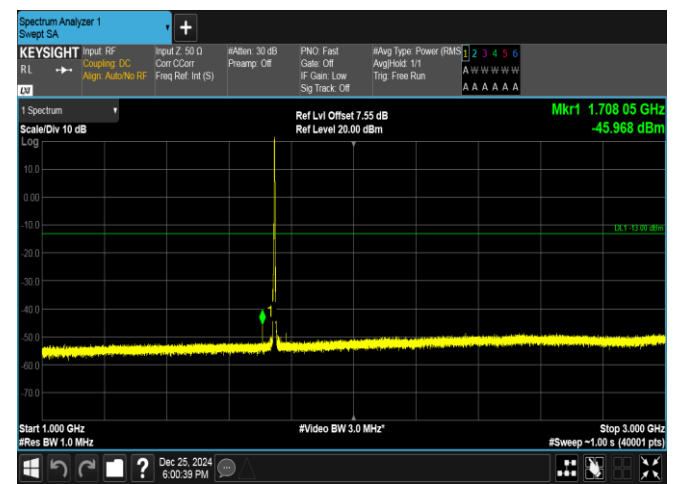
Band66-3MHz-QPSK-132322-1RB#14-1000~3000-PASS
