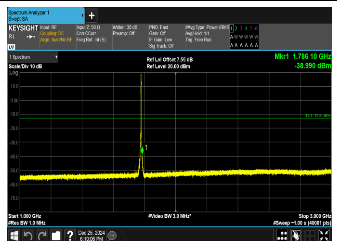
Band66-3MHz-QPSK-132657-15RB#0-1000~3000-PASS
