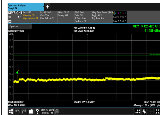
Band66-3MHz-16QAM-131987-1RB#14-3000~20000-PAS
