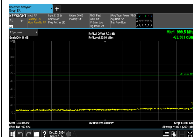
Band66-3MHz-QPSK-132657-15RB#0-30~1000-PASS
