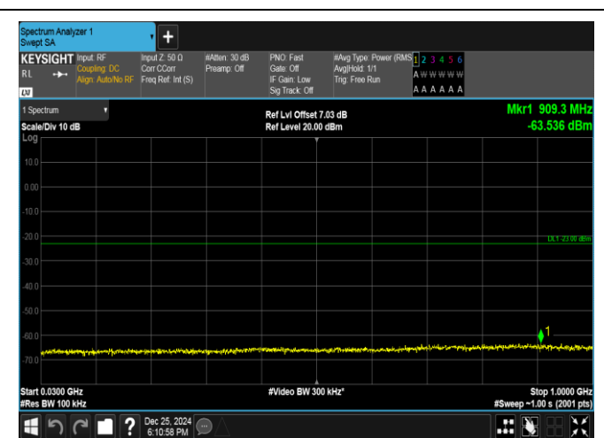
Band66-3MHz-16QAM-132657-15RB#0-30~1000-PASS
