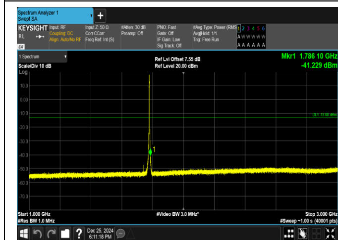
Band66-3MHz-16QAM-132657-15RB#0-1000~3000-PASS
