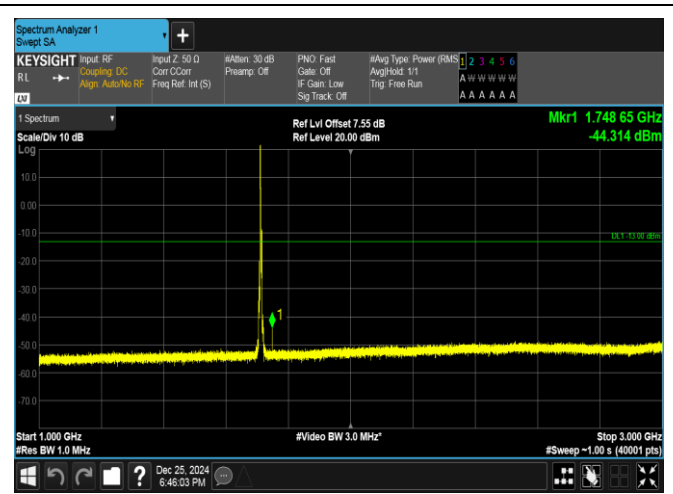
Band66-5MHz-QPSK-131997-1RB#0-1000~3000-PASS
