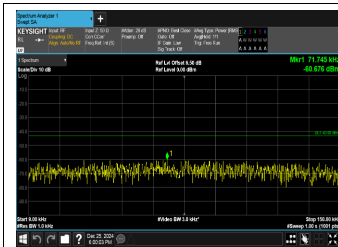
Band66-3MHz-QPSK-132322-1RB#14-0.009~0.15-PASS
