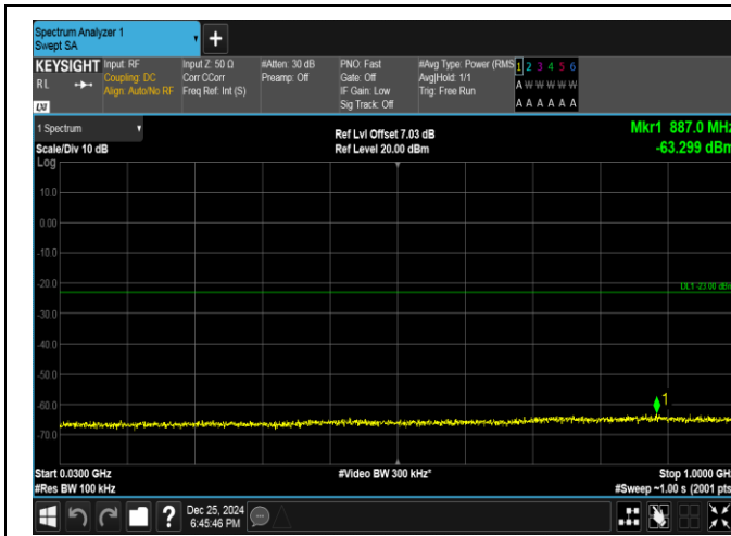
Band66-5MHz-QPSK-131997-1RB#0-30~1000-PASS
