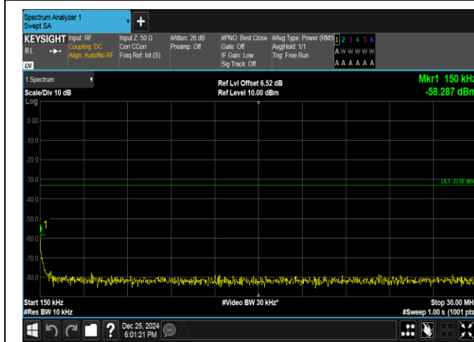
Band66-3MHz-16QAM-132322-1RB#14-0.15~30-PASS
