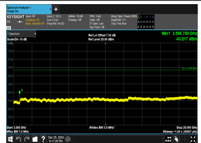
Band66-3MHz-16QAM-132657-15RB#0-3000~20000-PASS
