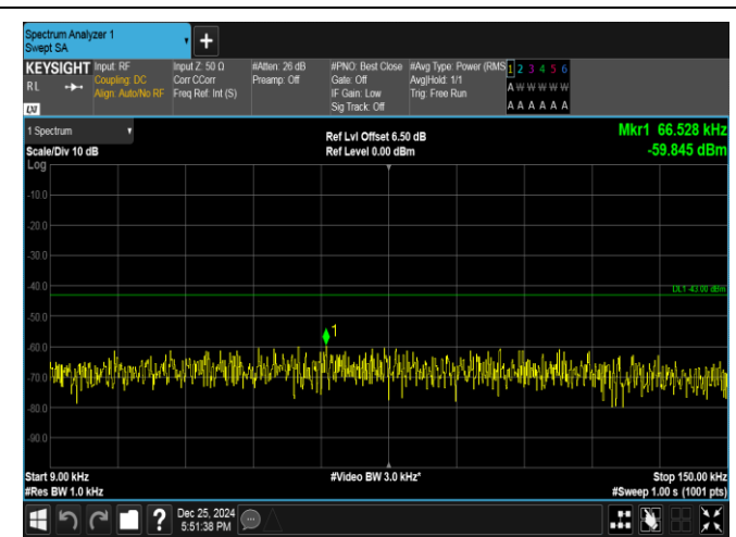
Band66-3MHz-16QAM-131987-1RB#0-0.009~0.15-PASS
