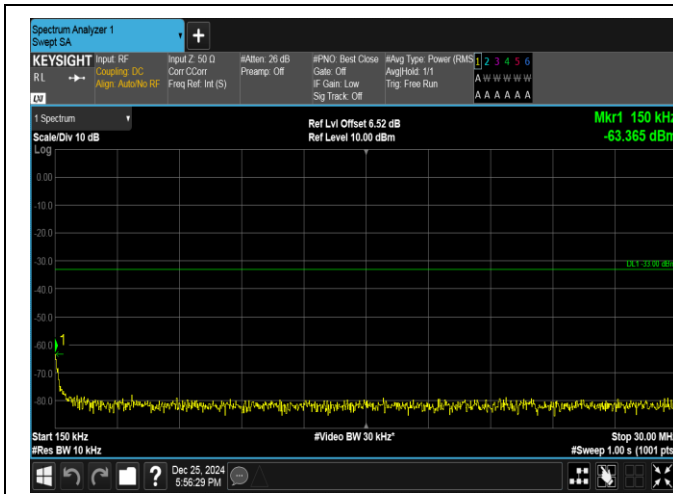
Band66-3MHz-16QAM-131987-15RB#0-0.15~30-PASS
