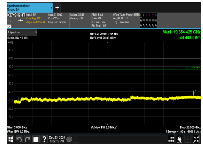
Band66-3MHz-16QAM-131987-15RB#0-3000~20000-PASS
