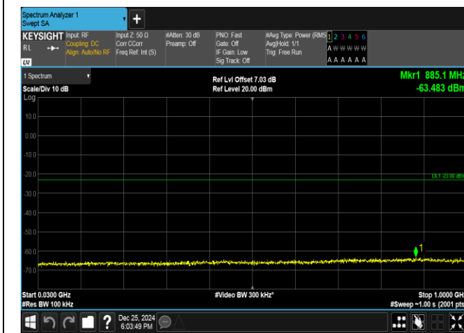
Band66-3MHz-16QAM-132322-15RB#0-30~1000-PASS
