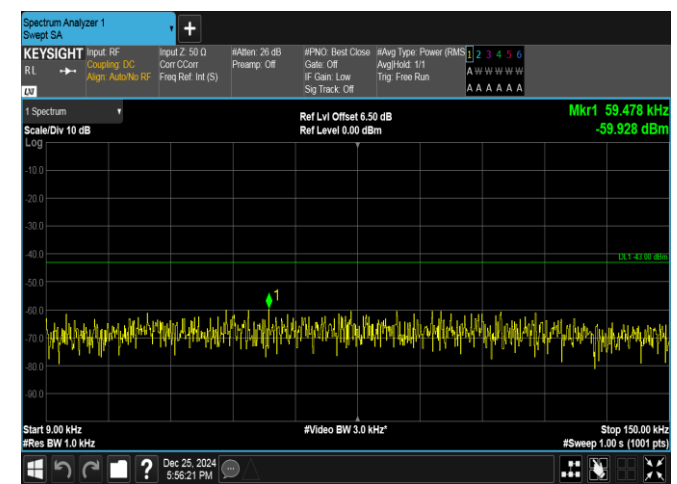
Band66-3MHz-16QAM-131987-15RB#0-0.009~0.15-PASS
