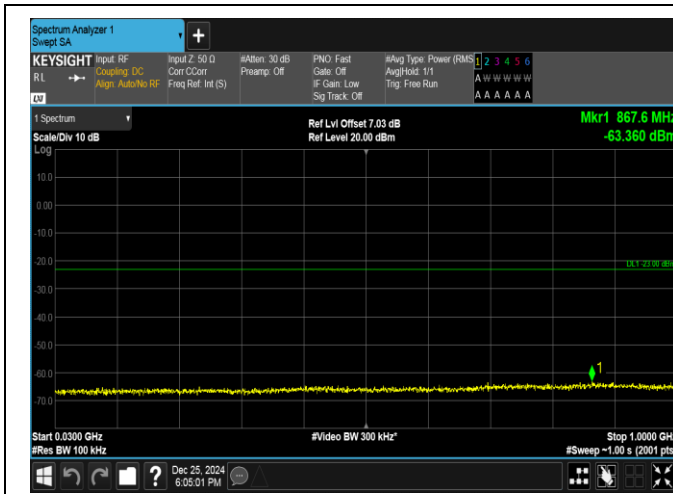
Band66-3MHz-QPSK-132657-1RB#0-30~1000-PASS
