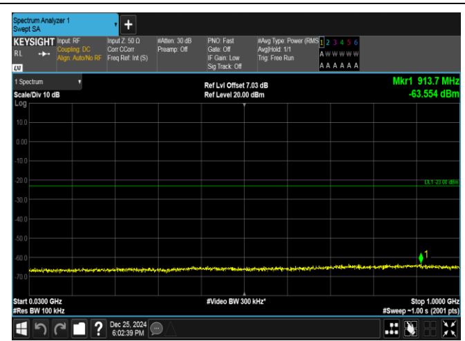
Band66-3MHz-QPSK-132322-15RB#0-30~1000-PASS
