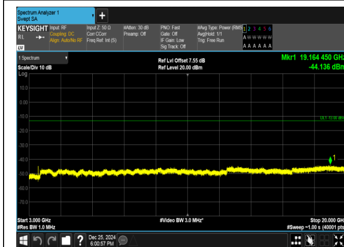
Band66-3MHz-QPSK-132322-1RB#14-3000~20000-PASS
