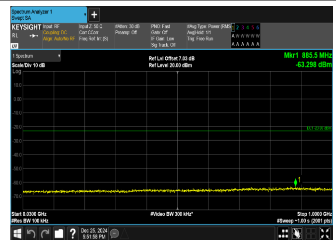
Band66-3MHz-16QAM-131987-1RB#0-30~1000-PASS
