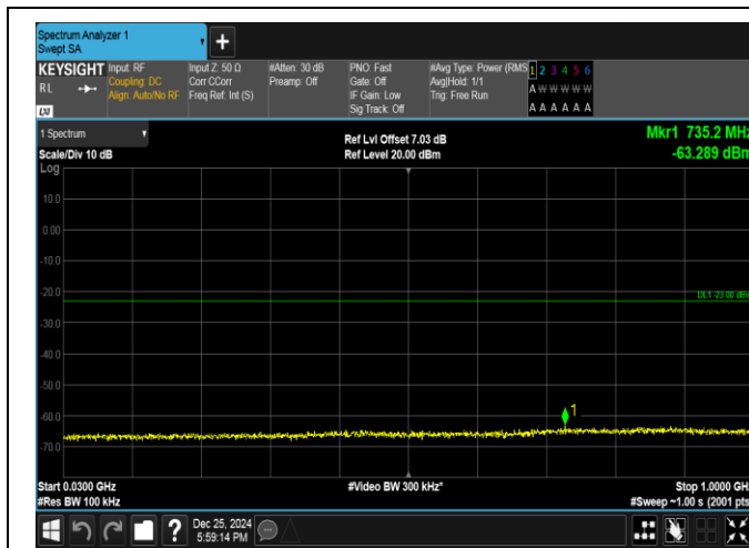
Band66-3MHz-16QAM-132322-1RB#0-30~1000-PASS
