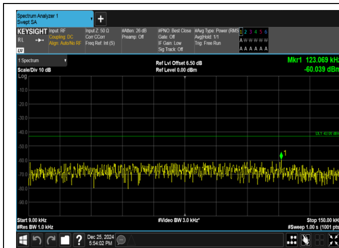
Band66-3MHz-16QAM-131987-1RB#14-0.009~0.15-PASS
