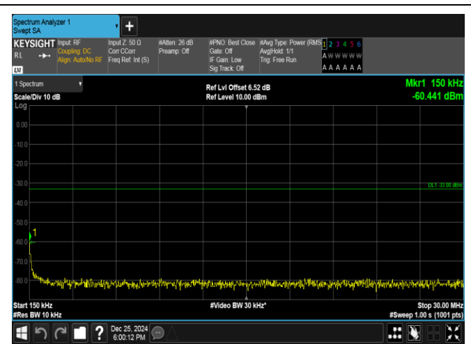
Band66-3MHz-QPSK-132322-1RB#14-0.15~30-PASS
