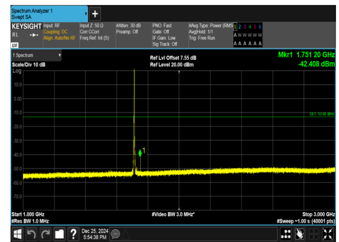
Band66-3MHz-16QAM-131987-1RB#14-1000~3000-PASS
