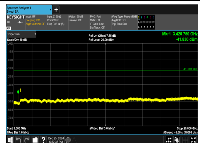
Band66-3MHz-16QAM-131987-1RB#0-3000~20000-PASS
