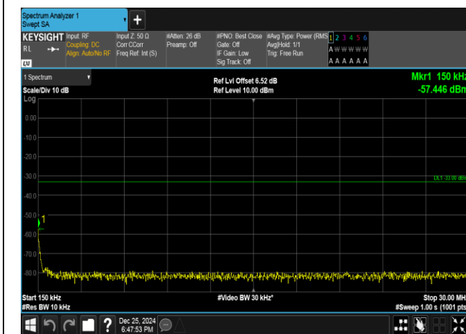
Band66-5MHz-QPSK-131997-1RB#24-0.15~30-PASS
