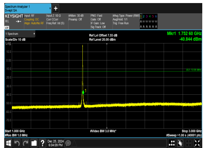
Band66-3MHz-16QAM-132322-15RB#0-1000~3000-PASS
