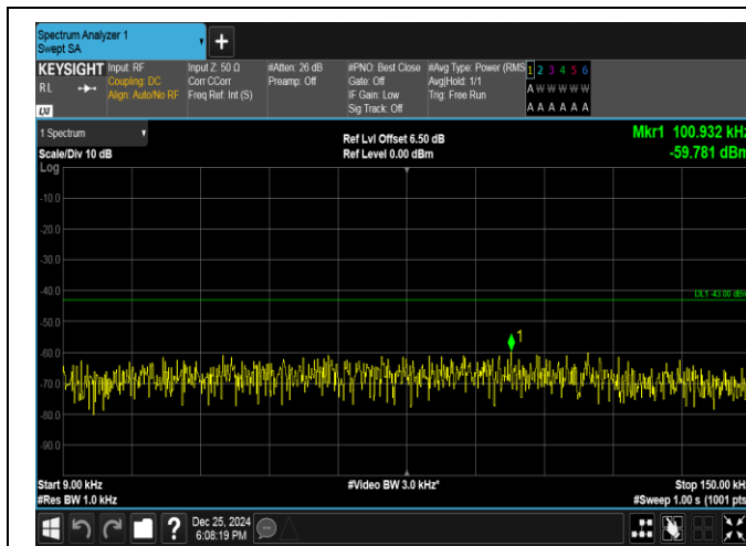
Band66-3MHz-16QAM-132657-1RB#14-0.009~0.15-PASS
