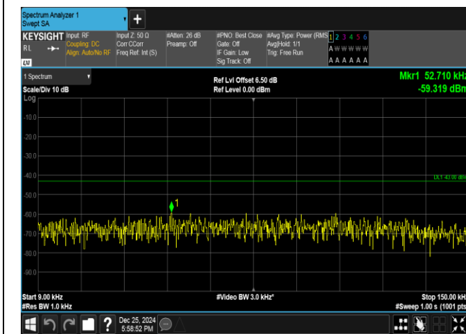
Band66-3MHz-16QAM-132322-1RB#0-0.009~0.15-PASS
