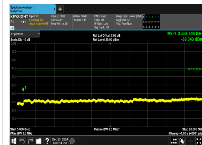
Band66-3MHz-16QAM-132657-1RB#14-3000~20000-PAS
