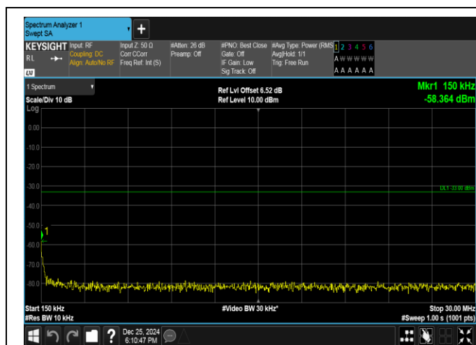
Band66-3MHz-16QAM-132657-15RB#0-0.15~30-PASS
