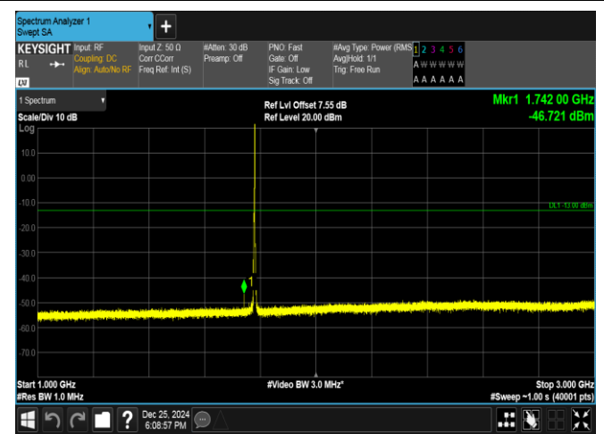
Band66-3MHz-16QAM-132657-1RB#14-1000~3000-PASS
