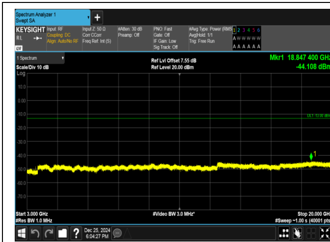
Band66-3MHz-16QAM-132322-15RB#0-3000~20000-PAS S
