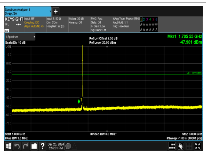
Band66-3MHz-16QAM-132322-1RB#0-1000~3000-PASS
