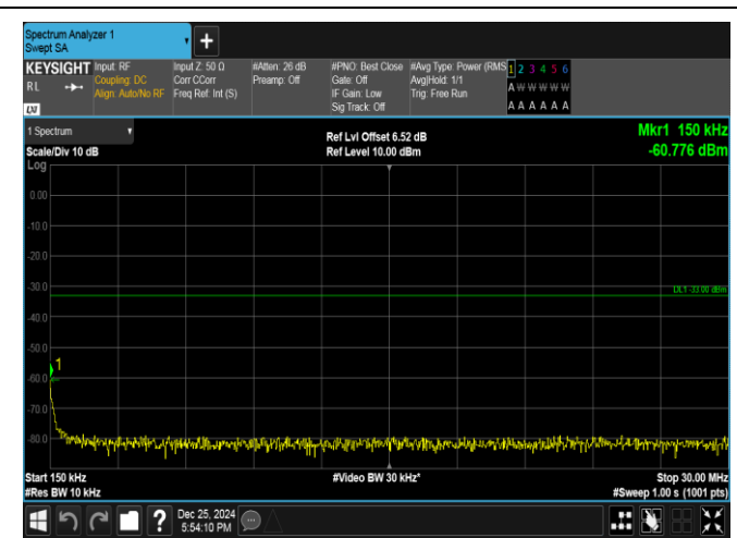
Band66-3MHz-16QAM-131987-1RB#14-0.15~30-PASS
