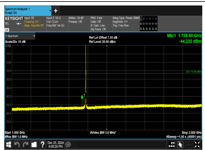
Band66-3MHz-QPSK-132657-1RB#0-1000~3000-PASS
