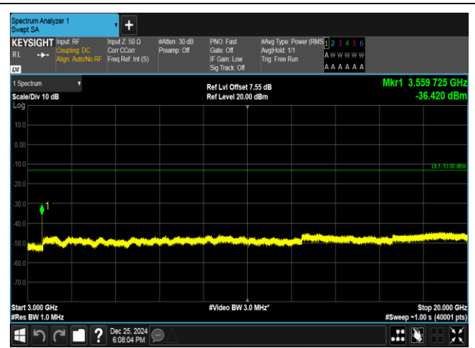
Band66-3MHz-QPSK-132657-1RB#14-3000~20000-PASS
