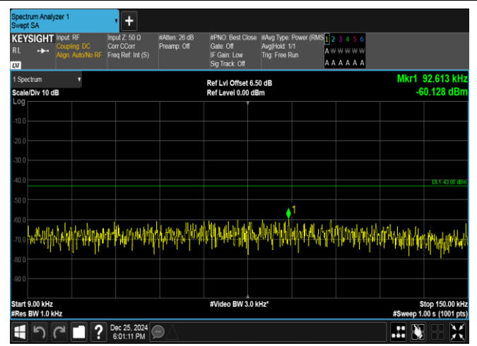
Band66-3MHz-16QAM-132322-1RB#14-0.009~0.15-PASS
