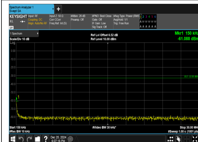
Band66-3MHz-QPSK-132657-1RB#14-0.15~30-PASS
