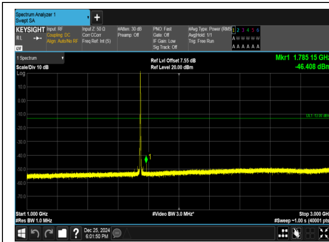
Band66-3MHz-16QAM-132322-1RB#14-1000~3000-PASS
