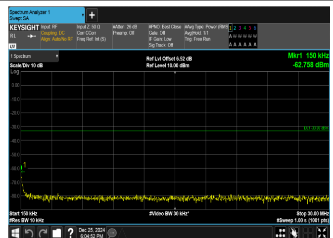
Band66-3MHz-QPSK-132657-1RB#0-0.15~30-PASS
