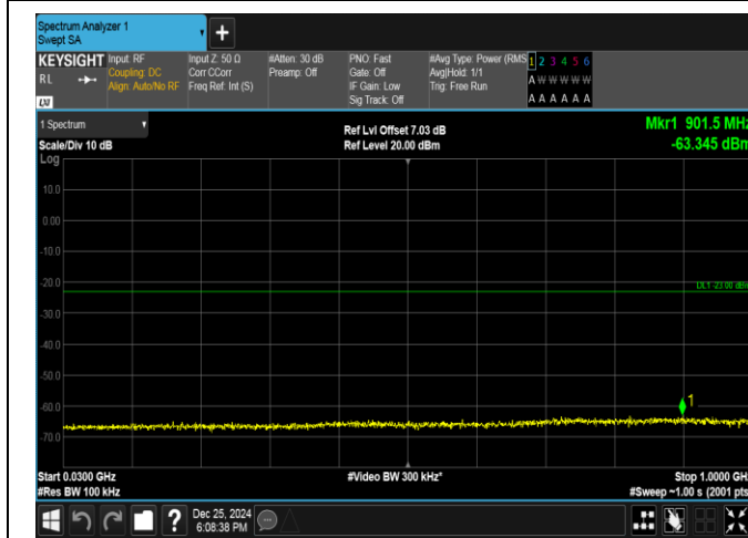
Band66-3MHz-16QAM-132657-1RB#14-30~1000-PASS
