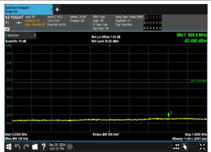
Band66-3MHz-16QAM-132322-1RB#14-30~1000-PASS
