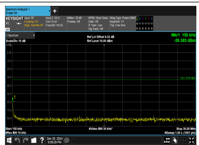
Band66-3MHz-16QAM-132657-1RB#14-0.15~30-PASS
