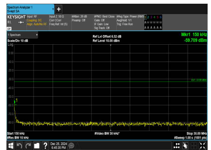
Band66-5MHz-QPSK-131997-1RB#0-0.15~30-PASS
