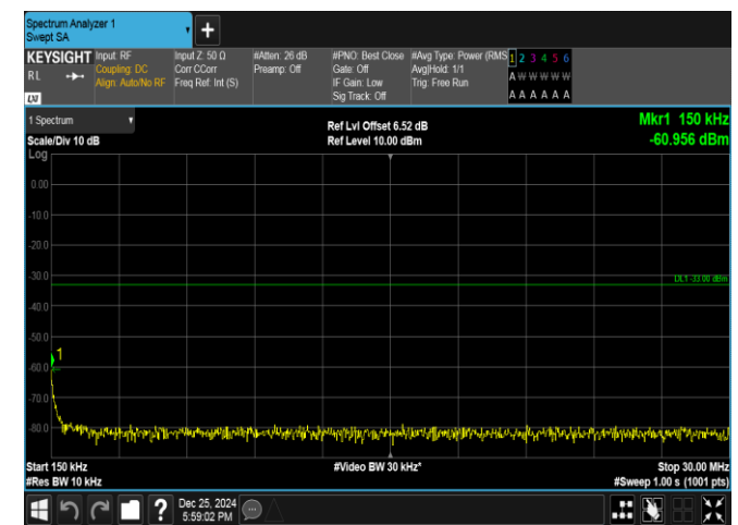
Band66-3MHz-16QAM-132322-1RB#0-0.15~30-PASS
