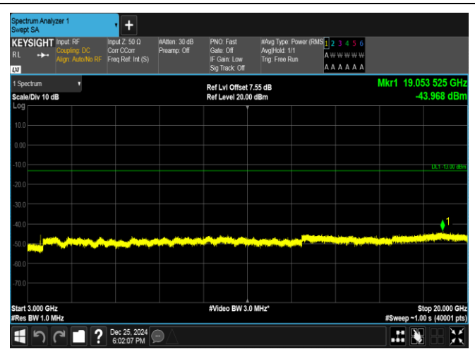
Band66-3MHz-16QAM-132322-1RB#14-3000~20000-PASS
