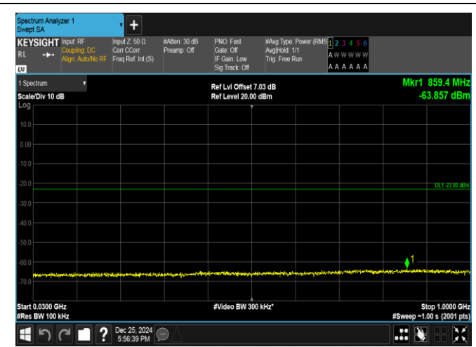
Band66-3MHz-16QAM-131987-15RB#0-30~1000-PASS
