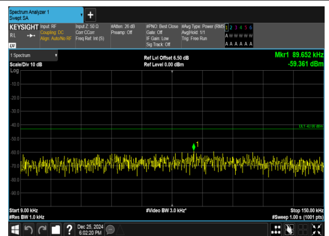
Band66-3MHz-QPSK-132322-15RB#0-0.009~0.15-PASS
