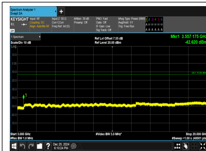
Band66-3MHz-QPSK-132657-15RB#0-3000~20000-PASS
