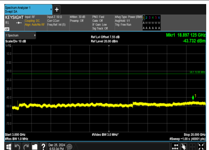
Band66-5MHz-QPSK-132322-1RB#0-3000~20000-PASS
