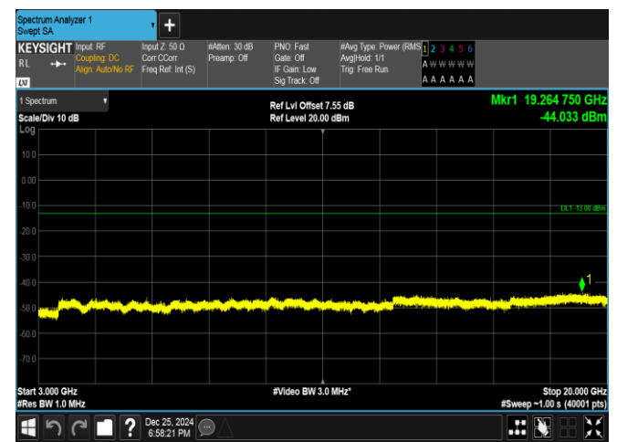
Band66-5MHz-QPSK-132322-25RB#0-3000~20000-PASS
