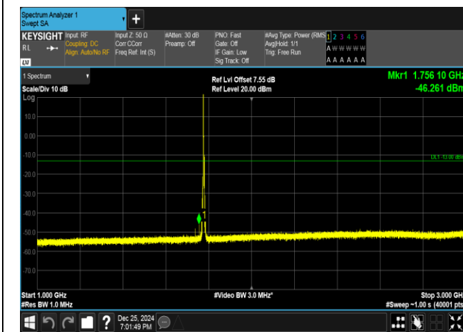
Band66-5MHz-16QAM-132647-1RB#0-1000~3000-PASS
