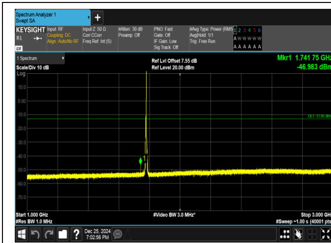
Band66-5MHz-QPSK-132647-1RB#24-1000~3000-PASS
