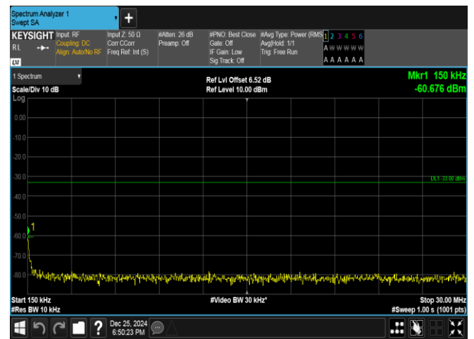
Band66-5MHz-QPSK-131997-25RB#0-0.15~30-PASS
