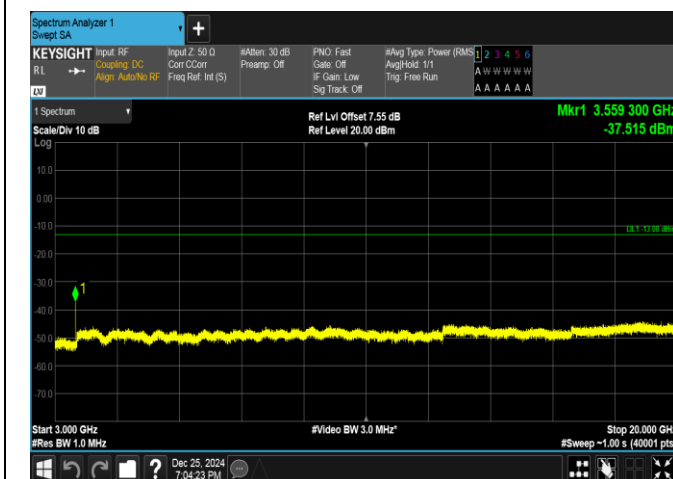
Band66-5MHz-16QAM-132647-1RB#24-3000~20000-PAS
