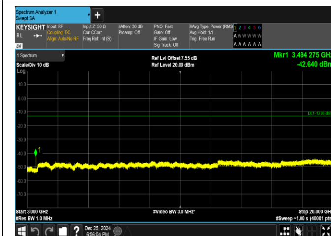
Band66-5MHz-QPSK-132322-1RB#24-3000~20000-PASS
