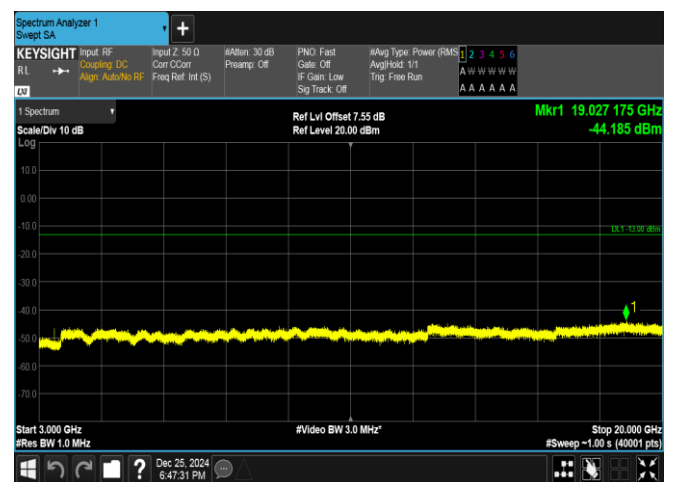
Band66-5MHz-16QAM-131997-1RB#0-3000~20000-PASS
