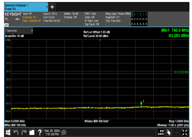
Band66-5MHz-16QAM-132647-1RB#0-30~1000-PASS
