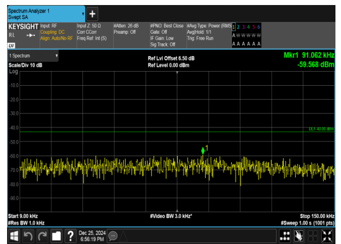
Band66-5MHz-16QAM-132322-1RB#24-0.009~0.15-PASS
