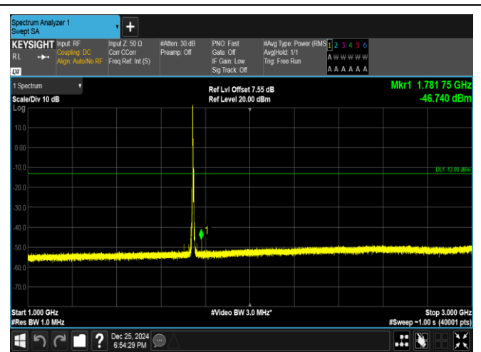
Band66-5MHz-16QAM-132322-1RB#0-1000~3000-PASS
