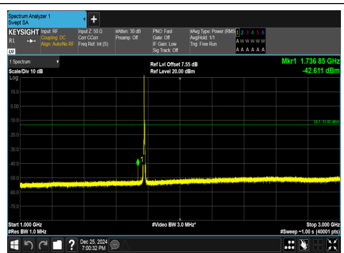
Band66-5MHz-QPSK-132647-1RB#0-1000~3000-PASS
