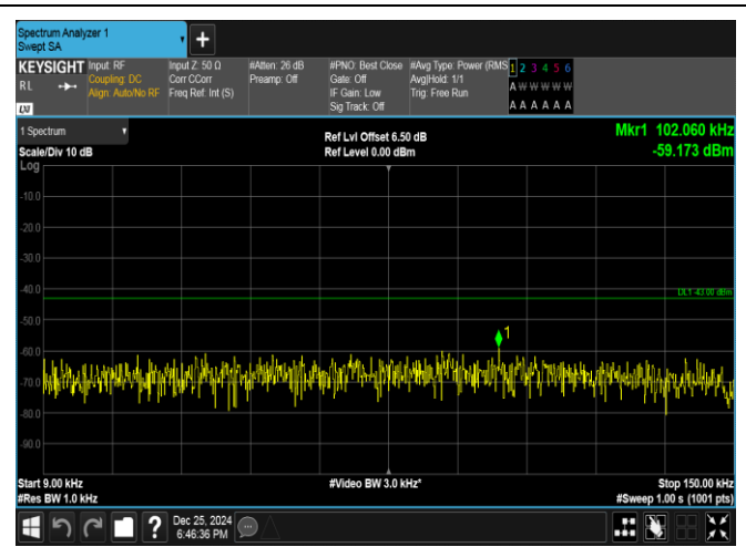
Band66-5MHz-16QAM-131997-1RB#0-0.009~0.15-PASS
