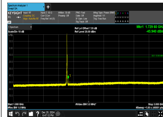
Band66-5MHz-16QAM-131997-1RB#0-1000~3000-PASS
