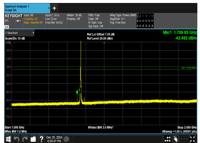
Band66-5MHz-QPSK-132322-1RB#24-1000~3000-PASS
