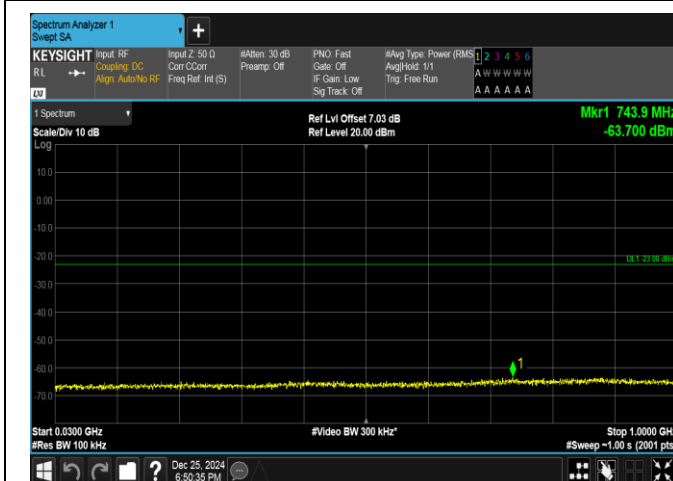
Band66-5MHz-QPSK-131997-25RB#0-30~1000-PASS
