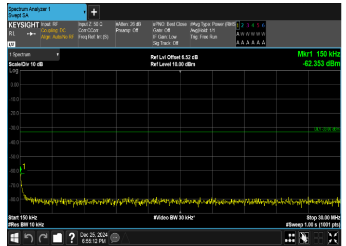
Band66-5MHz-QPSK-132322-1RB#24-0.15~30-PASS
