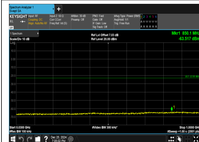
Band66-5MHz-QPSK-132647-25RB#0-30~1000-PASS
