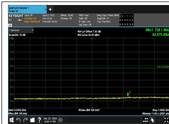
Band66-5MHz-16QAM-132322-1RB#0-30~1000-PASS
