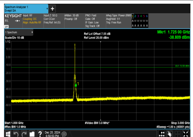
Band66-5MHz-QPSK-131997-25RB#0-1000~3000-PASS
