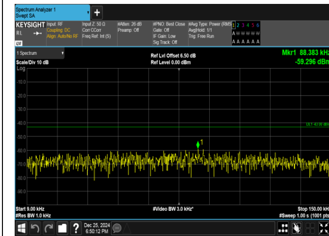
Band66-5MHz-QPSK-131997-25RB#0-0.009~0.15-PASS
