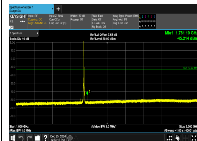
Band66-5MHz-QPSK-132322-1RB#0-1000~3000-PASS
