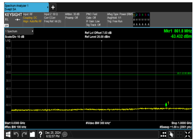
Band66-5MHz-QPSK-132322-1RB#0-30~1000-PASS
