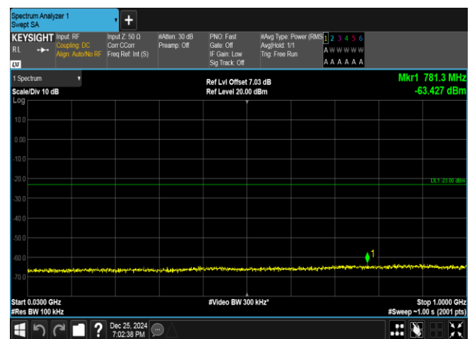
Band66-5MHz-QPSK-132647-1RB#24-30~1000-PASS
