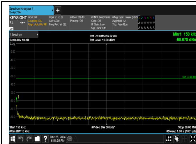
Band66-5MHz-16QAM-131997-25RB#0-0.15~30-PASS
