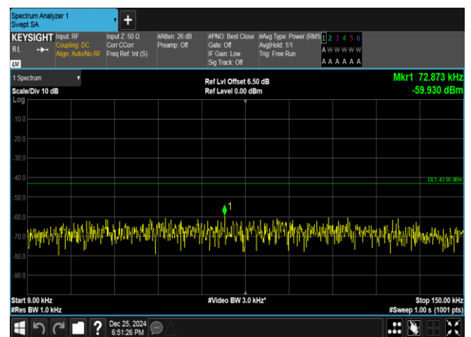
Band66-5MHz-16QAM-131997-25RB#0-0.009~0.15-PASS
