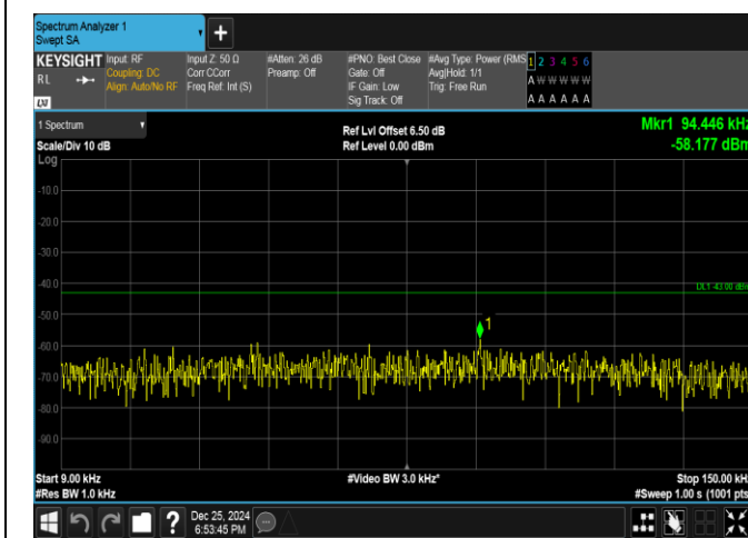
Band66-5MHz-16QAM-132322-1RB#0-0.009~0.15-PASS
