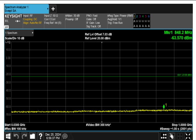
Band66-5MHz-16QAM-132322-1RB#24-30~1000-PASS
