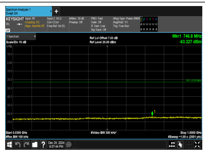
Band66-5MHz-QPSK-132322-25RB#0-30~1000-PASS
