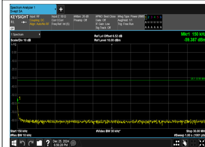
Band66-5MHz-16QAM-132322-1RB#24-0.15~30-PASS
