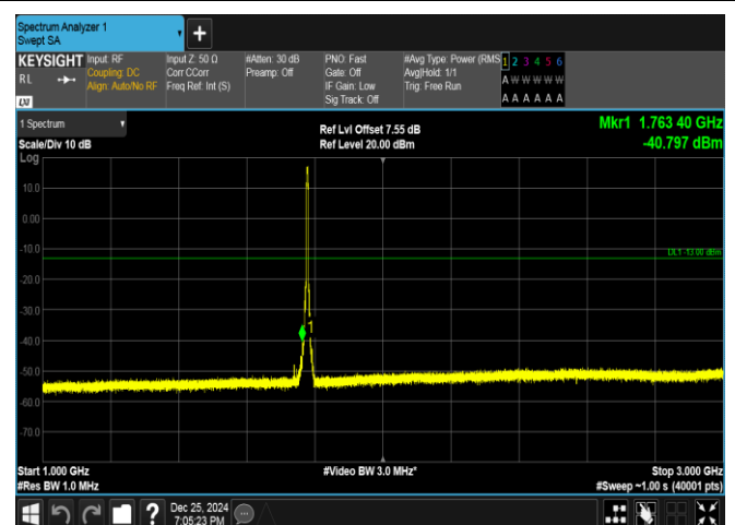
Band66-5MHz-QPSK-132647-25RB#0-1000~3000-PASS
