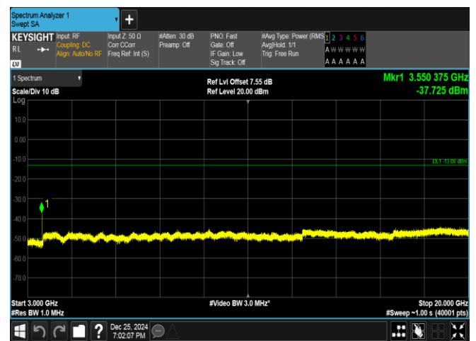
Band66-5MHz-16QAM-132647-1RB#0-3000~20000-PASS
