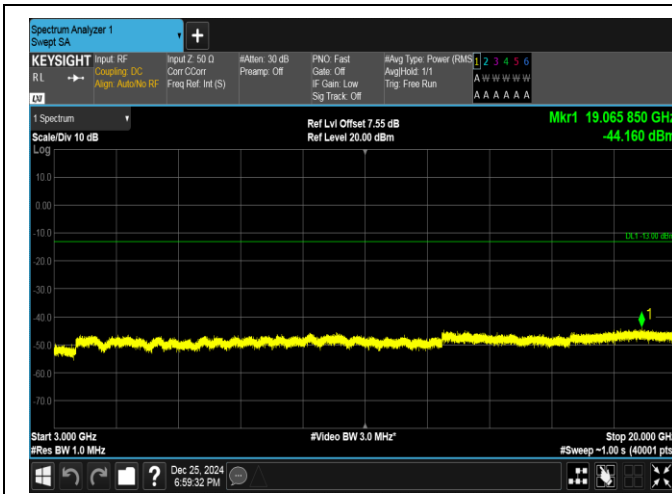
Band66-5MHz-16QAM-132322-25RB#0-3000~20000-PAS
