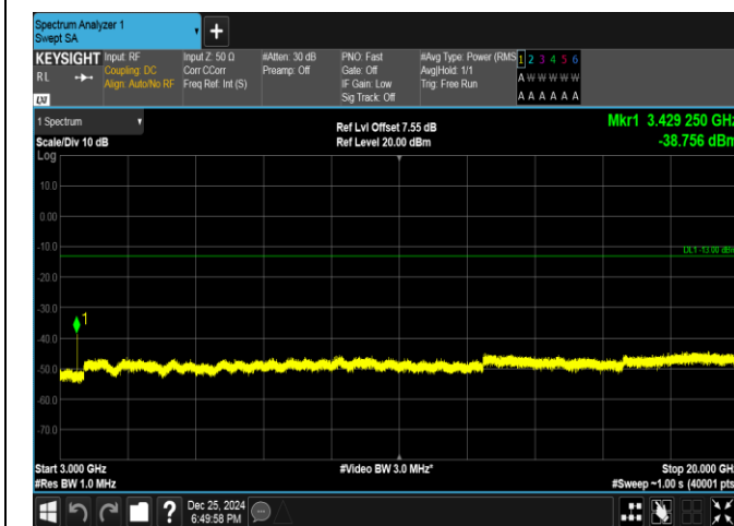
Band66-5MHz-16QAM-131997-1RB#24-3000~20000-PAS
