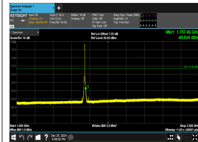
Band66-5MHz-QPSK-132322-25RB#0-1000~3000-PASS
