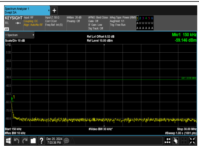
Band66-5MHz-16QAM-132647-1RB#24-0.15~30-PASS
