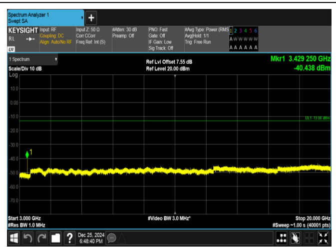
Band66-5MHz-QPSK-131997-1RB#24-3000~20000-PASS
