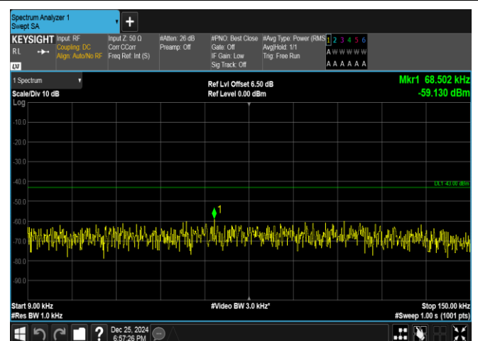
Band66-5MHz-QPSK-132322-25RB#0-0.009~0.15-PASS
