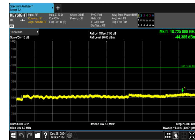
Band66-5MHz-16QAM-132322-1RB#0-3000~20000-PASS
