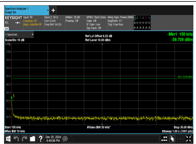
Band66-5MHz-16QAM-131997-1RB#24-0.15~30-PASS
