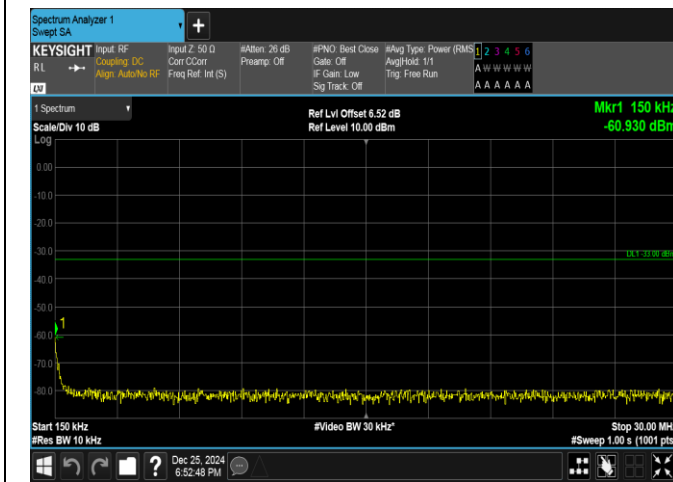
Band66-5MHz-QPSK-132322-1RB#0-0.15~30-PASS
