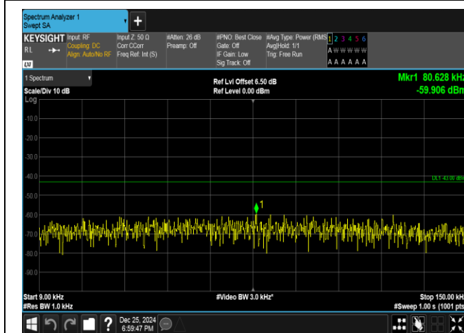
Band66-5MHz-QPSK-132647-1RB#0-0.009~0.15-PASS
