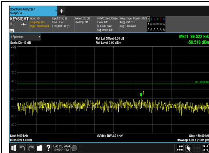
Band66-5MHz-QPSK-132322-1RB#24-0.009~0.15-PASS
