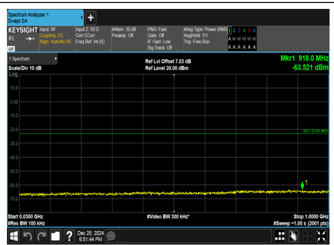
Band66-5MHz-16QAM-131997-25RB#0-30~1000-PASS
