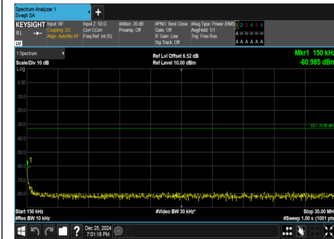
Band66-5MHz-16QAM-132647-1RB#0-0.15~30-PASS
