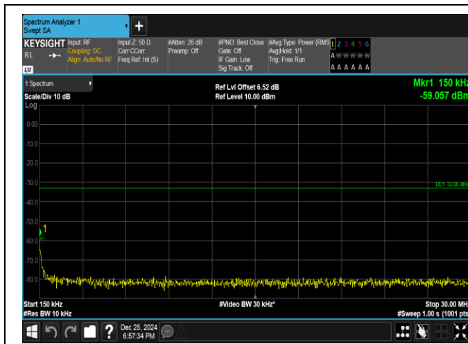
Band66-5MHz-QPSK-132322-25RB#0-0.15~30-PASS
