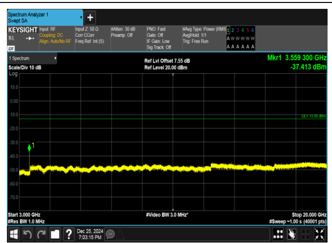
Band66-5MHz-QPSK-132647-1RB#24-3000~20000-PASS
