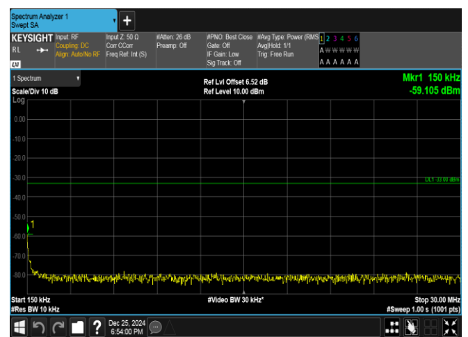
Band66-5MHz-16QAM-132322-1RB#0-0.15~30-PASS
