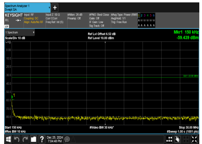
Band66-5MHz-QPSK-132647-25RB#0-0.15~30-PASS
