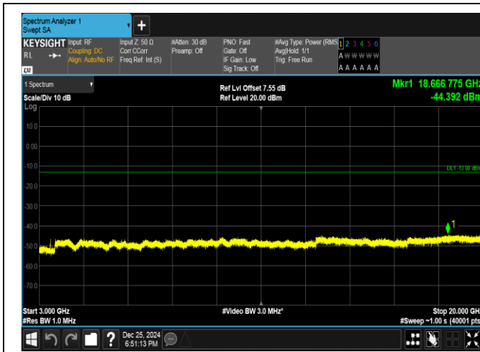
Band66-5MHz-QPSK-131997-25RB#0-3000~20000-PASS
