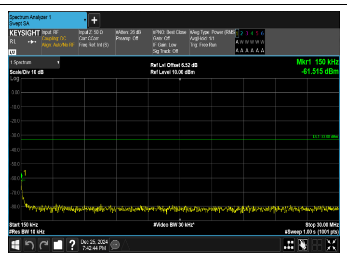
Band66-10MHz-16QAM-132022-1RB#49-0.15~30-PASS
