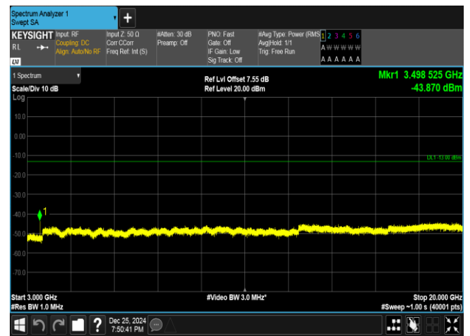
Band66-10MHz-16QAM-132322-1RB#49-3000~20000-PA
