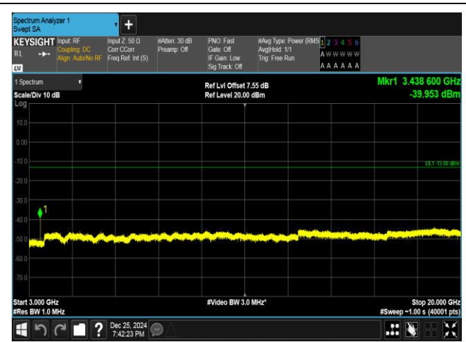
Band66-10MHz-QPSK-132022-1RB#49-3000~20000-PASS
