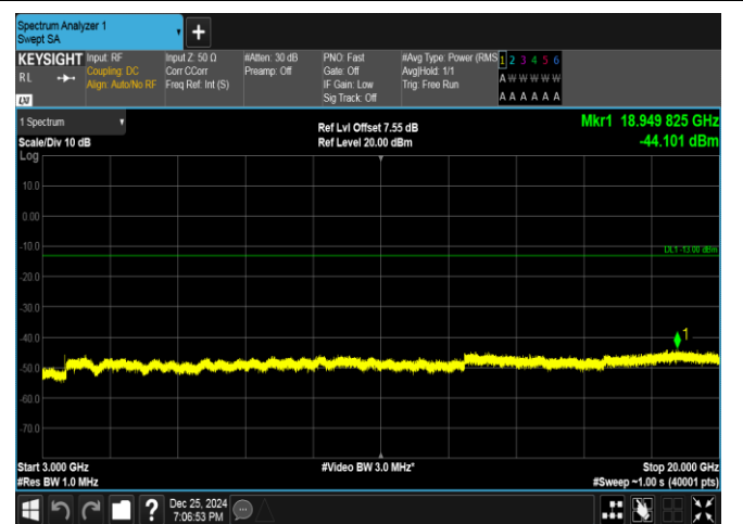
Band66-5MHz-16QAM-132647-25RB#0-3000~20000-PASS
