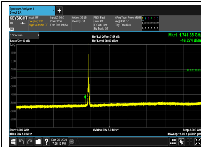
Band66-10MHz-QPSK-132622-1RB#49-1000~3000-PASS
