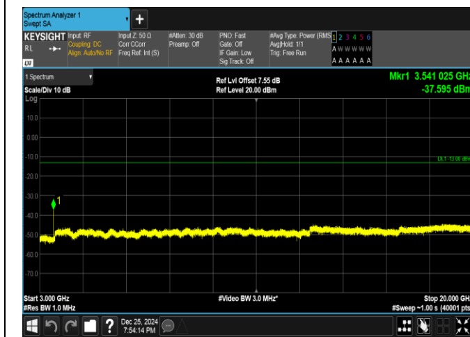
Band66-10MHz-QPSK-132622-1RB#0-3000~20000-PASS
