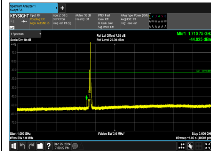
Band66-10MHz-16QAM-132322-1RB#49-1000~3000-PAS
