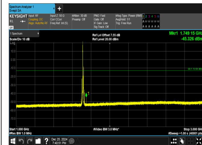
Band66-10MHz-16QAM-132022-1RB#0-1000~3000-PASS
