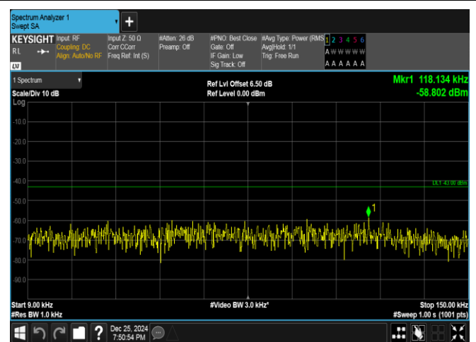
Band66-10MHz-QPSK-132322-50RB#0-0.009~0.15-PASS
