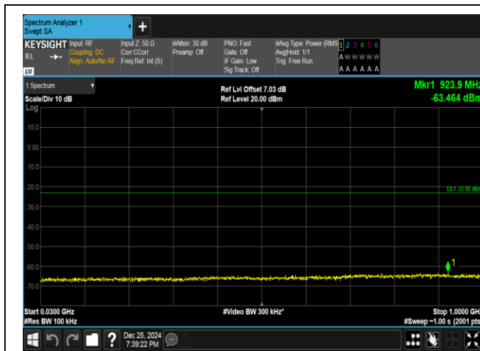
Band66-10MHz-QPSK-132022-1RB#0-30~1000-PASS
