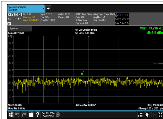
Band66-10MHz-QPSK-132322-1RB#49-0.009~0.15-PASS
