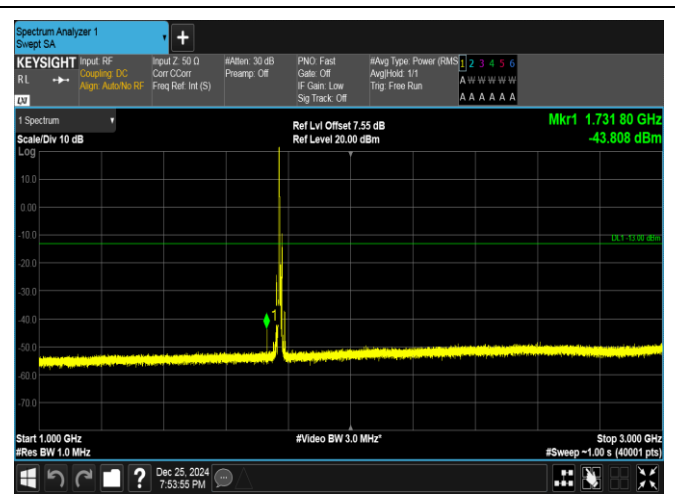
Band66-10MHz-QPSK-132622-1RB#0-1000~3000-PASS
