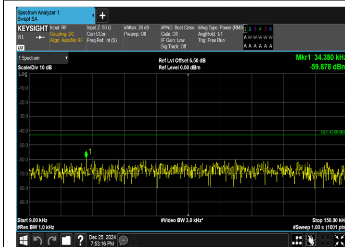
Band66-10MHz-QPSK-132622-1RB#0-0.009~0.15-PASS
