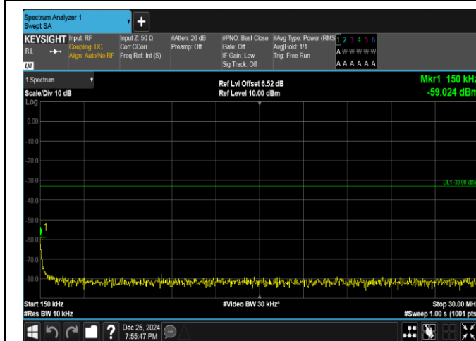
Band66-10MHz-QPSK-132622-1RB#49-0.15~30-PASS
