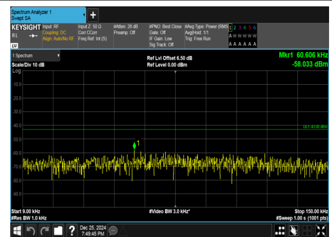
Band66-10MHz-16QAM-132322-1RB#49-0.009~0.15-PAS
