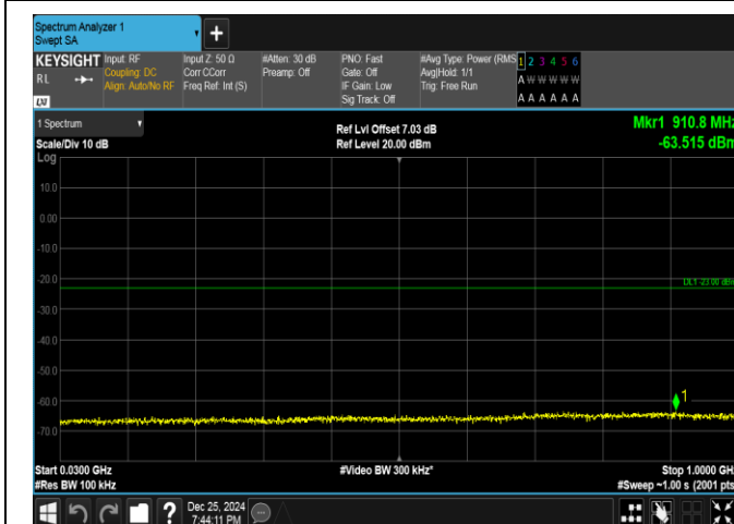
Band66-10MHz-QPSK-132022-50RB#0-30~1000-PASS
