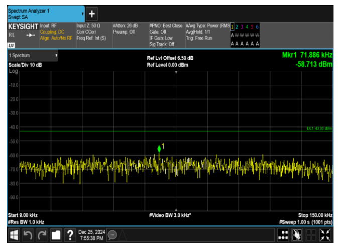
Band66-10MHz-QPSK-132622-1RB#49-0.009~0.15-PASS
