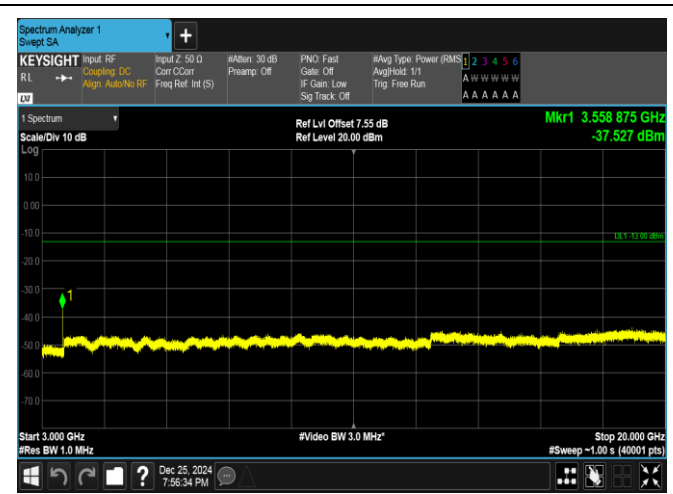
Band66-10MHz-QPSK-132622-1RB#49-3000~20000-PASS
