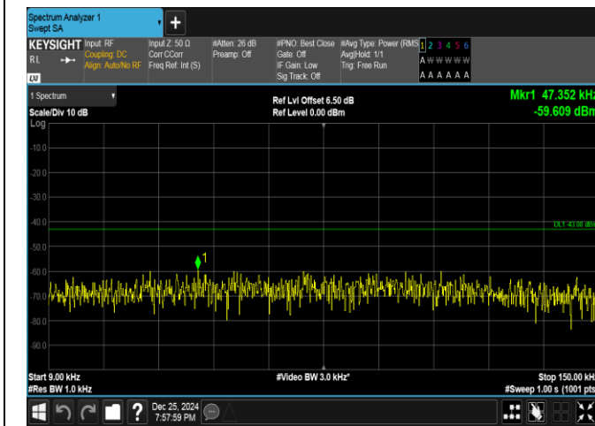
Band66-10MHz-QPSK-132622-50RB#0-0.009~0.15-PASS
