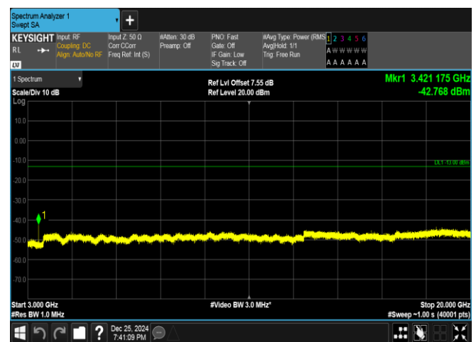
Band66-10MHz-16QAM-132022-1RB#0-3000~20000-PAS
