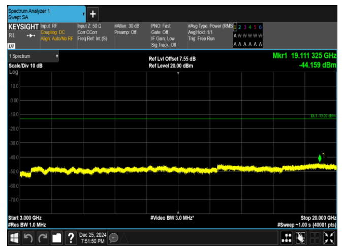
Band66-10MHz-QPSK-132322-50RB#0-3000~20000-PASS
