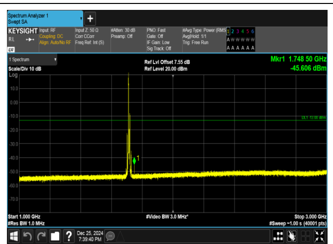
Band66-10MHz-QPSK-132022-1RB#0-1000~3000-PASS
