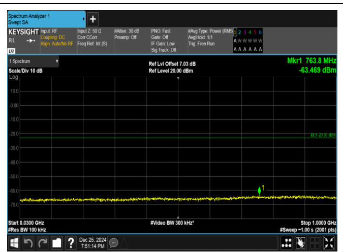
Band66-10MHz-QPSK-132322-50RB#0-30~1000-PASS
