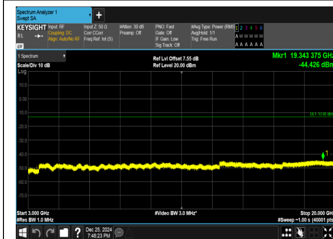
Band66-10MHz-16QAM-132322-1RB#0-3000~20000-PAS
