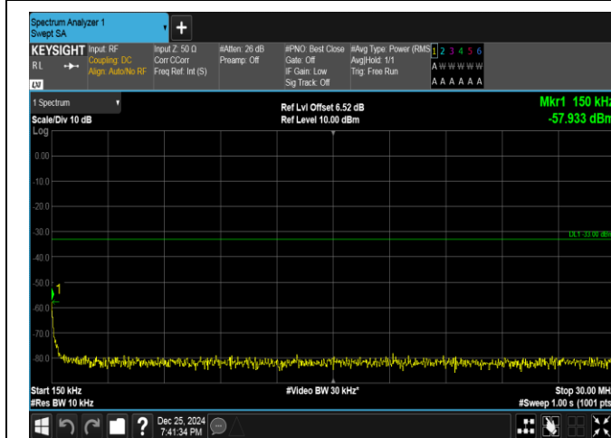
Band66-10MHz-QPSK-132022-1RB#49-0.15~30-PASS
