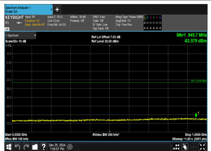
Band66-10MHz-QPSK-132622-1RB#49-30~1000-PASS
