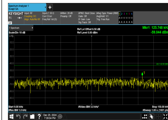
Band66-10MHz-QPSK-132022-1RB#0-0.009~0.15-PASS
