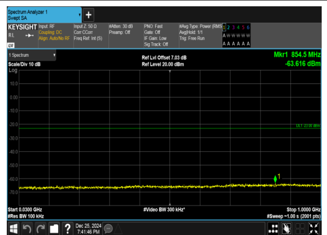
Band66-10MHz-QPSK-132022-1RB#49-30~1000-PASS
