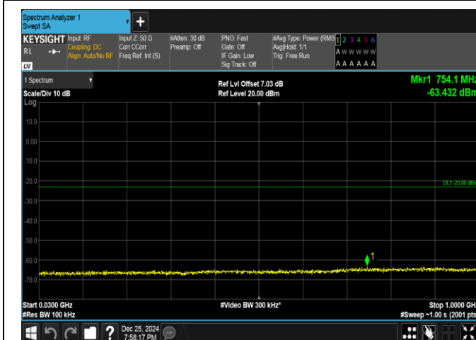
Band66-10MHz-QPSK-132622-50RB#0-30~1000-PASS
