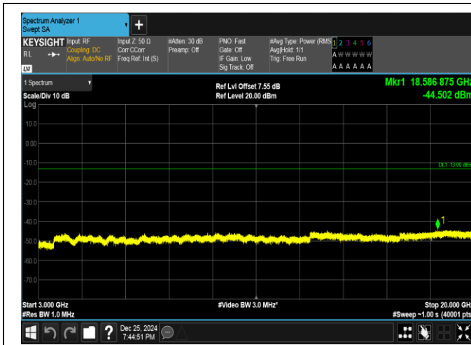
Band66-10MHz-QPSK-132022-50RB#0-3000~20000-PASS
