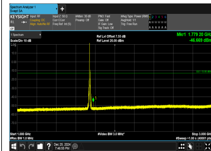
Band66-10MHz-QPSK-132322-1RB#0-1000~3000-PASS
