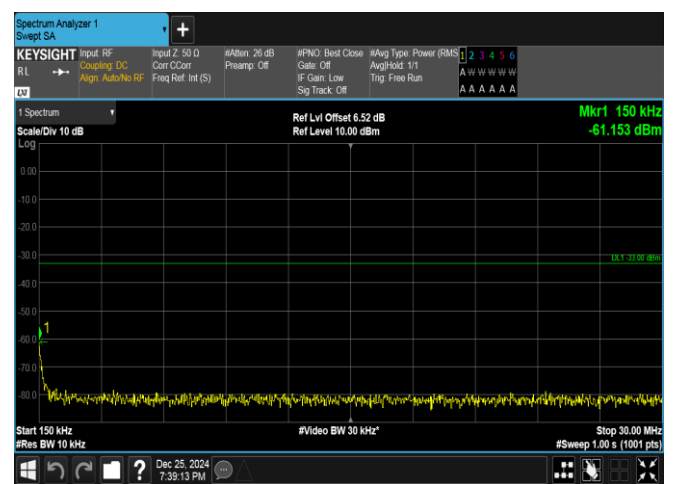
Band66-10MHz-QPSK-132022-1RB#0-0.15~30-PASS
