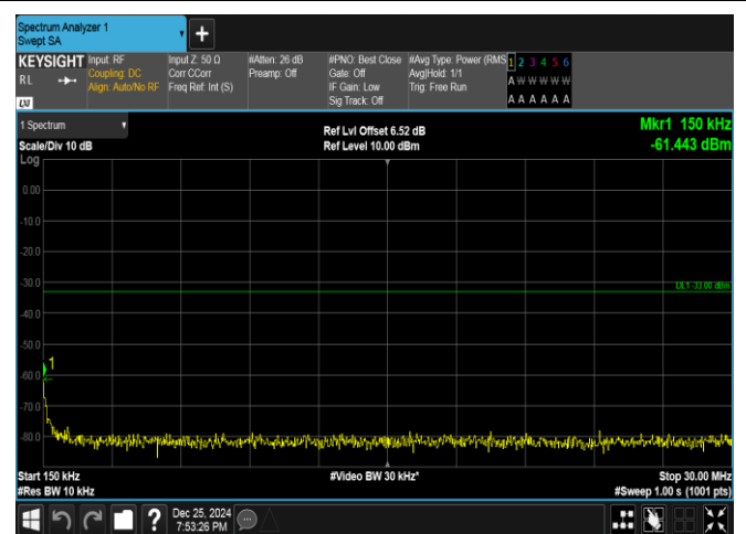
Band66-10MHz-QPSK-132622-1RB#0-0.15~30-PASS
