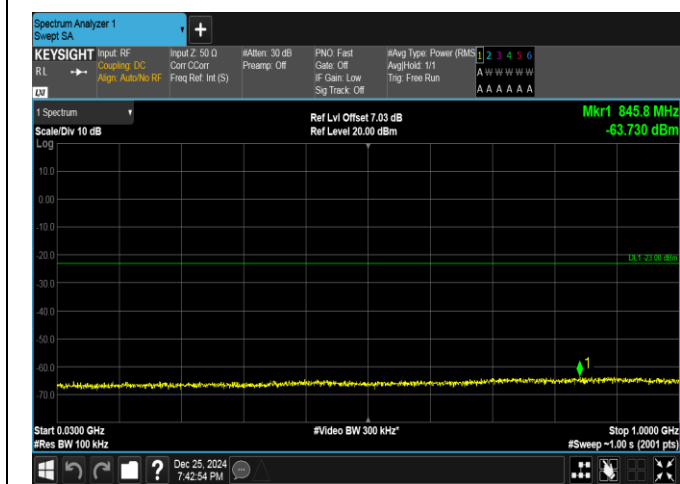
Band66-10MHz-16QAM-132022-1RB#49-30~1000-PASS
