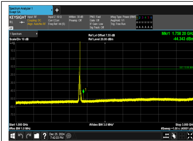
Band66-10MHz-QPSK-132022-1RB#49-1000~3000-PASS
