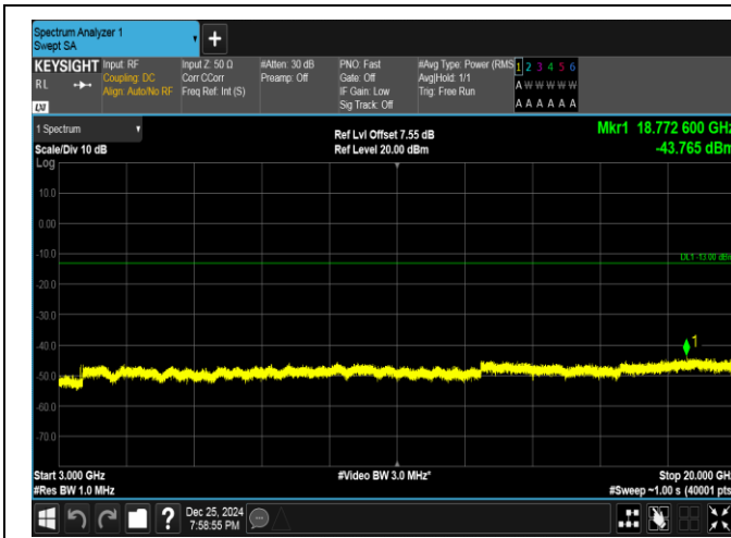
Band66-10MHz-QPSK-132622-50RB#0-3000~20000-PASS
