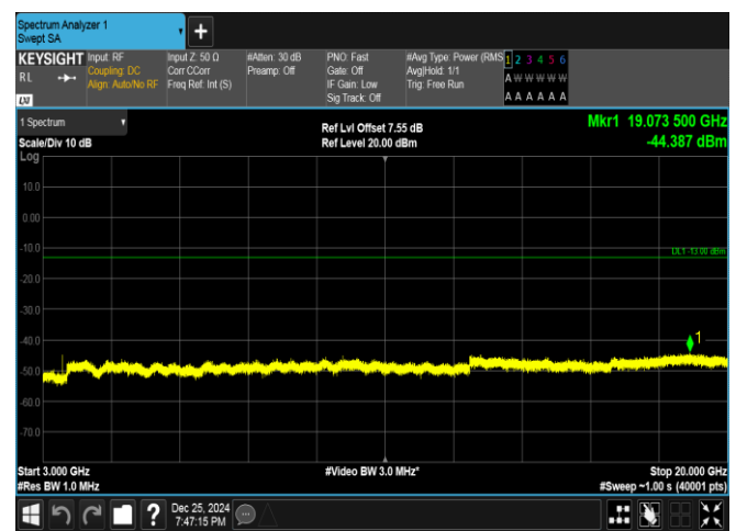
Band66-10MHz-QPSK-132322-1RB#0-3000~20000-PASS
