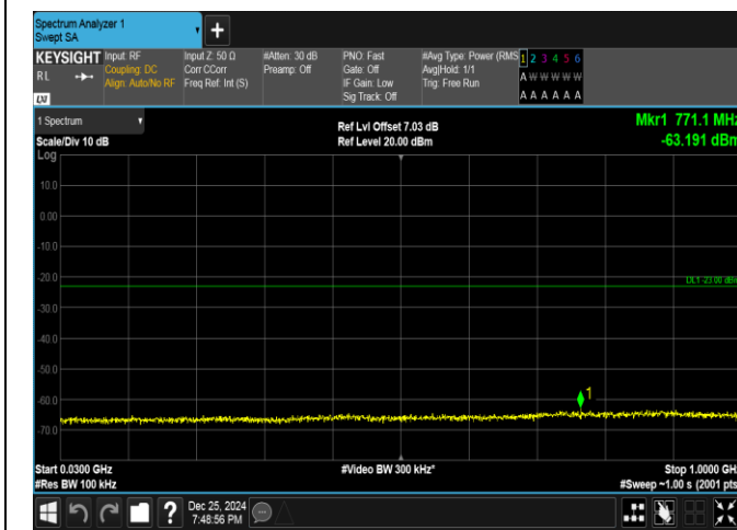
Band66-10MHz-QPSK-132322-1RB#49-30~1000-PASS
