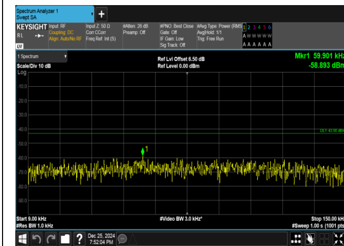
Band66-10MHz-16QAM-132322-50RB#0-0.009~0.15-PAS
