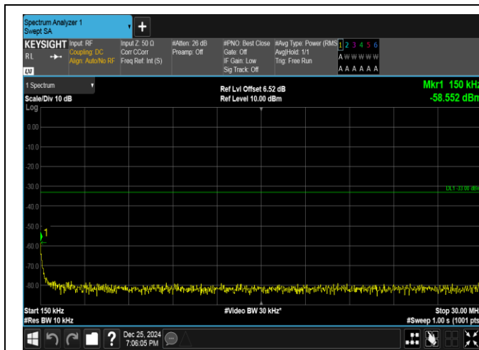
Band66-5MHz-16QAM-132647-25RB#0-0.15~30-PASS
