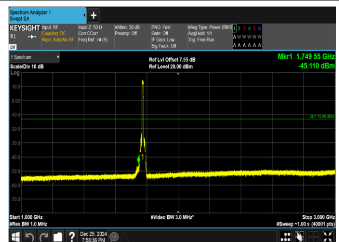
Band66-10MHz-QPSK-132622-50RB#0-1000~3000-PASS
