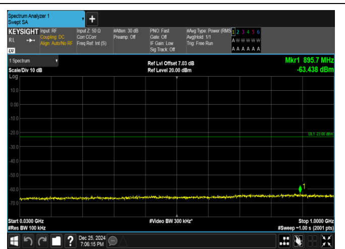
Band66-5MHz-16QAM-132647-25RB#0-30~1000-PASS
