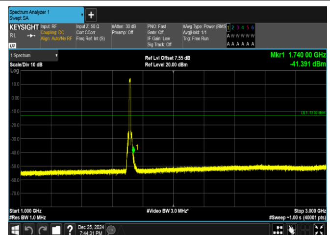
Band66-10MHz-QPSK-132022-50RB#0-1000~3000-PASS
