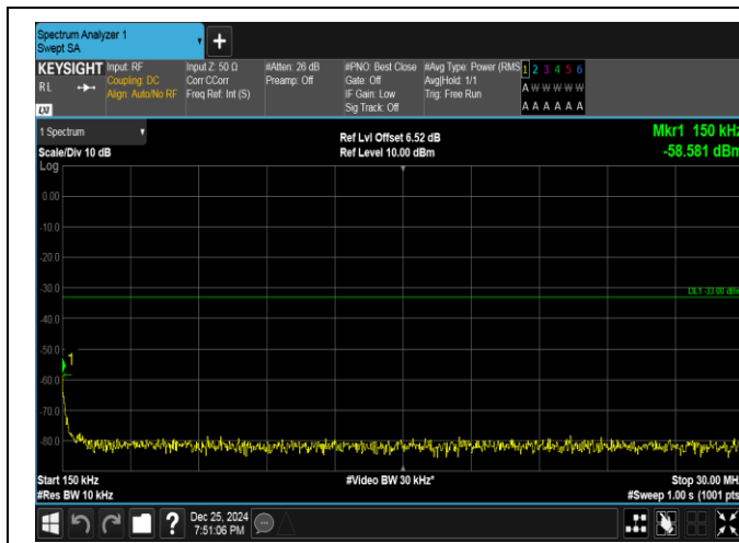
Band66-10MHz-QPSK-132322-50RB#0-0.15~30-PASS
