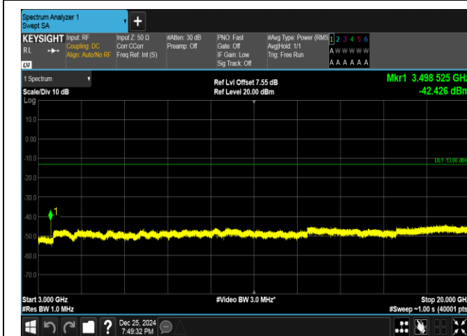
Band66-10MHz-QPSK-132322-1RB#49-3000~20000-PASS
