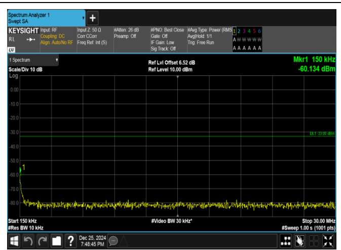
Band66-10MHz-QPSK-132322-1RB#49-0.15~30-PASS
