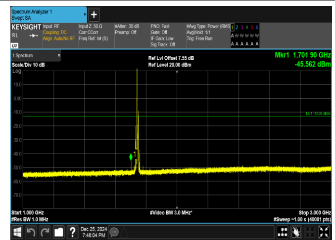
Band66-10MHz-16QAM-132322-1RB#0-1000~3000-PASS
