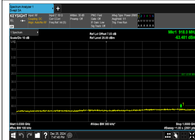
Band66-10MHz-16QAM-132322-1RB#0-30~1000-PASS
