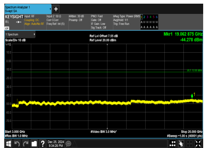
Band66-20MHz-QPSK-132322-1RB#0-3000~20000-PASS
