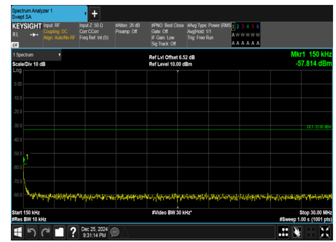
Band66-20MHz-QPSK-132072-100RB#0-0.15~30-PASS
