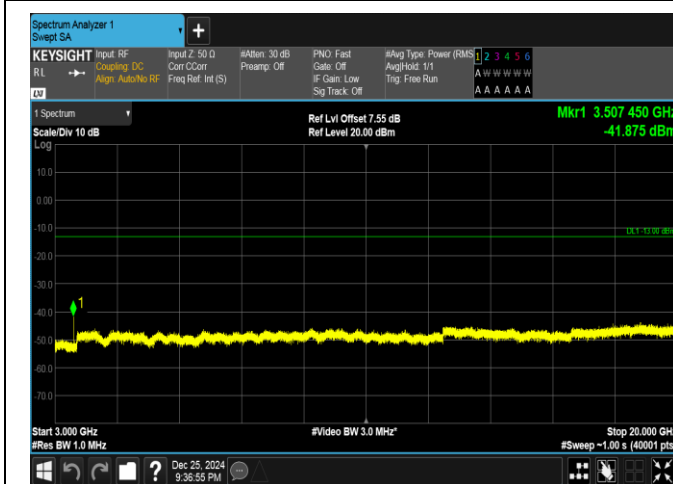
Band66-20MHz-QPSK-132322-1RB#99-3000~20000-PASS
