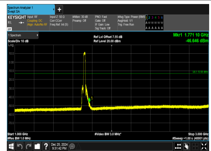
Band66-20MHz-QPSK-132072-100RB#0-1000~3000-PASS
