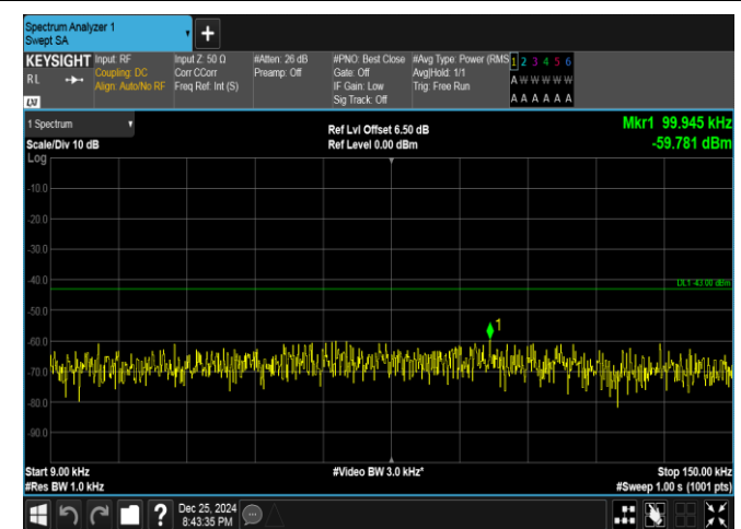
Band66-15MHz-16QAM-132322-1RB#74-0.009~0.15-PAS
