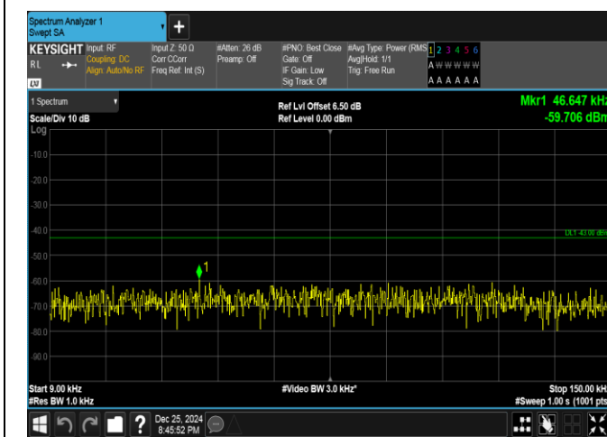
Band66-15MHz-16QAM-132322-75RB#0-0.009~0.15-PAS
