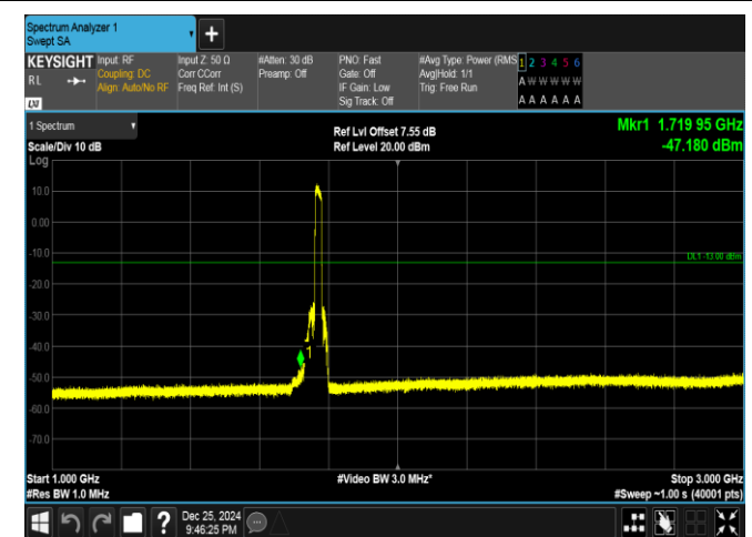
Band66-20MHz-QPSK-132572-100RB#0-1000~3000-PASS
