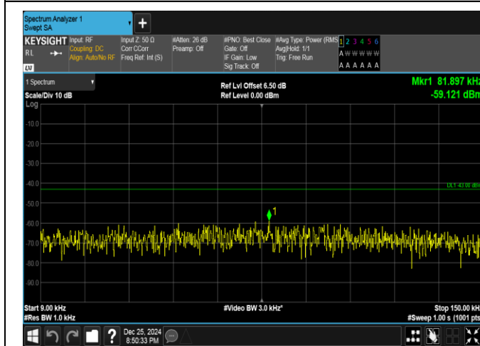
Band66-15MHz-16QAM-132597-1RB#74-0.009~0.15-PAS
