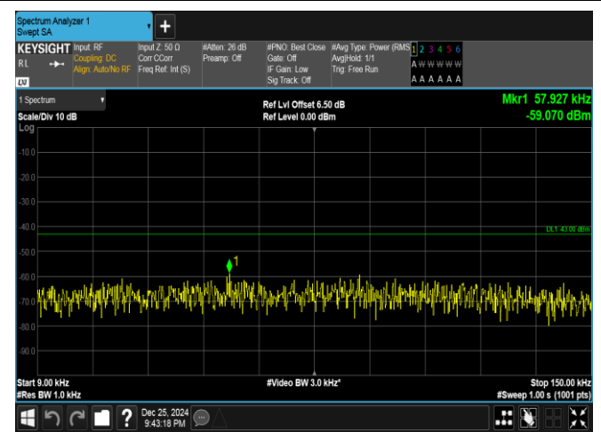
Band66-20MHz-QPSK-132572-1RB#99-0.009~0.15-PASS
