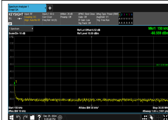
Band66-20MHz-QPSK-132072-1RB#99-0.15~30-PASS
