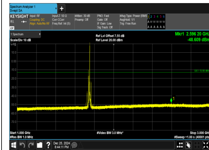
Band66-15MHz-16QAM-132322-1RB#74-1000~3000-PAS
