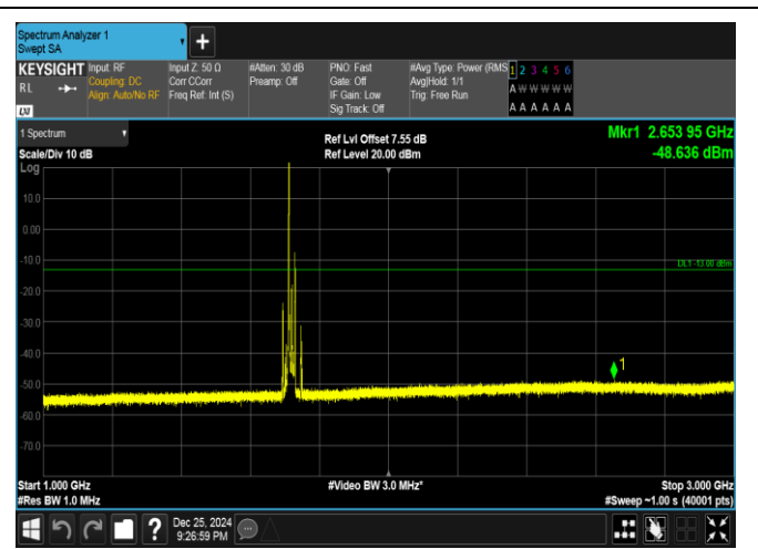
Band66-20MHz-QPSK-132072-1RB#0-1000~3000-PASS
