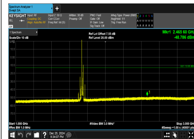
Band66-20MHz-QPSK-132322-1RB#0-1000~3000-PASS
