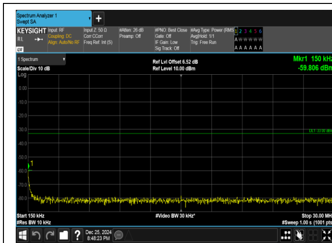
Band66-15MHz-16QAM-132597-1RB#0-0.15~30-PASS
