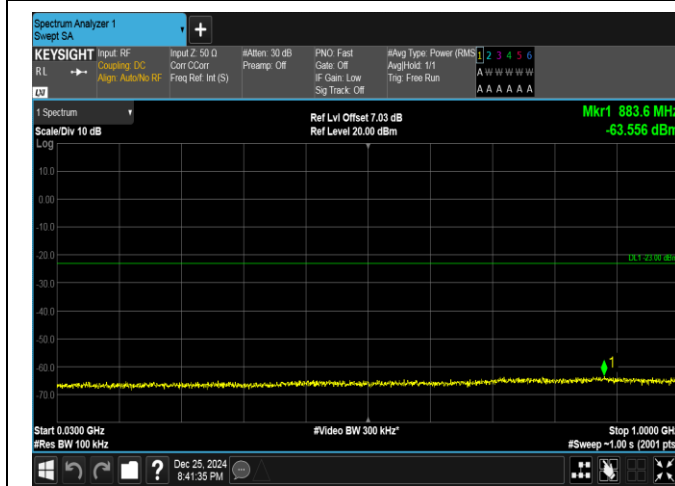
Band66-15MHz-16QAM-132322-1RB#0-30~1000-PASS
