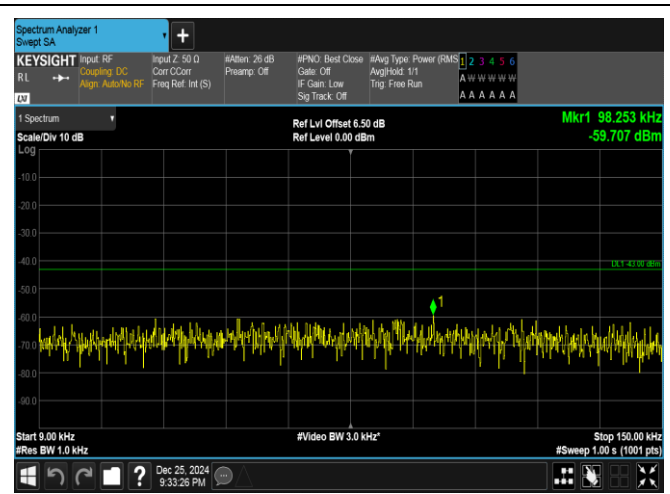
Band66-20MHz-QPSK-132322-1RB#0-0.009~0.15-PASS
