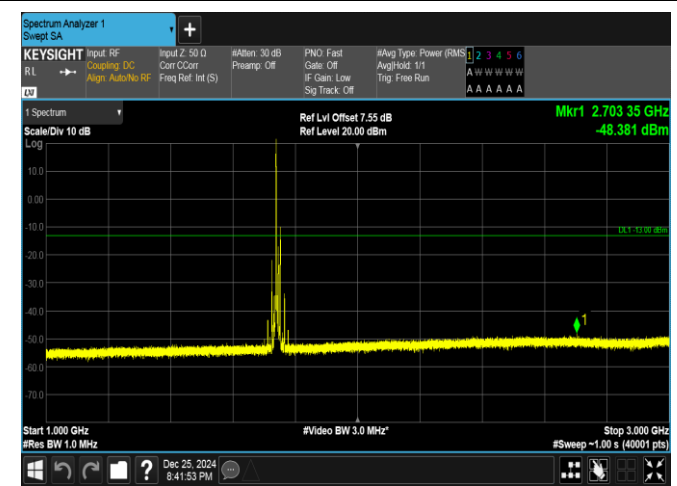
Band66-15MHz-16QAM-132322-1RB#0-1000~3000-PASS
