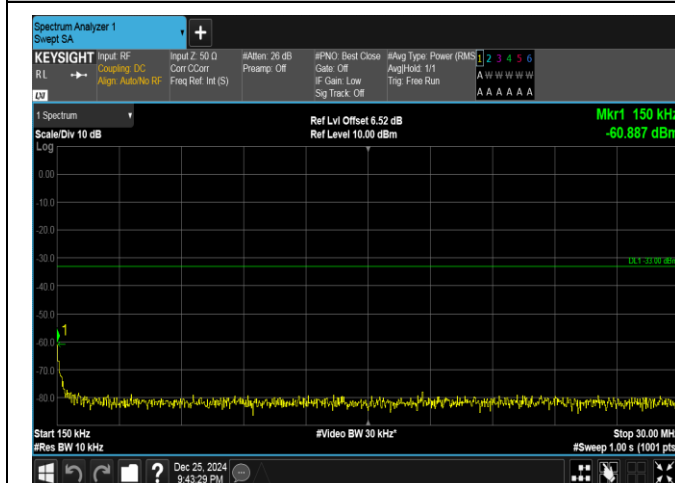
Band66-20MHz-QPSK-132572-1RB#99-0.15~30-PASS
