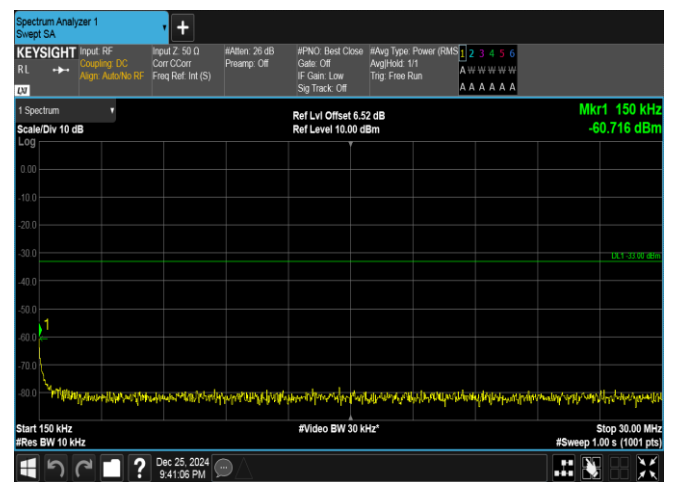
Band66-20MHz-QPSK-132572-1RB#0-0.15~30-PASS
