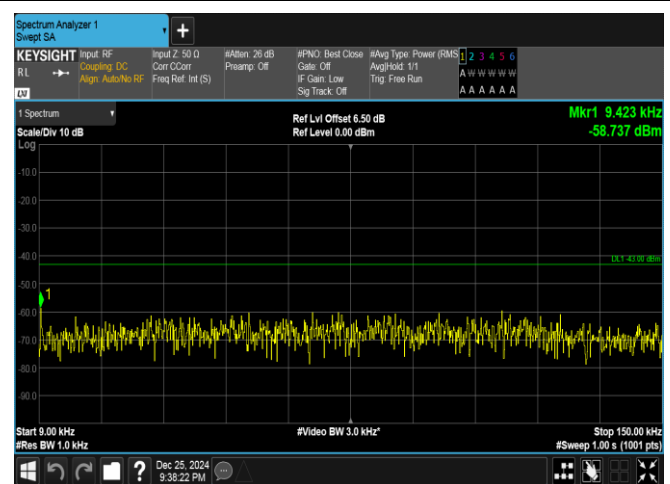
Band66-20MHz-QPSK-132322-100RB#0-0.009~0.15-PASS
