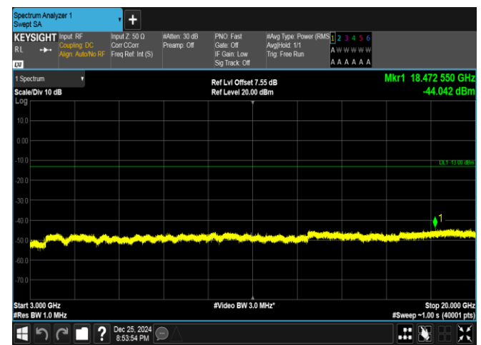
Band66-15MHz-16QAM-132597-75RB#0-3000~20000-PA
