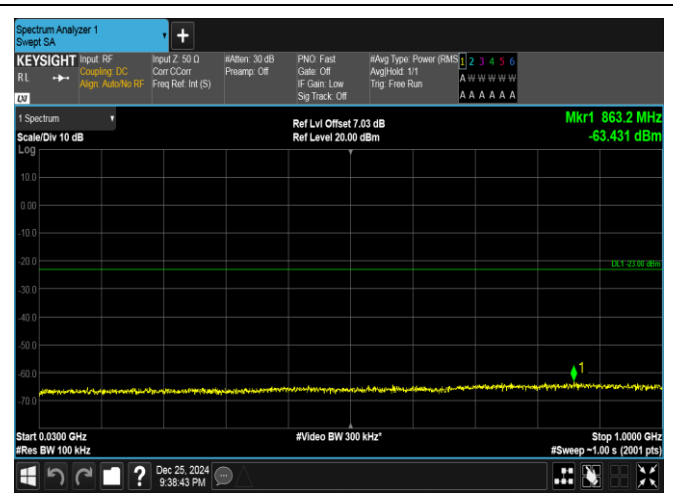
Band66-20MHz-QPSK-132322-100RB#0-30~1000-PASS
