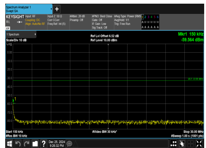
Band66-20MHz-QPSK-132072-1RB#0-0.15~30-PASS
