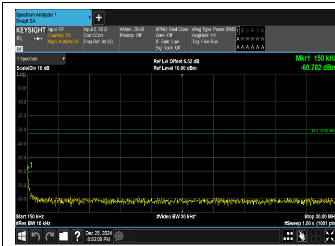
Band66-15MHz-16QAM-132597-75RB#0-0.15~30-PASS
