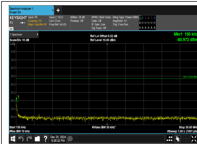
Band66-20MHz-QPSK-132322-100RB#0-0.15~30-PASS
