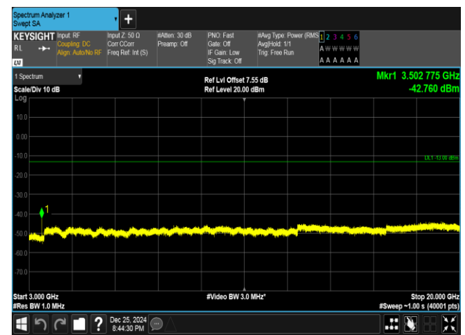
Band66-15MHz-16QAM-132322-1RB#74-3000~20000-PA
