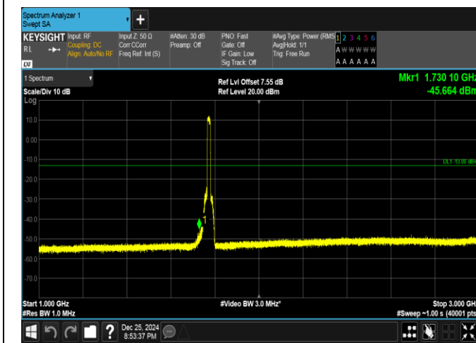
Band66-15MHz-16QAM-132597-75RB#0-1000~3000-PAS
