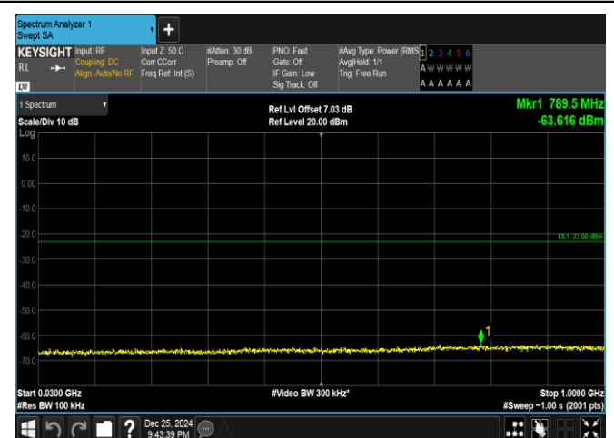
Band66-20MHz-QPSK-132572-1RB#99-30~1000-PASS
