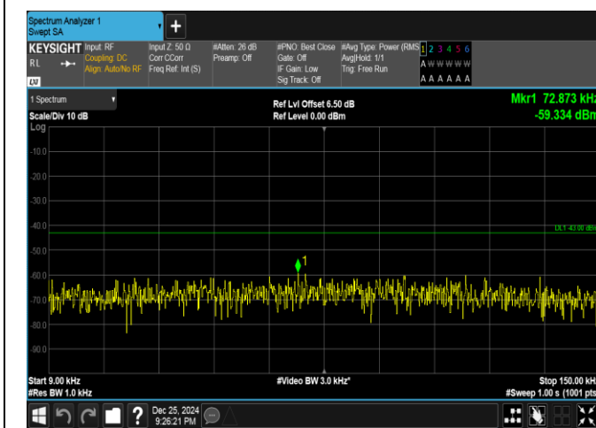
Band66-20MHz-QPSK-132072-1RB#0-0.009~0.15-PASS
