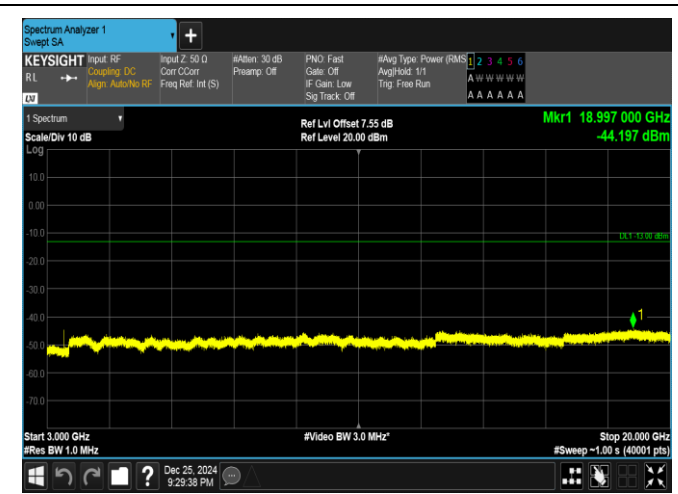
Band66-20MHz-QPSK-132072-1RB#99-3000~20000-PASS
