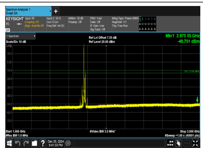
Band66-20MHz-QPSK-132572-1RB#0-1000~3000-PASS
