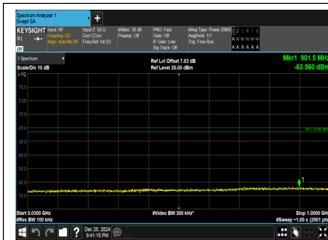
Band66-20MHz-QPSK-132572-1RB#0-30~1000-PASS
