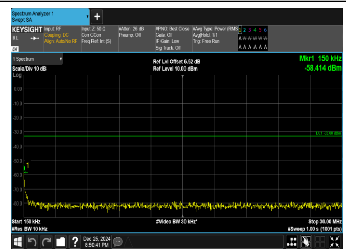
Band66-15MHz-16QAM-132597-1RB#74-0.15~30-PASS
