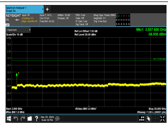
Band66-20MHz-QPSK-132572-1RB#99-3000~20000-PASS
