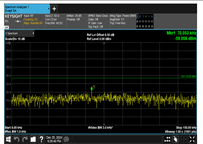
Band66-20MHz-QPSK-132072-1RB#99-0.009~0.15-PASS
