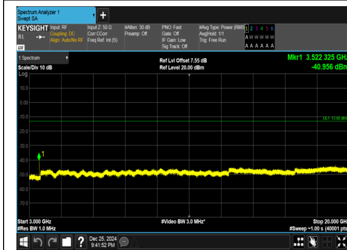
Band66-20MHz-QPSK-132572-1RB#0-3000~20000-PASS
