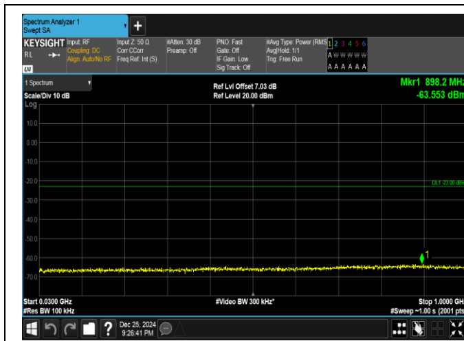
Band66-20MHz-QPSK-132072-1RB#0-30~1000-PASS
