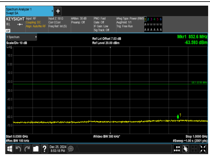
Band66-15MHz-16QAM-132597-75RB#0-30~1000-PASS
