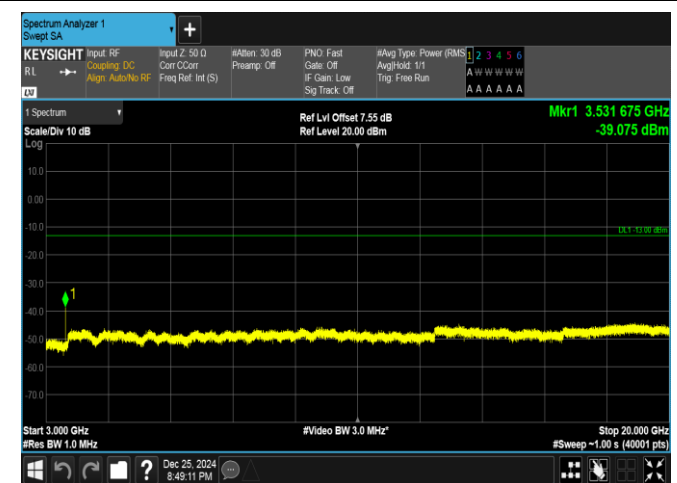
Band66-15MHz-16QAM-132597-1RB#0-3000~20000-PAS S
