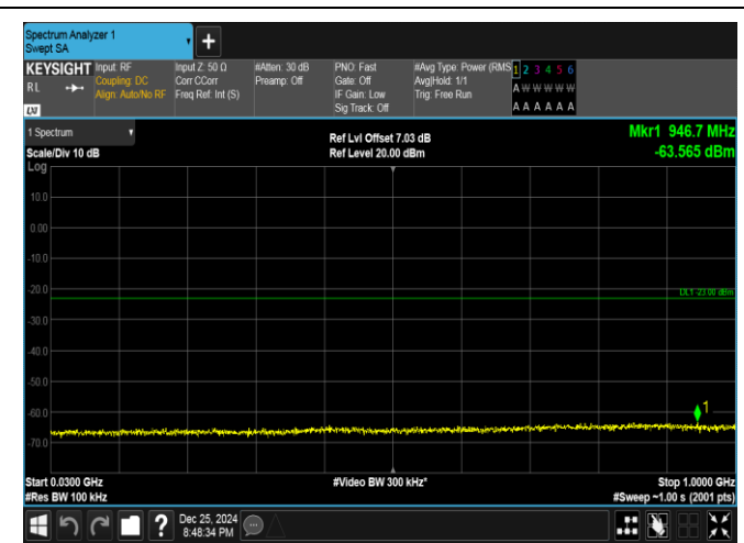
Band66-15MHz-16QAM-132597-1RB#0-30~1000-PASS
