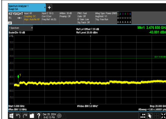
Band66-15MHz-16QAM-132322-1RB#0-3000~20000-PAS
