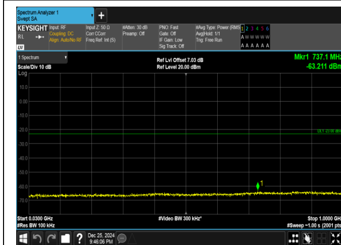
Band66-20MHz-QPSK-132572-100RB#0-30~1000-PASS
