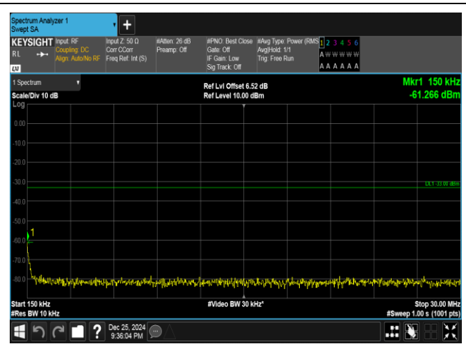
Band66-20MHz-QPSK-132322-1RB#99-0.15~30-PASS
