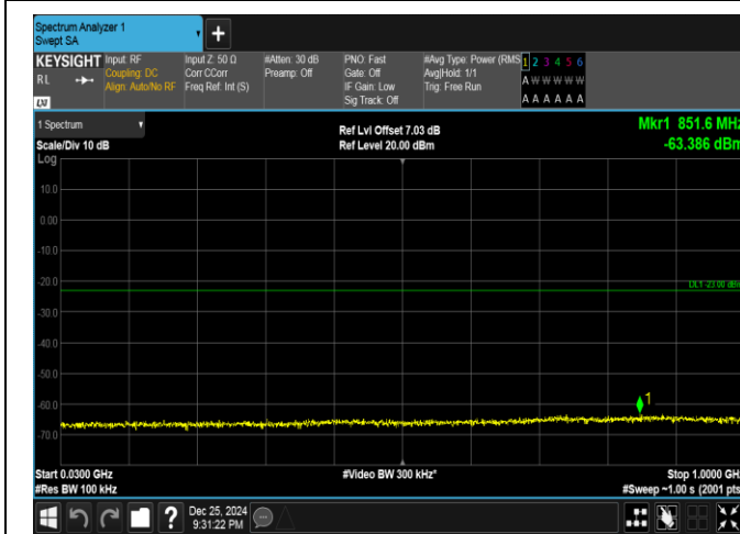
Band66-20MHz-QPSK-132072-100RB#0-30~1000-PASS
