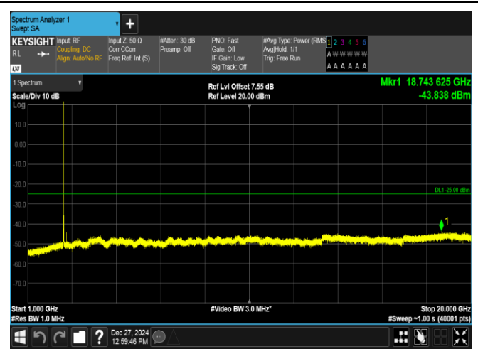
Band7-5MHz-16QAM-21100-1RB#0-1000~20000-PASS
