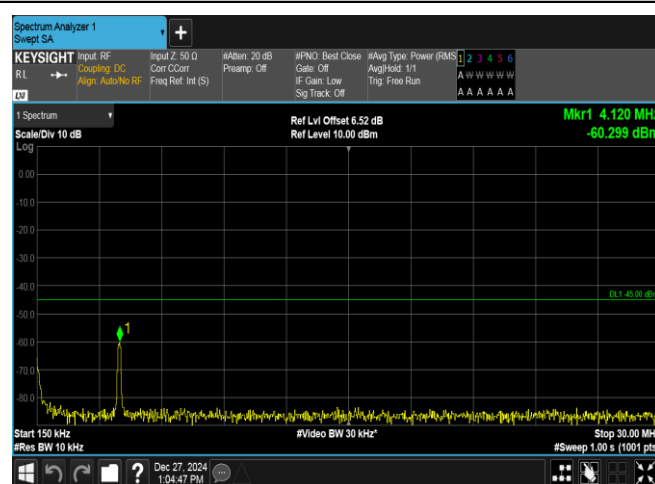
Band7-5MHz-QPSK-21425-1RB#0-0.15~30-PASS
