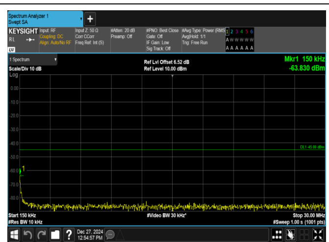
Band7-5MHz-16QAM-20775-1RB#24-0.15~30-PASS
