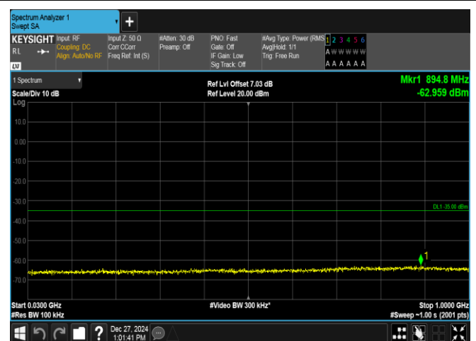
Band7-5MHz-16QAM-21100-1RB#24-30~1000-PASS
