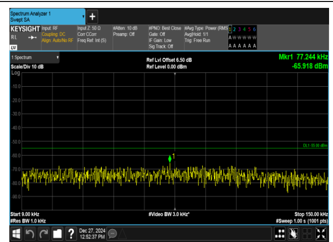
Band7-5MHz-16QAM-20775-1RB#0-0.009~0.15-PASS
