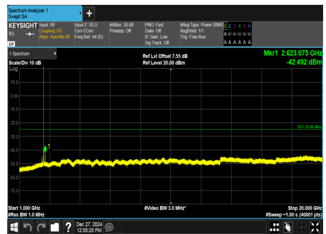
Band7-5MHz-16QAM-20775-1RB#24-1000~20000-PASS
