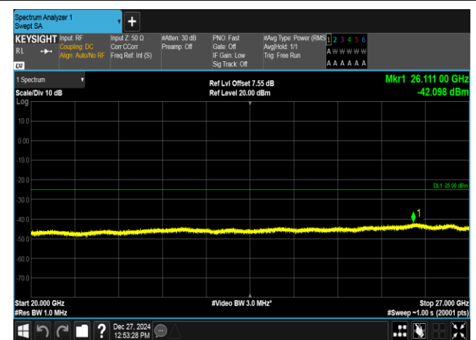
Band7-5MHz-16QAM-20775-1RB#0-20000~27000-PASS
