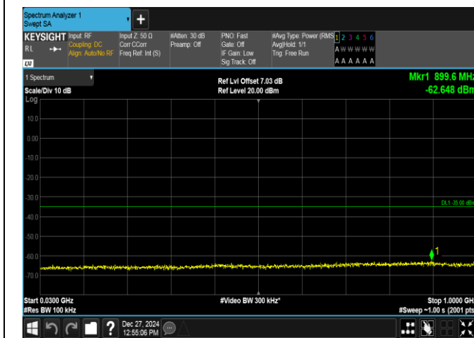
Band7-5MHz-16QAM-20775-1RB#24-30~1000-PASS
