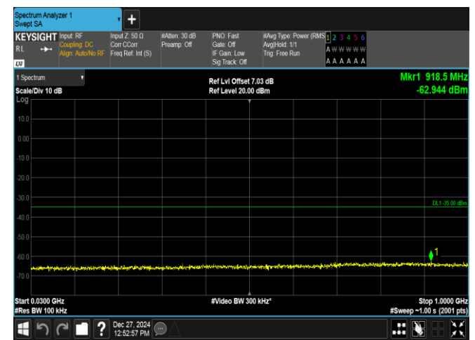
Band7-5MHz-16QAM-20775-1RB#0-30~1000-PASS
