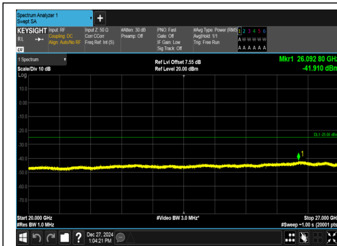
Band7-5MHz-16QAM-21100-25RB#0-20000~27000-PASS
