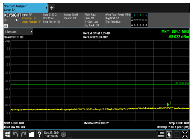
Band7-5MHz-16QAM-21425-1RB#0-30~1000-PASS
