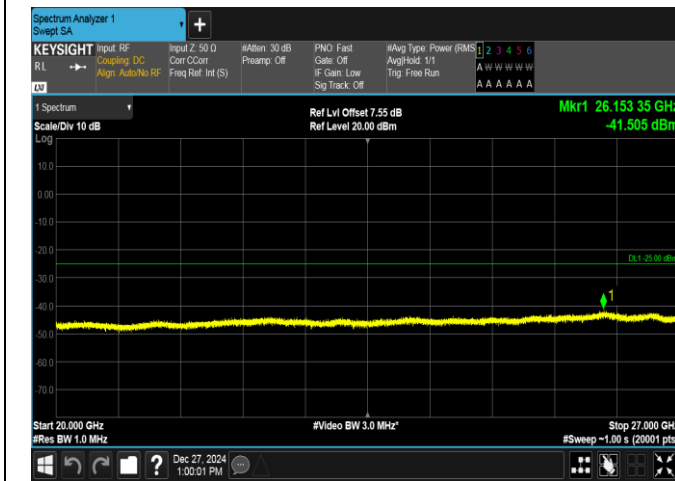
Band7-5MHz-16QAM-21100-1RB#0-20000~27000-PASS
