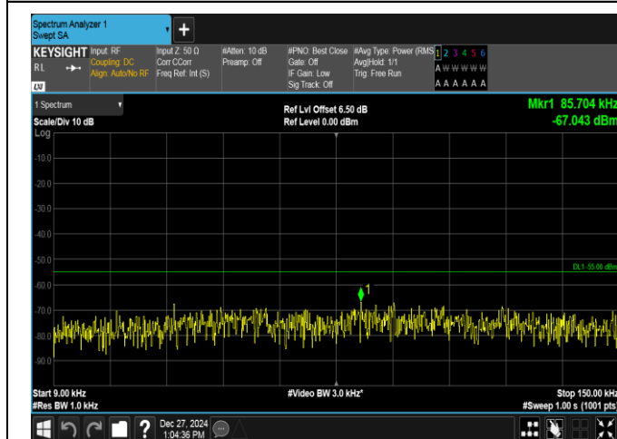
Band7-5MHz-QPSK-21425-1RB#0-0.009~0.15-PASS
