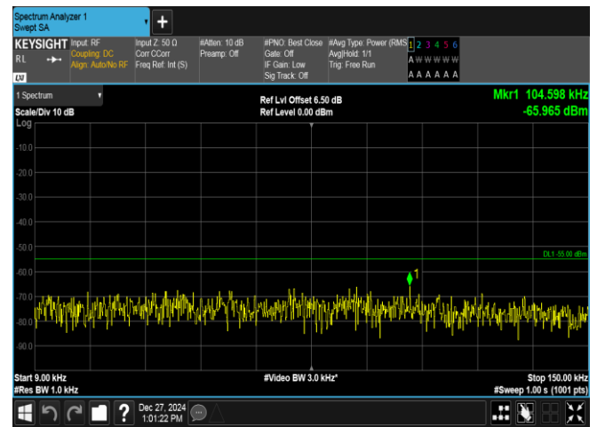
Band7-5MHz-16QAM-21100-1RB#24-0.009~0.15-PASS
