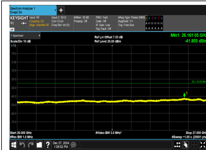
Band7-5MHz-QPSK-21425-25RB#0-20000~27000-PASS
