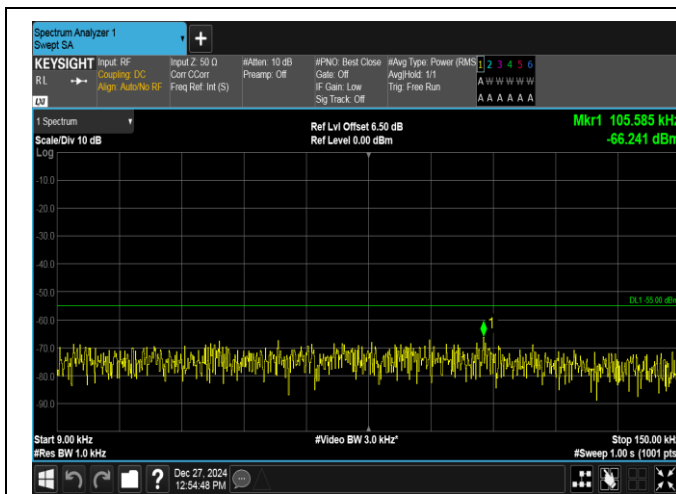
Band7-5MHz-16QAM-20775-1RB#24-0.009~0.15-PASS
