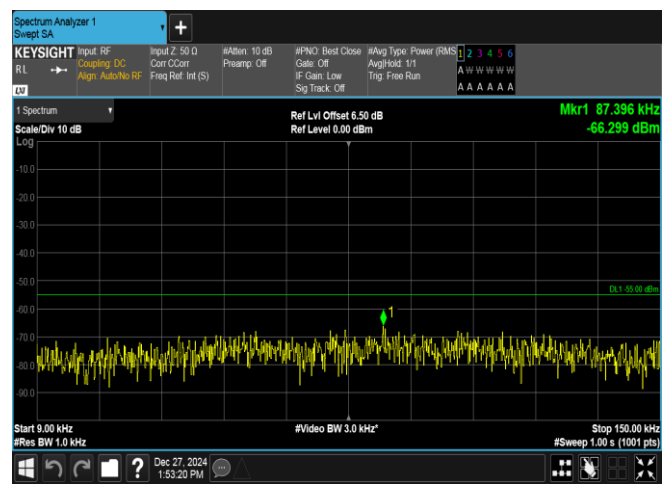
Band7-20MHz-QPSK-20850-1RB#99-0.009~0.15-PASS
