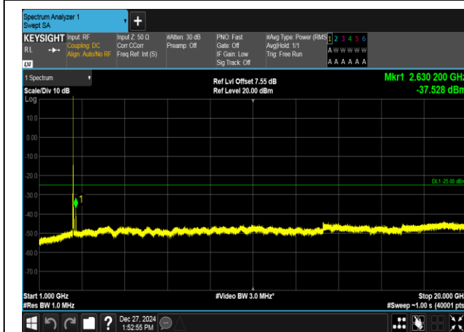
Band7-20MHz-16QAM-20850-1RB#0-1000~20000-PASS
