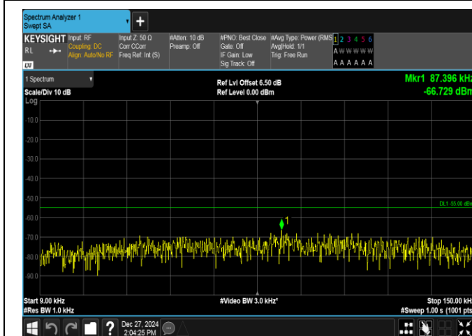
Band7-20MHz-QPSK-21350-1RB#0-0.009~0.15-PASS
