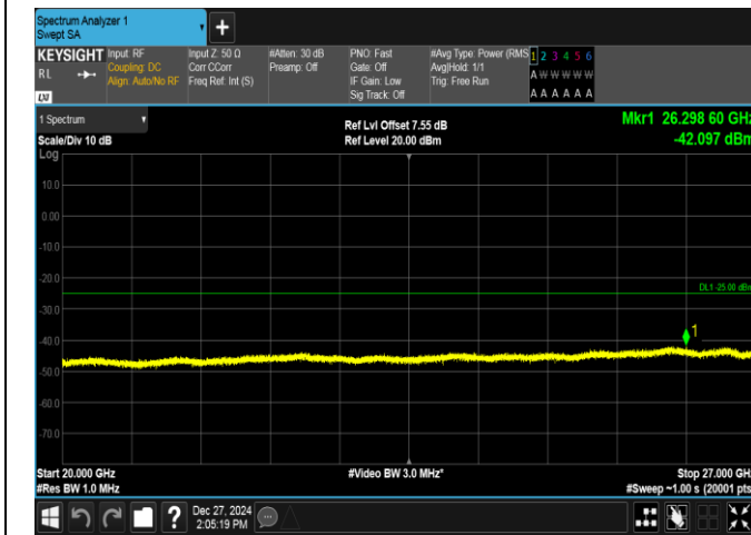
Band7-20MHz-QPSK-21350-1RB#0-20000~27000-PASS
