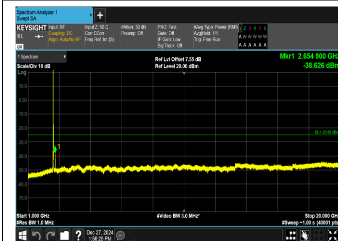
Band7-20MHz-QPSK-21100-1RB#0-1000~20000-PASS
