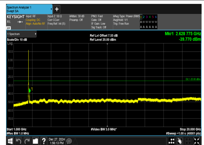
Band7-20MHz-QPSK-20850-100RB#0-1000~20000-PASS
