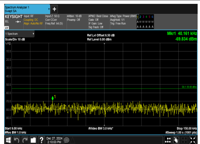
Band7-20MHz-16QAM-21350-100RB#0-0.009~0.15-PASS
