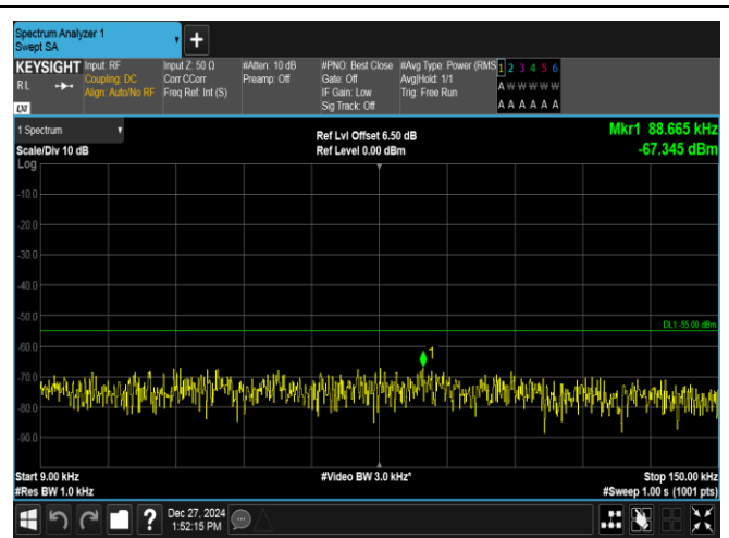
Band7-20MHz-16QAM-20850-1RB#0-0.009~0.15-PASS
