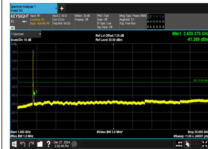
Band7-20MHz-QPSK-21100-100RB#0-1000~20000-PASS
