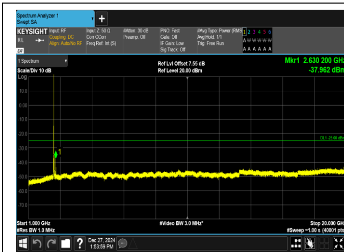
Band7-20MHz-QPSK-20850-1RB#99-1000~20000-PASS
