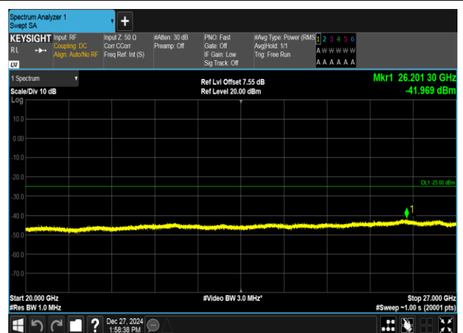
Band7-20MHz-QPSK-21100-1RB#0-20000~27000-PASS
