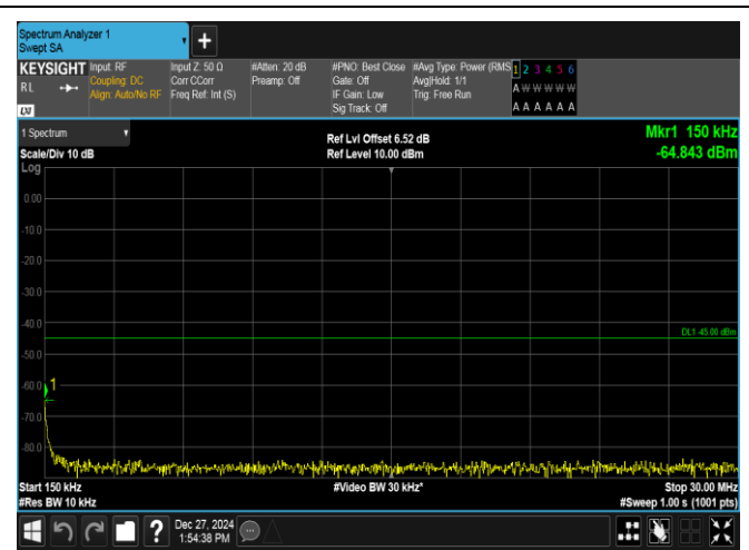
Band7-20MHz-16QAM-20850-1RB#99-0.15~30-PASS
