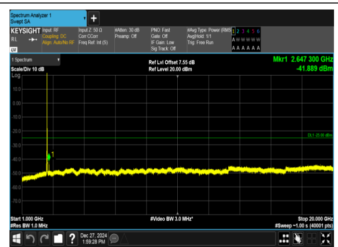
Band7-20MHz-16QAM-21100-1RB#0-1000~20000-PASS
