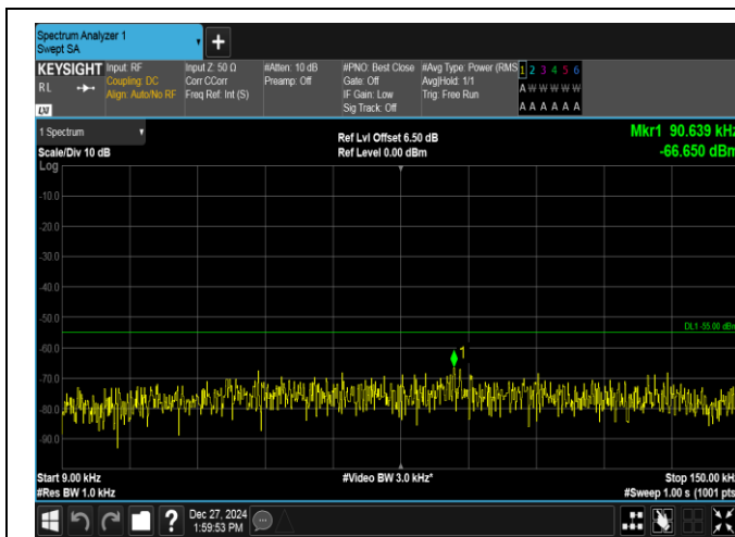
Band7-20MHz-QPSK-21100-1RB#99-0.009~0.15-PASS
