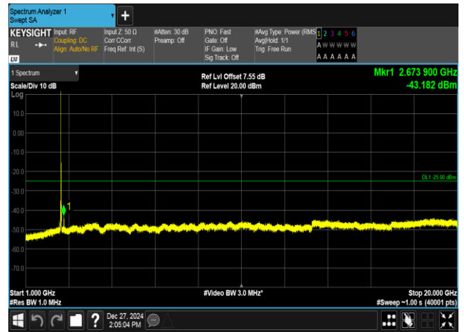
Band7-20MHz-QPSK-21350-1RB#0-1000~20000-PASS
