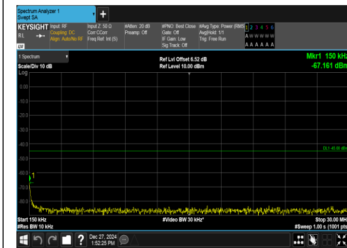
Band7-20MHz-16QAM-20850-1RB#0-0.15~30-PASS
