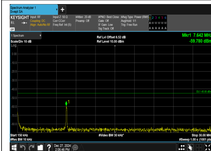
Band7-20MHz-QPSK-21350-1RB#99-0.15~30-PASS
