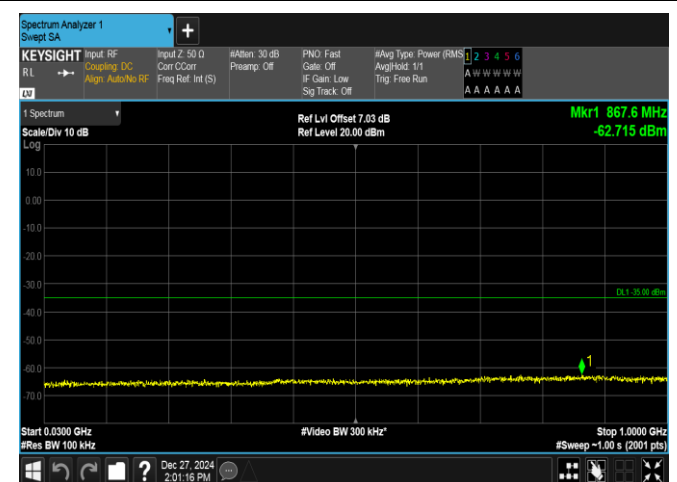
Band7-20MHz-16QAM-21100-1RB#99-30~1000-PASS
