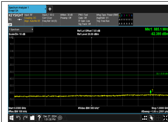
Band7-20MHz-QPSK-20850-1RB#0-30~1000-PASS
