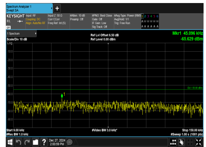
Band7-20MHz-16QAM-21100-1RB#99-0.009~0.15-PASS
