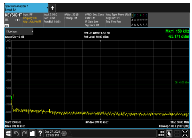
Band7-20MHz-QPSK-21350-100RB#0-0.15~30-PASS
