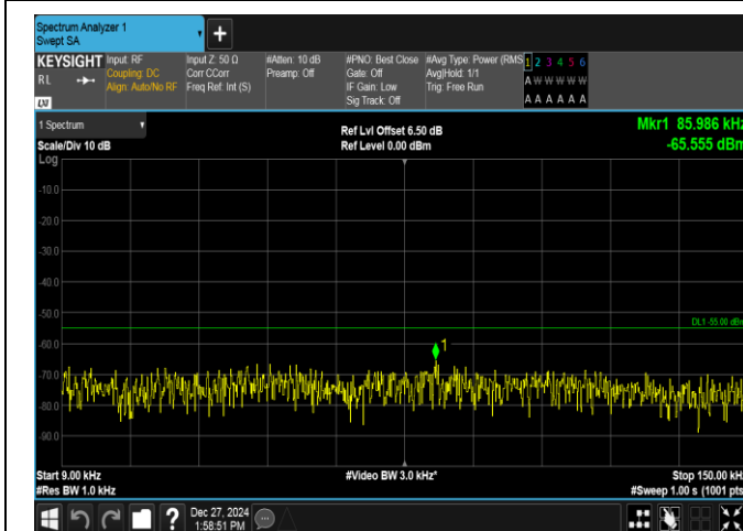
Band7-20MHz-16QAM-21100-1RB#0-0.009~0.15-PASS
