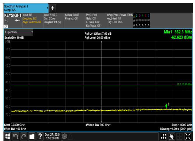
Band7-20MHz-16QAM-20850-1RB#0-30~1000-PASS
