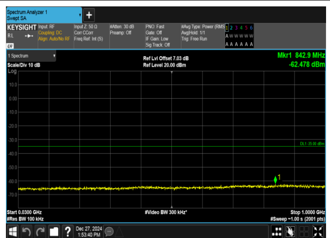
Band7-20MHz-QPSK-20850-1RB#99-30~1000-PASS
