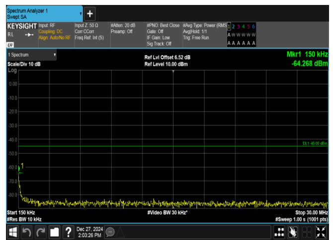
Band7-20MHz-16QAM-21100-100RB#0-0.15~30-PASS
