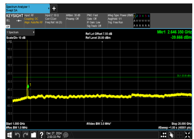
Band7-20MHz-QPSK-21100-1RB#99-1000~20000-PASS
