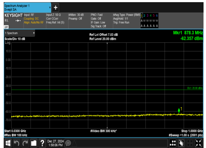
Band7-20MHz-QPSK-21100-1RB#0-30~1000-PASS
