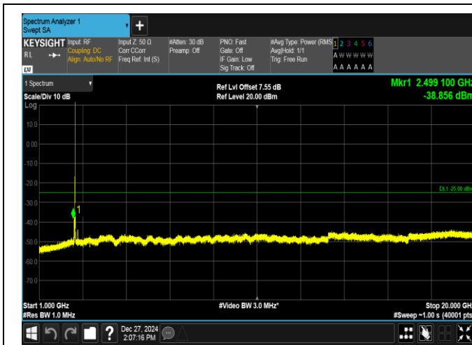
Band7-20MHz-QPSK-21350-1RB#99-1000~20000-PASS
