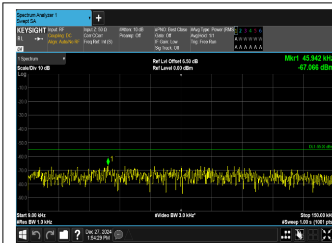
Band7-20MHz-16QAM-20850-1RB#99-0.009~0.15-PASS
