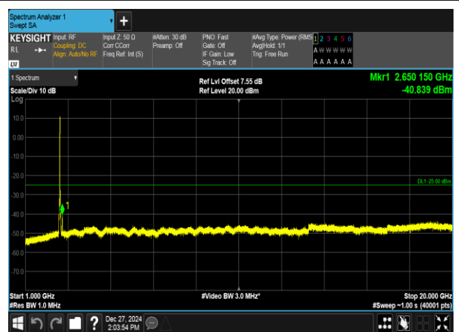
Band7-20MHz-16QAM-21100-100RB#0-1000~20000-PASS
