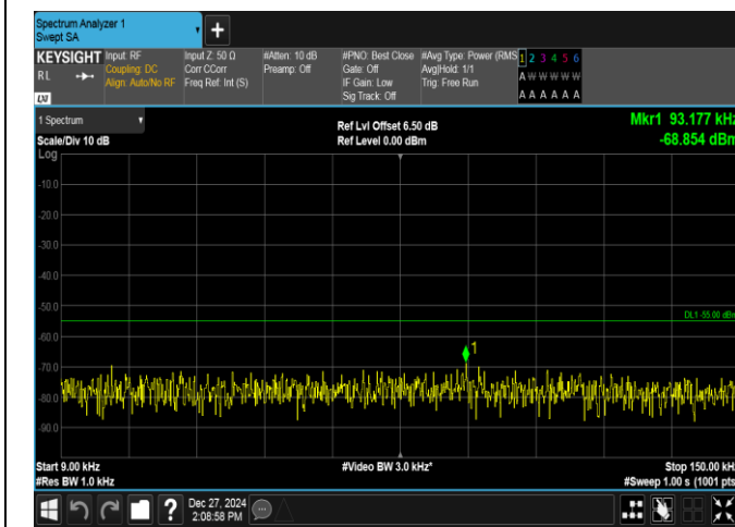
Band7-20MHz-QPSK-21350-100RB#0-0.009~0.15-PASS
