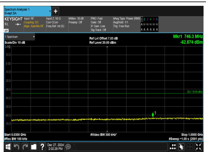
Band7-20MHz-QPSK-21100-100RB#0-30~1000-PASS
