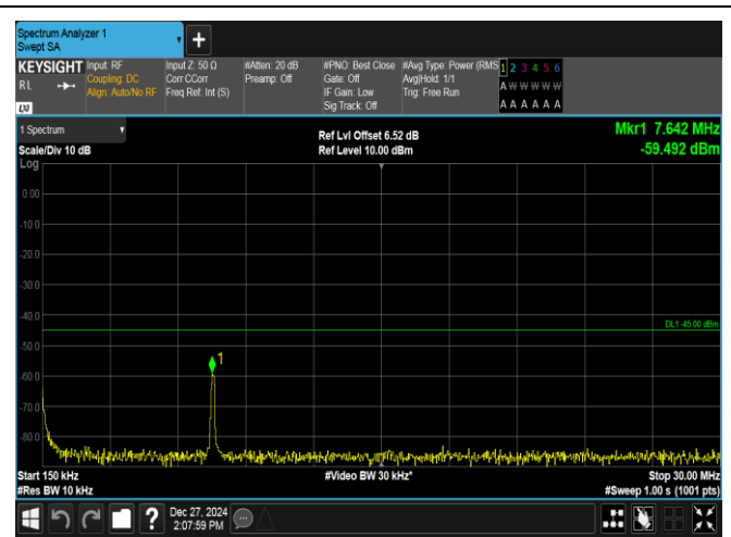
Band7-20MHz-16QAM-21350-1RB#99-0.15~30-PASS
