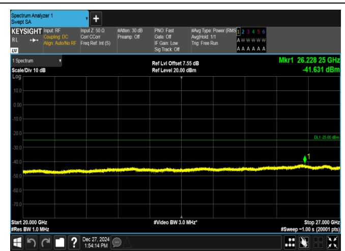
Band7-20MHz-QPSK-20850-1RB#99-20000~27000-PASS
