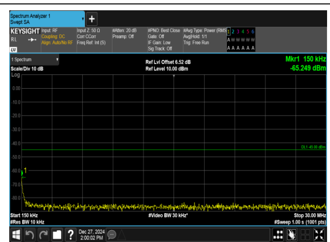
Band7-20MHz-QPSK-21100-1RB#99-0.15~30-PASS
