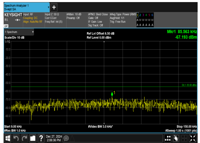
Band7-20MHz-QPSK-21350-1RB#99-0.009~0.15-PASS
