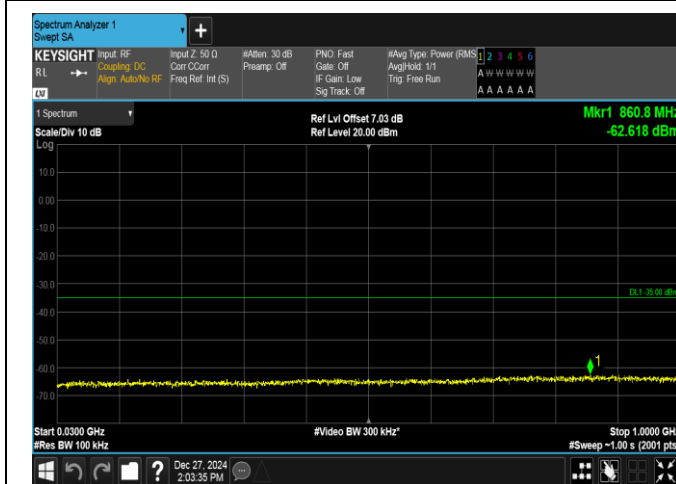
Band7-20MHz-16QAM-21100-100RB#0-30~1000-PASS
