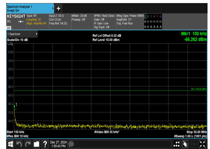
Band7-20MHz-QPSK-20850-100RB#0-0.15~30-PASS
