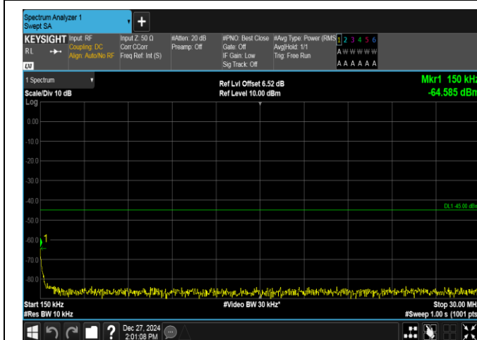
Band7-20MHz-16QAM-21100-1RB#99-0.15~30-PASS
