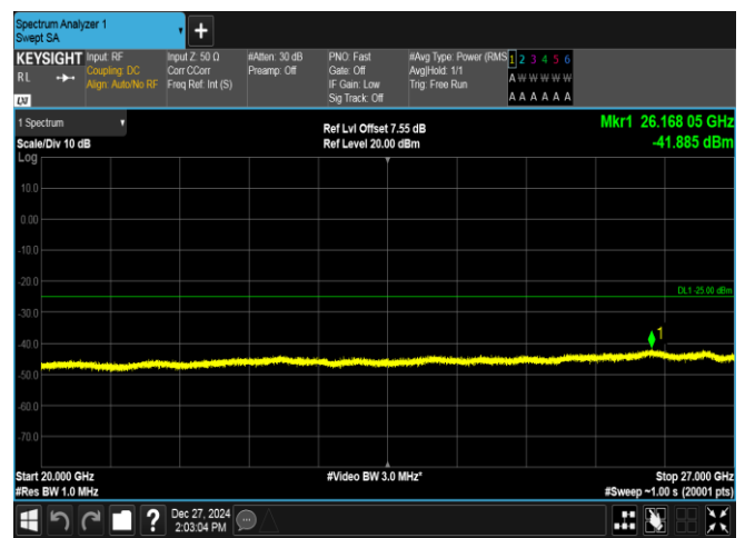
Band7-20MHz-QPSK-21100-100RB#0-20000~27000-PASS
