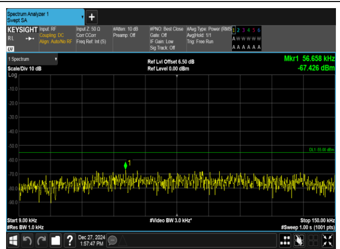
Band7-20MHz-QPSK-21100-1RB#0-0.009~0.15-PASS
