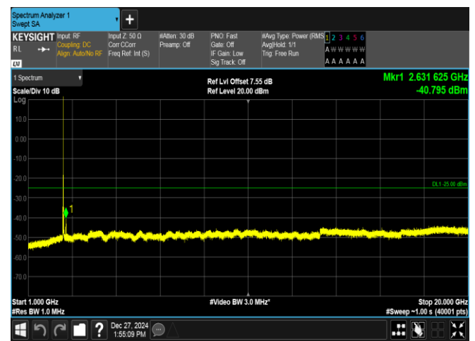
Band7-20MHz-16QAM-20850-1RB#99-1000~20000-PASS
