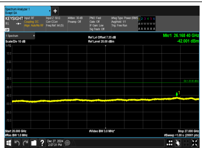
Band7-20MHz-QPSK-21350-1RB#99-20000~27000-PASS
