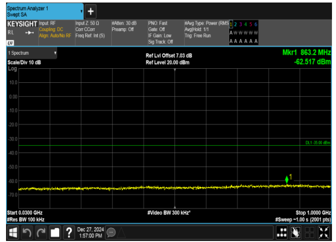
Band7-20MHz-16QAM-20850-100RB#0-30~1000-PASS
