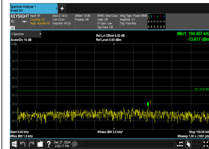
Band7-20MHz-16QAM-21100-100RB#0-0.009~0.15-PASS
