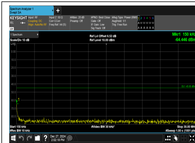
Band7-20MHz-QPSK-21100-100RB#0-0.15~30-PASS
