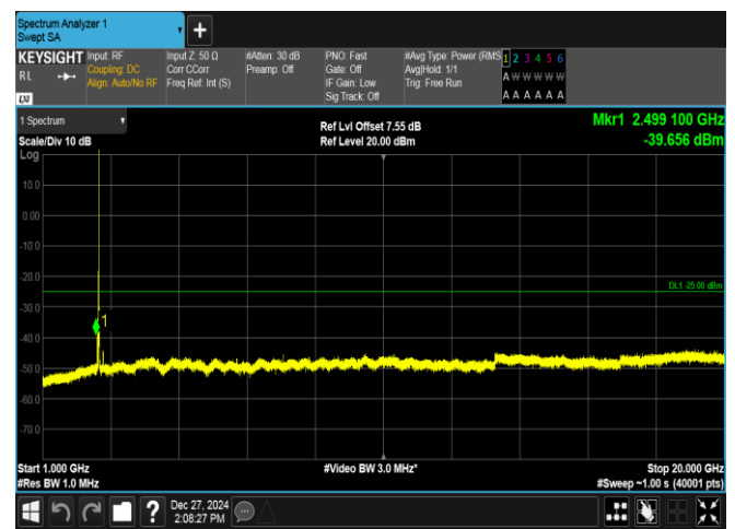
Band7-20MHz-16QAM-21350-1RB#99-1000~20000-PASS
