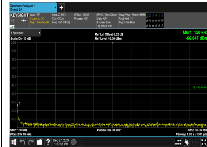
Band7-20MHz-QPSK-21100-1RB#0-0.15~30-PASS
