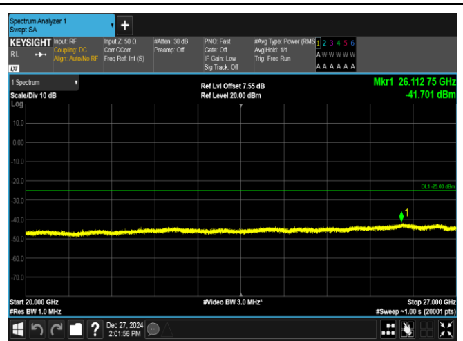
Band7-20MHz-16QAM-21100-1RB#99-20000~27000-PASS
