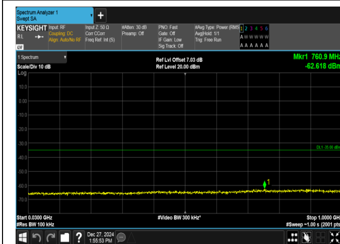
Band7-20MHz-QPSK-20850-100RB#0-30~1000-PASS
