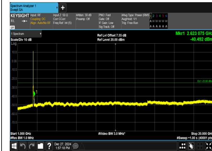
Band7-20MHz-16QAM-20850-100RB#0-1000~20000-PASS
