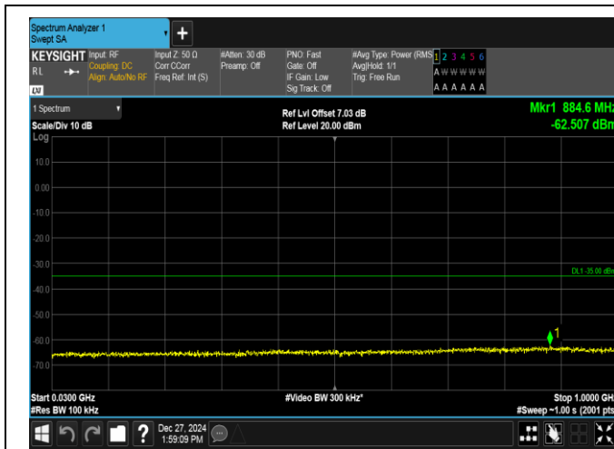
Band7-20MHz-16QAM-21100-1RB#0-30~1000-PASS
