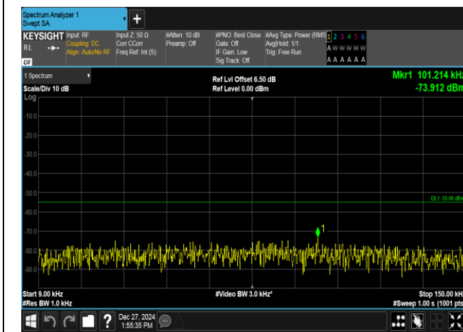
Band7-20MHz-QPSK-20850-100RB#0-0.009~0.15-PASS
