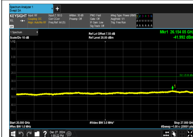
Band7-20MHz-16QAM-20850-1RB#99-20000~27000-PASS
