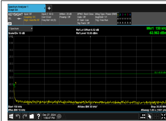
Band7-20MHz-16QAM-20850-100RB#0-0.15~30-PASS
