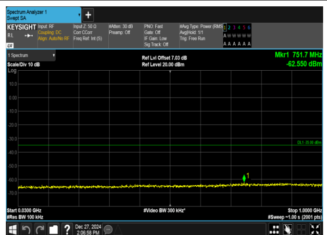
Band7-20MHz-QPSK-21350-1RB#99-30~1000-PASS
