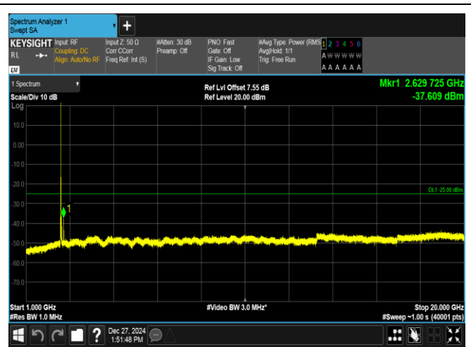
Band7-20MHz-QPSK-20850-1RB#0-1000~20000-PASS
