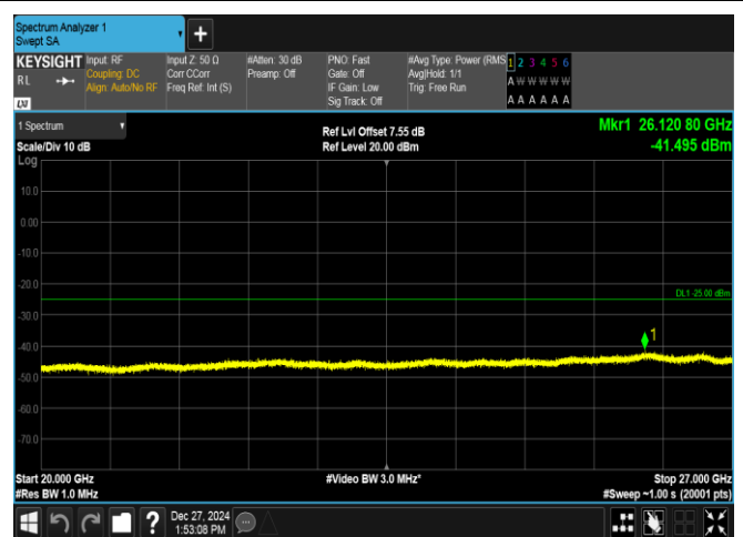
Band7-20MHz-16QAM-20850-1RB#0-20000~27000-PASS
