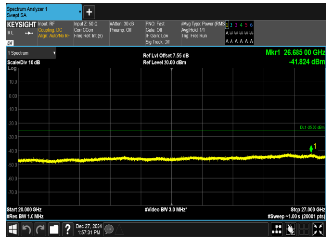
Band7-20MHz-16QAM-20850-100RB#0-20000~27000-PASS
