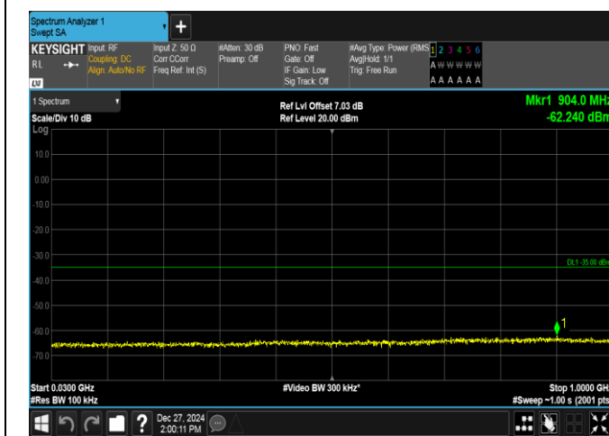
Band7-20MHz-QPSK-21100-1RB#99-30~1000-PASS
