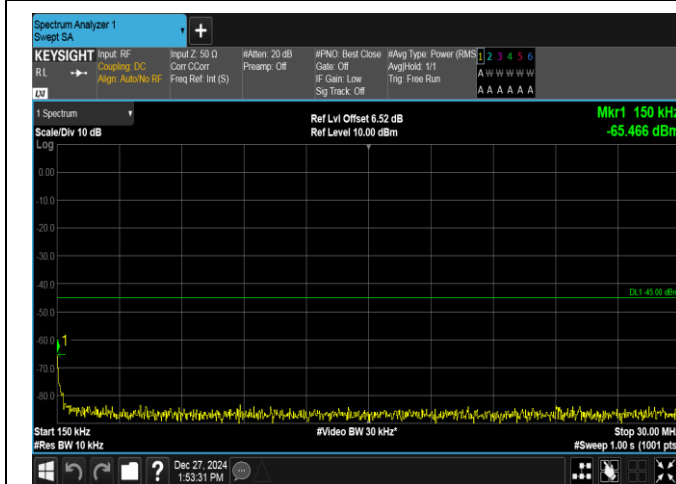
Band7-20MHz-QPSK-20850-1RB#99-0.15~30-PASS
