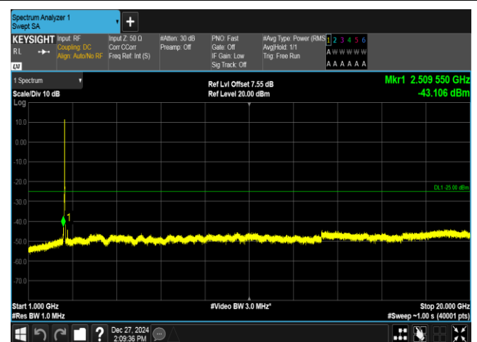
Band7-20MHz-QPSK-21350-100RB#0-1000~20000-PASS
