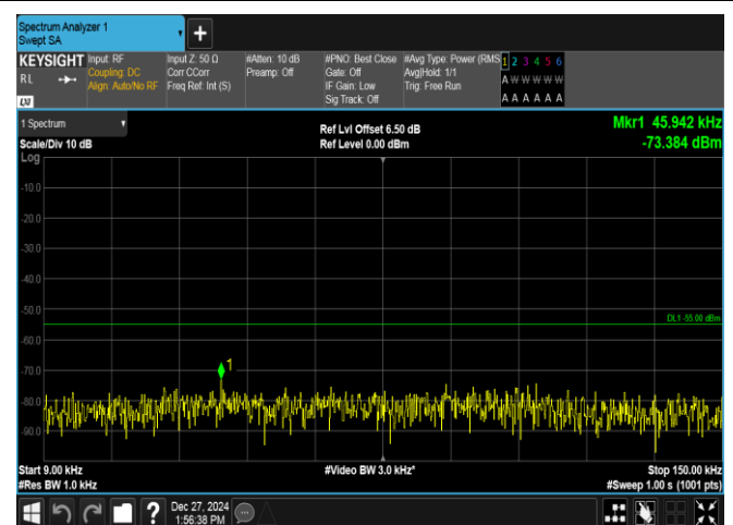
Band7-20MHz-16QAM-20850-100RB#0-0.009~0.15-PASS
