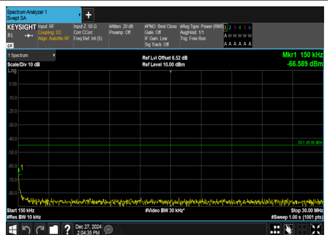
Band7-20MHz-QPSK-21350-1RB#0-0.15~30-PASS
