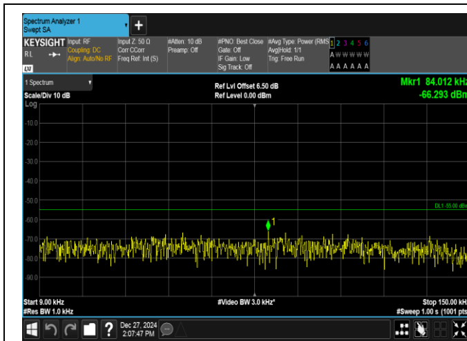
Band7-20MHz-16QAM-21350-1RB#99-0.009~0.15-PASS
