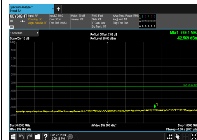
Band7-20MHz-QPSK-21350-100RB#0-30~1000-PASS
