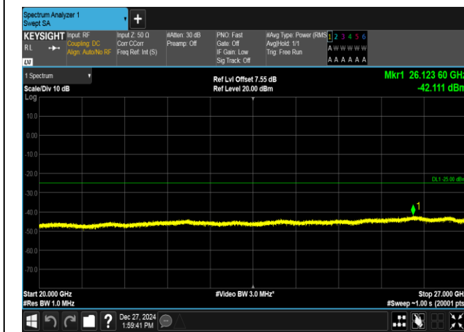
Band7-20MHz-16QAM-21100-1RB#0-20000~27000-PASS
