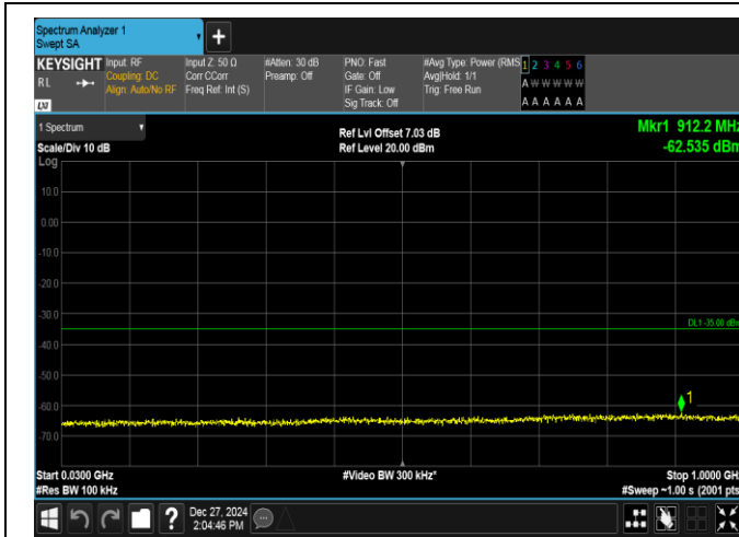
Band7-20MHz-QPSK-21350-1RB#0-30~1000-PASS
