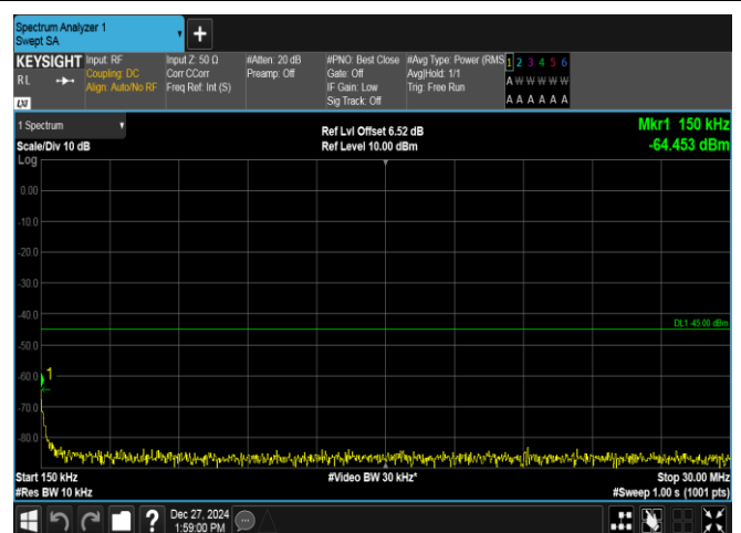
Band7-20MHz-16QAM-21100-1RB#0-0.15~30-PASS
