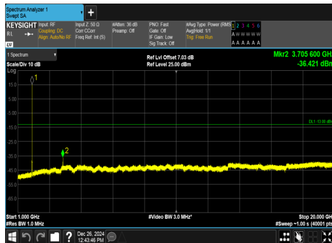
Band2-9262-2-1000~20000MHz-PASS
