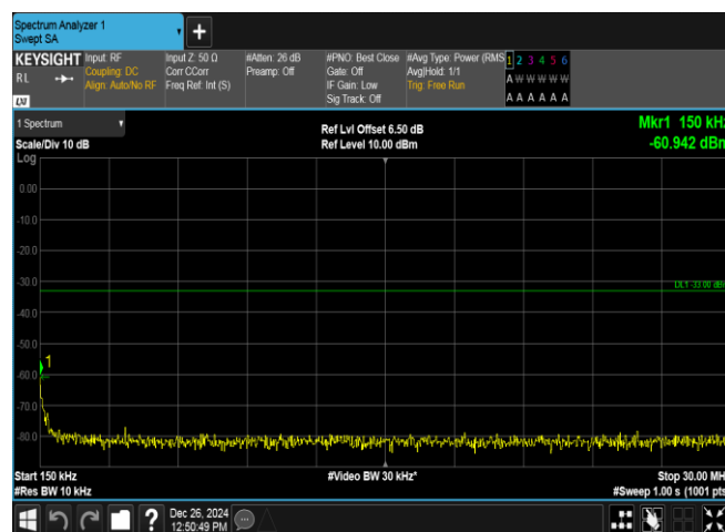
Band2-9262-5-0.15~30MHz-PASS
