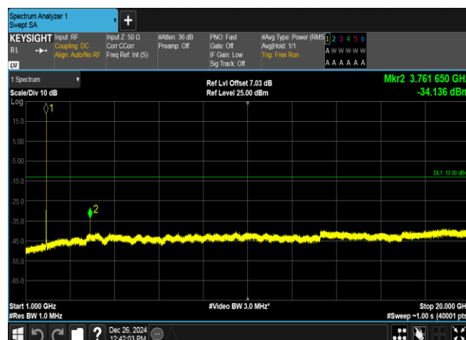
Band2-9400-1-1000~20000MHz-PASS
