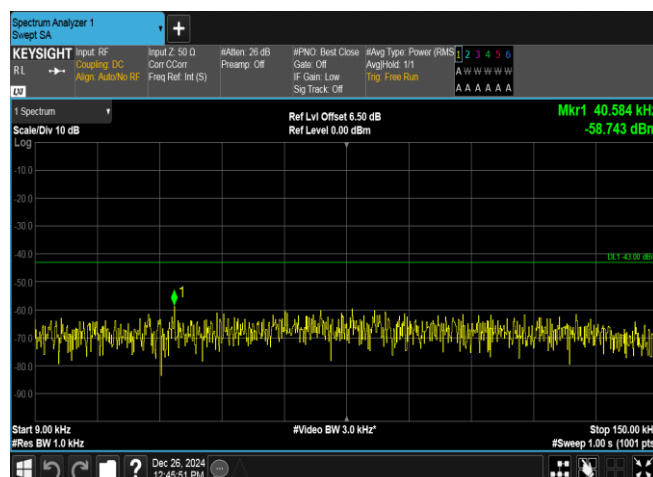
Band2-9262-3-0.009~0.15MHz-PASS
