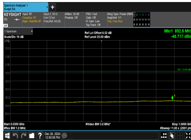
Band2-9262-5-30~1000MHz-PASS
