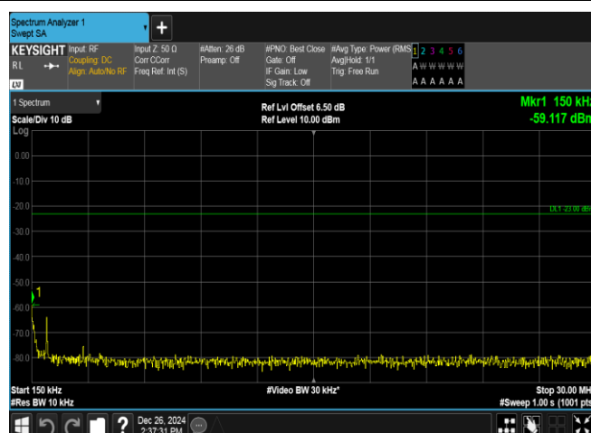
Band5-4132-2-0.15~30MHz-PASS
