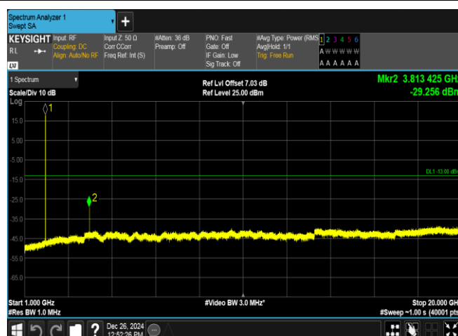
Band2-9538-5-1000~20000MHz-PASS
