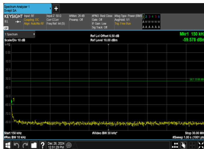
Band2-9400-5-0.15~30MHz-PASS
