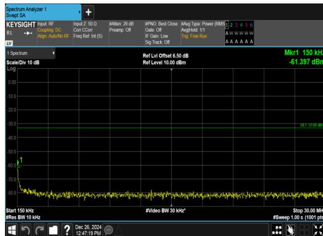
Band2-9538-3-0.15~30MHz-PASS
