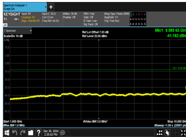
Band5-4132-1-1000~10000MHz-PASS
