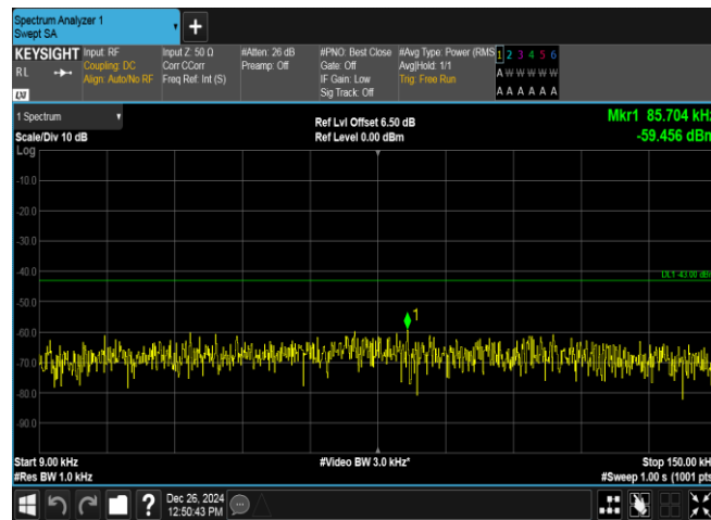
Band2-9262-5-0.009~0.15MHz-PASS
