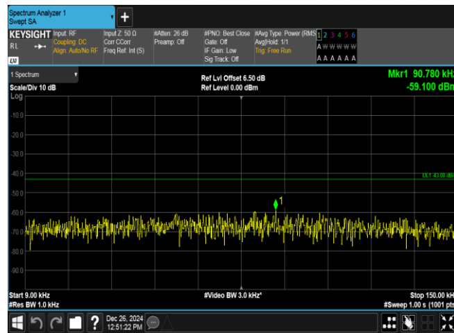
Band2-9400-5-0.009~0.15MHz-PASS
