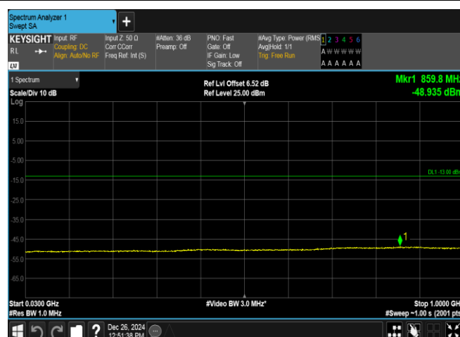
Band2-9400-5-30~1000MHz-PASS
