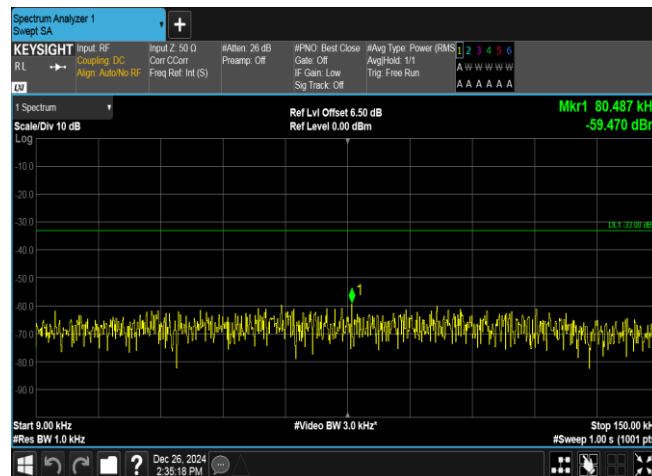
Band5-4132-1-0.009~0.15MHz-PASS
