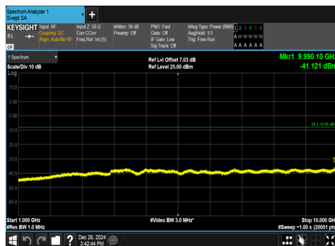
Band5-4132-3-1000~10000MHz-PASS
