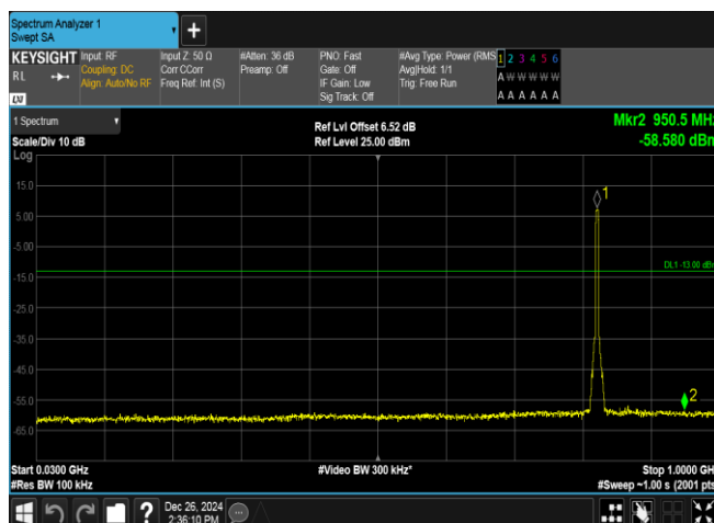
Band5-4182-1-30~1000MHz-PASS
