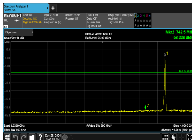
Band5-4233-2-30~1000MHz-PASS
