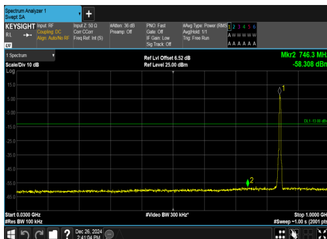
Band5-4233-3-30~1000MHz-PASS
