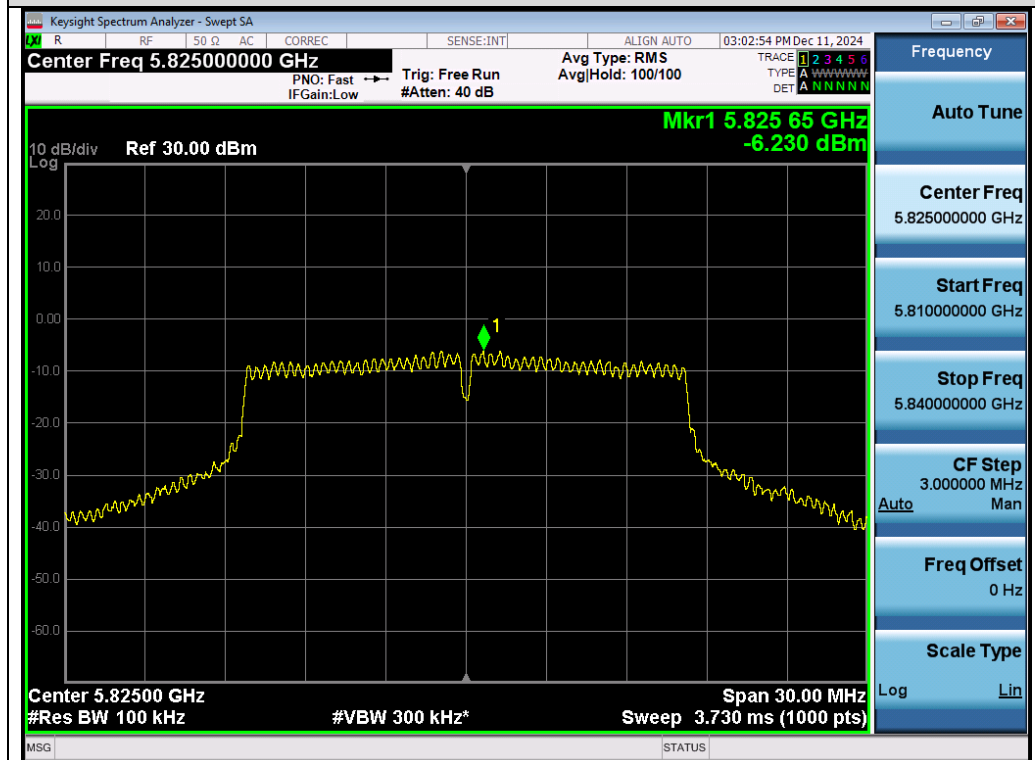
Test_Graph_802.11a_ANT1_5825_6Mbps_PSD
