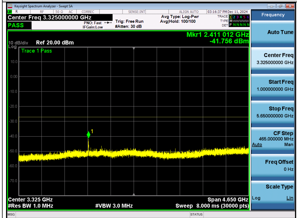
Test_Graph_802.11ac80_ANT1_5775_MCS0_Frequency Band2
