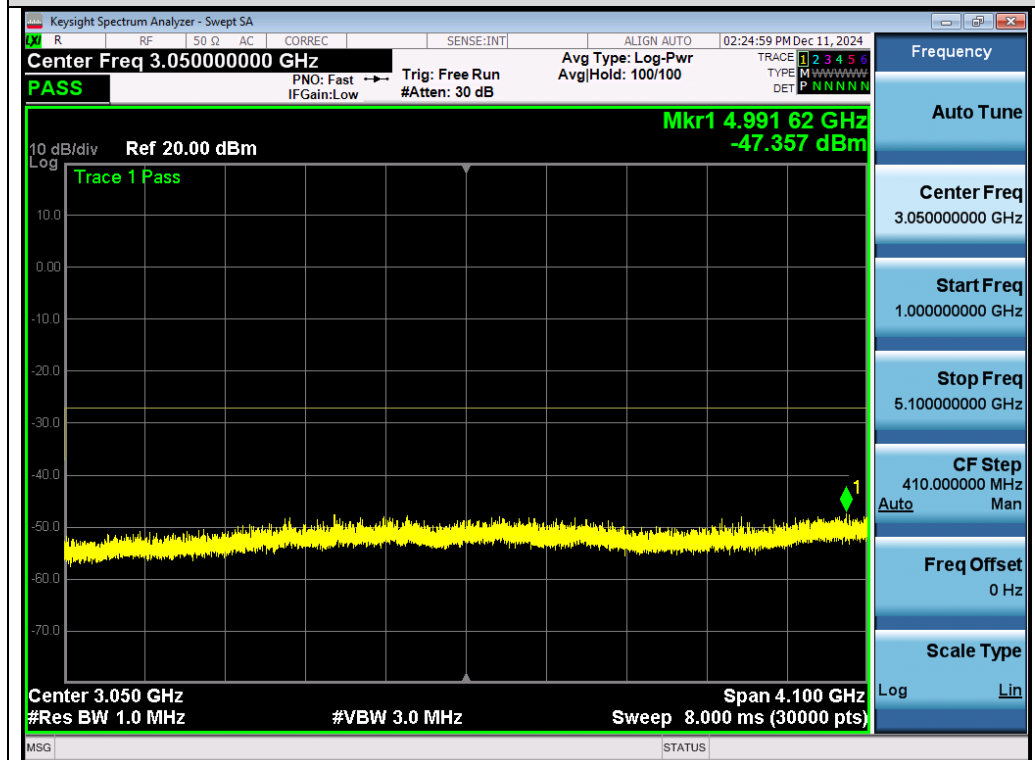
Test_Graph_802.11ac80_ANT1_5290_MCS0_Frequency Band 2
