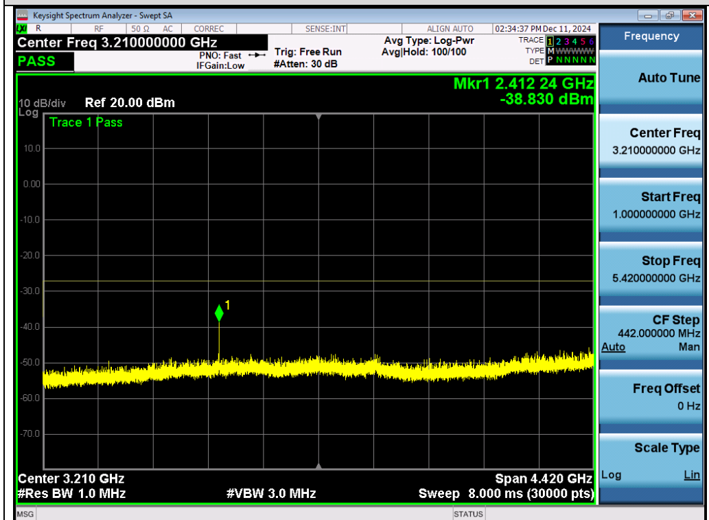
Test_Graph_802.11a_ANT1_5500_6Mbps_Frequency Band 2
