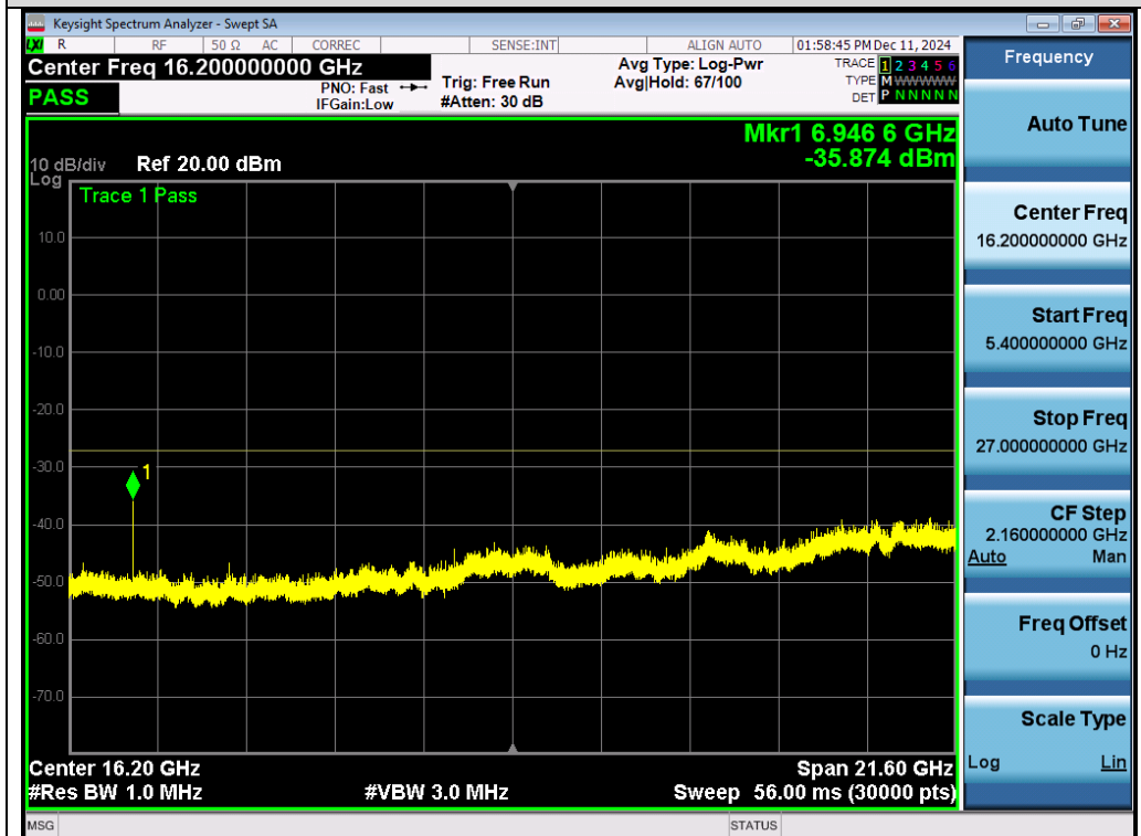
Test_Graph_802.11ac80_ANT1_5210_MCS0_Frequency Band 4
