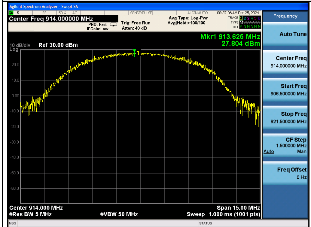
Test_Graph_802.11ah_ANT1_914.0_BW 4MHz_Peak Power
