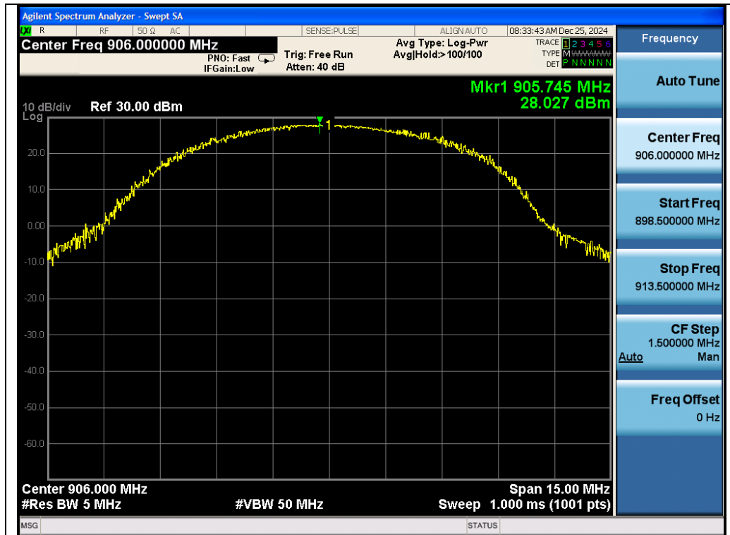
Test_Graph_802.11ah_ANT1_906.0_BW 4MHz_Peak Power
